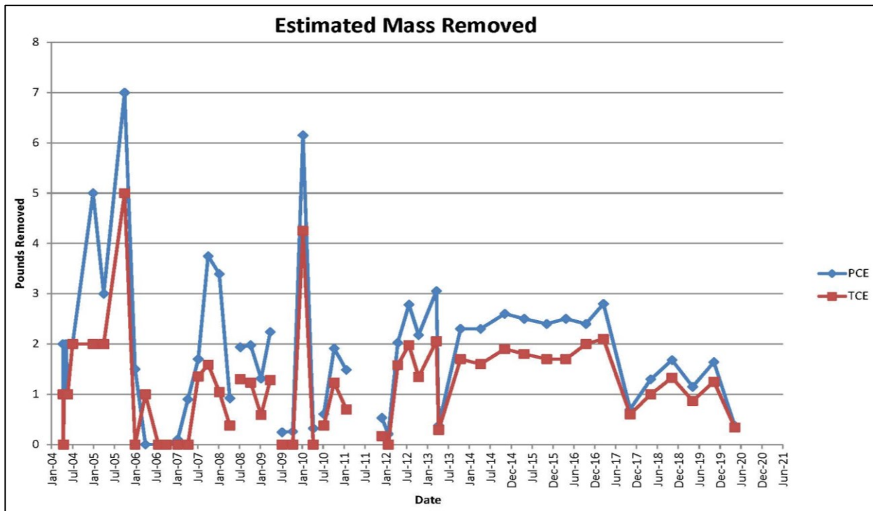
Figure A5. ARP SVE Wells Performance Monitoring – Estimated Mass Removed
