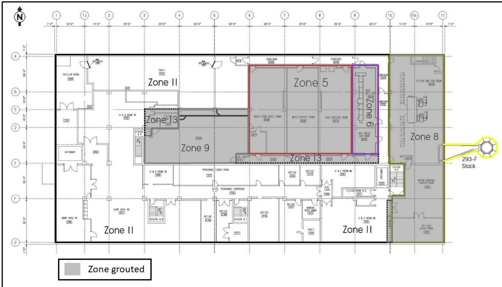
Figure 15. Alternative A-2. ISD First and Second Level Process Areas /Engineered Roof (Second Level View)
