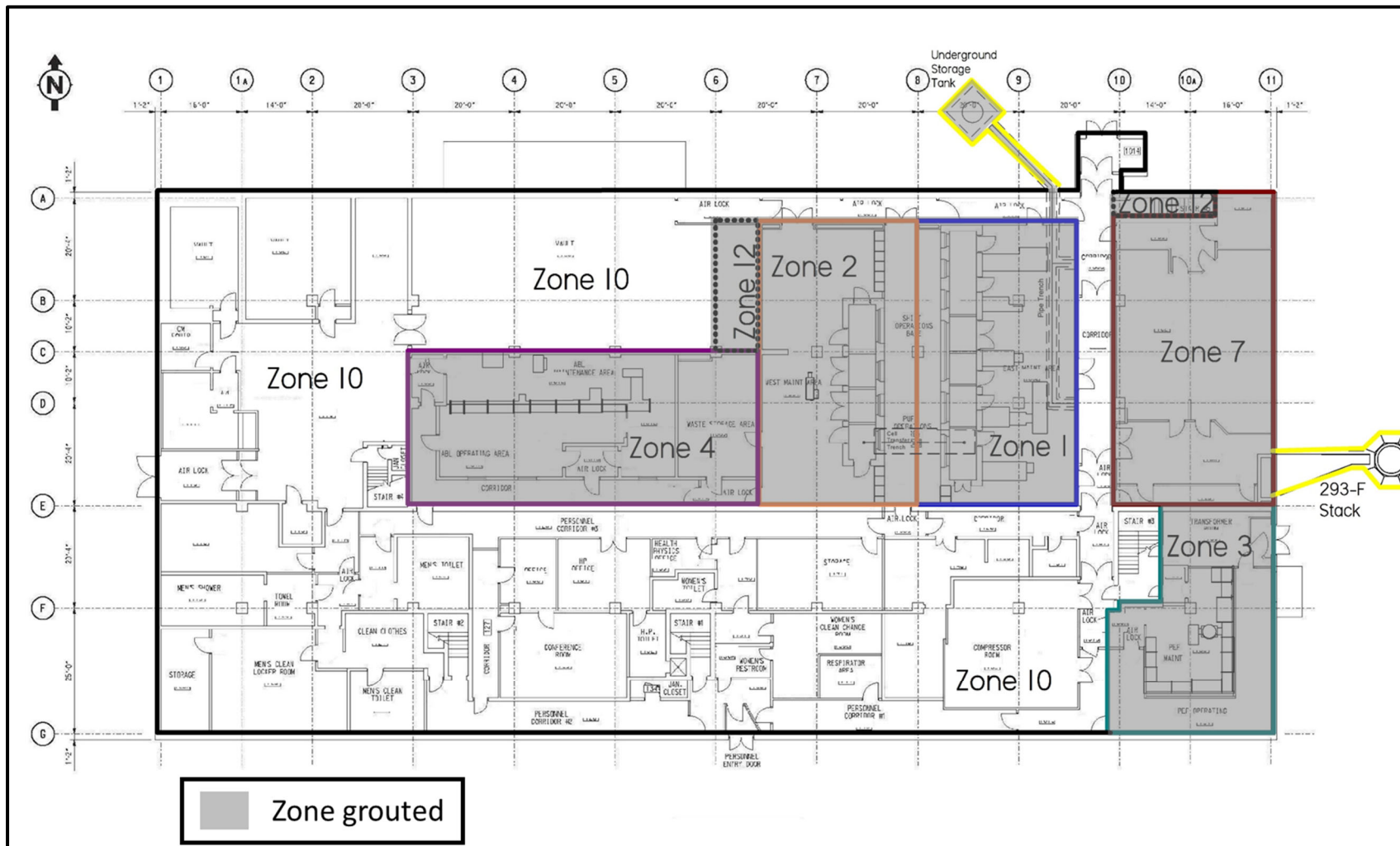
Figure 14. Alternative A-2. ISD First and Second Level Process Areas /Engineered Roof (First Level View)
