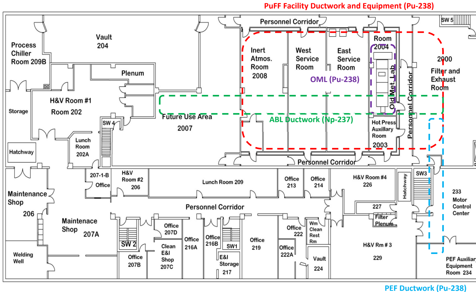
Figure 7. Layout of Building 235-F Second Level
