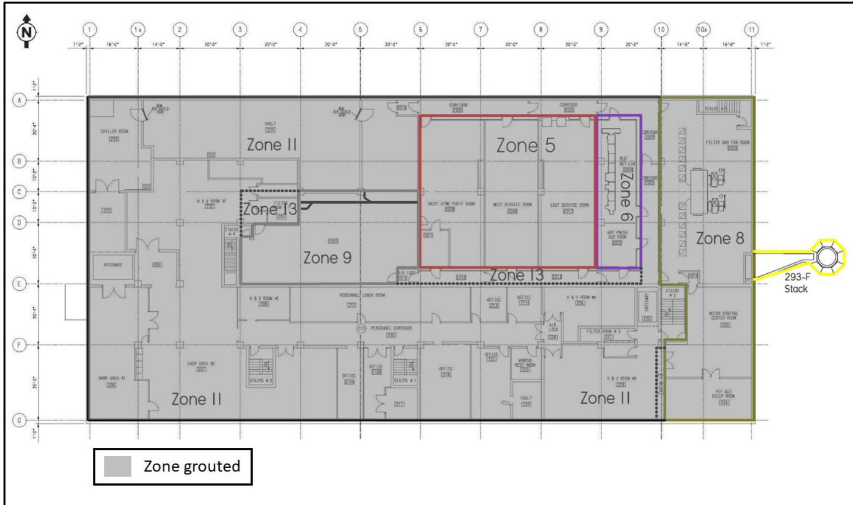
Figure 17. Alternative A-3. ISD Entire Building 235-F/Engineered Roof (Second Level View)
