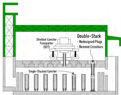
Figure 4-2—Double Stacking
