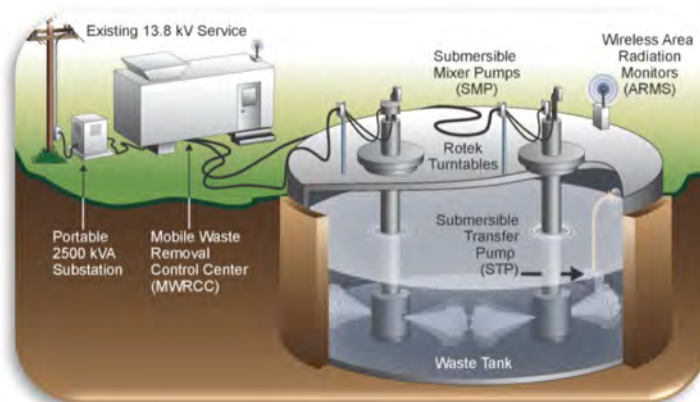
Figure 4-4—Temporary Waste Removal
