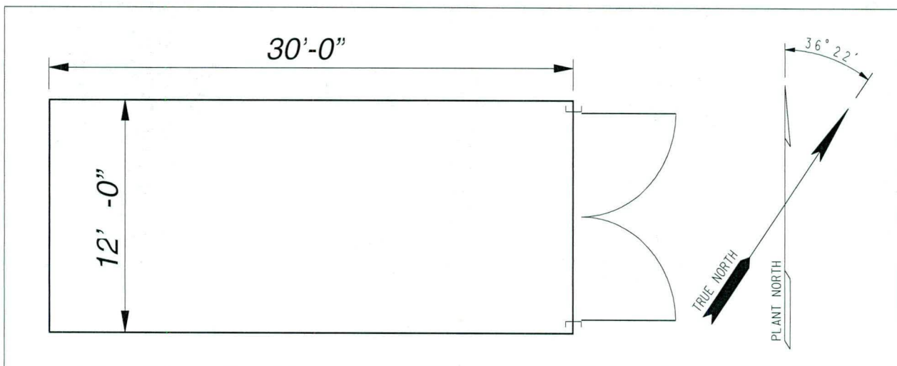
Figure 2. Building 484-5D, Storage Building (Layout)
