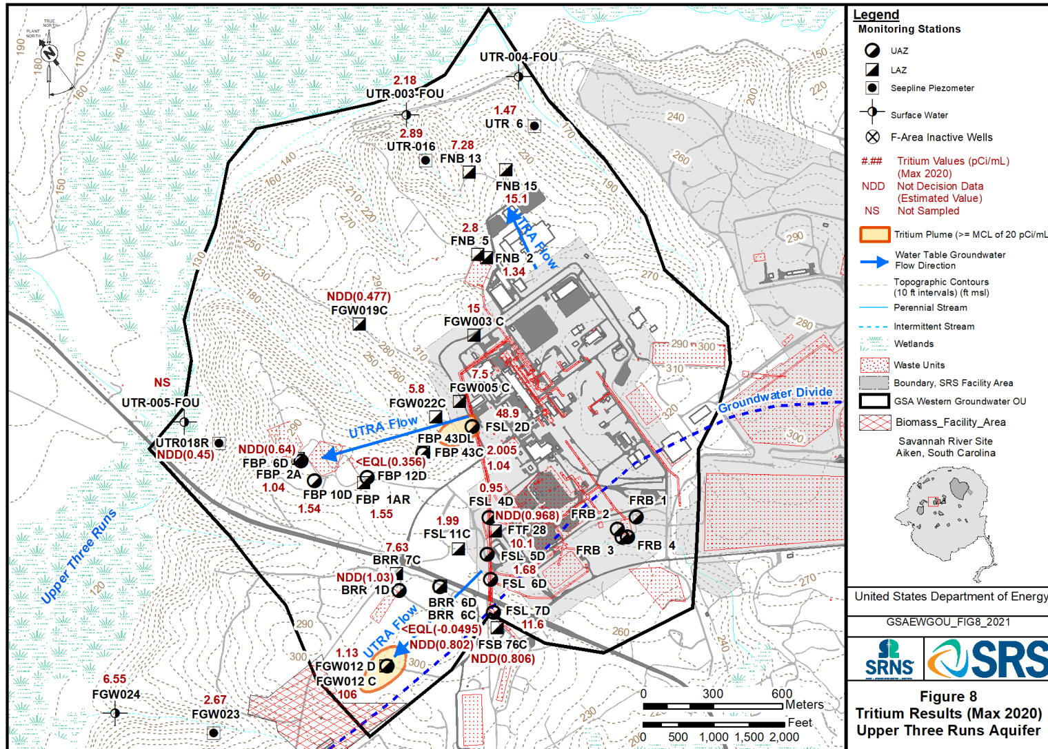
Figure 8. Tritium Results (Max 2020) Upper Three Runs Aquifer
