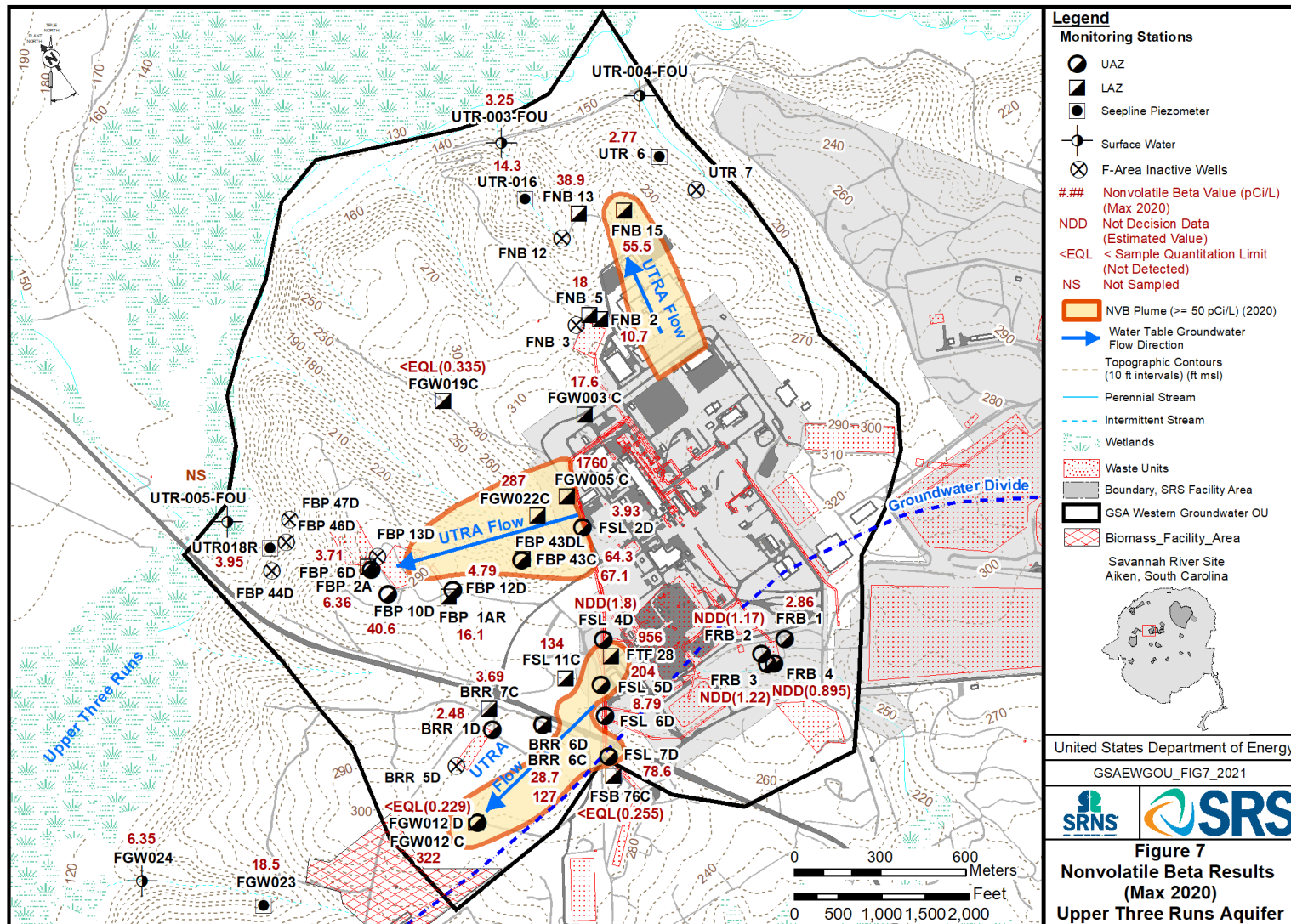
Figure 7. Nonvolatile Beta Results (Max 2020) Upper Three Runs Aquifer
