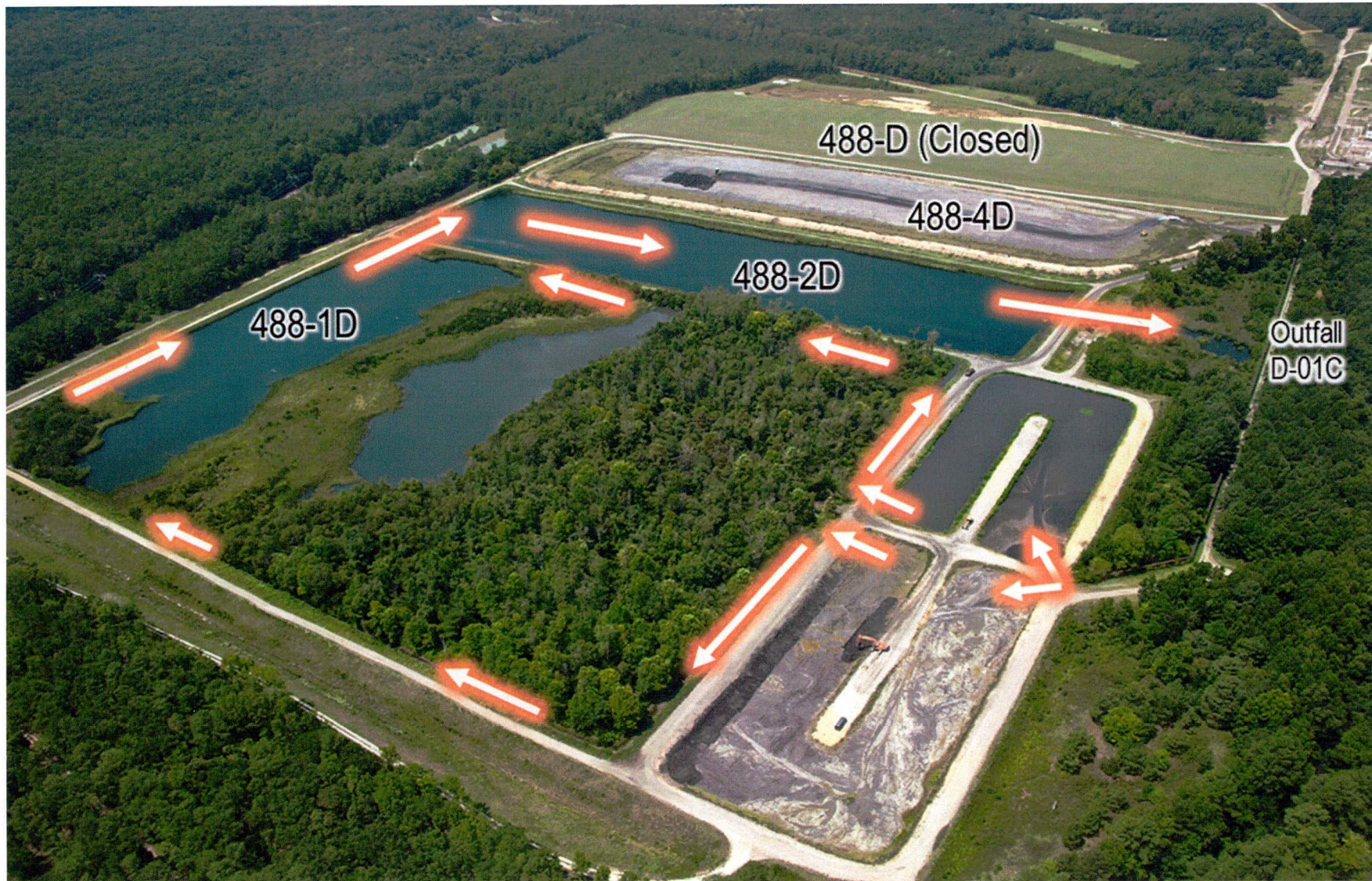
Figure 4. D-Area Ash Basins Waste Water Flow Pattern During Operations
