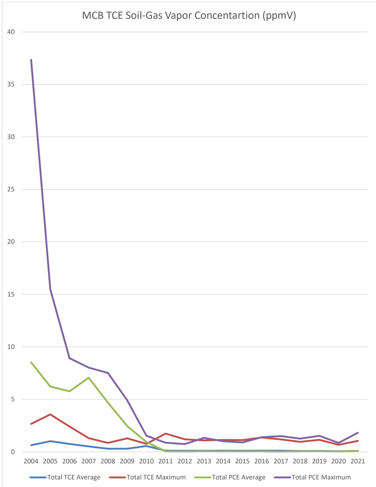
Figure 6. MCB Soil-Gas Vapor Concentration Over Time Trend Diagram
