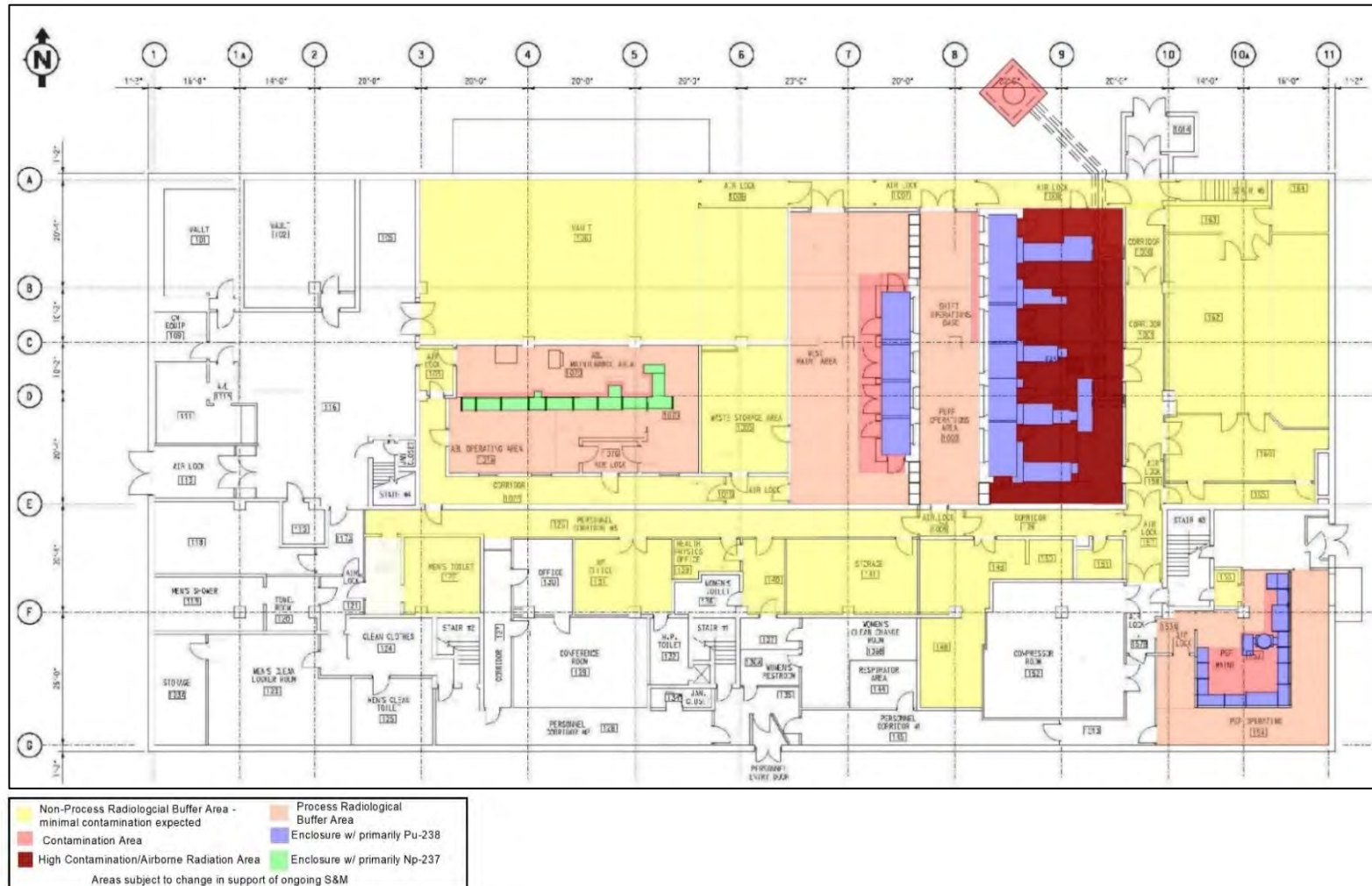
Figure 10. Building 235-F First Level Contamination (Radiological Holdup)
