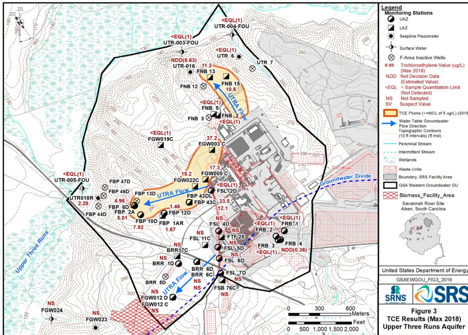
Figure 3. Trichloroethylene Results (Max 2018) Upper Three Runs Aquifer
