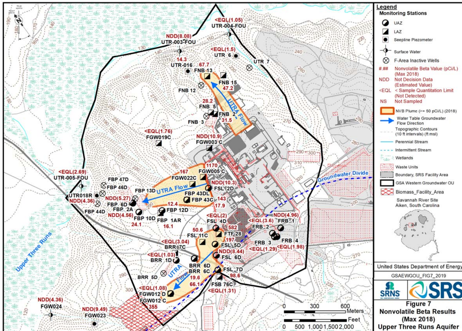
Figure 7. Nonvolatile Beta Results (Max 2018) Upper Three Runs Aquifer
