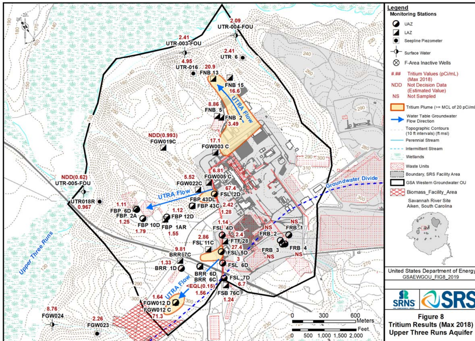
Figure 8. Tritium Results (Max 2018) Upper Three Runs Aquifer
