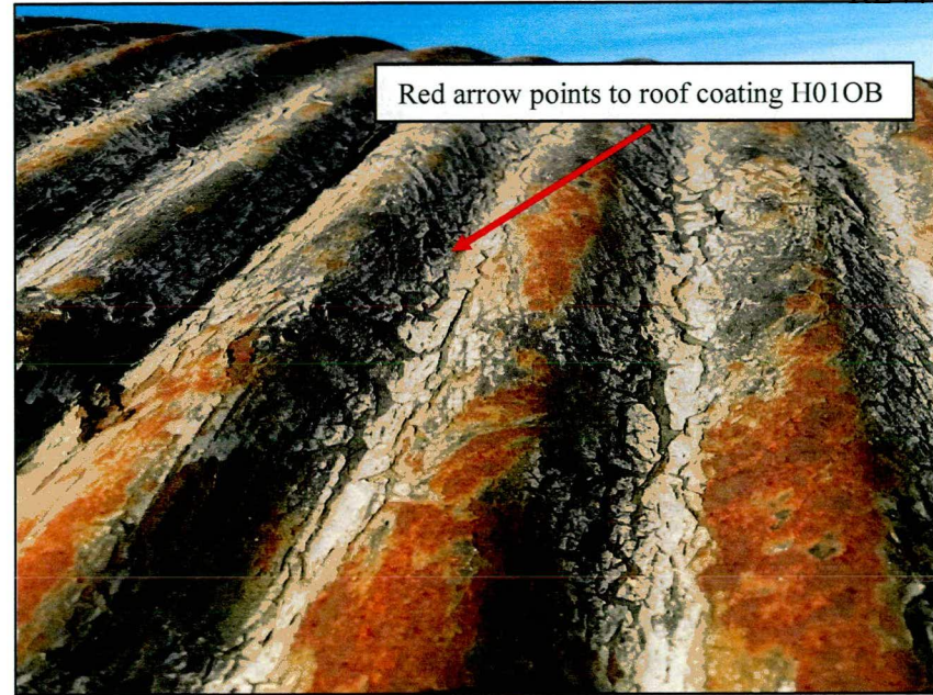
Photograph 1. Roof panel coating H01OB. Closeup view of roof panel.
