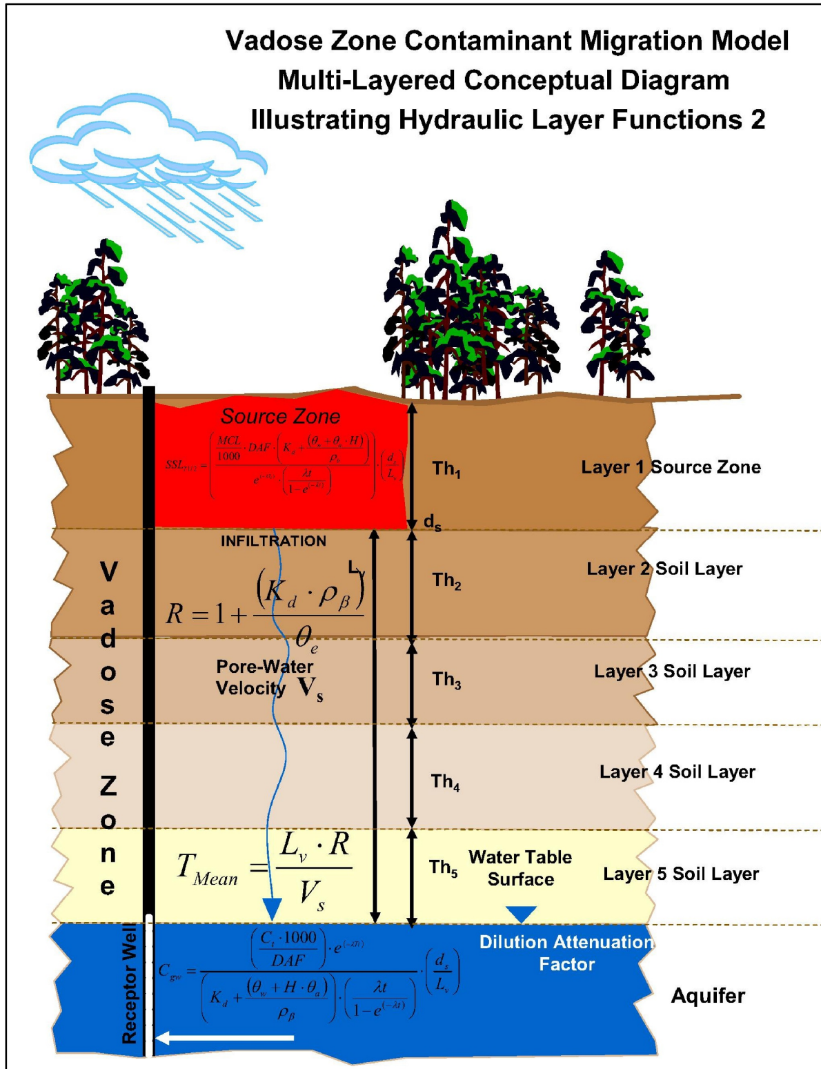
Figure 3-1. 5-layer VZCOMML model (Rucker 2011)
