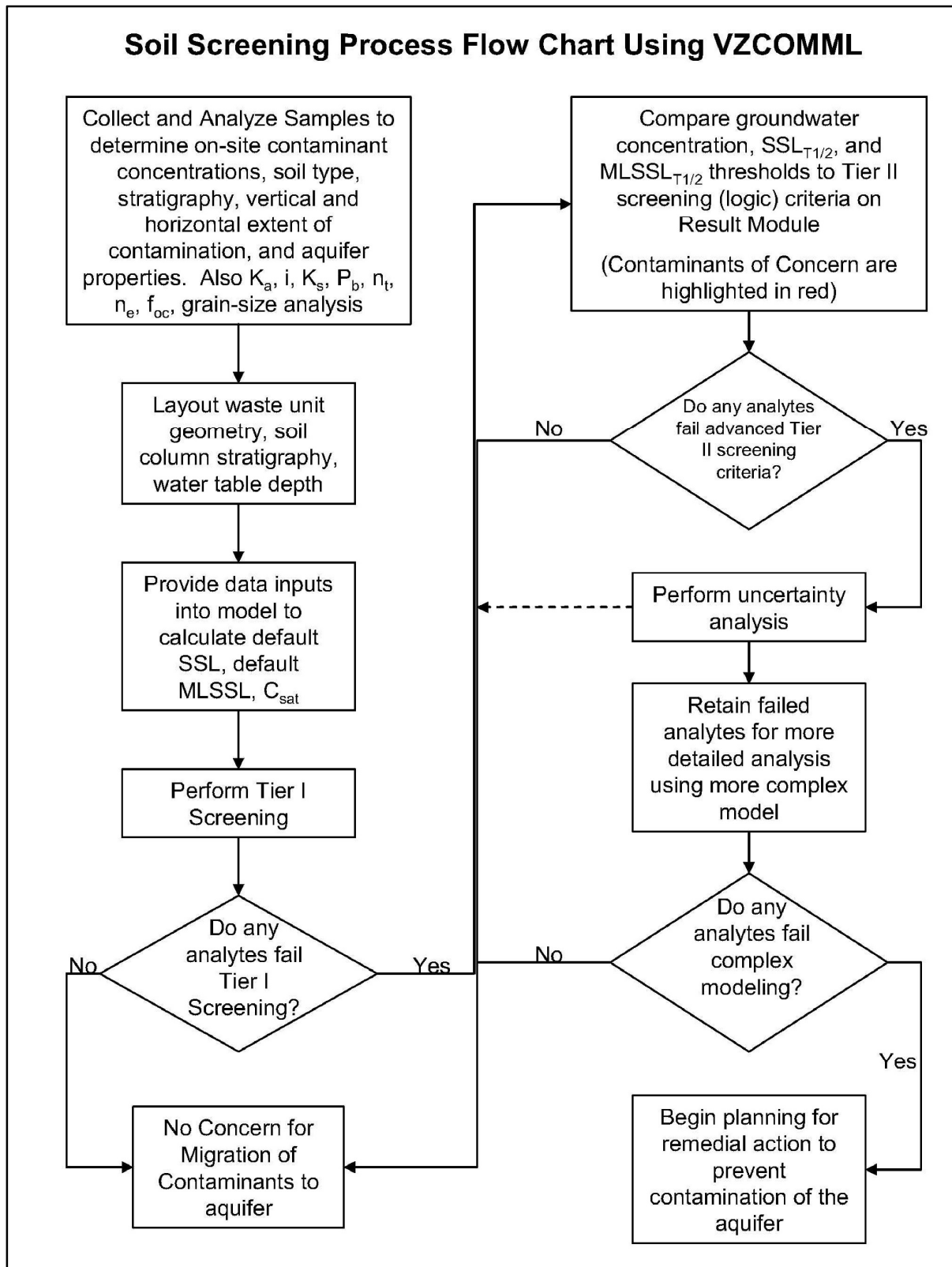
Figure 3-2. Flow Chart of Soil Screening Process (Rucker 2011)
