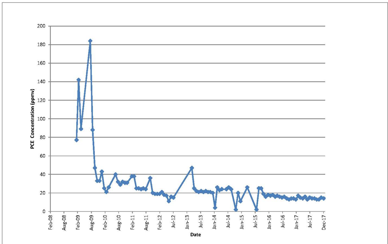
Figure 9. Graph Illustrating at MH-01 PCE Soil Gas Concentrations
