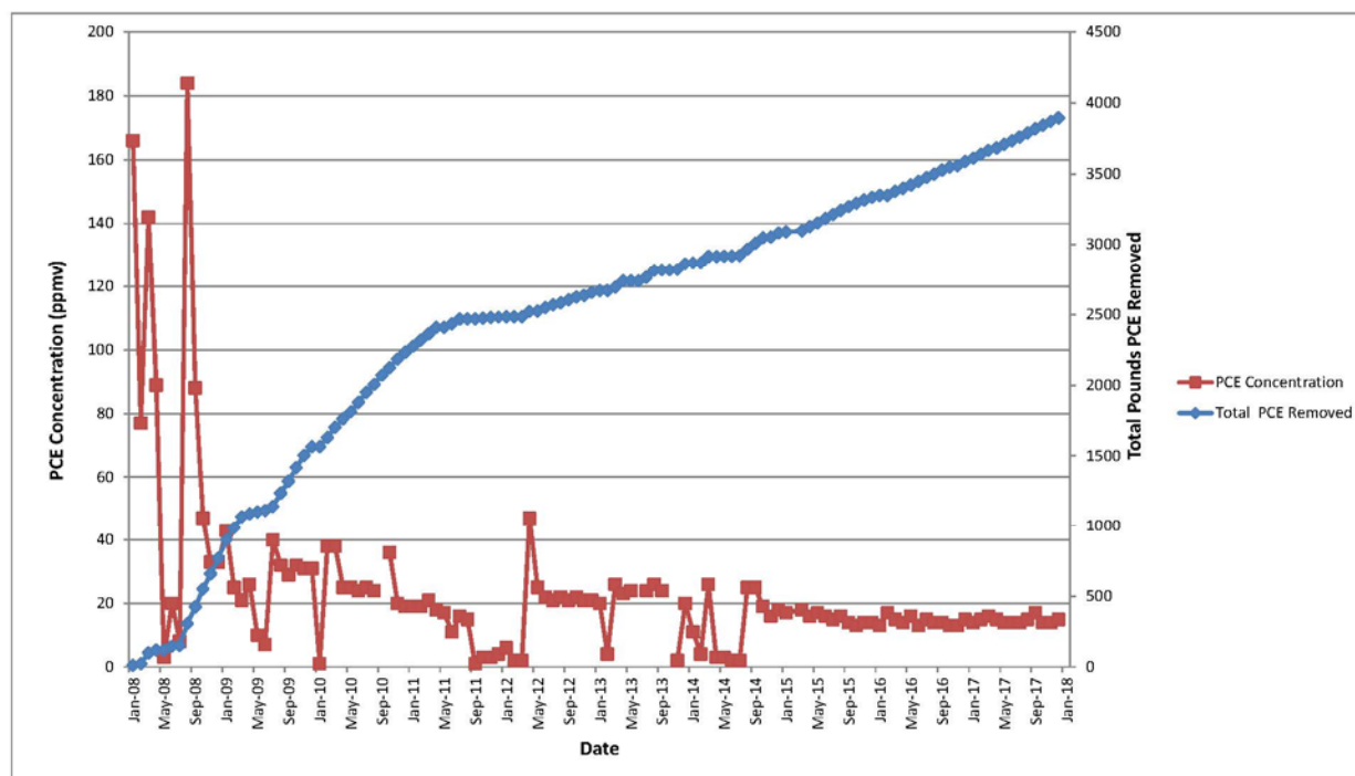
Figure 10. Process Graph Illustrating Asymptotic Curve with Mass Removal by ASVE
