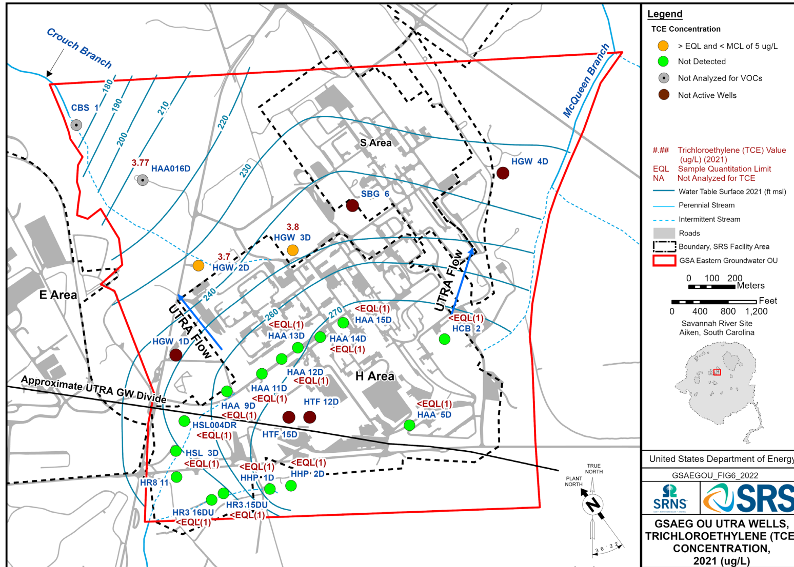
Figure 5. 2021 Upper Three Runs Aquifer TCE Concentration
