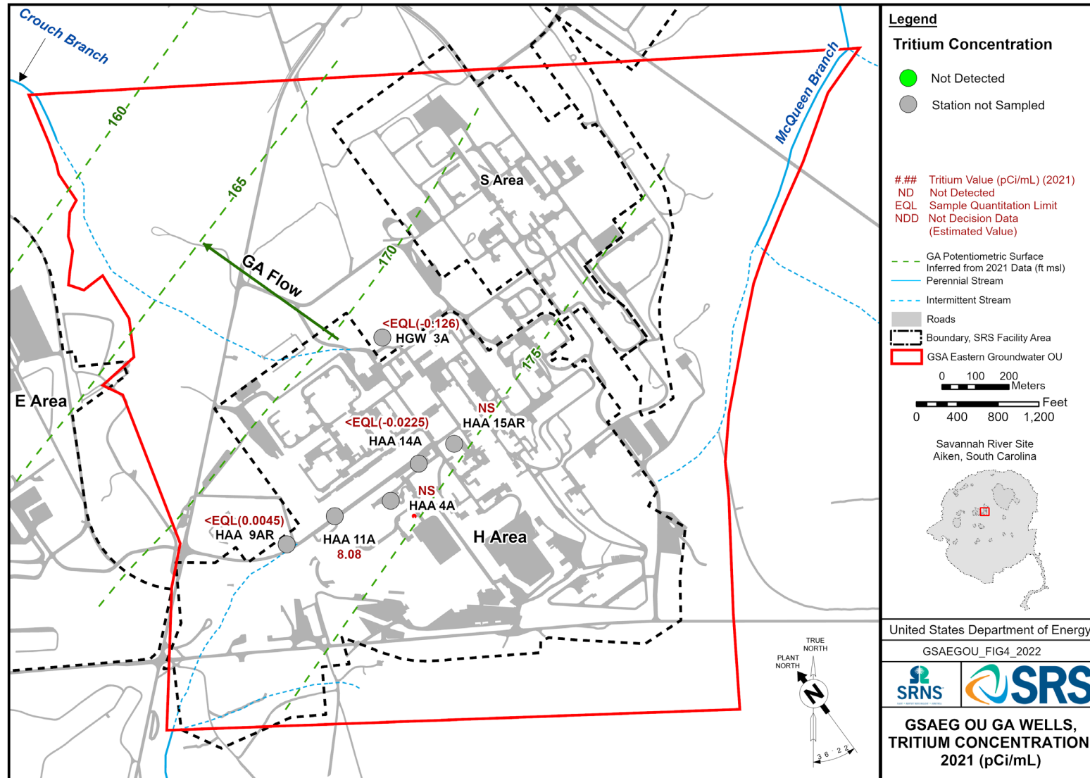
Figure 4. 2021 Gordon Aquifer Tritium Concentration
