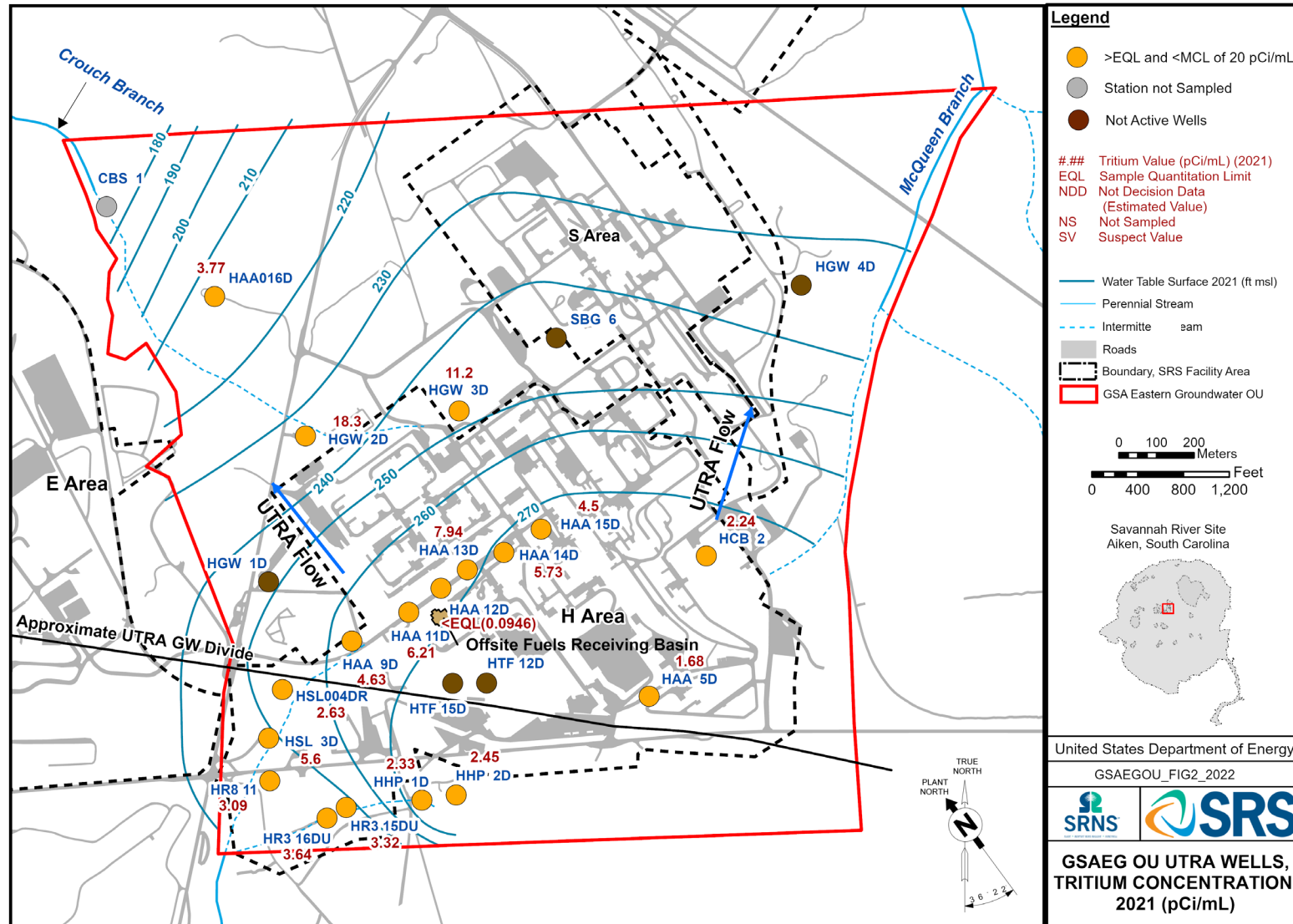
Figure 2. 2021 Upper Three Runs Aquifer Tritium Concentration
