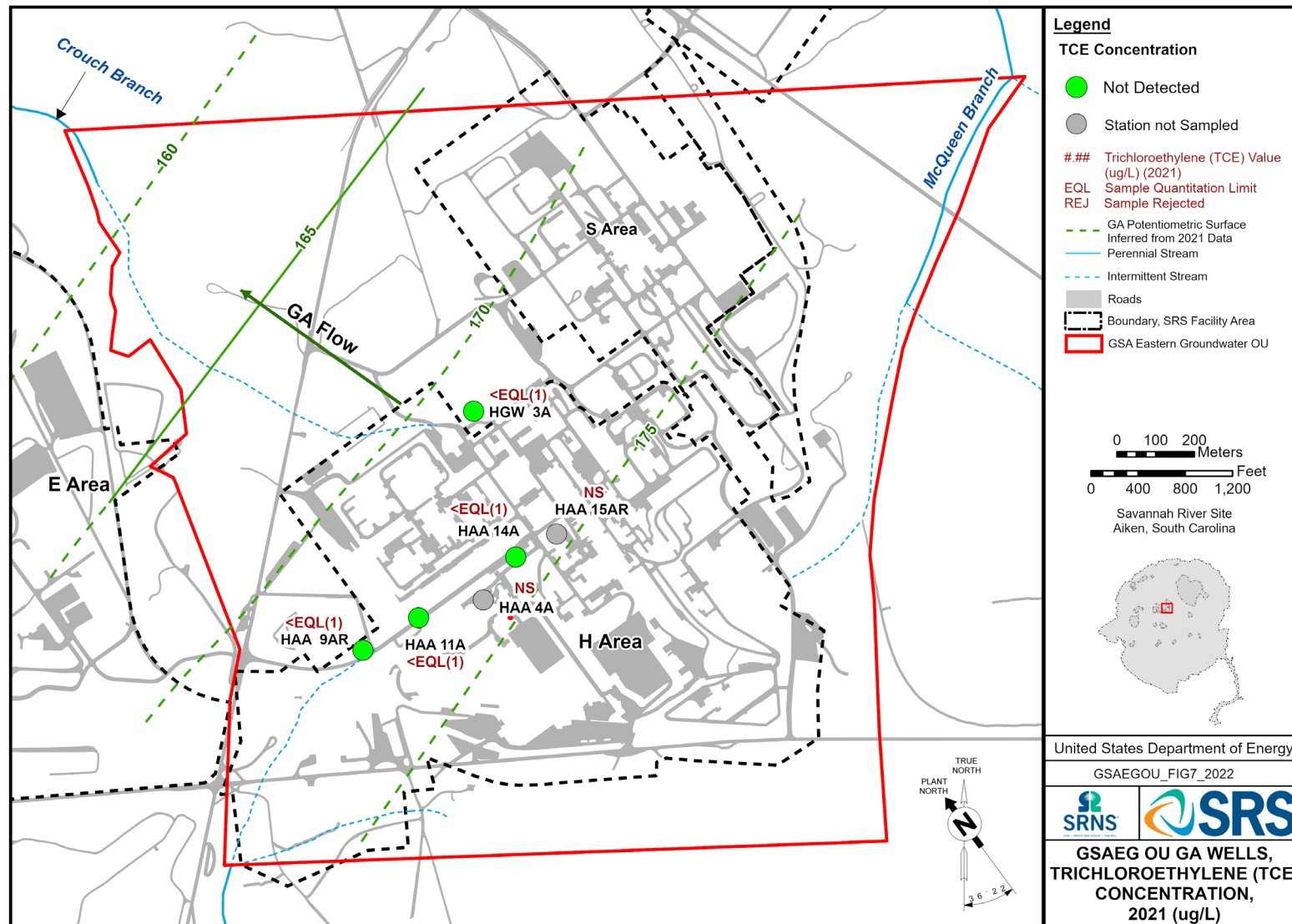
Figure 6. 2021 Gordon Aquifer TCE Concentration
