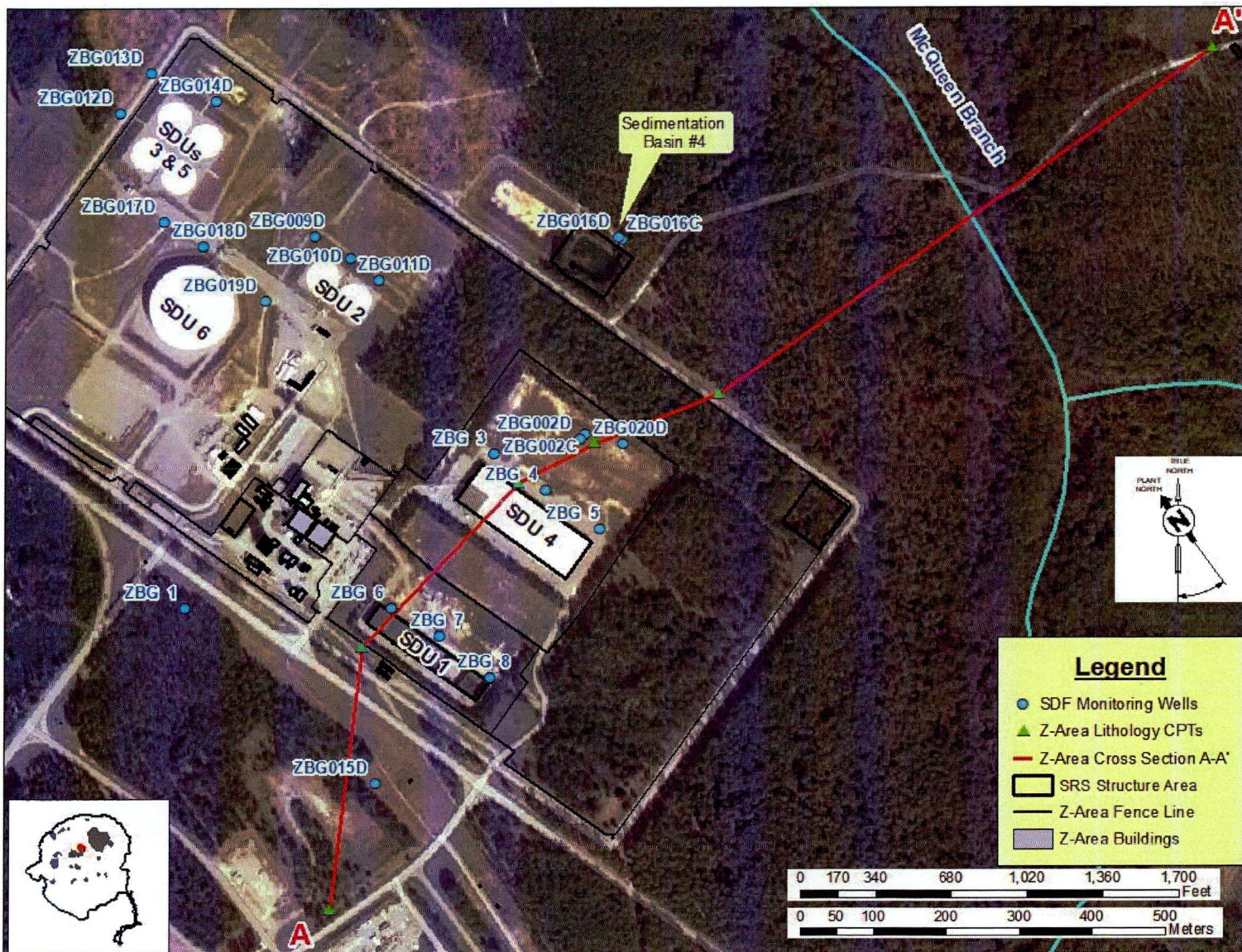
Figure 2. Monitoring Well Locations at the SDF
