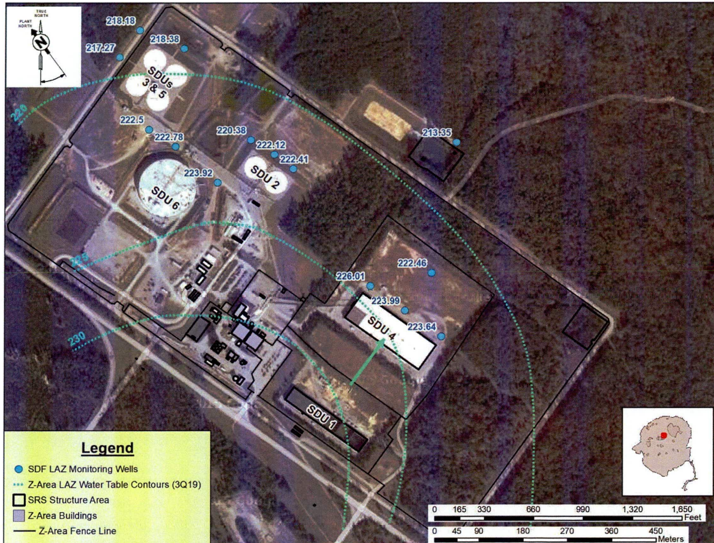
Figure 4. 3Q19 LAZ Water Table Elevations (ft-msl)
