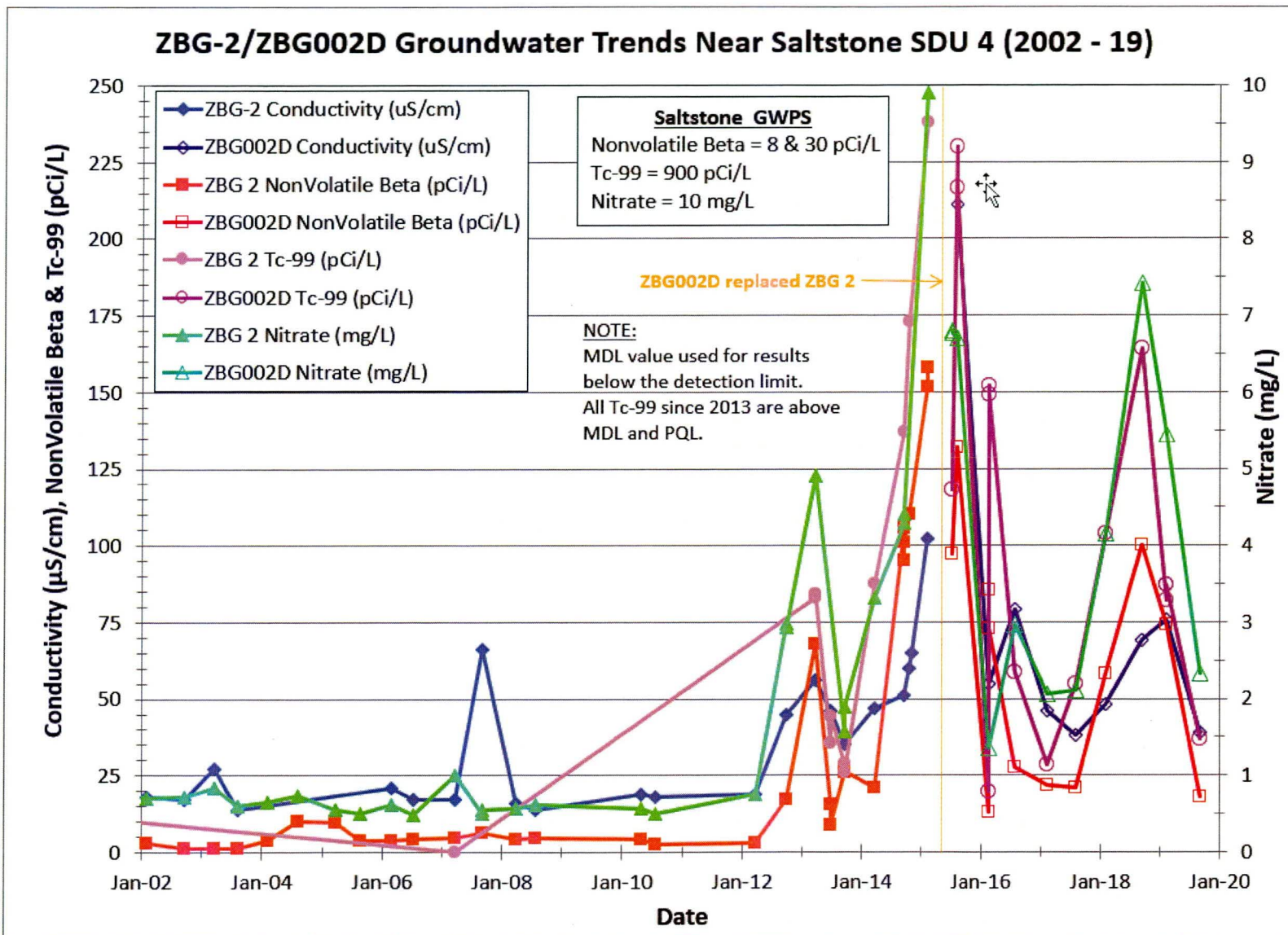
Figure 8. ZBG 2 / ZBG002D Tc-99 Groundwater Trends
