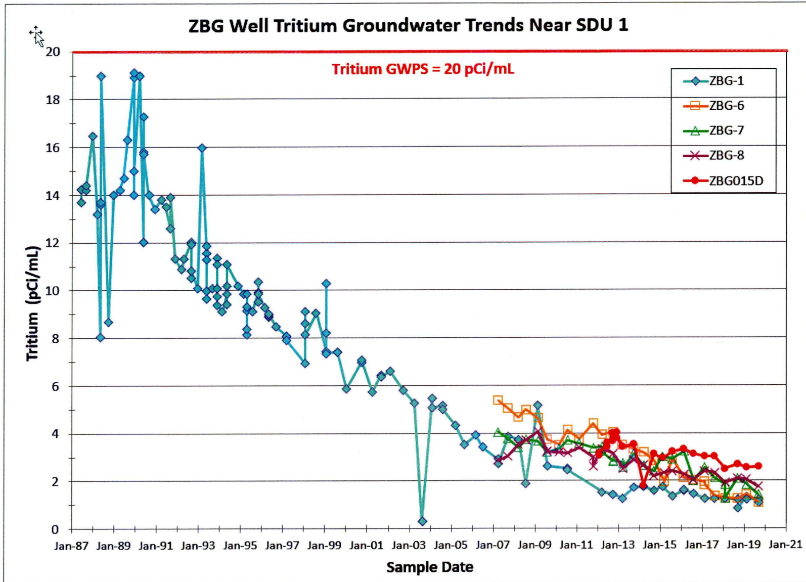
Figure 13. ZBG Well Tritium Groundwater Trends
