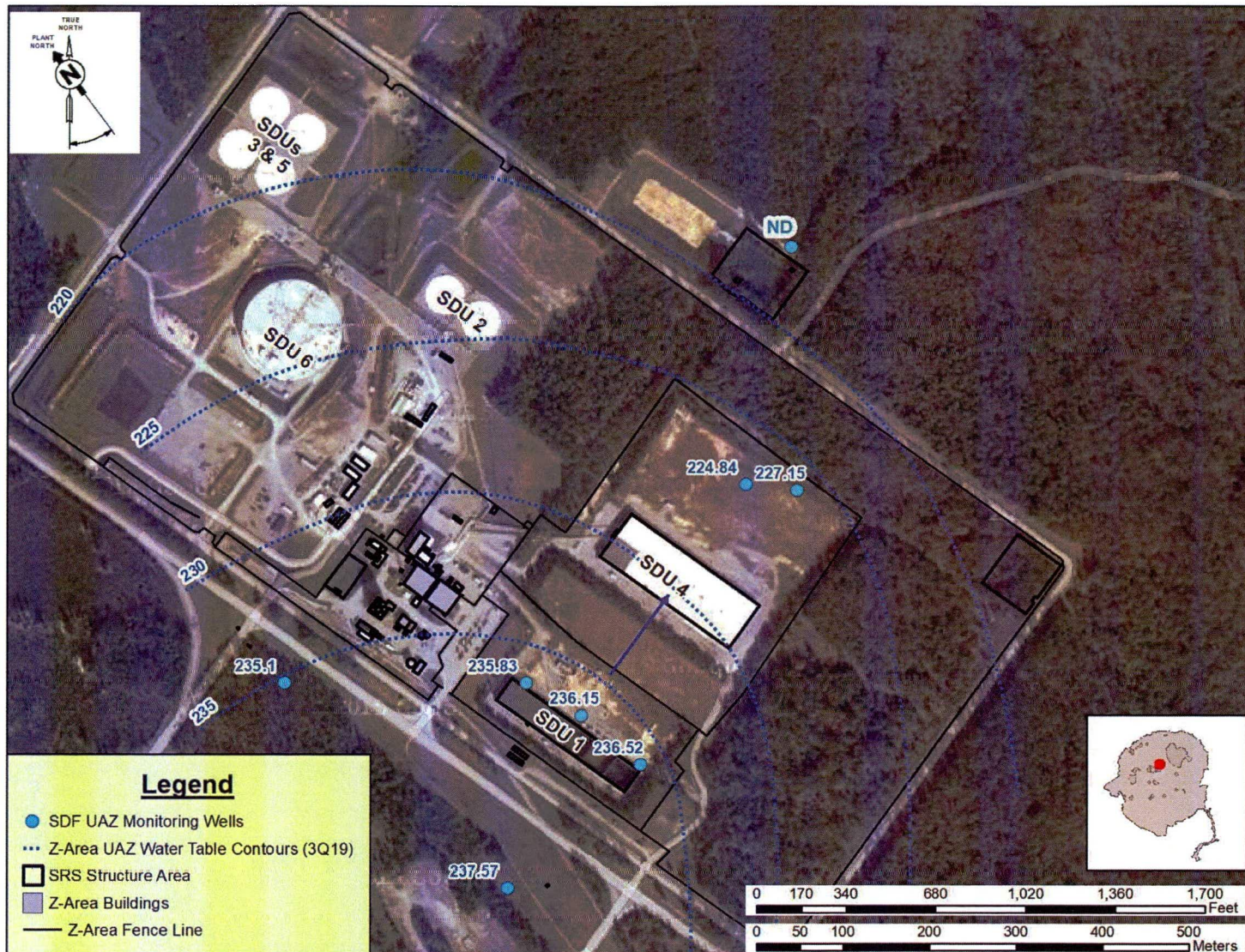
Figure 5. 3Q19 UAZ Water Table Elevations (ft-msl)
