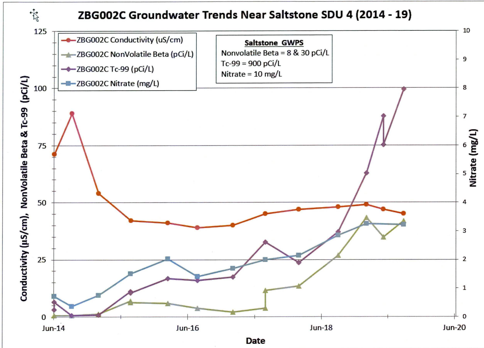
Figure 10. ZBG002C Groundwater Trends
