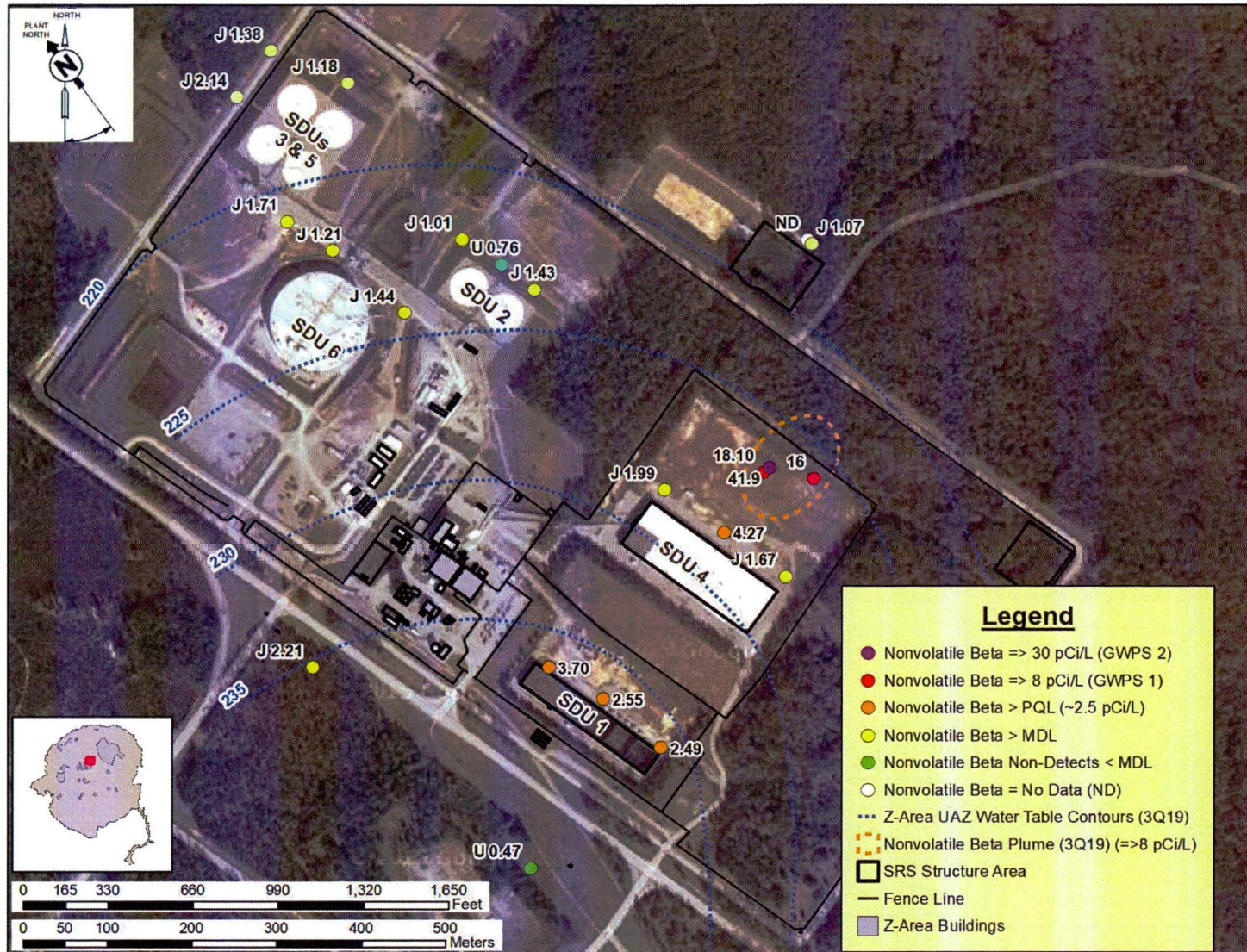
Figure 9. Approximate Nonvolatile Beta Groundwater Plume (3Q19)
