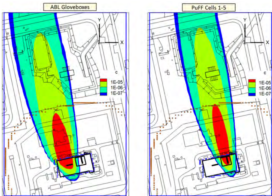
Figure B-8. PORFLOW-Based Steady-State Aquifer Tracer Plume Contours from Glovebox Source Terms Originating Within the ABL and Puff Facilities, Respectively
