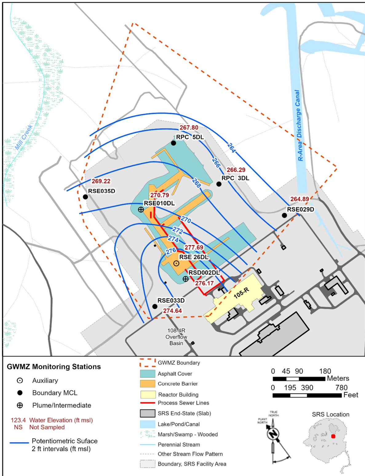
Figure B-6. Potentiometric Surface in the Transmissive Zone (1Q2022)
