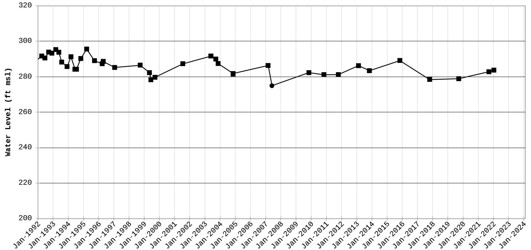
Hydrograph for Station RSE 1A
