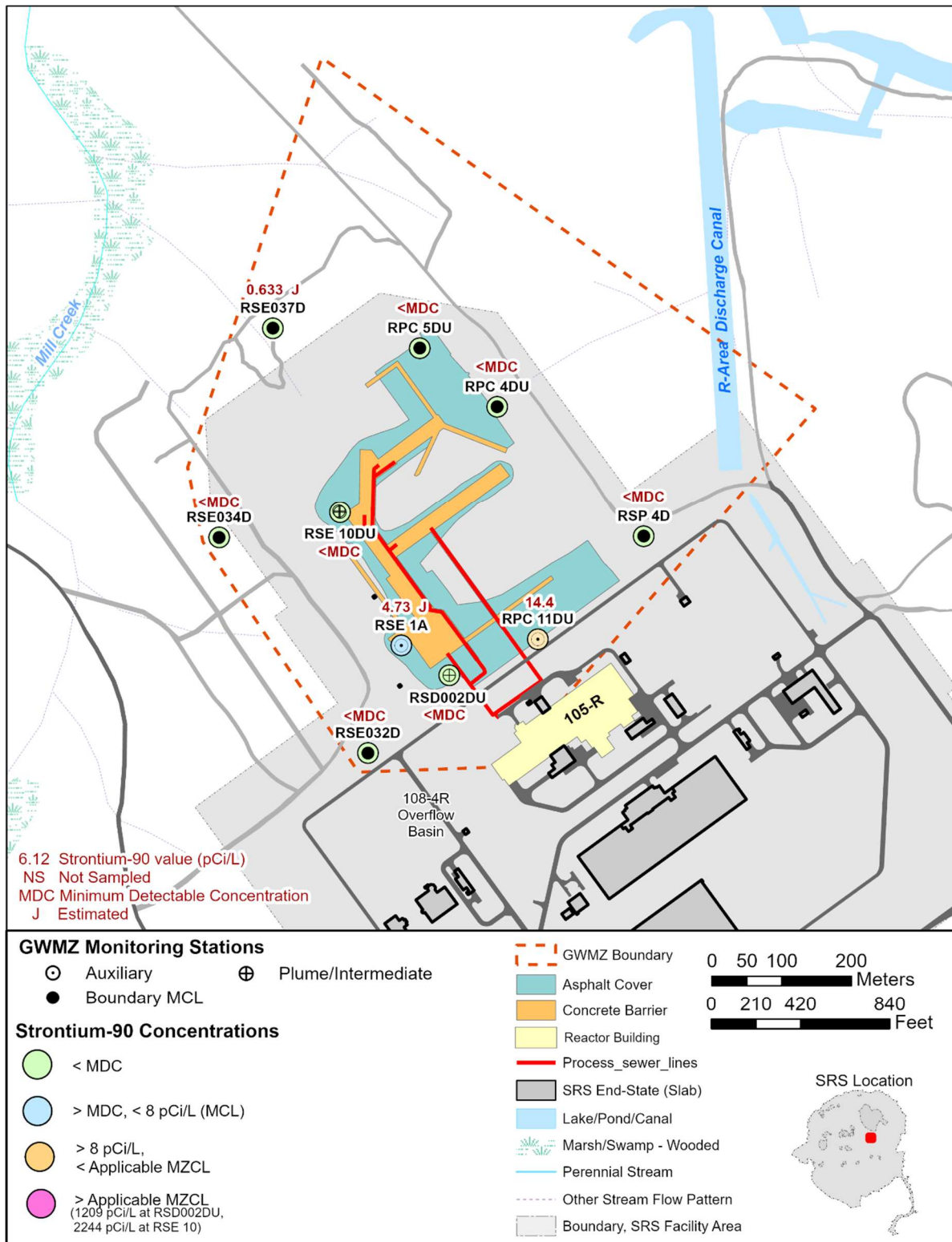
Figure B-7. Strontium-90 Concentrations in A/AA Horizons (1Q2022)
