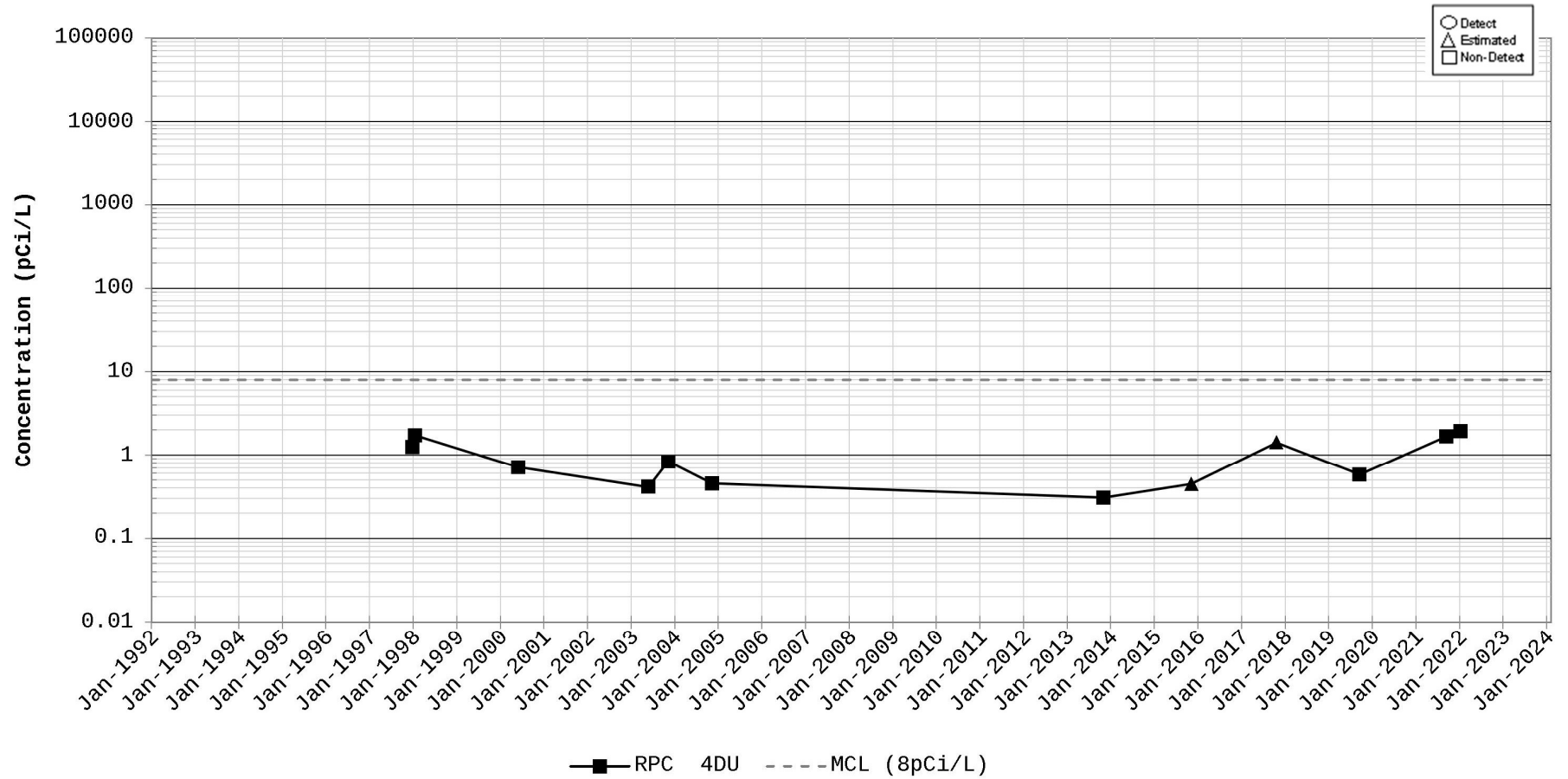
Time Series Plot for Strontium-90 Station for RPC 4
