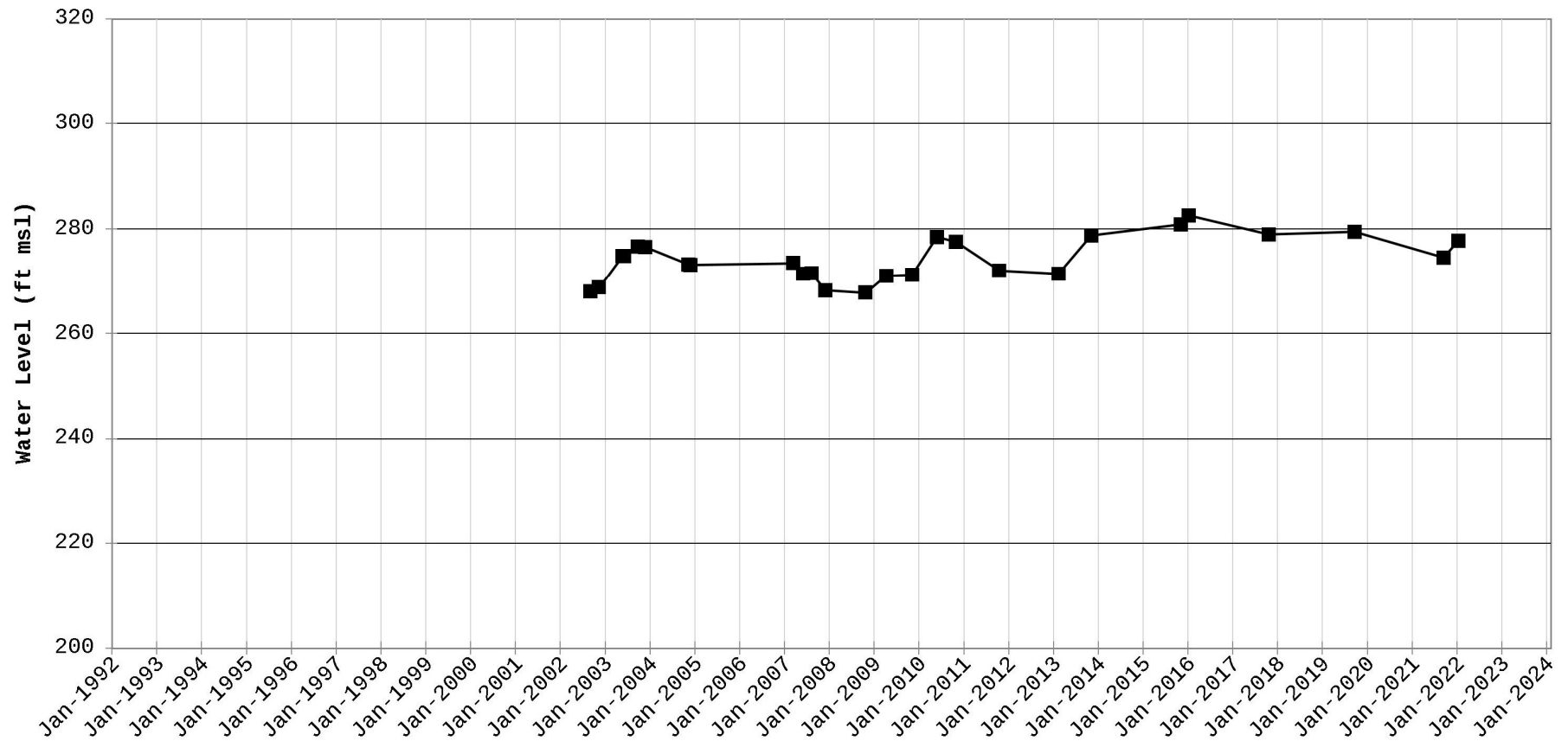
Hydrograph for Station RSE 26DL
