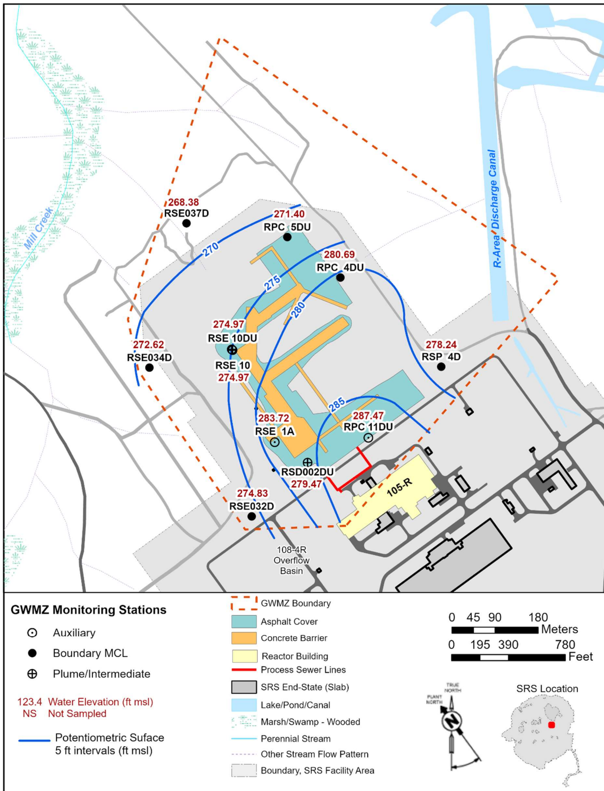
Figure B-5. Potentiometric Surface in A/AA Horizons (1Q2022)
