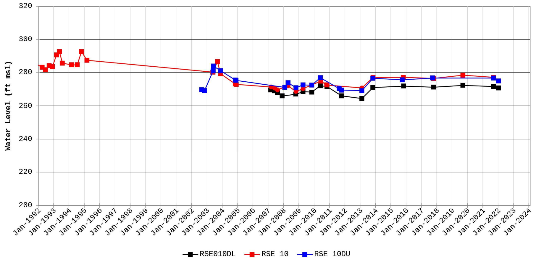
Hydrograph for Station RSE010
