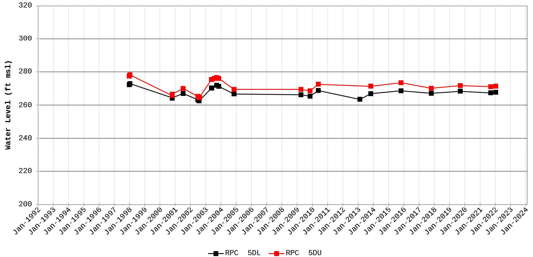
Hydrograph for Station RPC 5
