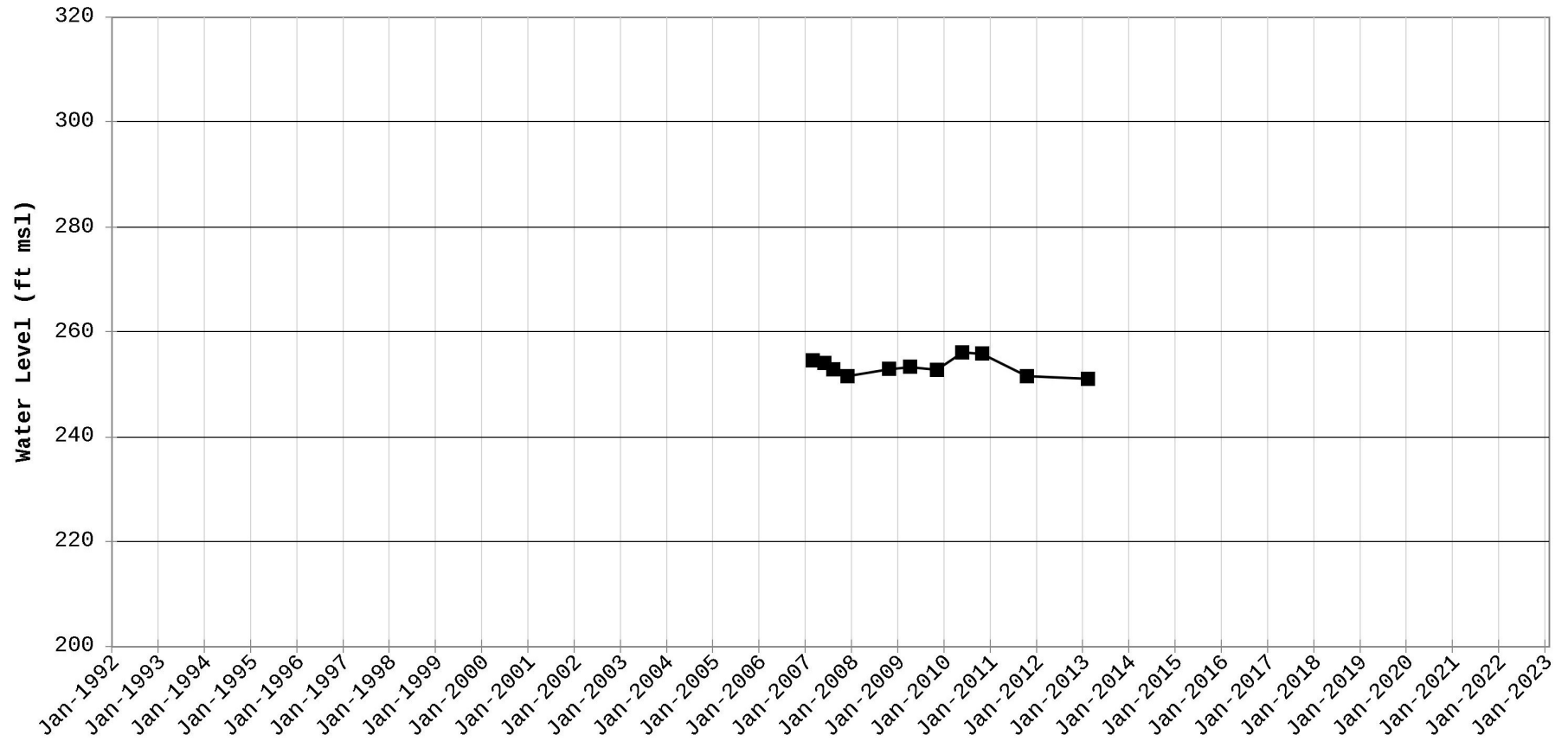
Hydrograph for Station RSE038B
