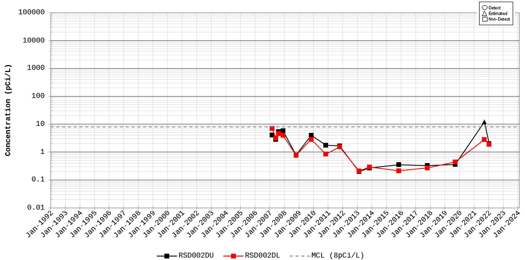
Time Series Plot for Strontium-90 Station for RSD002
