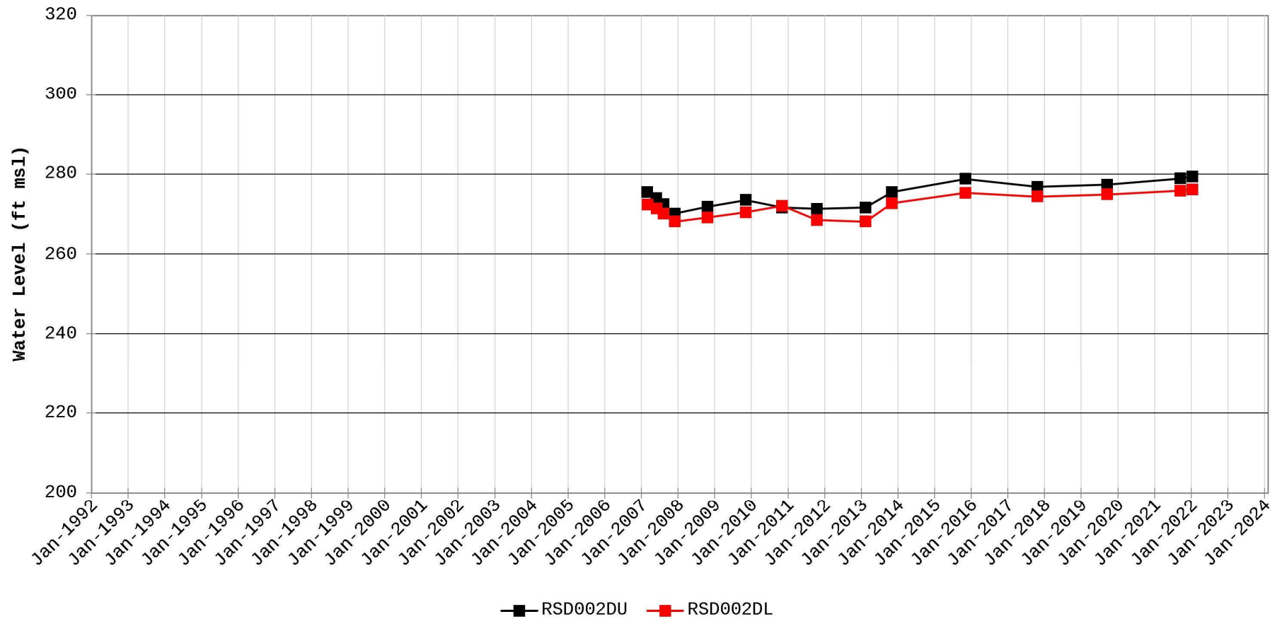
Hydrograph for Station RSD002
