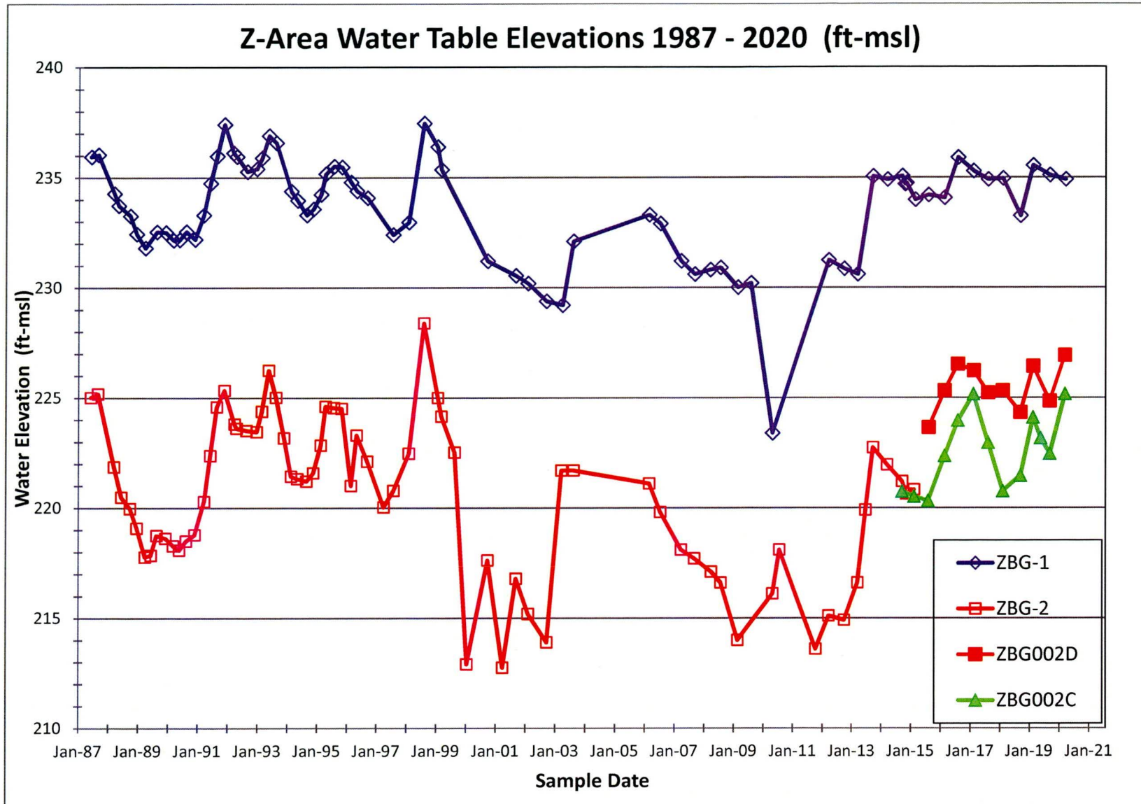
Figure 5. Z-Area Water Table Elevations (ft-msl)
