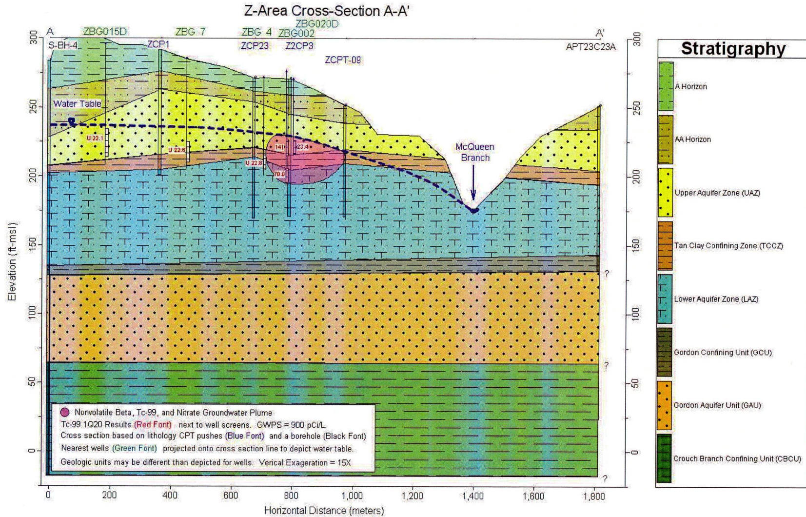
Figure 6. Z-Area Cross Section with 1Q20 Water Table
