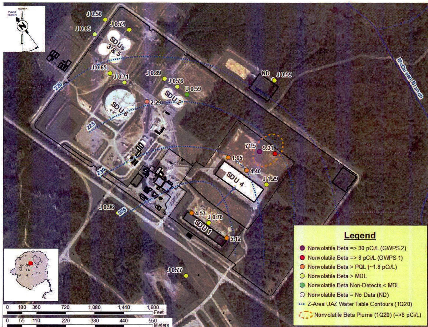
Figure 8. Approximate Nonvolatile Beta Groundwater Plume (1Q20)
