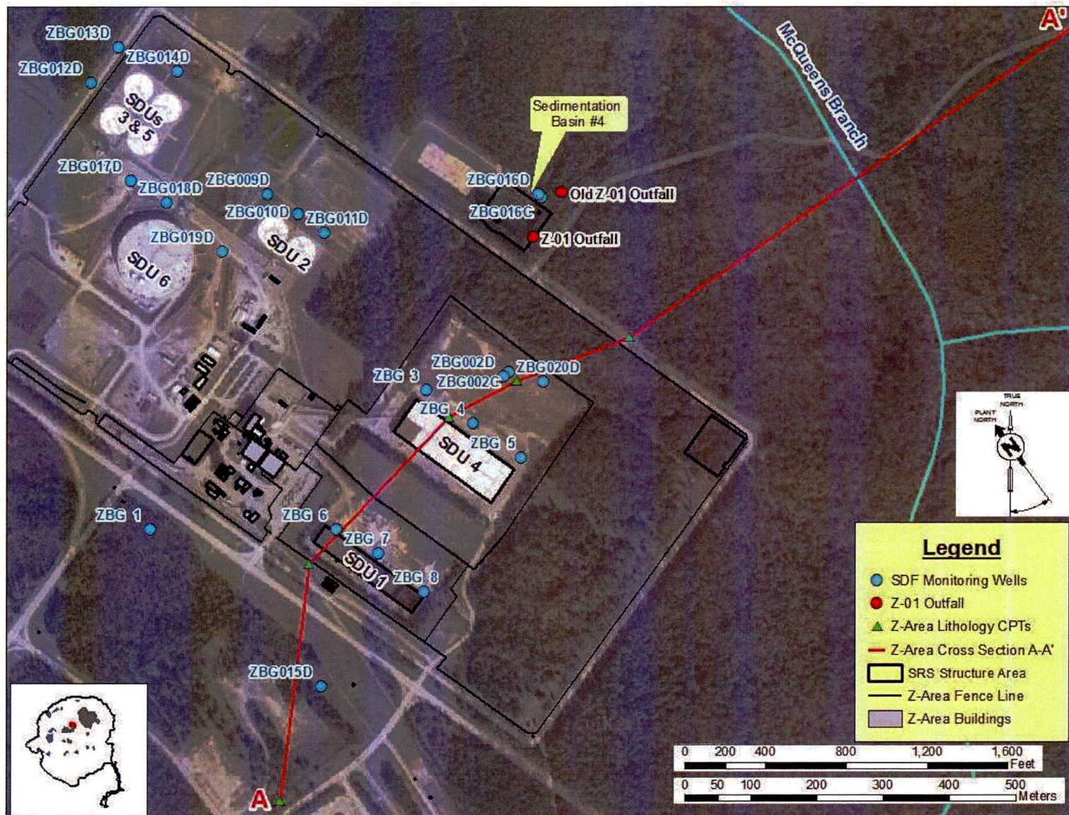
Figure 2. Monitoring Well Locations at the Saltstone Disposal Facility (SDF)
