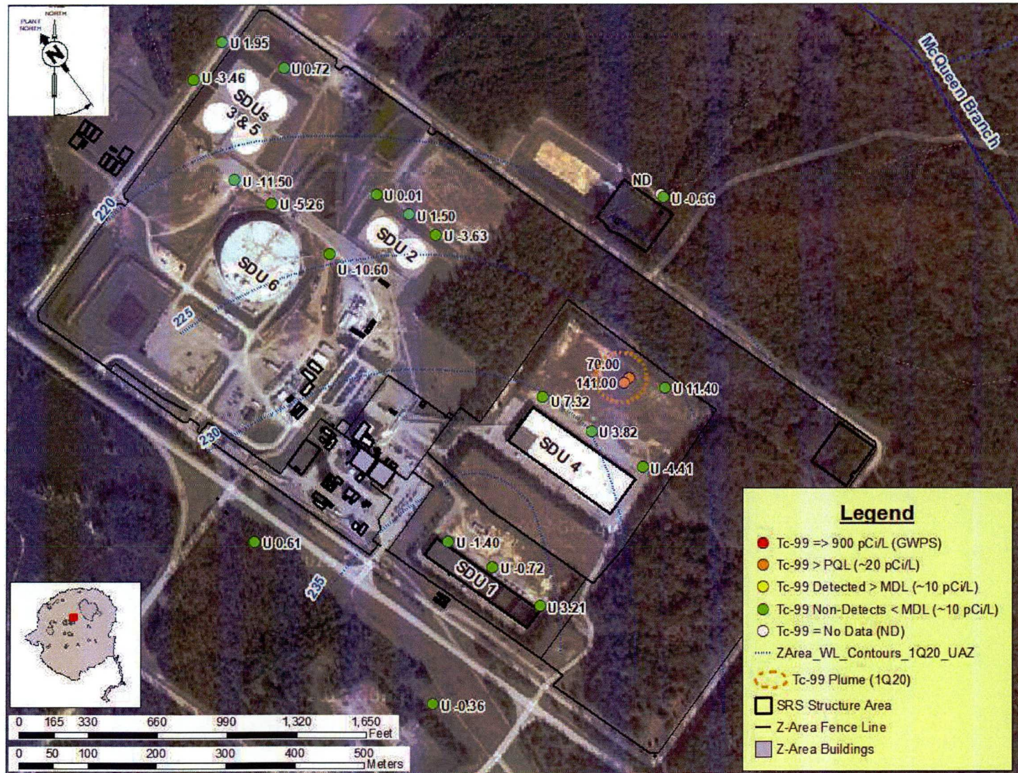
Figure 9. Approximate Tc-99 Groundwater Plume (1Q20)
