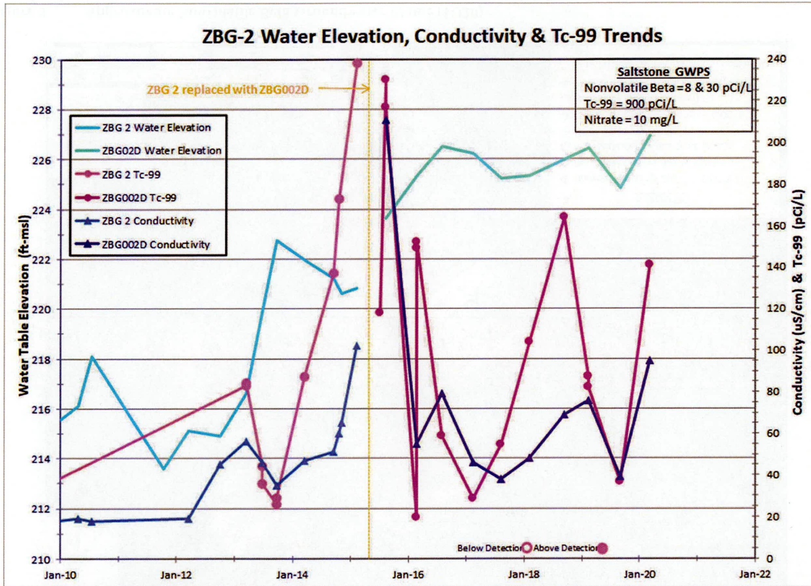
Figure 7. ZBG 2 / ZBG002D Tc-99 Groundwater Trends
