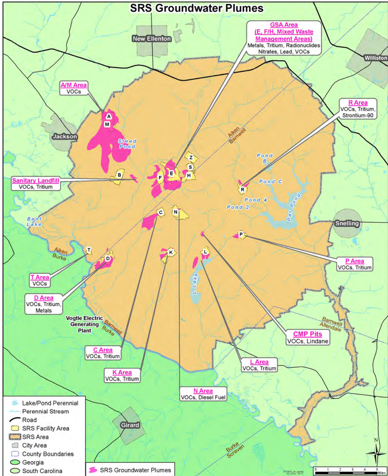
Figure 1. Groundwater Contamination Areas
