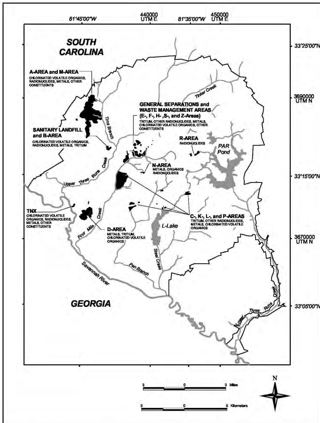
Figure 18 Facilities Monitored by the SRS Monitoring Well Network; Shaded Areas Indicate Extent of Groundwater Contamination.
