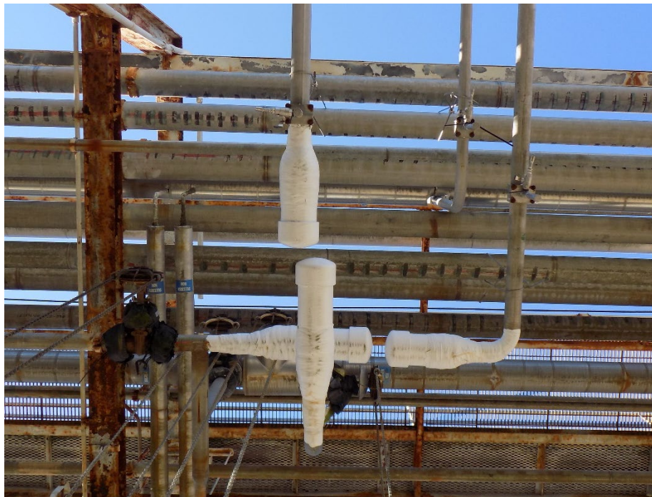
Photo 7 - Pipe Caps/Wraps and Pipe Taps
