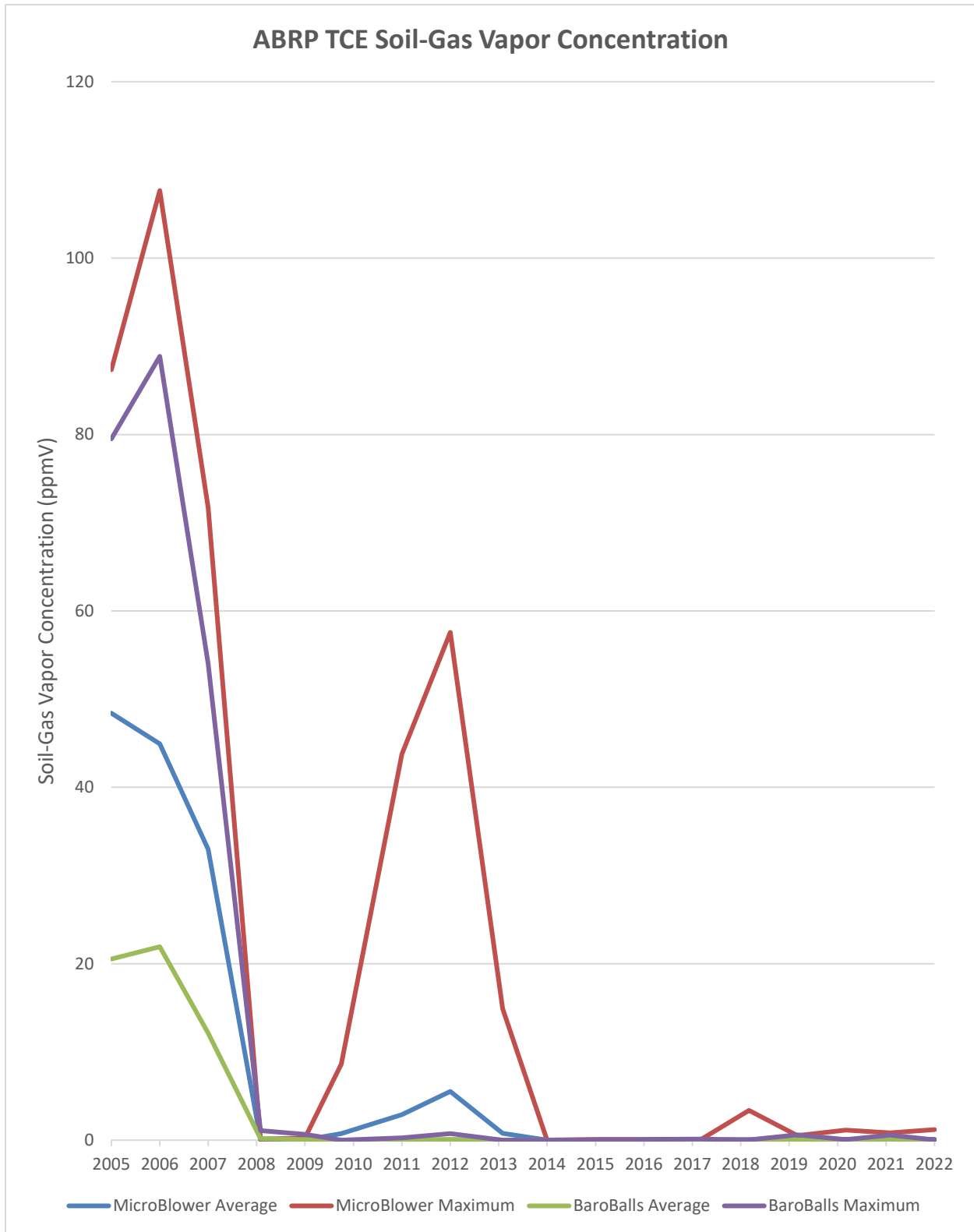
Figure 7. ABRP Soil-Gas Vapor Concentration Over Time Trend Diagram
