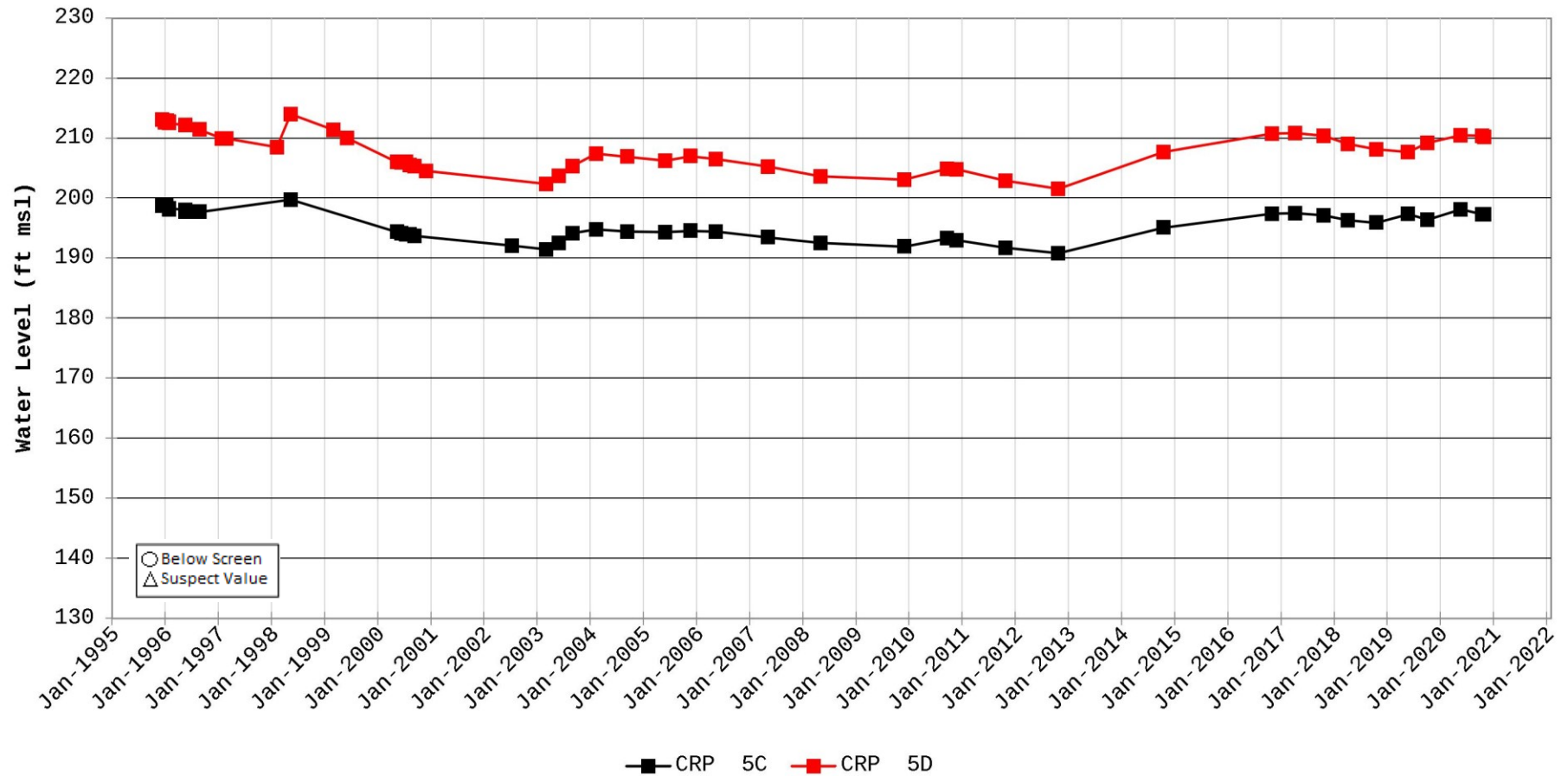
Figure B-2. Hydrograph for Station CRP 5
