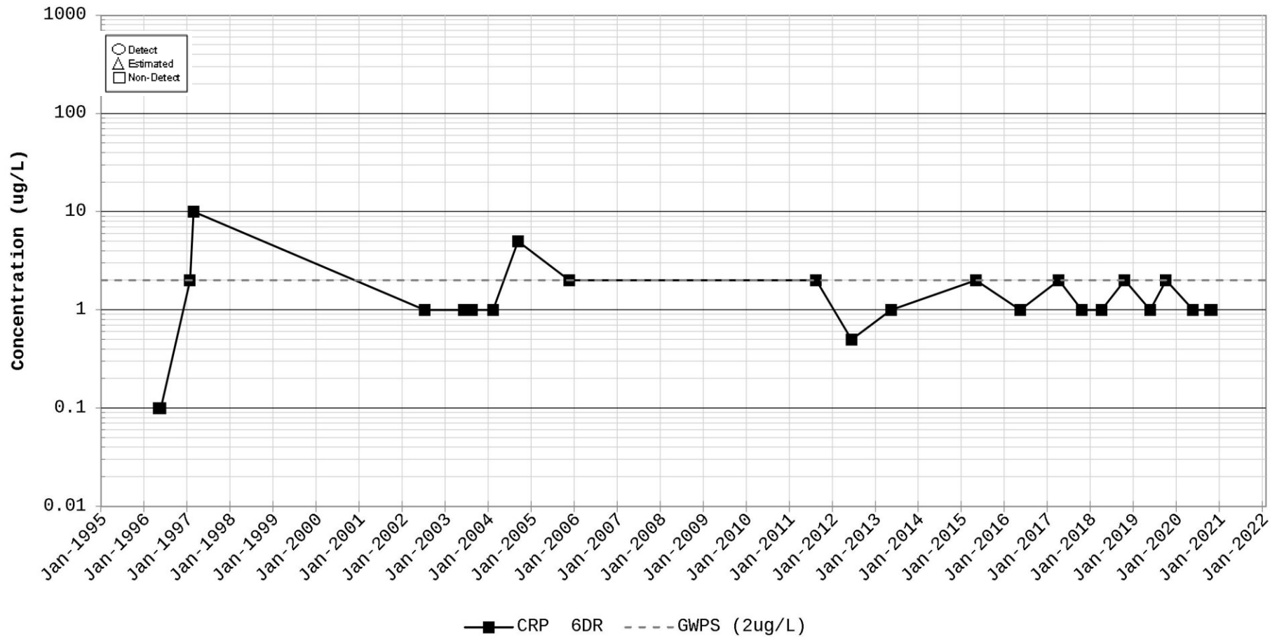
Time Series Plot for Chloroethene (Vinyl Chloride) Station for CRP 6
