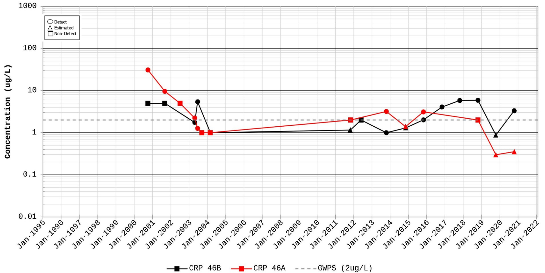
Time Series Plot for Chloroethene (Vinyl Chloride) Station for CRP 46
