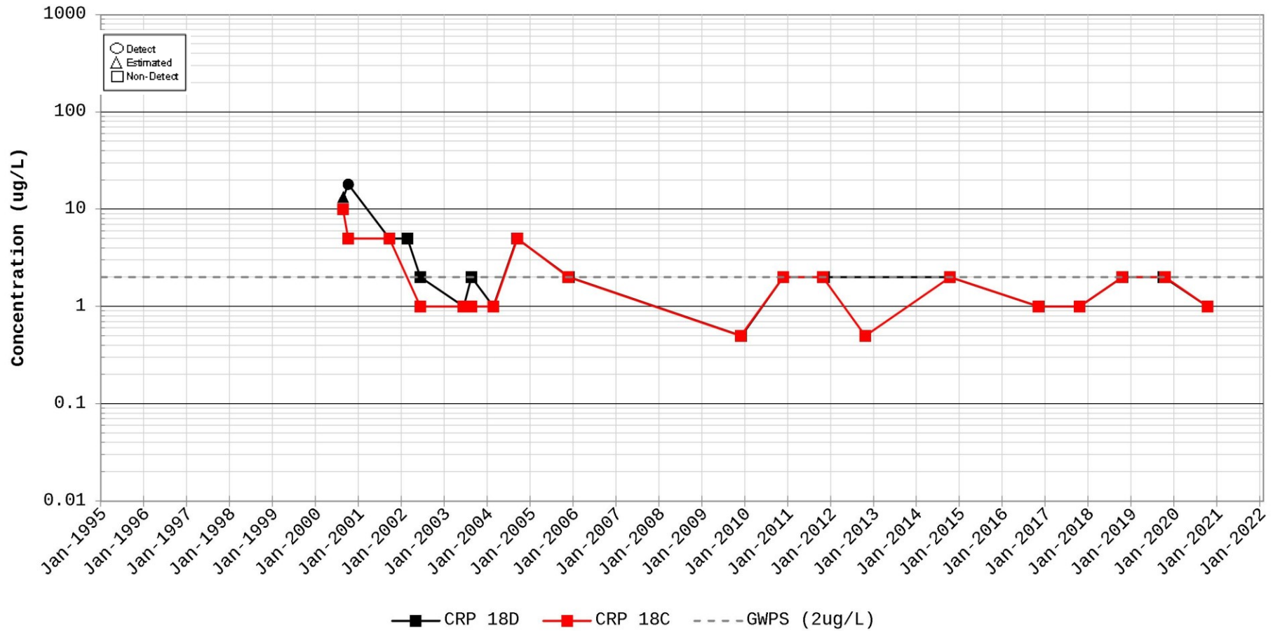
Figure C-21. Time Series Plot for Chloroethene (Vinyl Chloride) Station for CRP 18
