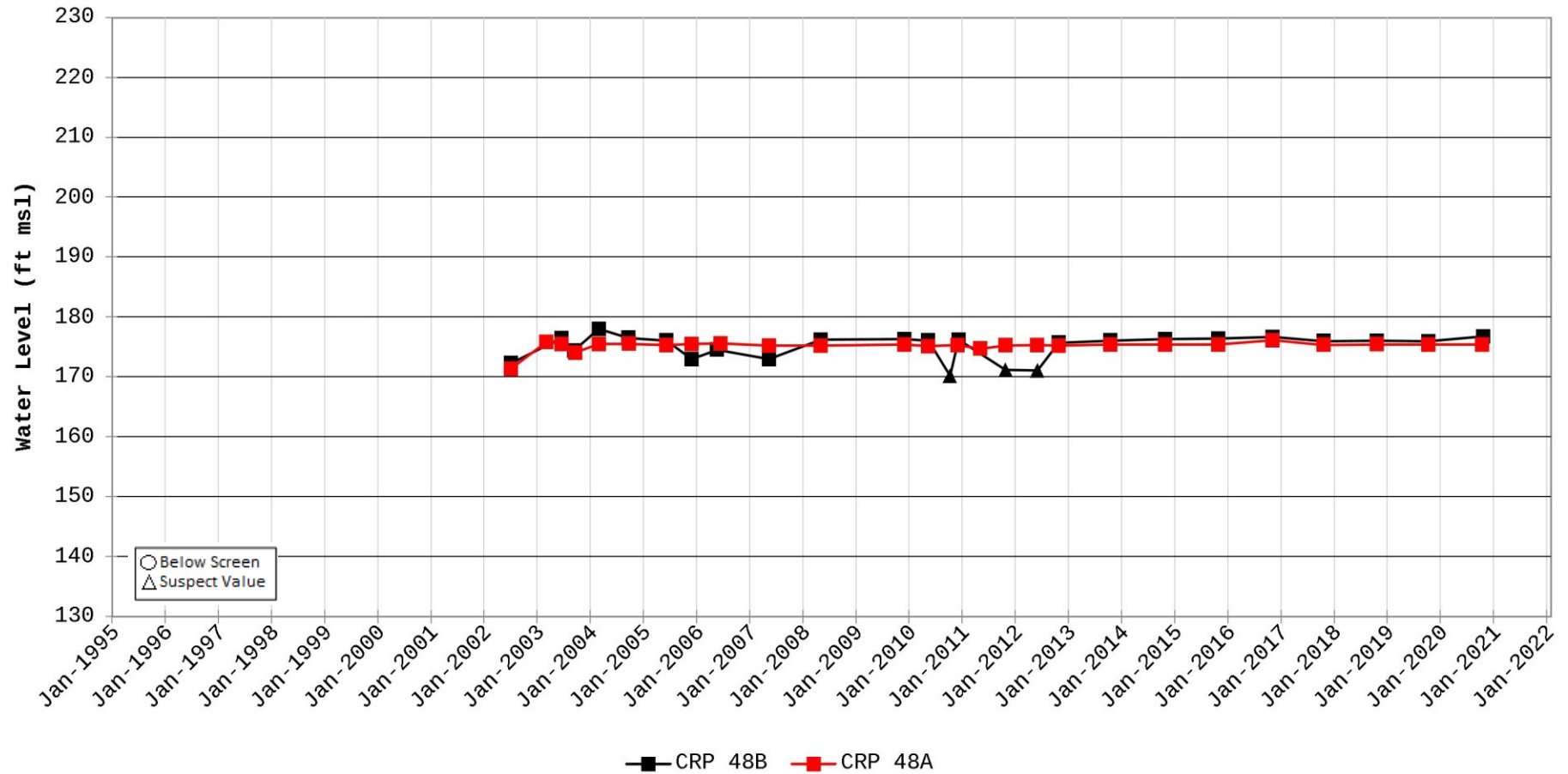
Hydrograph for Station CRP 48
