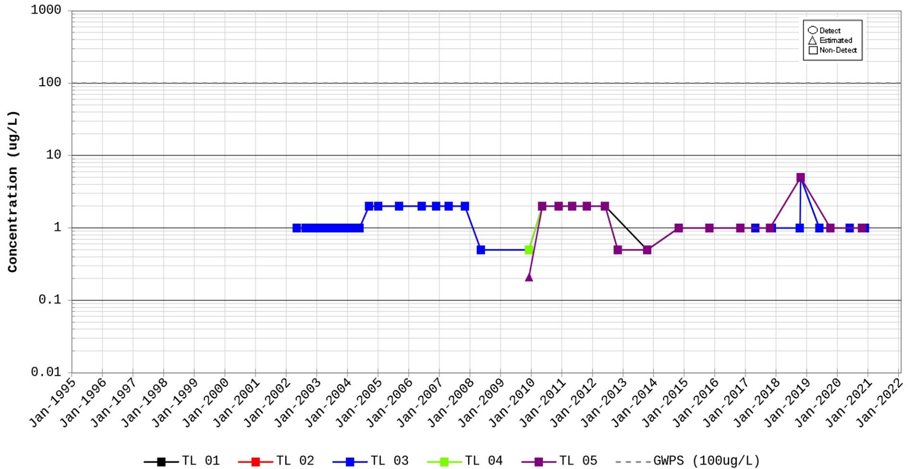
Time Series Plot for Trans-1,2-dichloroethylene Station for TL 01
