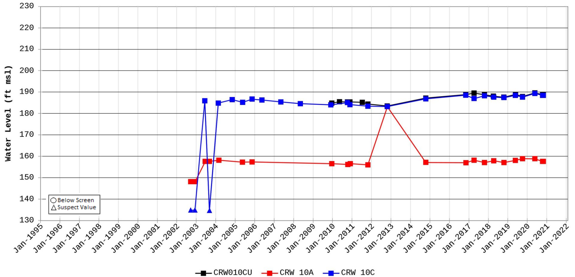
Hydrograph for Station CRW010
