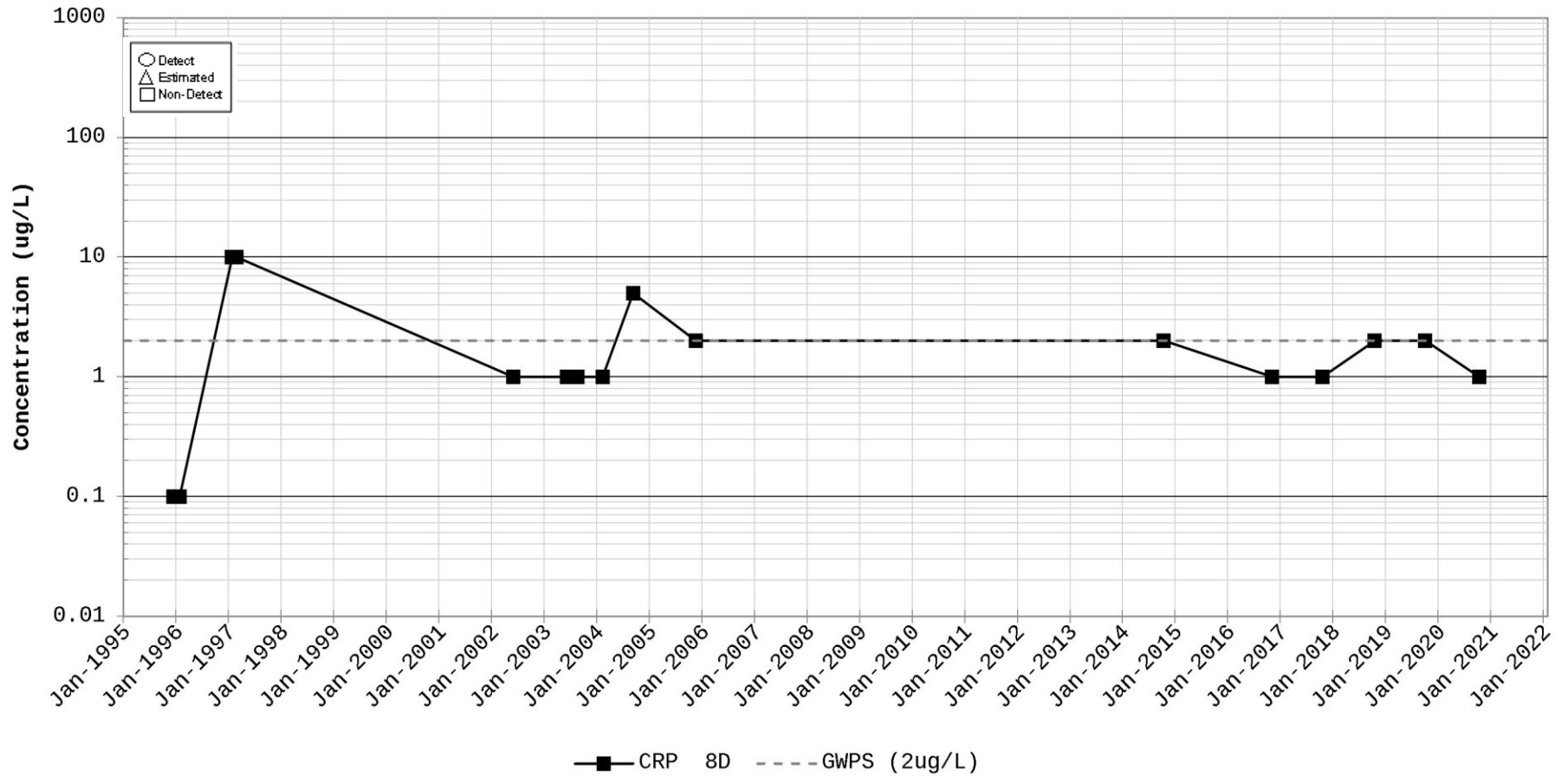
Time Series Plot for Chloroethene (Vinyl Chloride) Station for CRP 8
