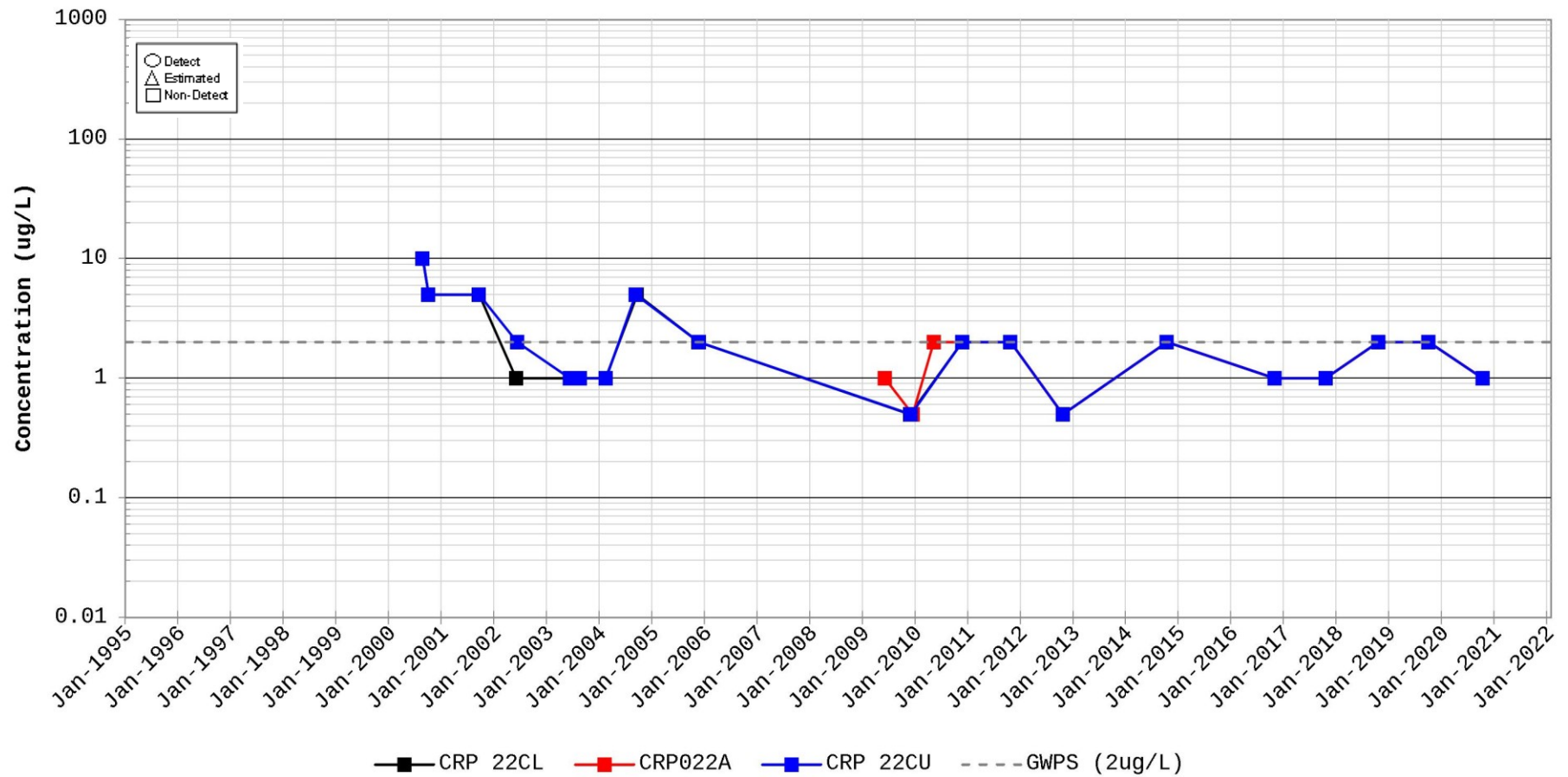
Time Series Plot for Chloroethene (Vinyl Chloride) Station for CRP 22
