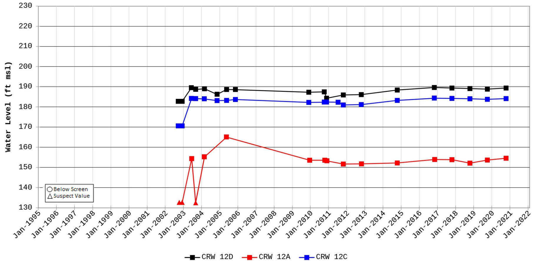
Hydrograph for Station CRW 12
