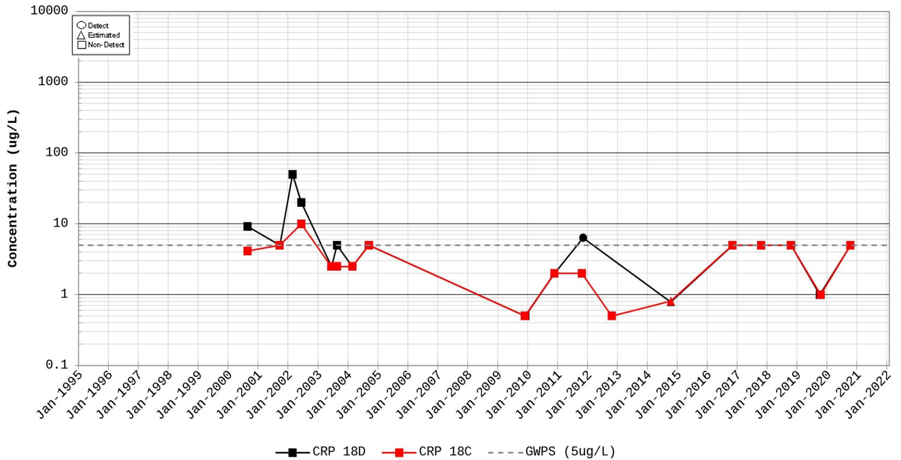
Time Series Plot for Dichloromethane (Methylene Chloride) Station for CRP 18
