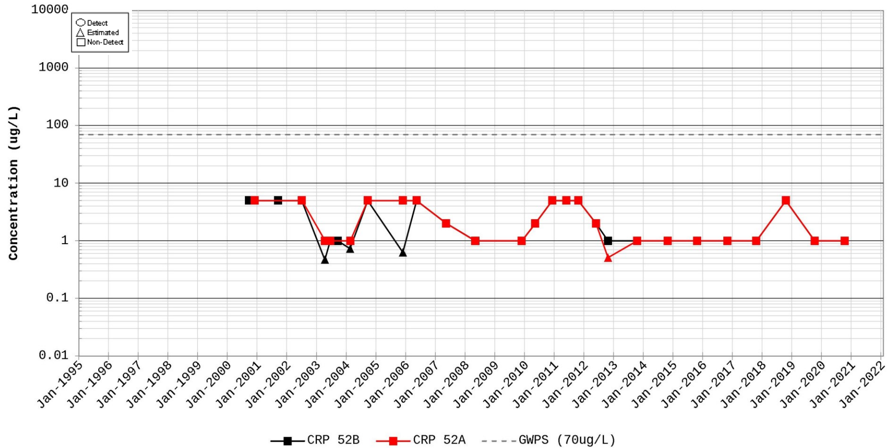
Time Series Plot for cis-1,2-Dichloroethylene Station for CRP 52
