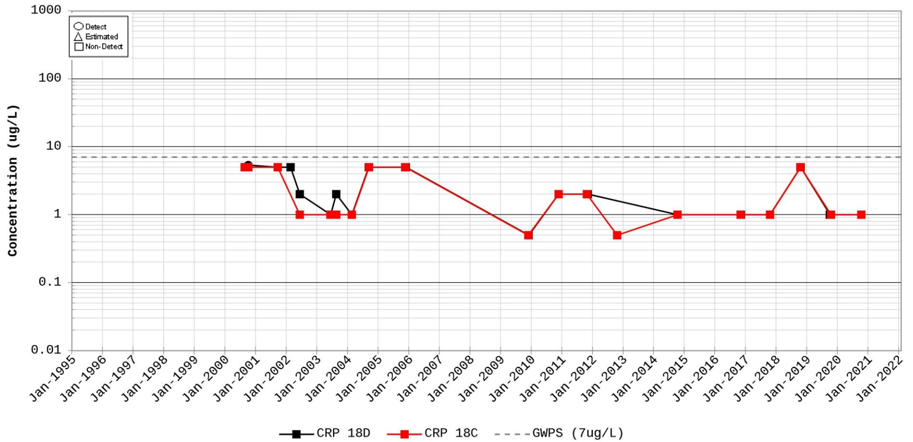
Time Series Plot for 1,1-Dichloroethylene Station for CRP 18
