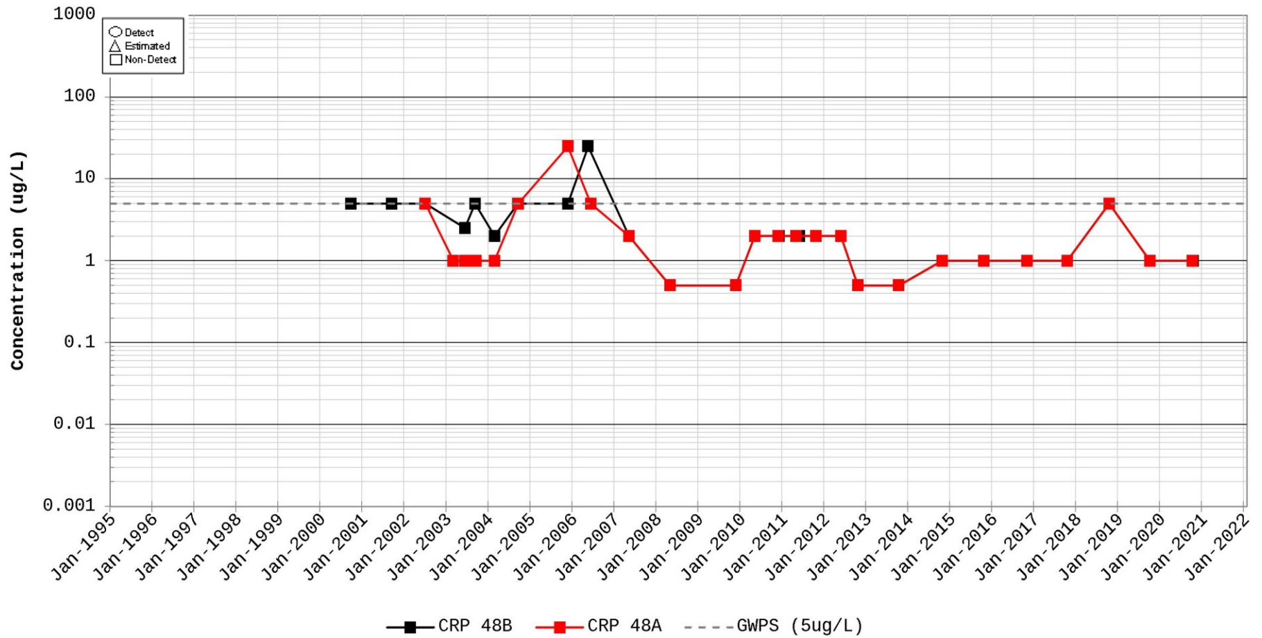
Figure C-81. Time Series Plot for Tetrachloroethylene (PCE) Station for CRP 48
