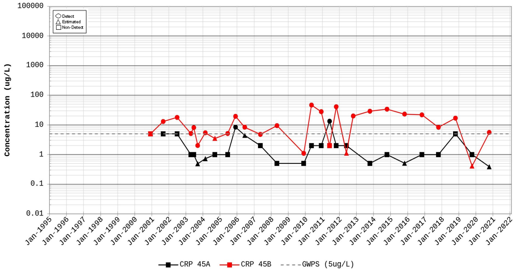
Figure C-111. Time Series Plot for Trichloroethylene (TCE) Station for CRP 45
