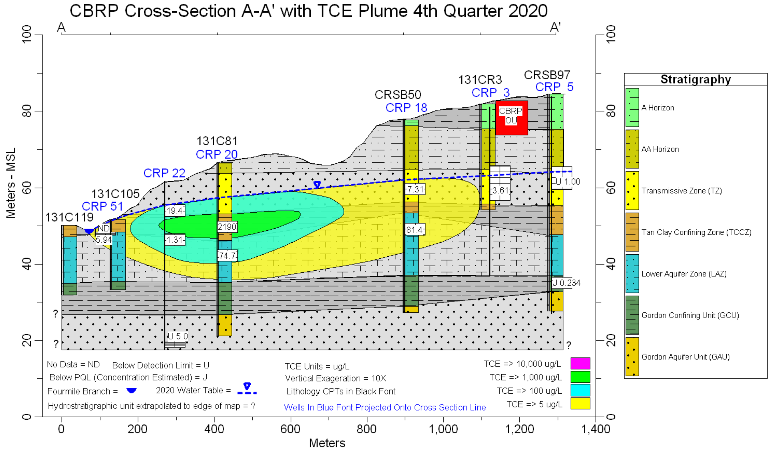
Figure 7. CBRP Plume Cross Section, Fourth Quarter 2020
