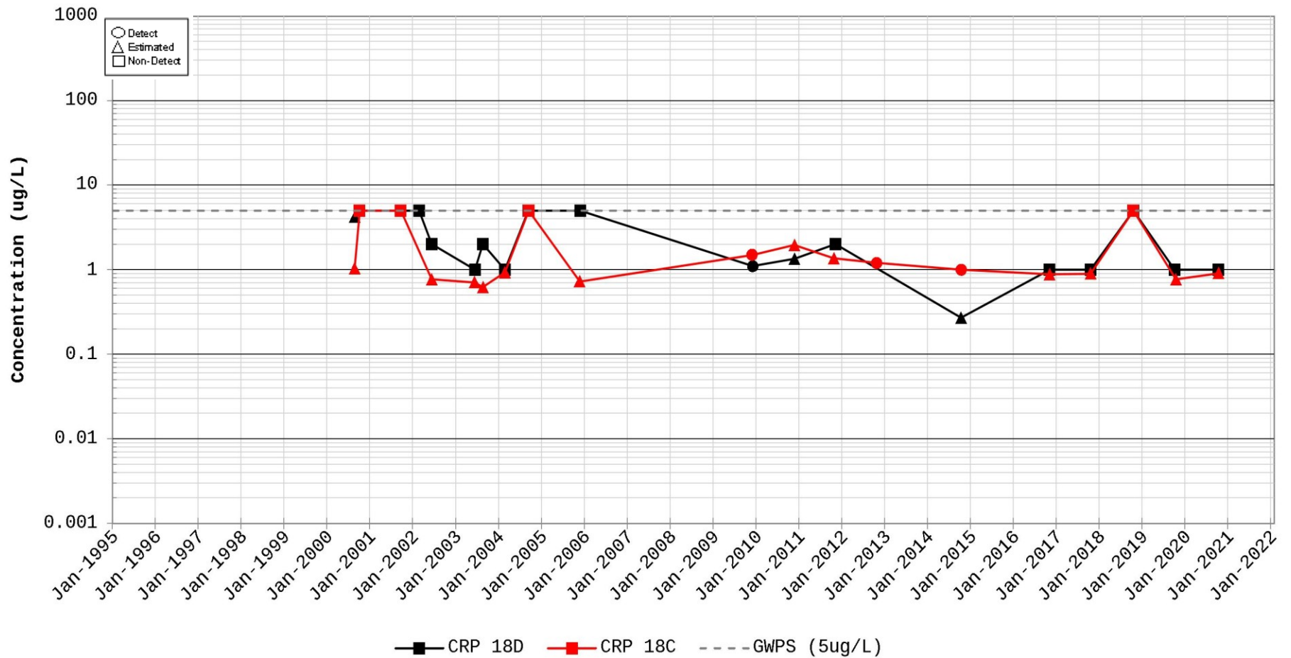
Time Series Plot for Tetrachloroethylene (PCE) Station for CRP 18
