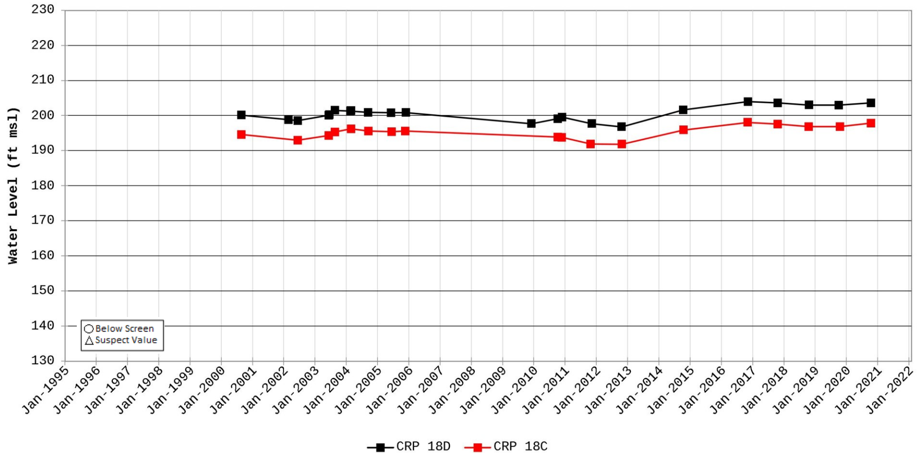
Hydrograph for Station CRP 18
