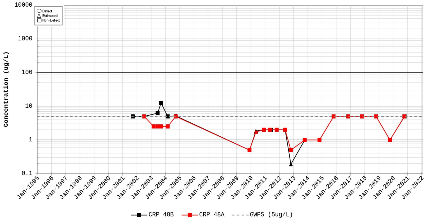
Time Series Plot for Dichloromethane (Methylene Chloride) Station for CRP 48
