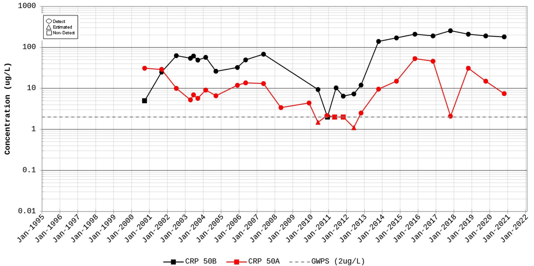
Time Series Plot for Chloroethene (Vinyl Chloride) Station for CRP 50
