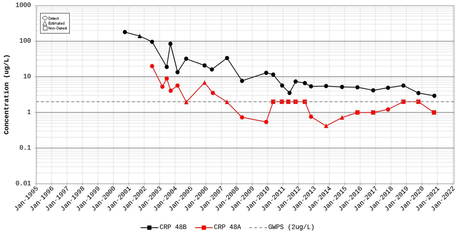
Time Series Plot for Chloroethene (Vinyl Chloride) Station for CRP 48
