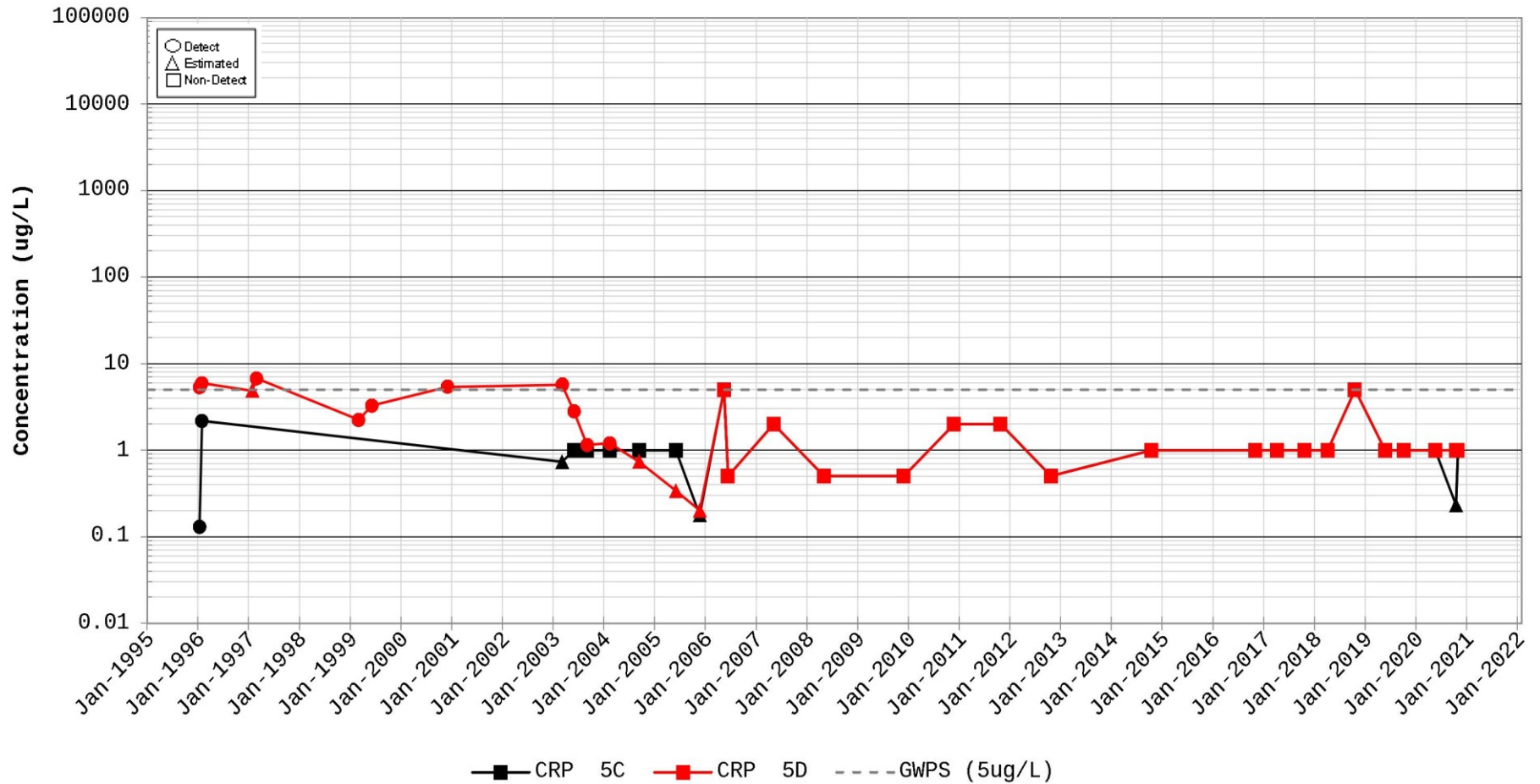
Time Series Plot for Trichloroethylene (TCE) Station for CRP 5
