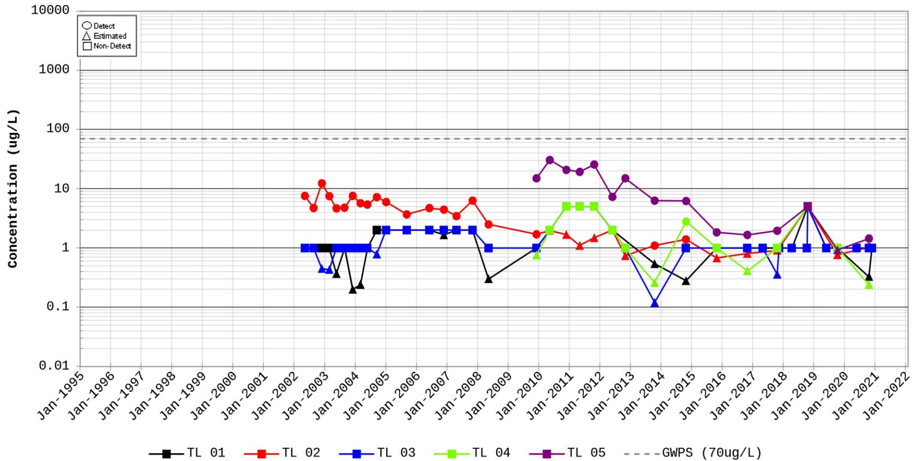
Time Series Plot for cis-1,2-Dichloroethylene Station for TL 01
