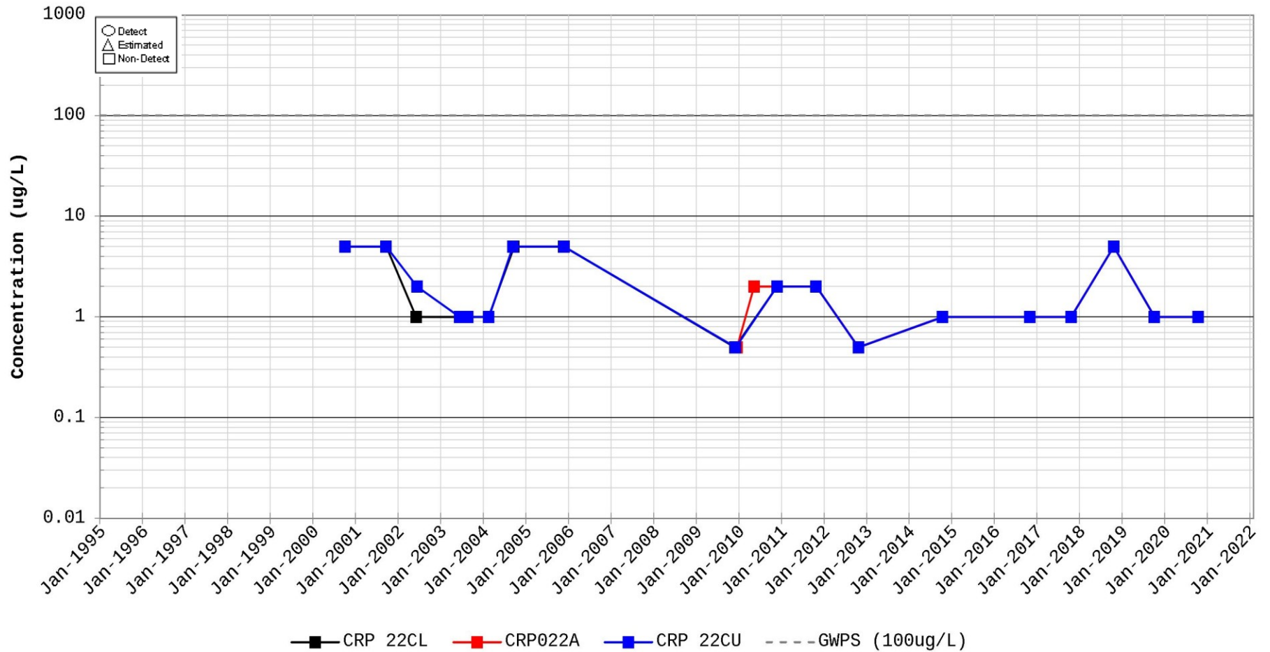
Time Series Plot for Trans-1,2-dichloroethylene Station for CRP 22
