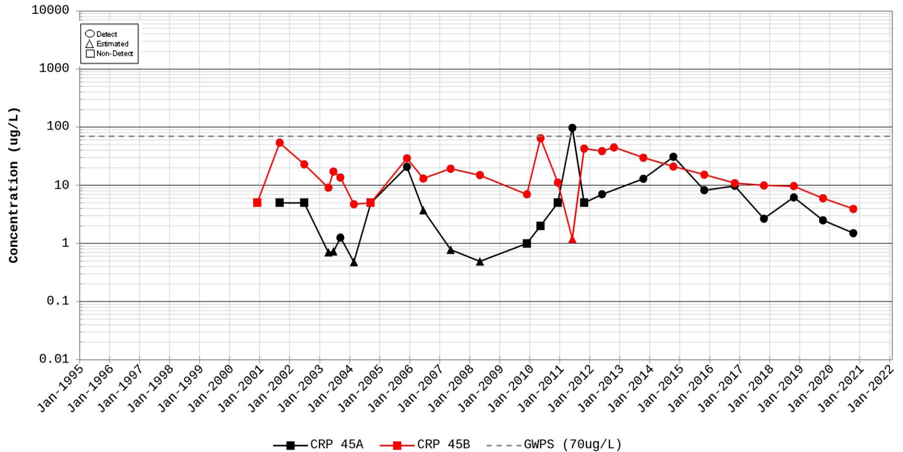
Time Series Plot for cis-1,2-Dichloroethylene Station for CRP 45
