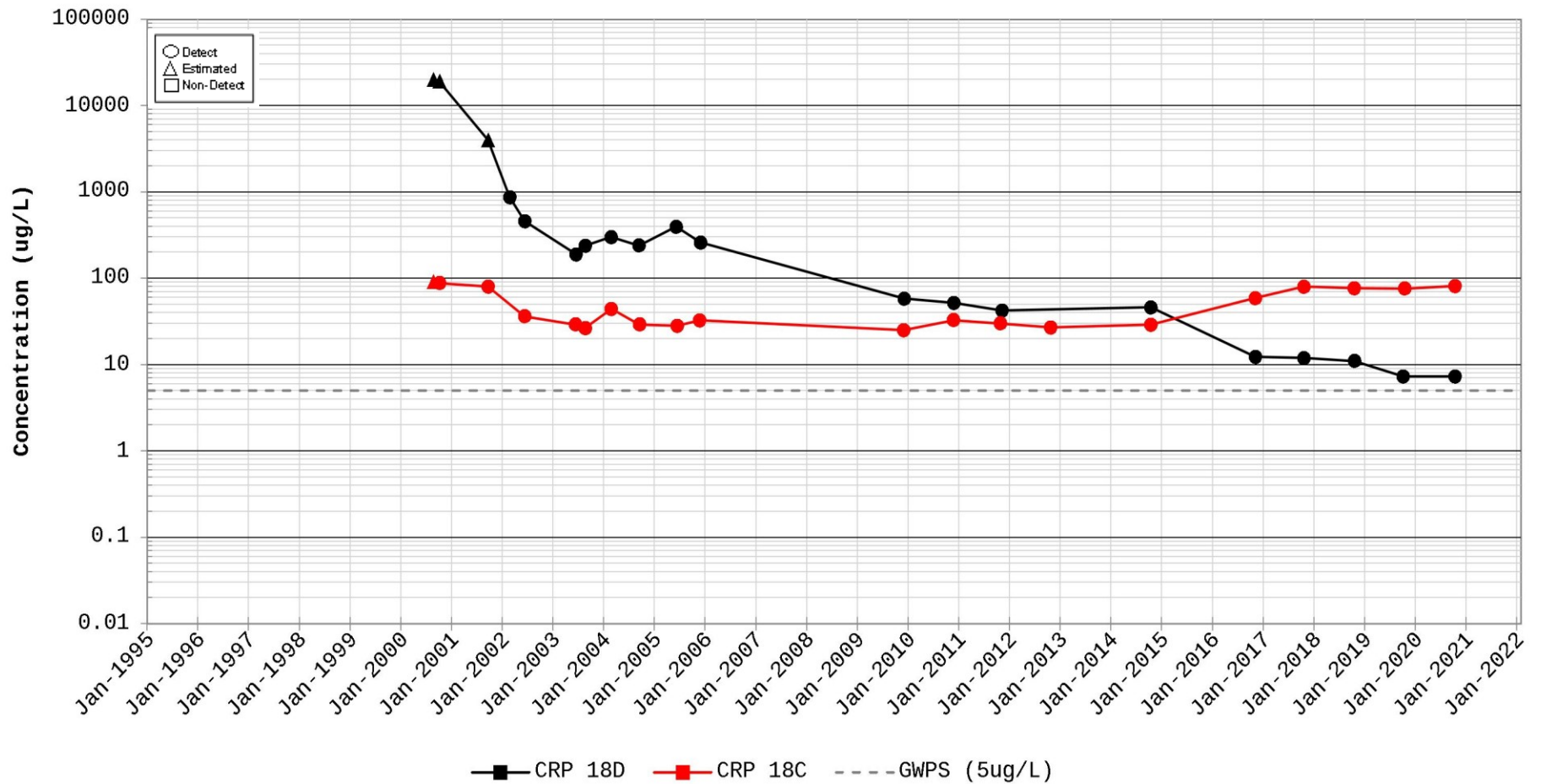
Time Series Plot for Trichloroethylene (TCE) Station for CRP 18
