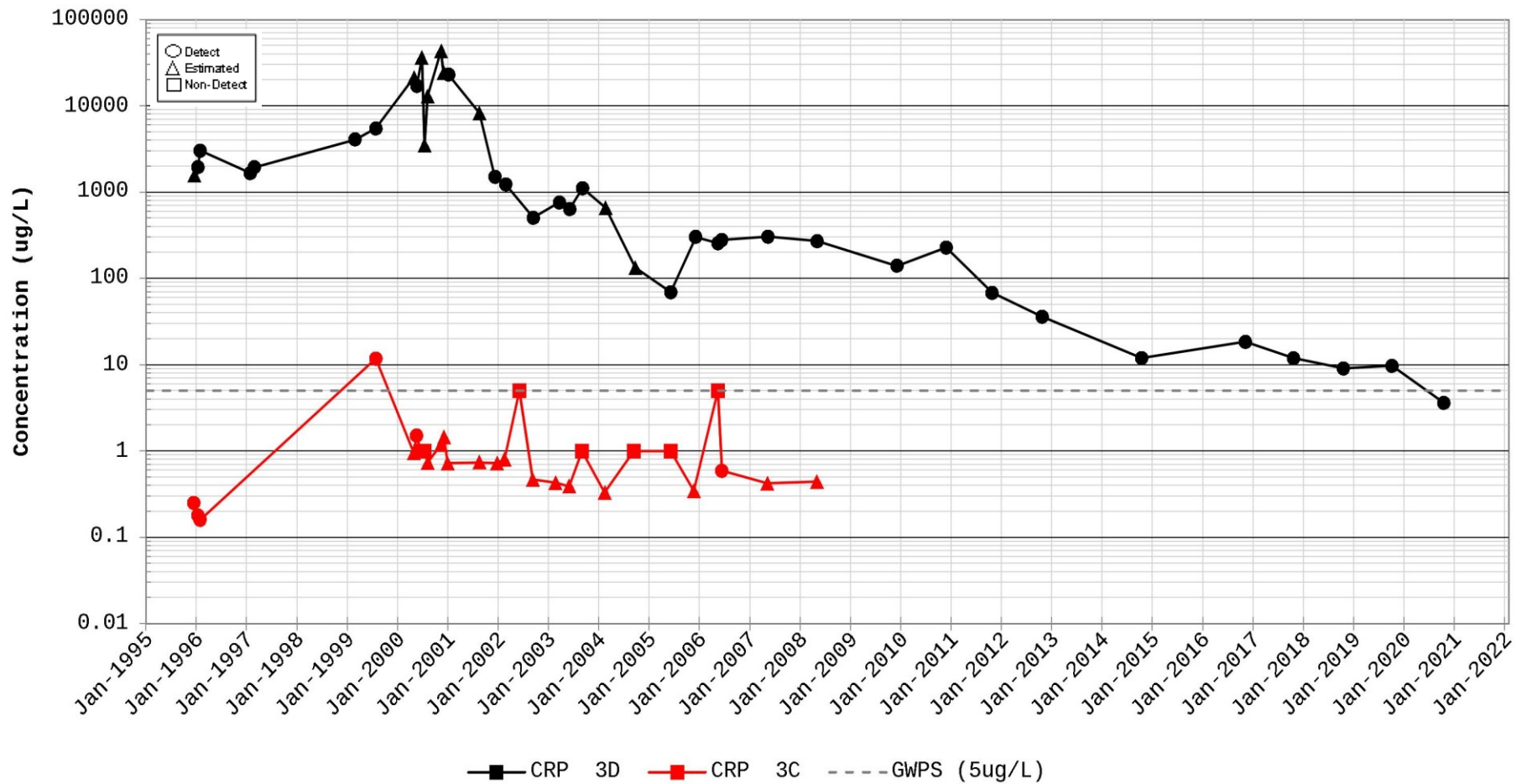
Time Series Plot for Trichloroethylene (TCE) Station for CRP 3
