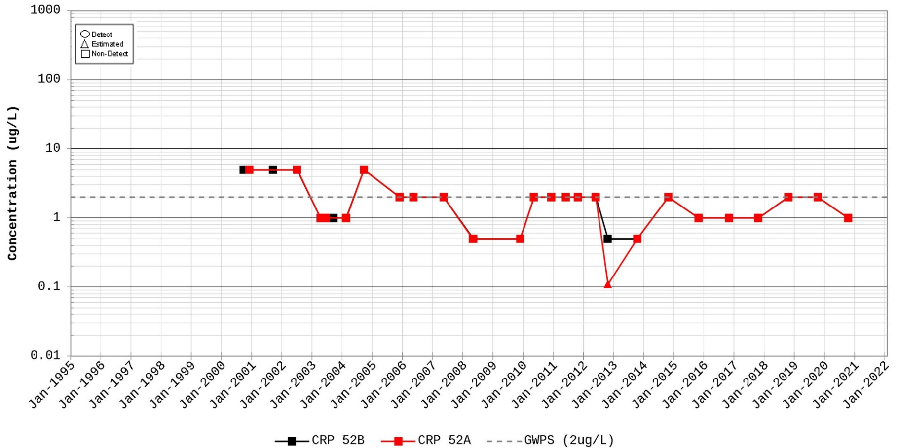
Time Series Plot for Chloroethene (Vinyl Chloride) Station for CRP 52
