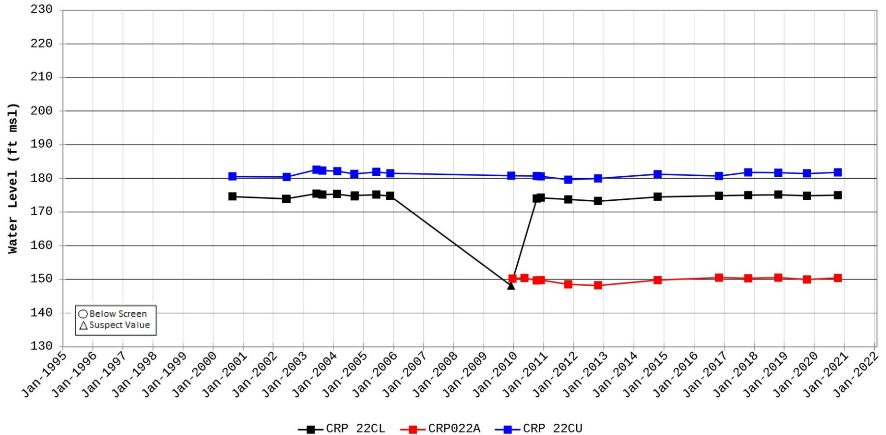
Hydrograph for Station CRP 22
