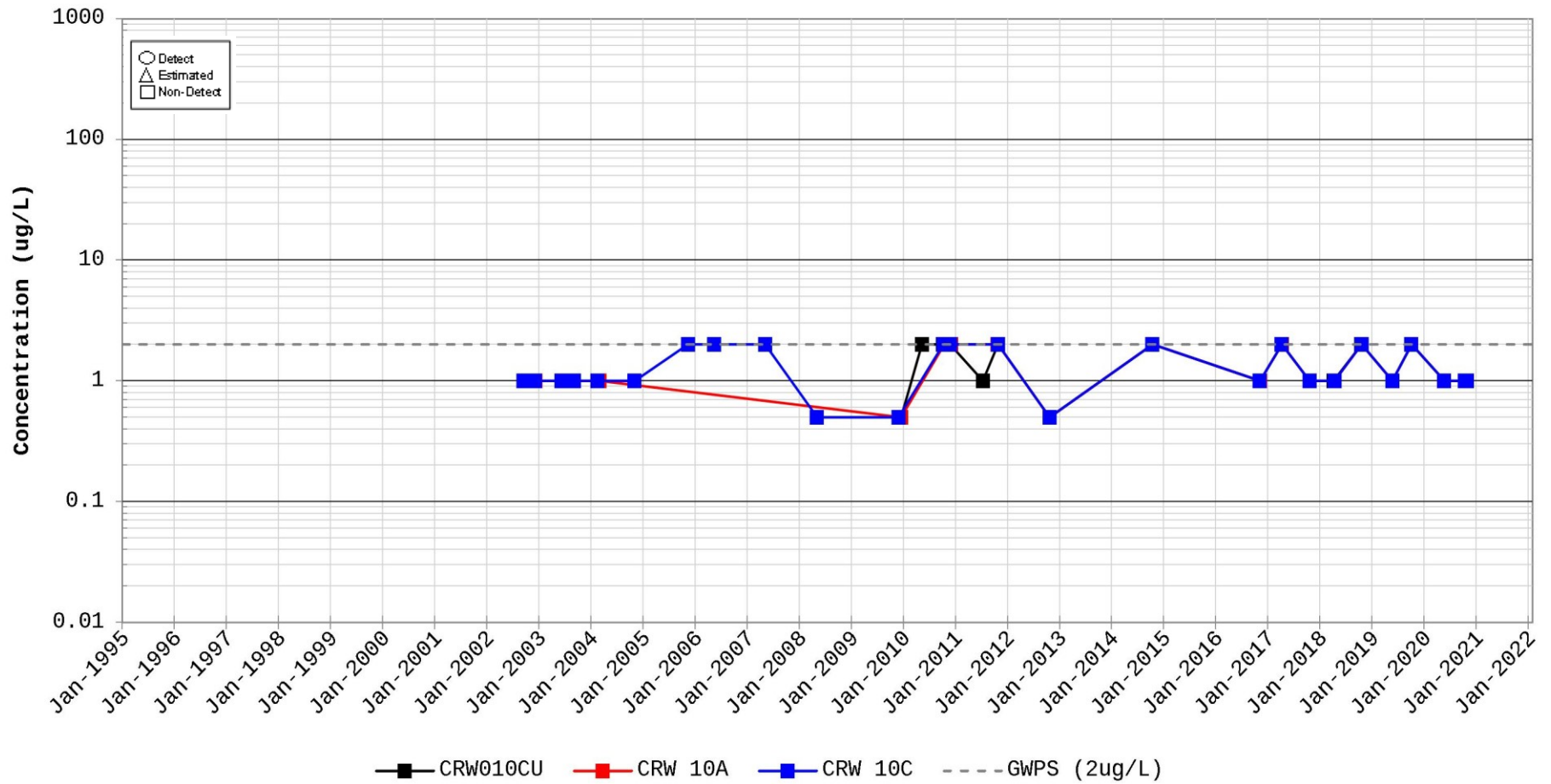
Time Series Plot for Chloroethene (Vinyl Chloride) Station for CRW010
