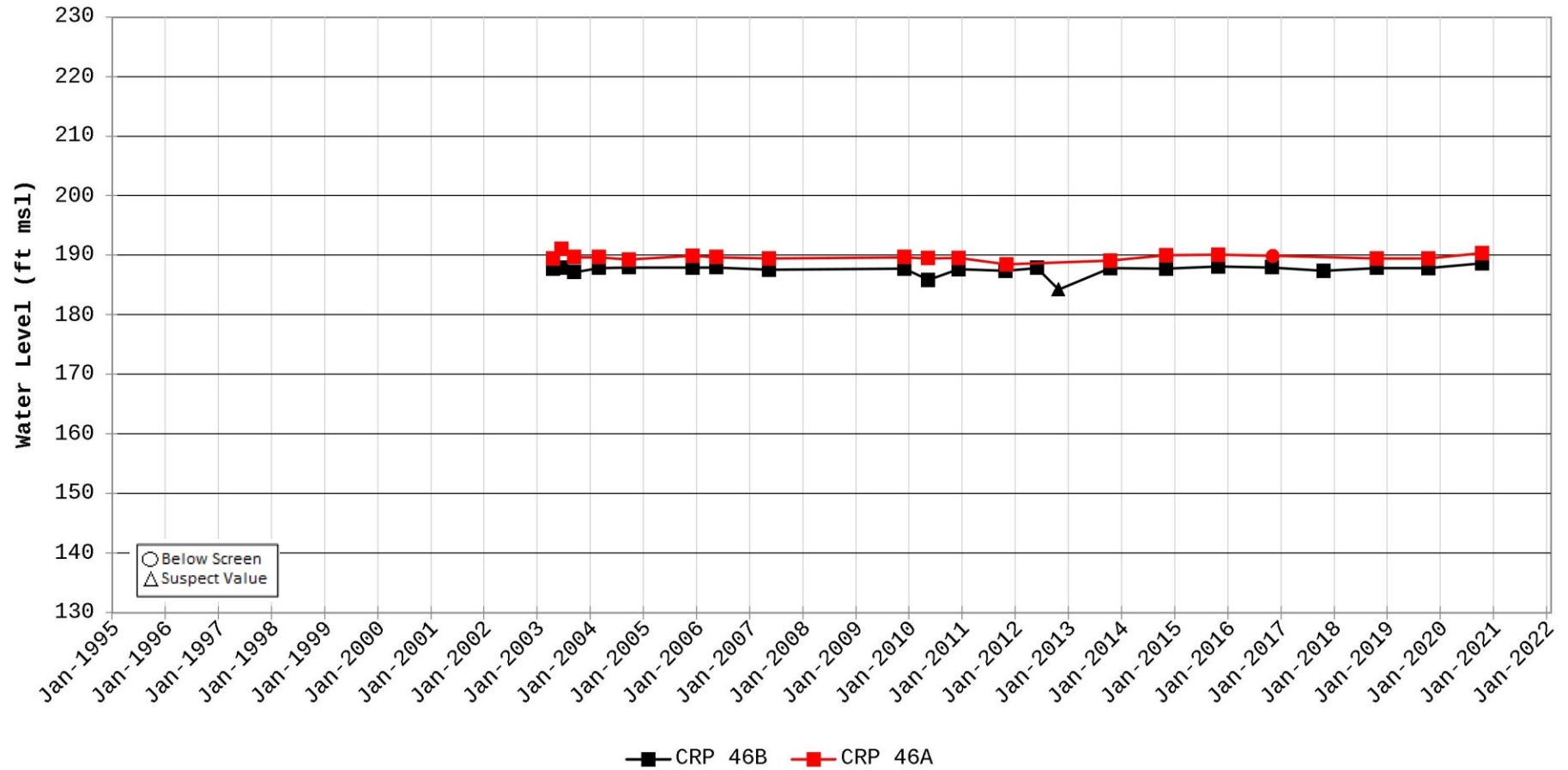
Hydrograph for Station CRP 46
