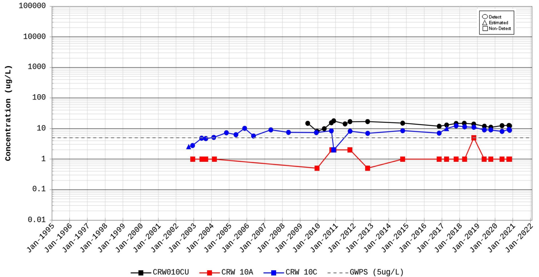
Figure C-117. Time Series Plot for Trichloroethylene (TCE) Station for CRW010
