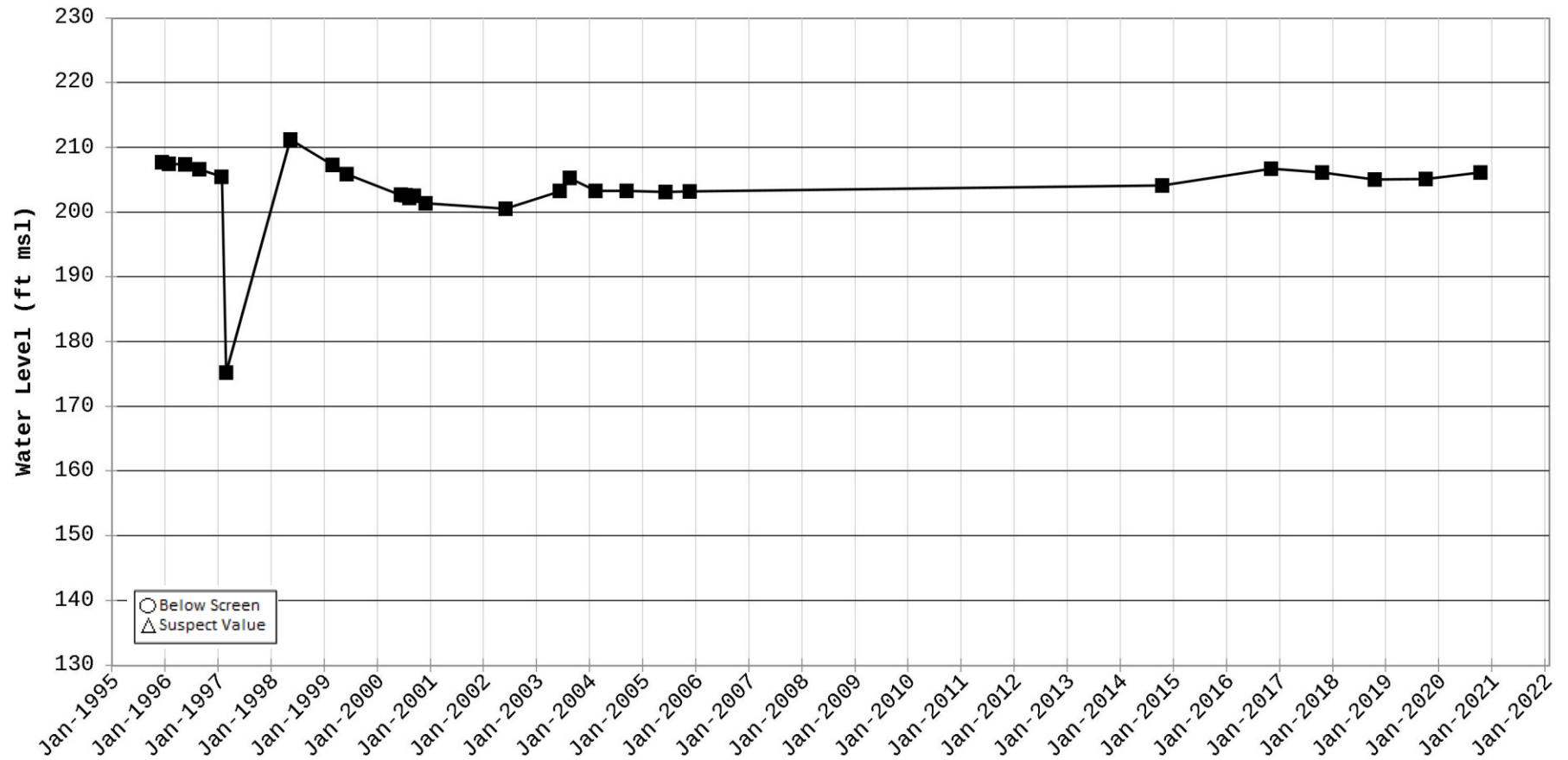
Figure B-4. Hydrograph for Station CRP 8D
