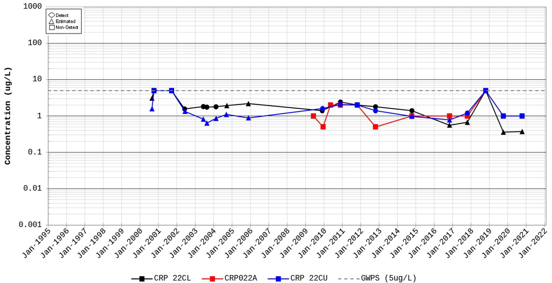
Time Series Plot for Tetrachloroethylene (PCE) Station for CRP 22
