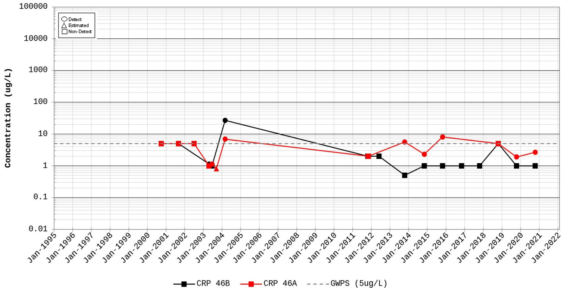
Figure C-112. Time Series Plot for Trichloroethylene (TCE) Station for CRP 46
