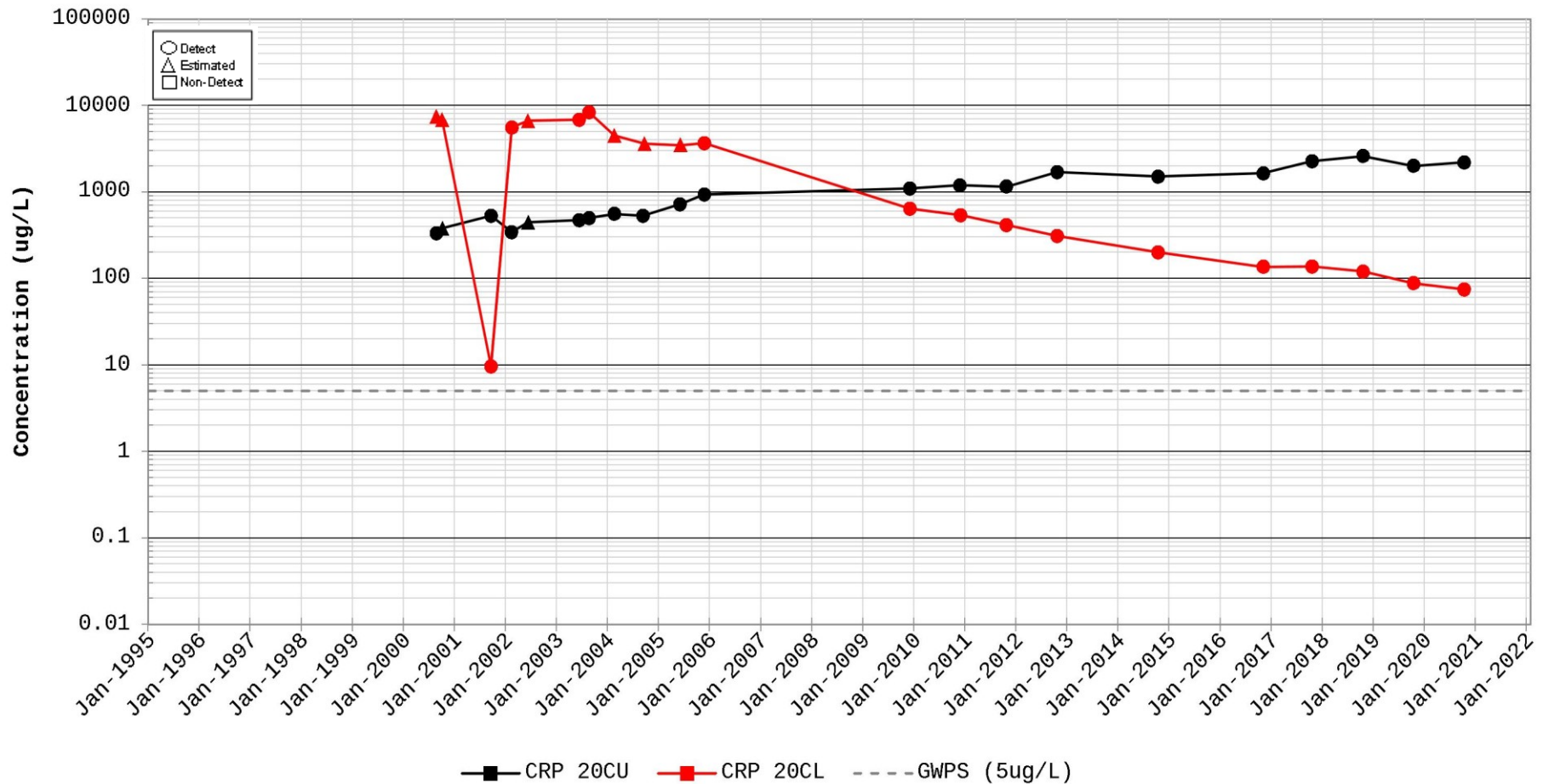
Figure C-109. Time Series Plot for Trichloroethylene (TCE) Station for CRP 20
