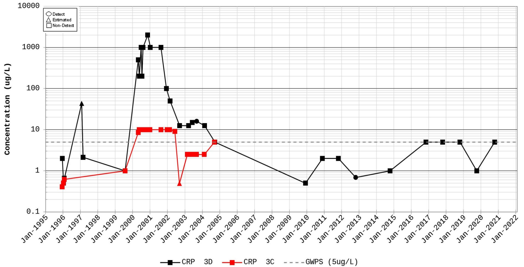
Time Series Plot for Dichloromethane (Methylene Chloride) Station for CRP 3
