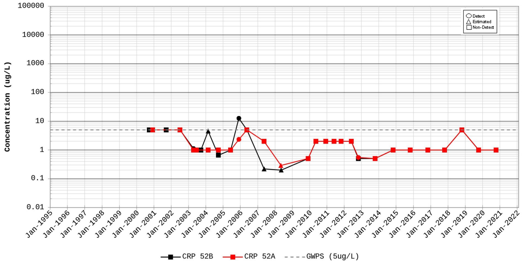
Figure C-116. Time Series Plot for Trichloroethylene (TCE) Station for CRP 52
