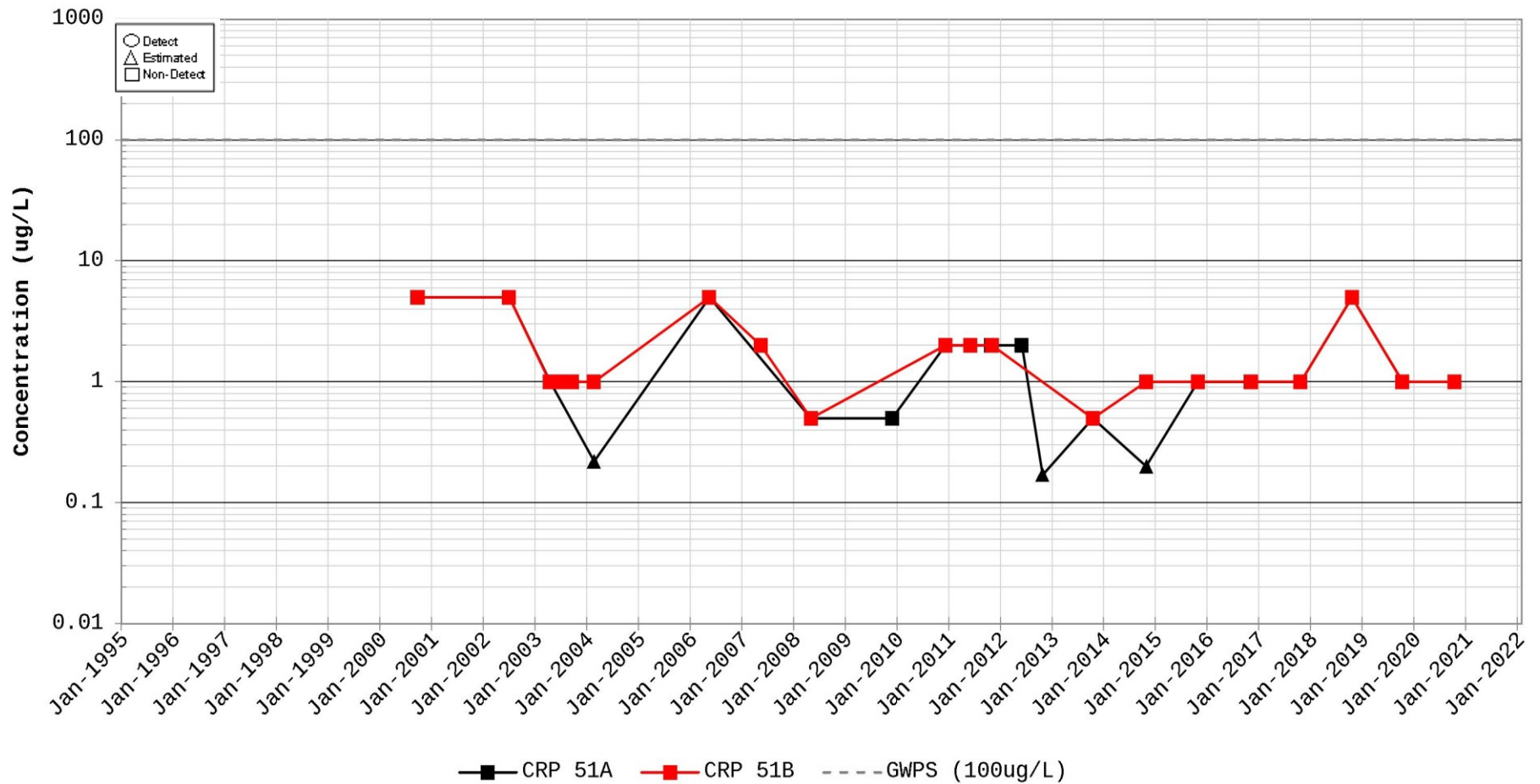
Time Series Plot for Trans-1,2-dichloroethylene Station for CRP 51
