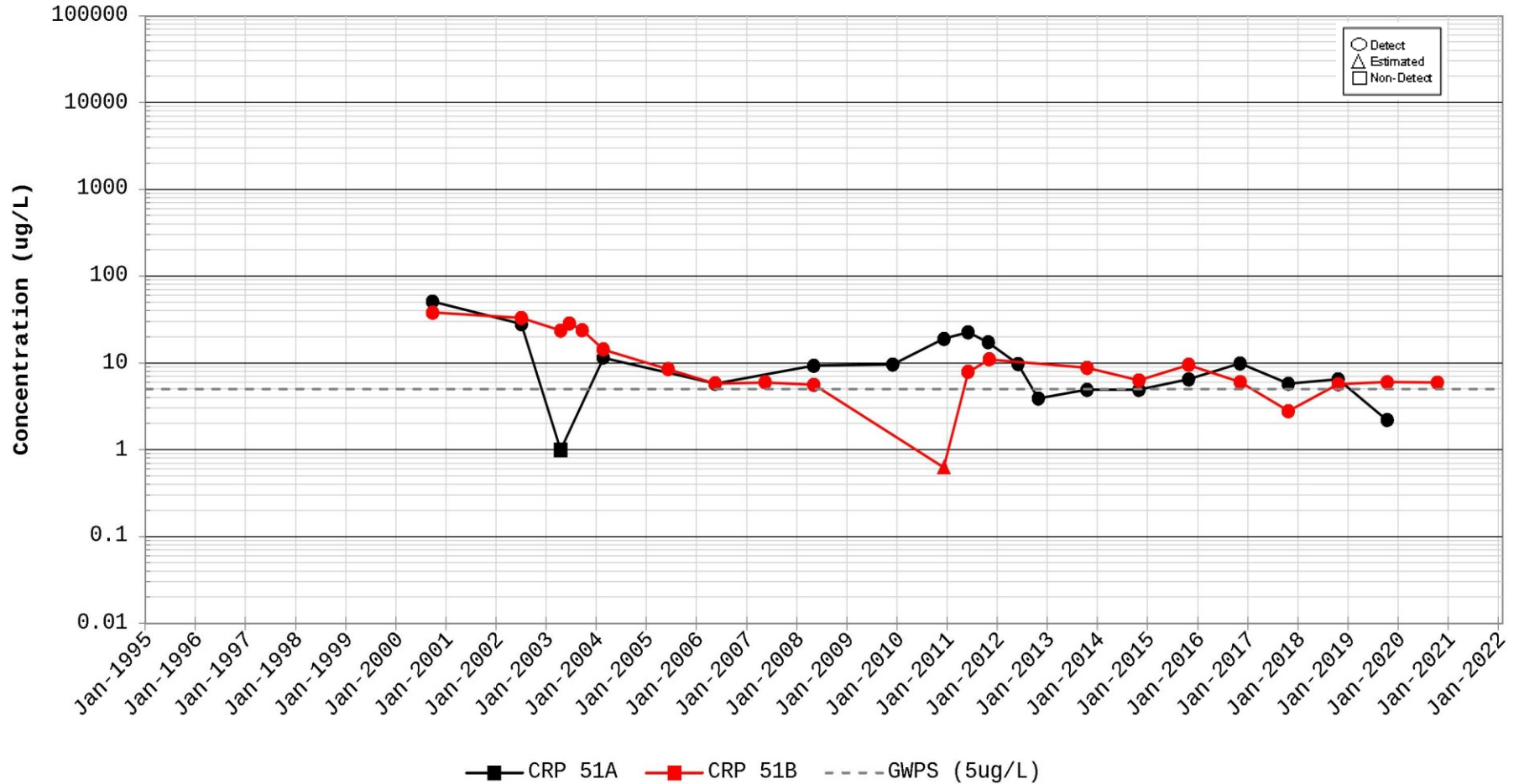
Figure C-115. Time Series Plot for Trichloroethylene (TCE) Station for CRP 51
