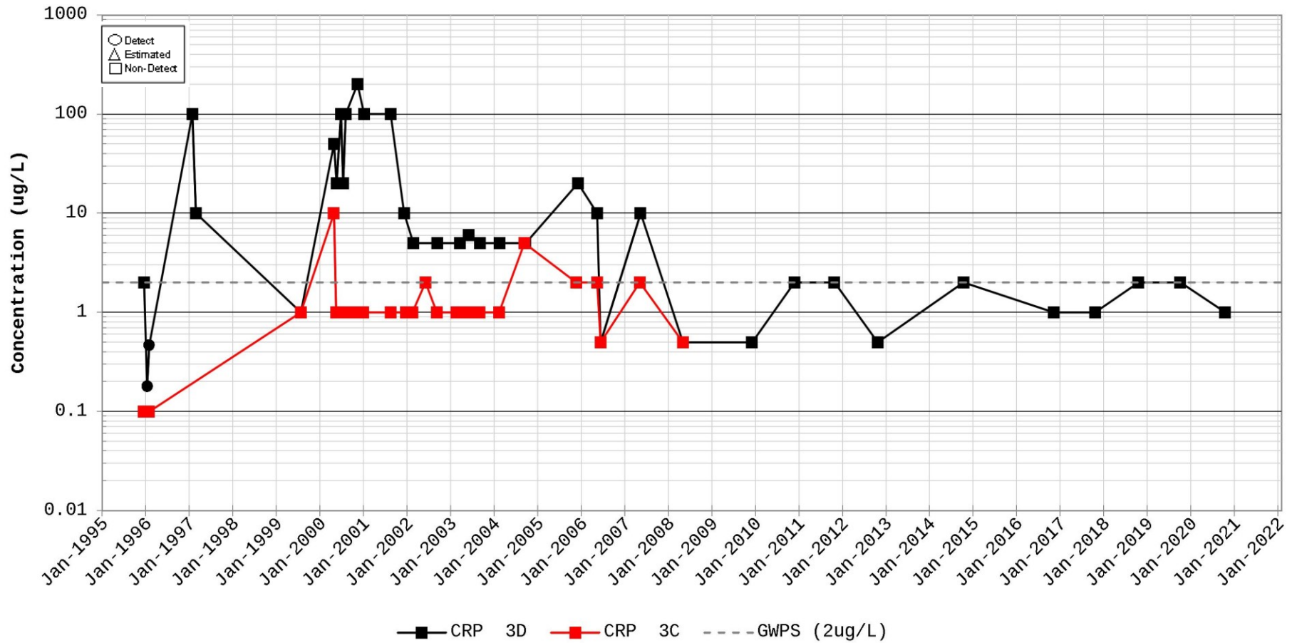
Time Series Plot for Chloroethene (Vinyl Chloride) Station for CRP 3
