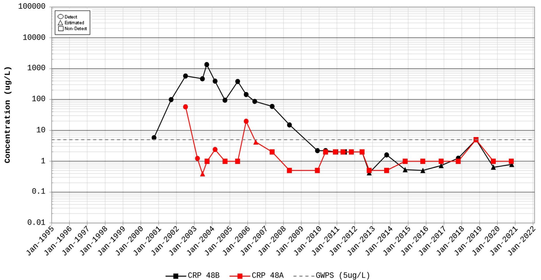
Figure C-113. Time Series Plot for Trichloroethylene (TCE) Station for CRP 48
