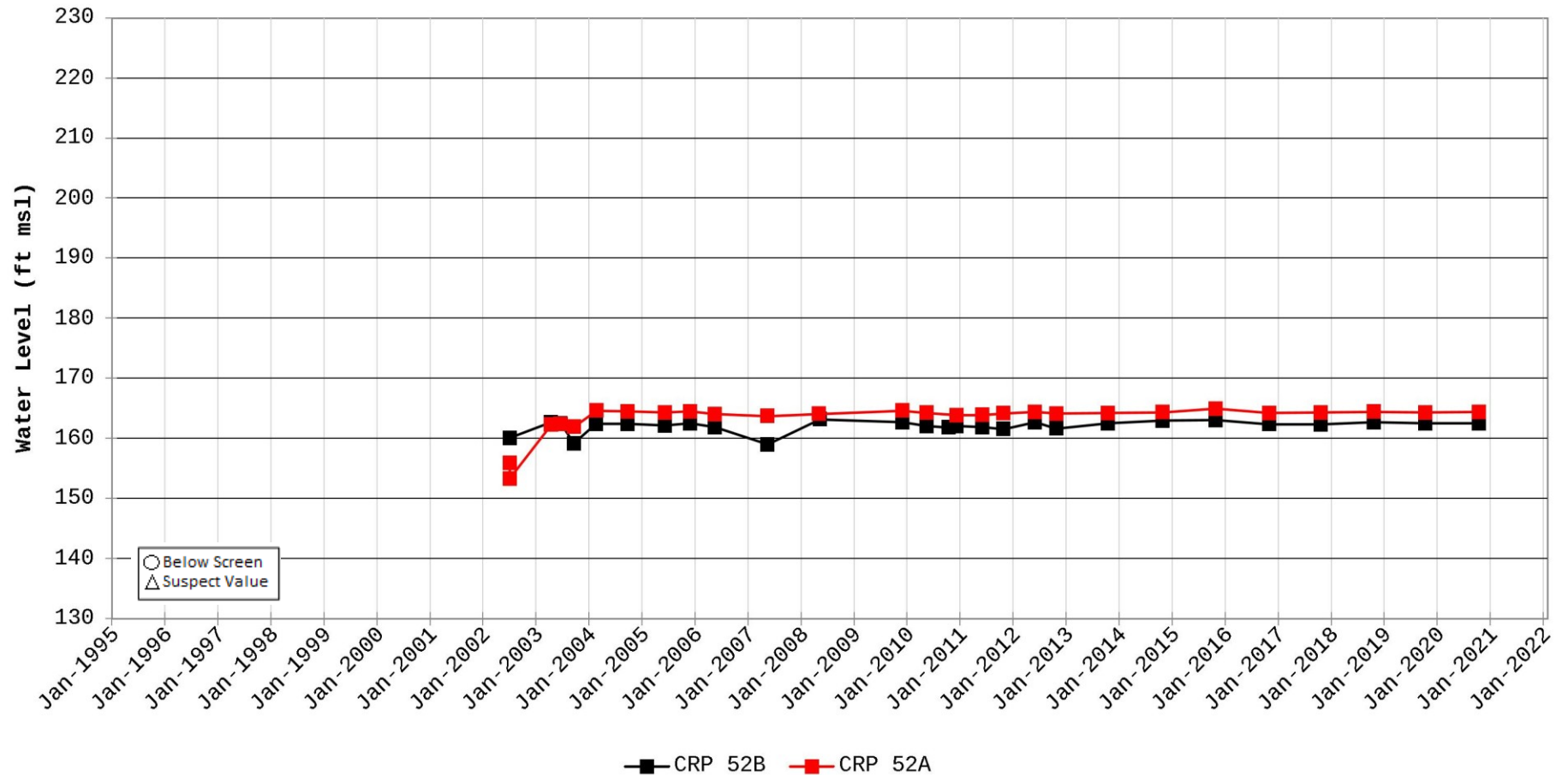
Hydrograph for Station CRP 52
