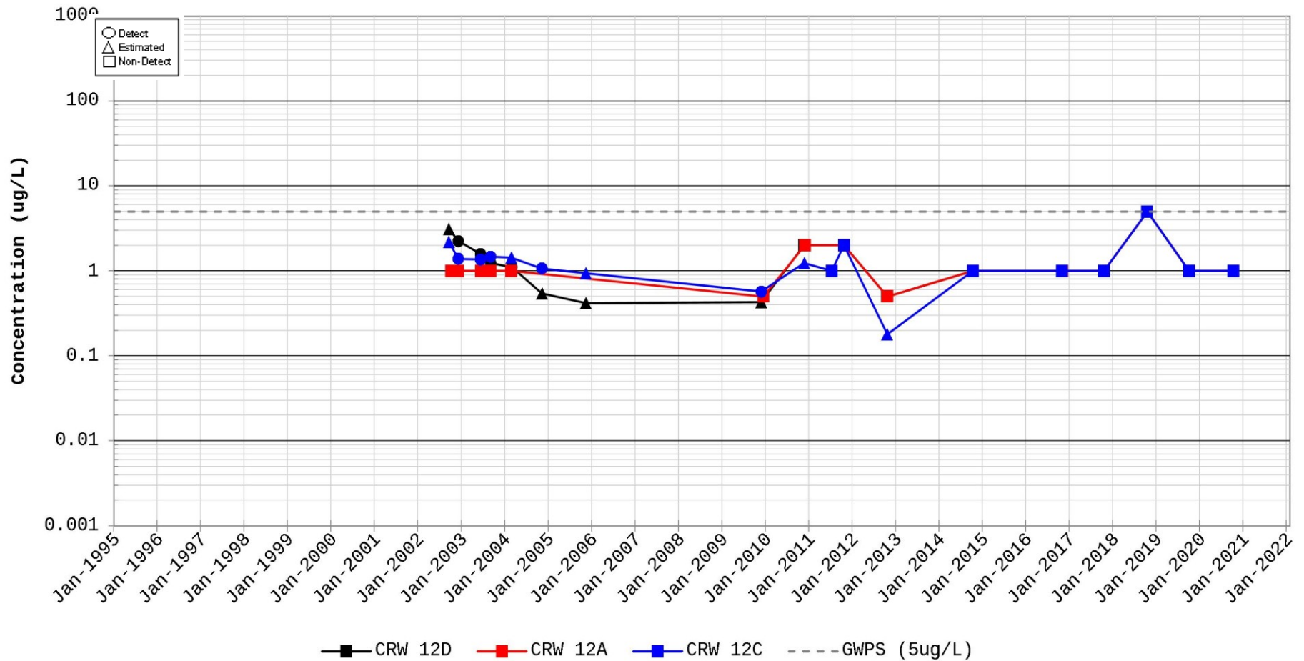
Figure C-86. Time Series Plot for Tetrachloroethylene (PCE) Station for CRW 12
