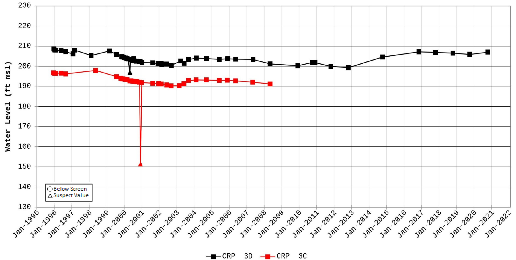
Hydrograph for Station CRP 3
