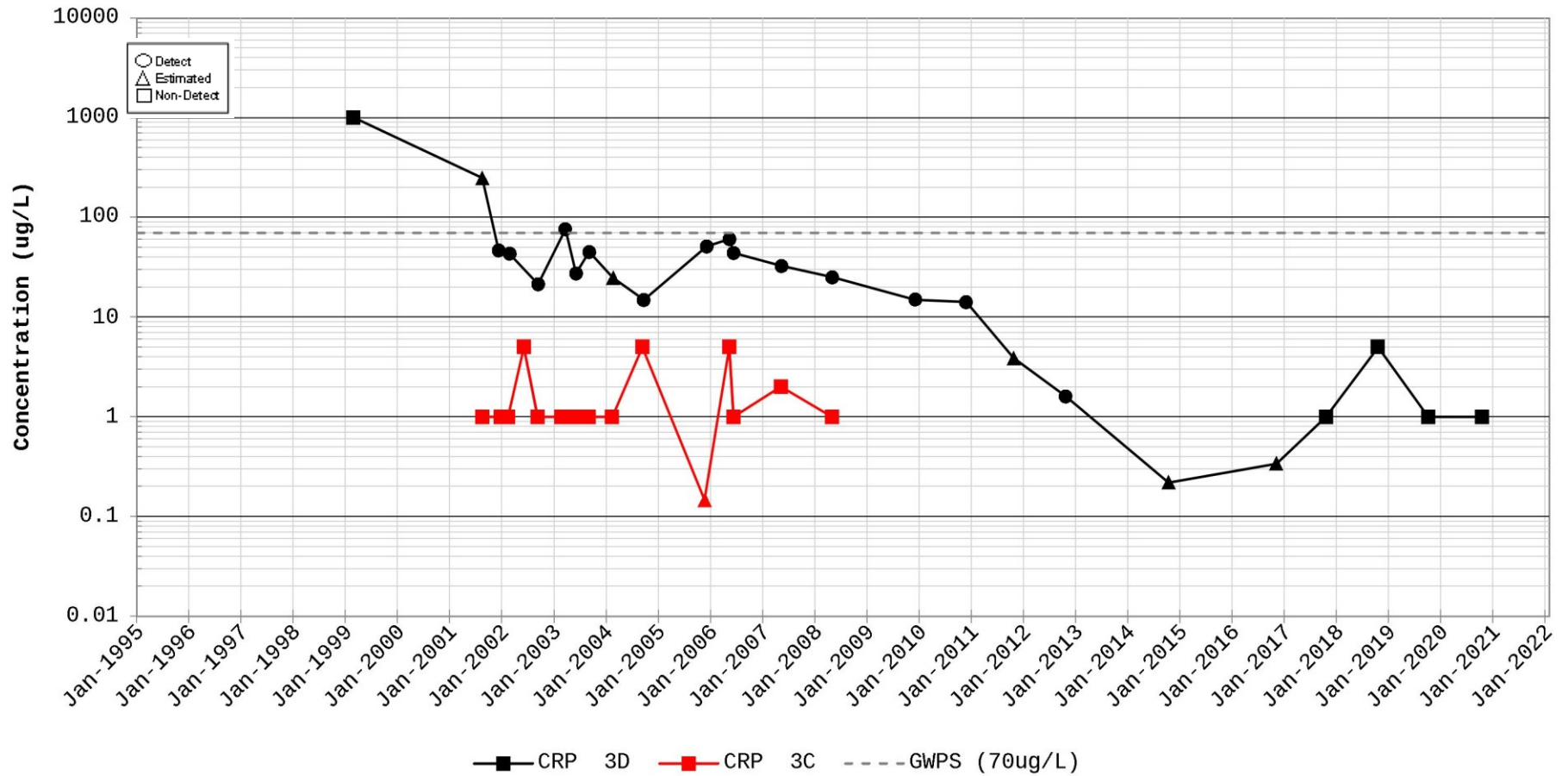
Time Series Plot for cis-1,2-Dichloroethylene Station for CRP 3
