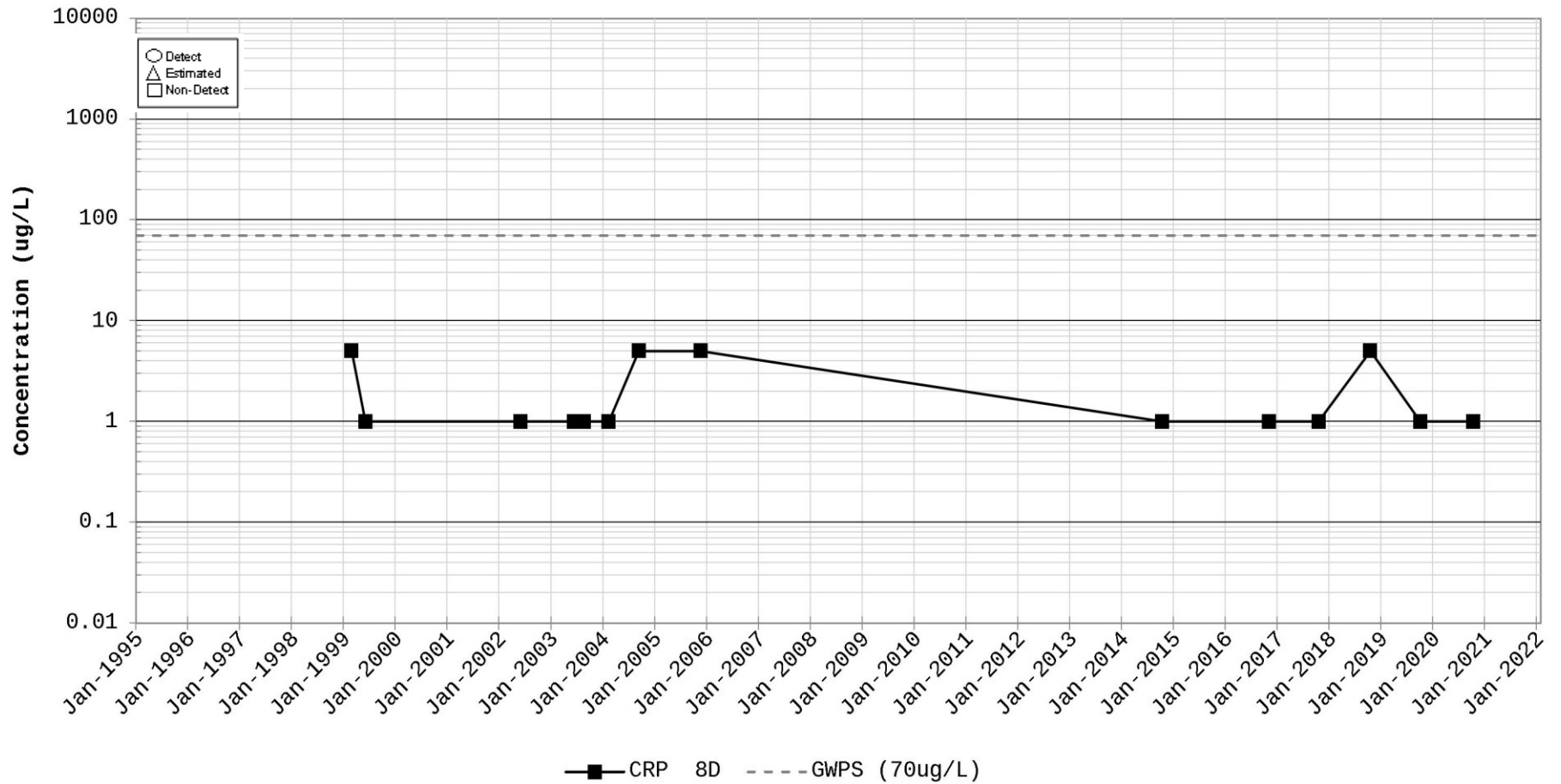
Time Series Plot for cis-1,2-Dichloroethylene Station for CRP 8
