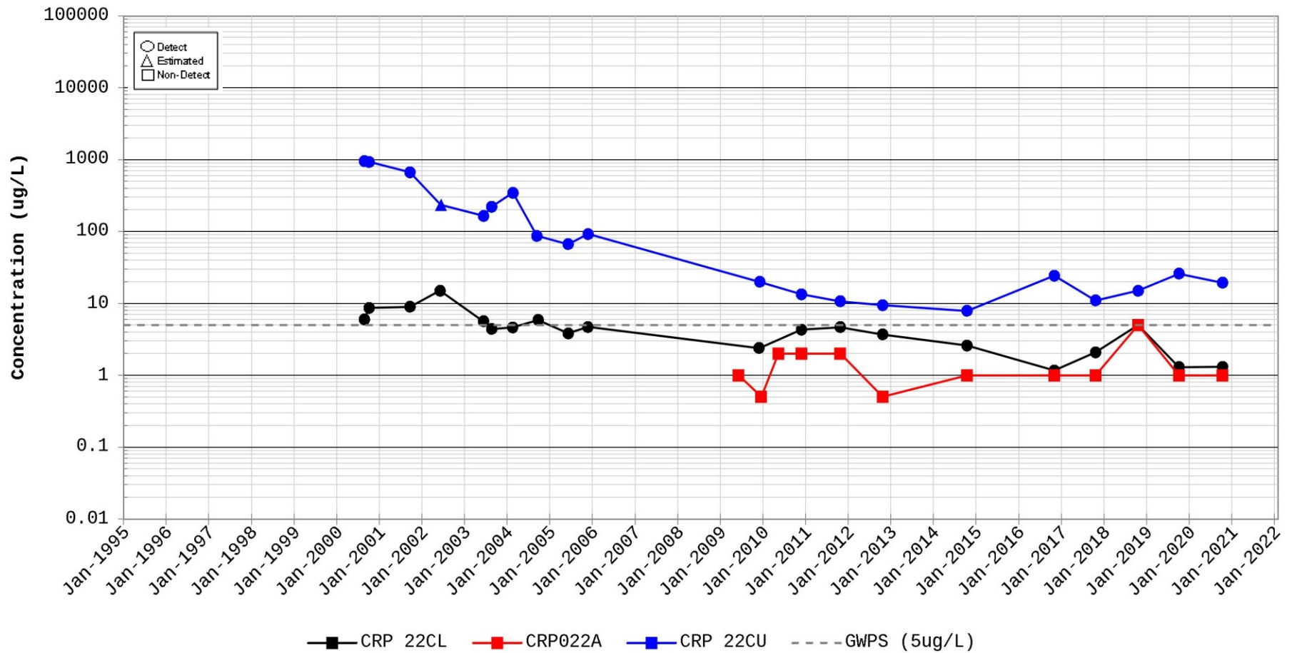
Figure C-110. Time Series Plot for Trichloroethylene (TCE) Station for CRP 22
