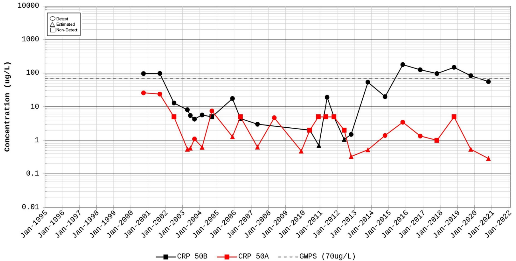
Time Series Plot for cis-1,2-Dichloroethylene Station for CRP 50
