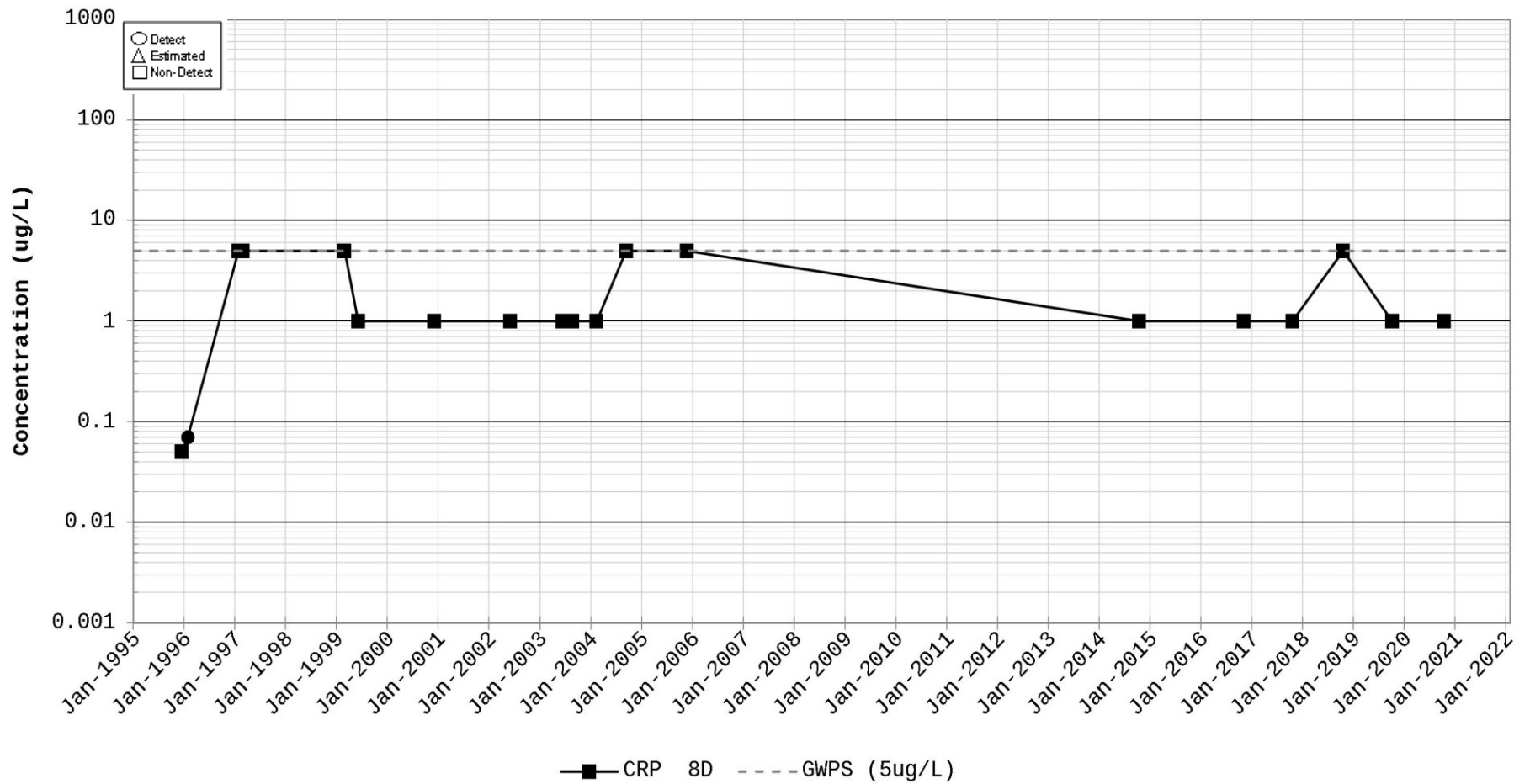
Time Series Plot for Tetrachloroethylene (PCE) Station for CRP 8
