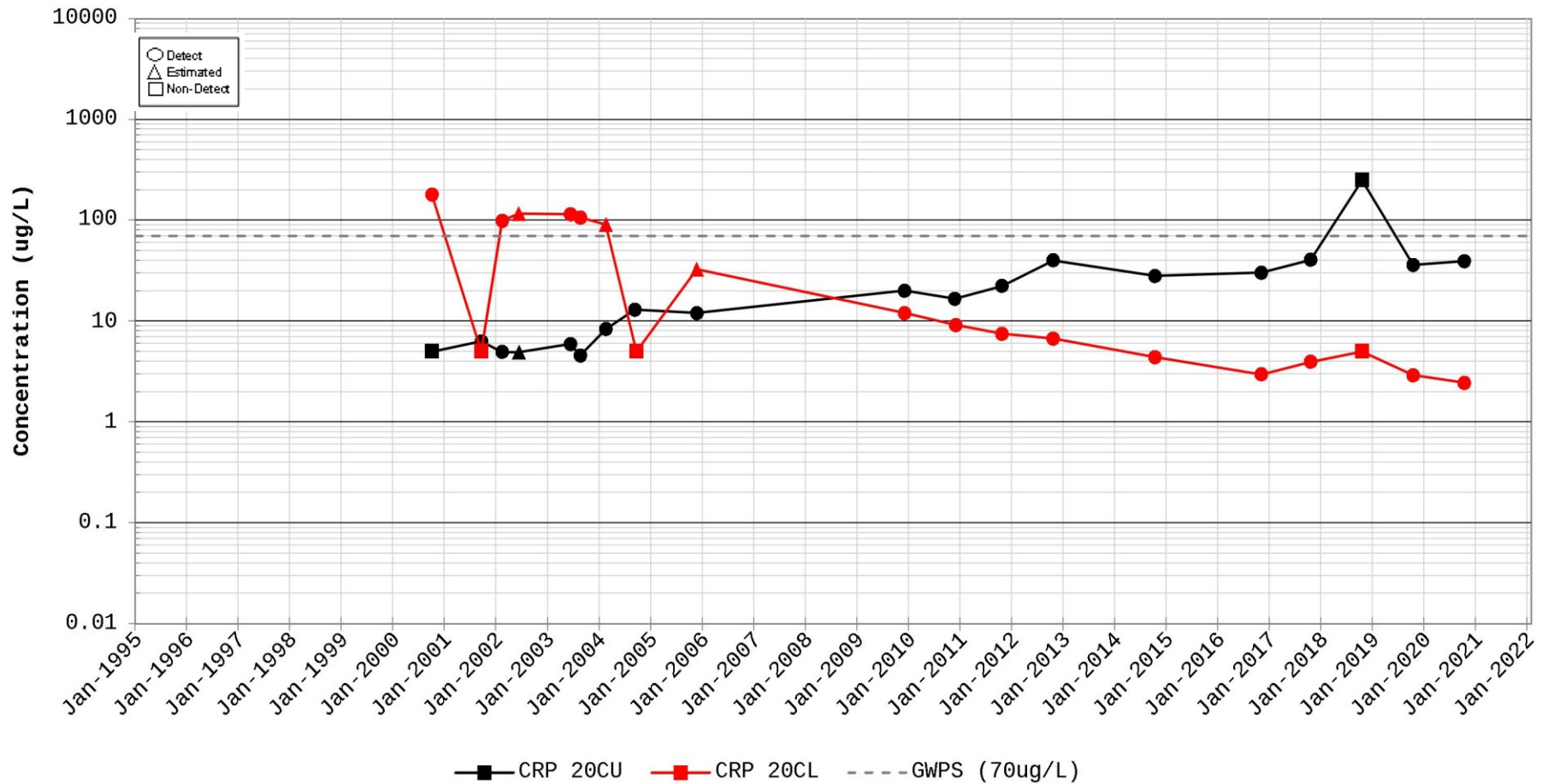
Time Series Plot for cis-1,2-Dichloroethylene Station for CRP 20
