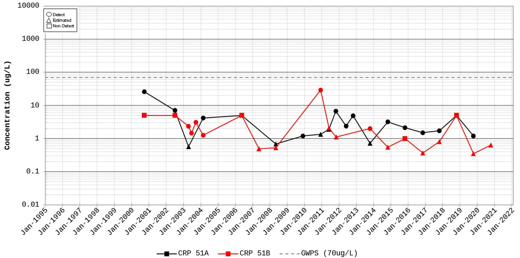
Time Series Plot for cis-1,2-Dichloroethylene Station for CRP 51
