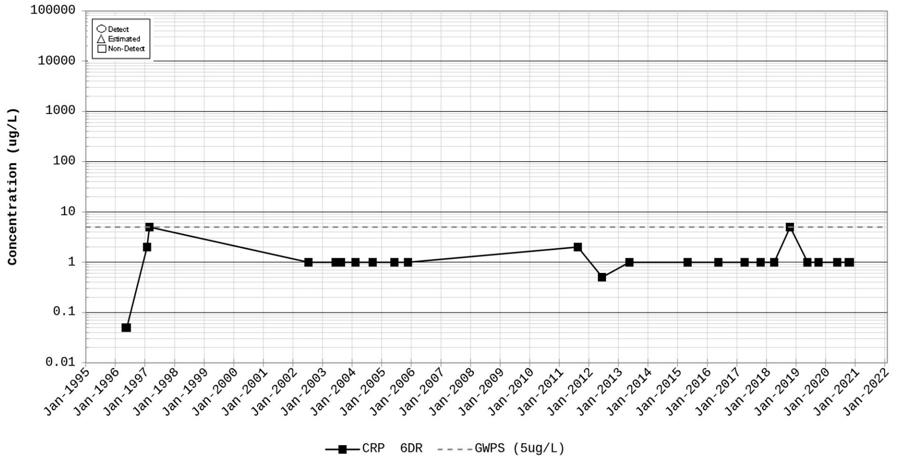
Time Series Plot for Trichloroethylene (TCE) Station for CRP 6
