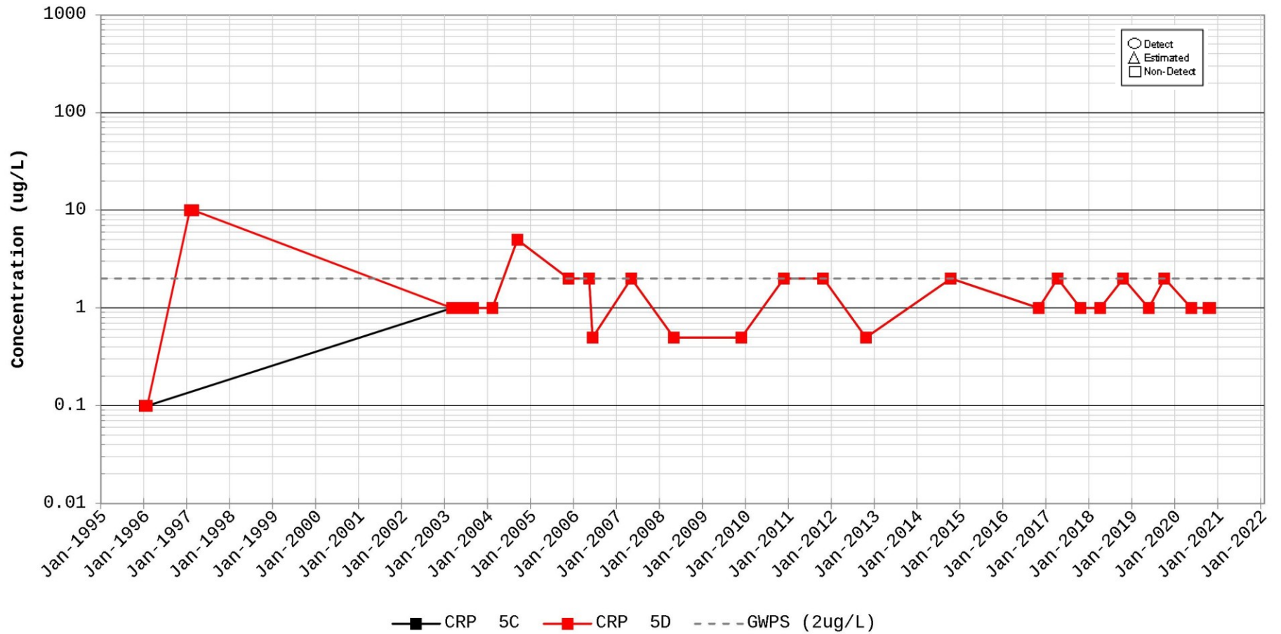
Time Series Plot for Chloroethene (Vinyl Chloride) Station for CRP 5
