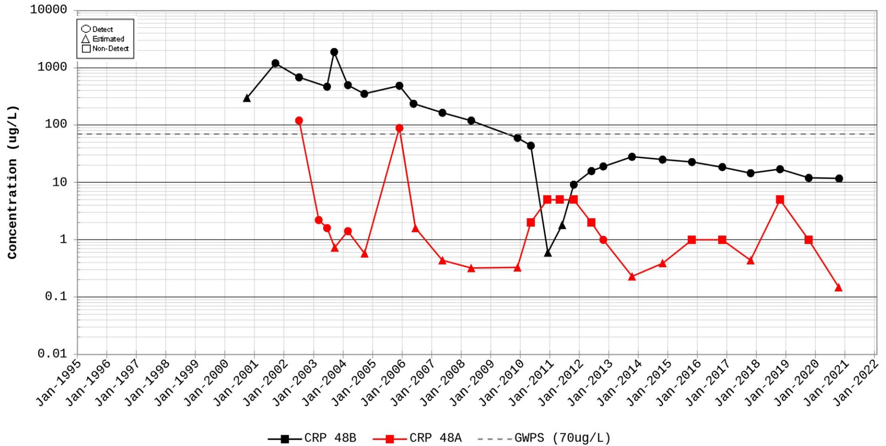
Time Series Plot for cis-1,2-Dichloroethylene Station for CRP 48
