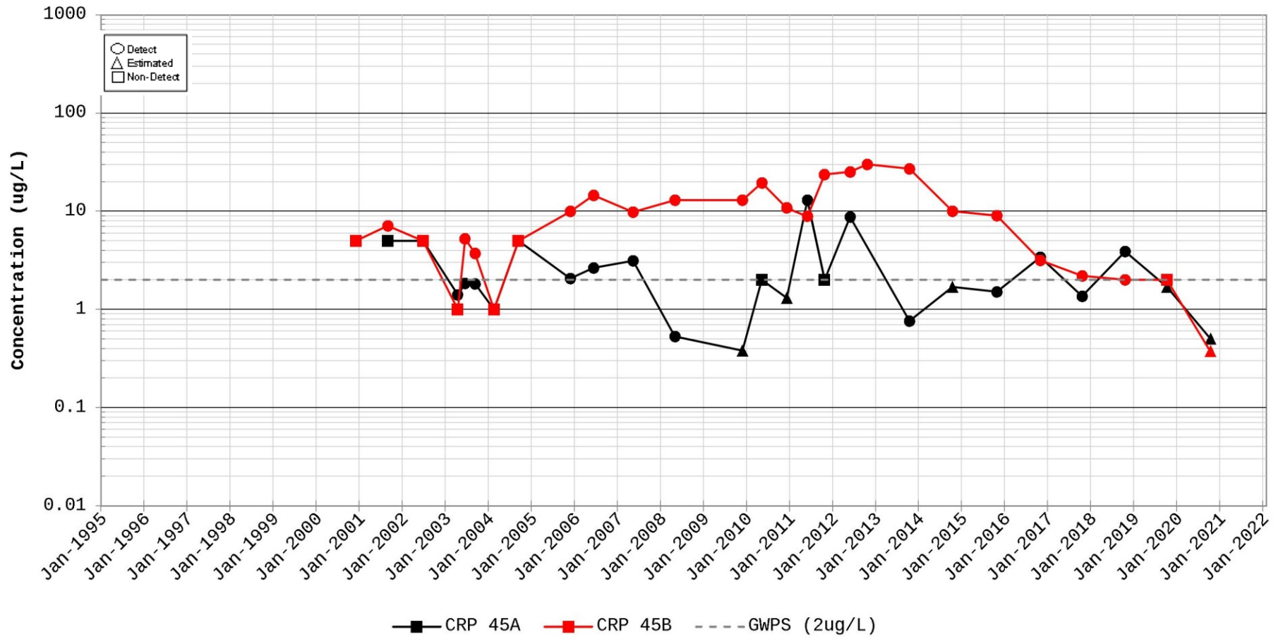
Time Series Plot for Chloroethene (Vinyl Chloride) Station for CRP 45
