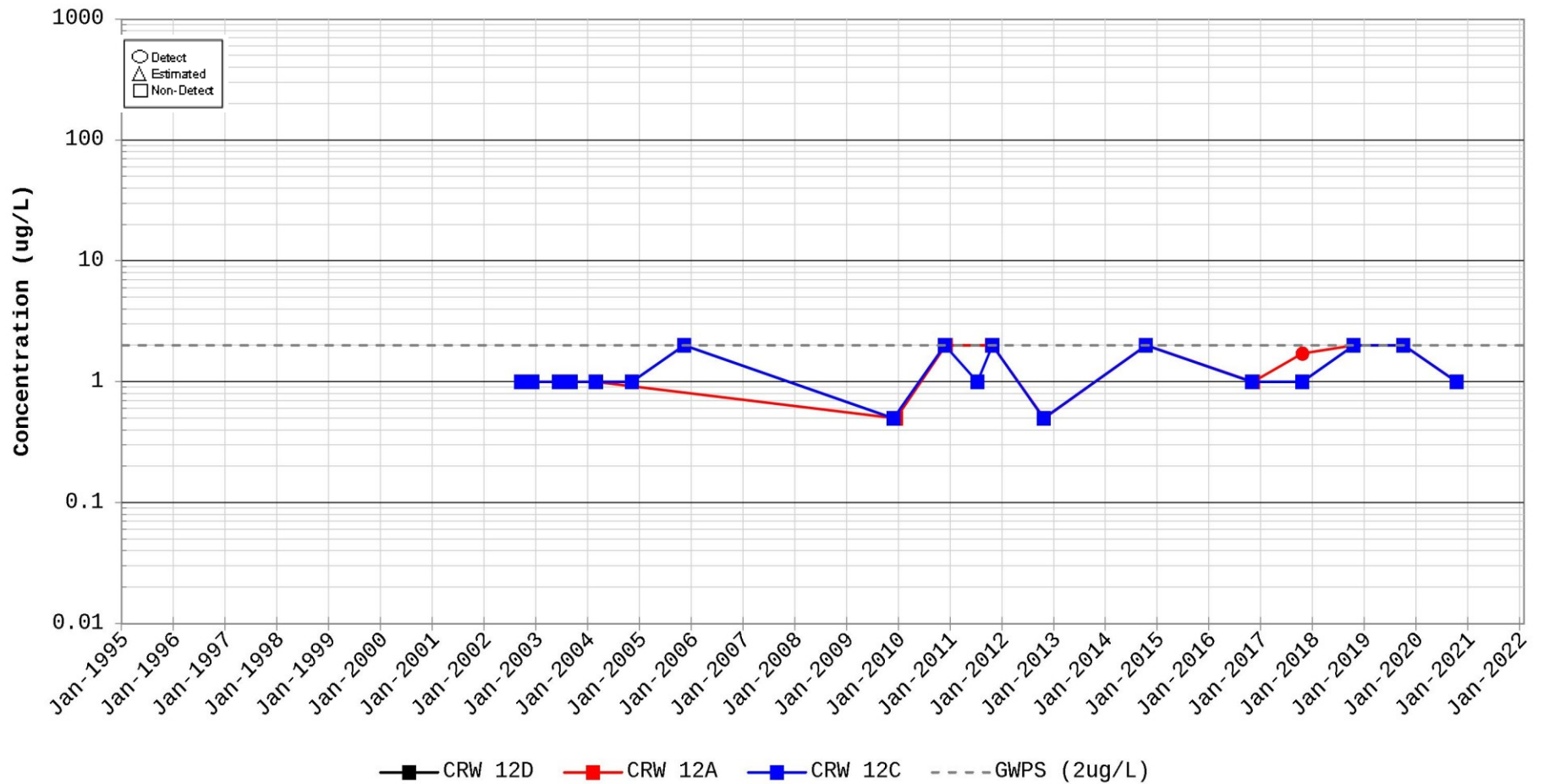
Figure C-32. Time Series Plot for Chloroethene (Vinyl Chloride) Station for CRW 12
