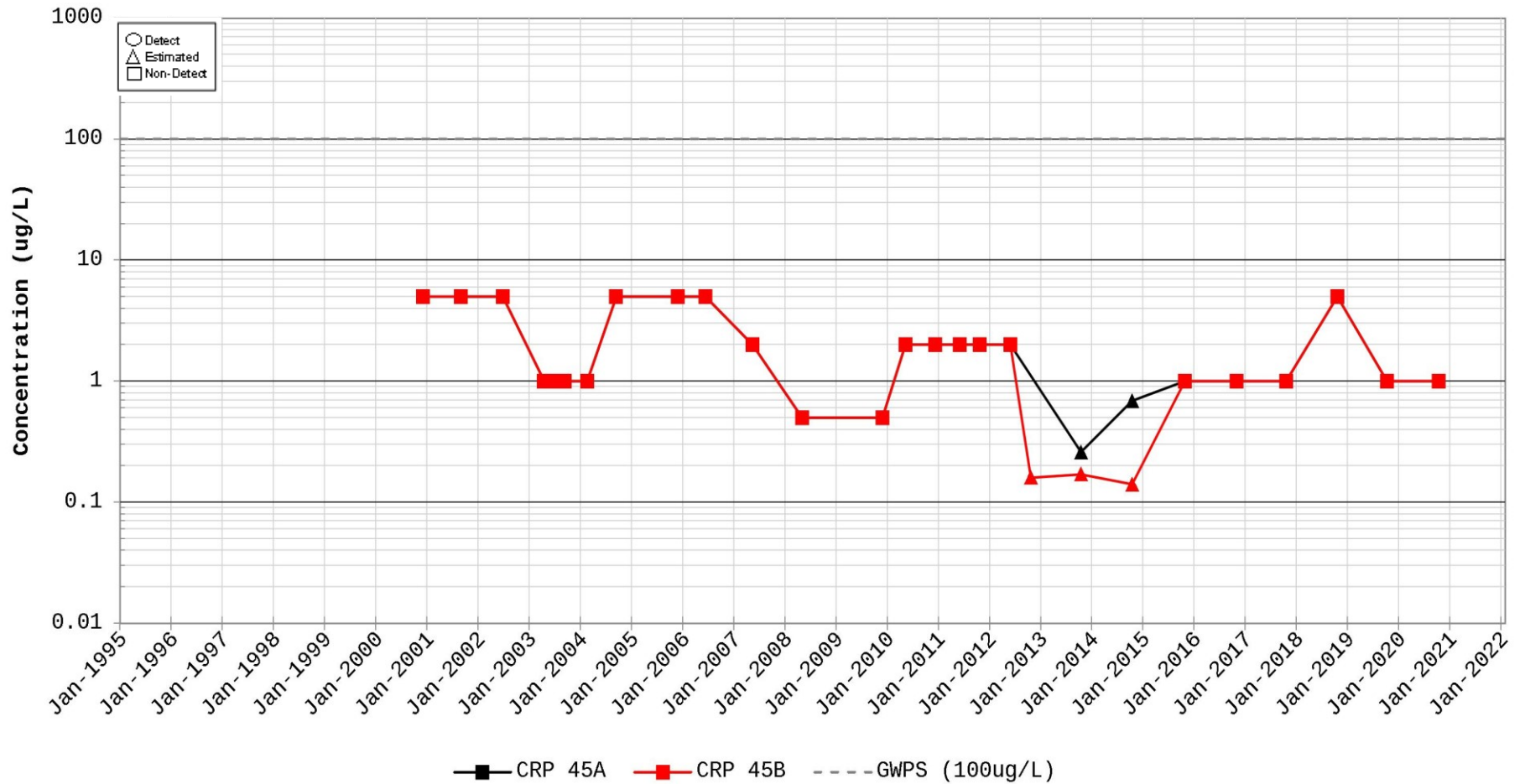
Time Series Plot for Trans-1,2-dichloroethylene Station for CRP 45
