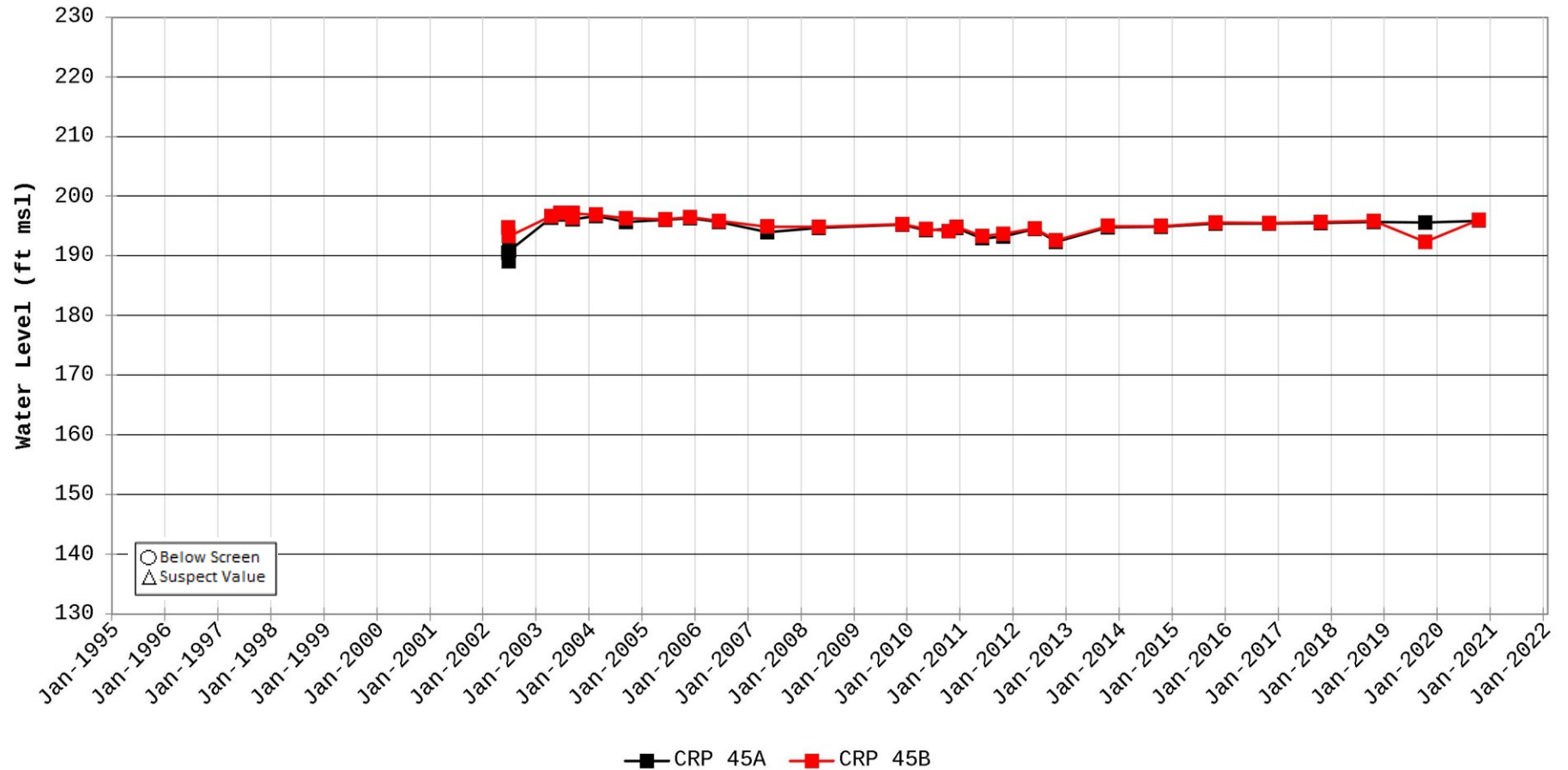
Hydrograph for Station CRP 45
