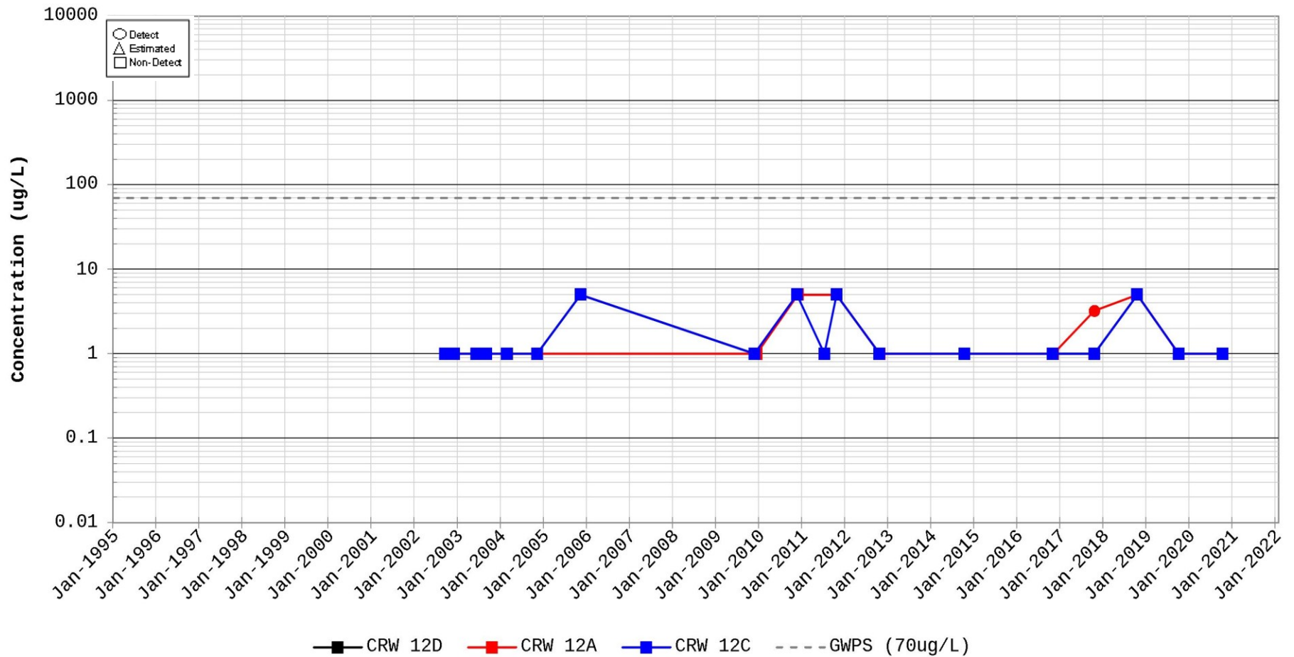
Time Series Plot for cis-1,2-Dichloroethylene Station for CRW 12
