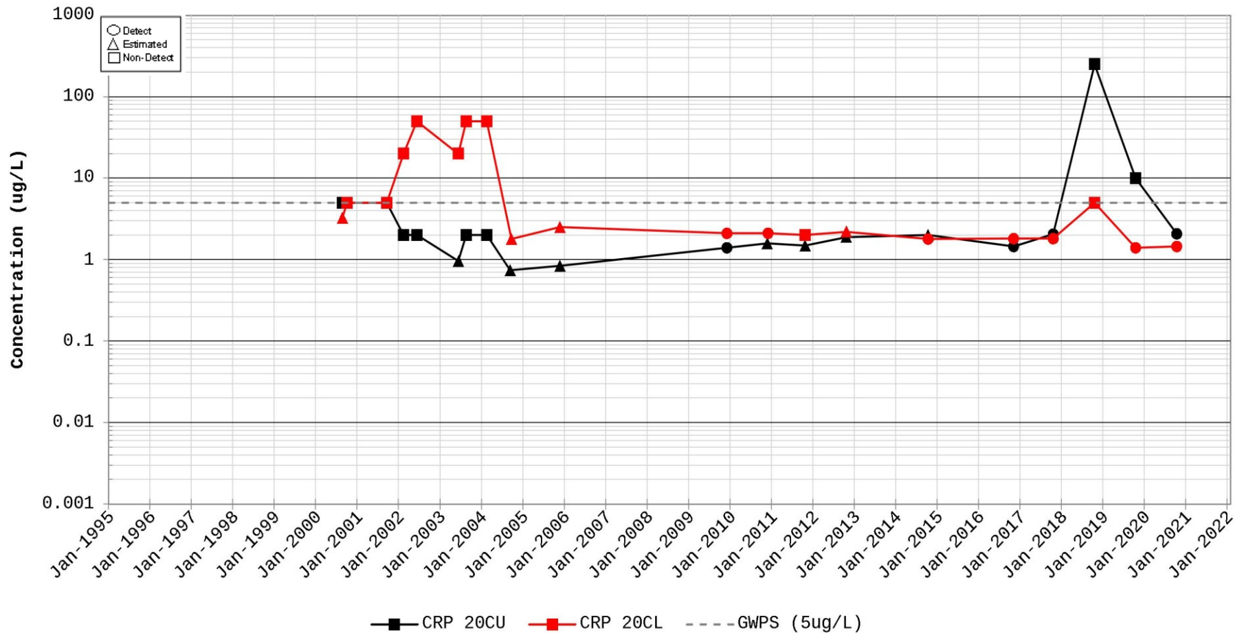
Time Series Plot for Tetrachloroethylene (PCE) Station for CRP 20
