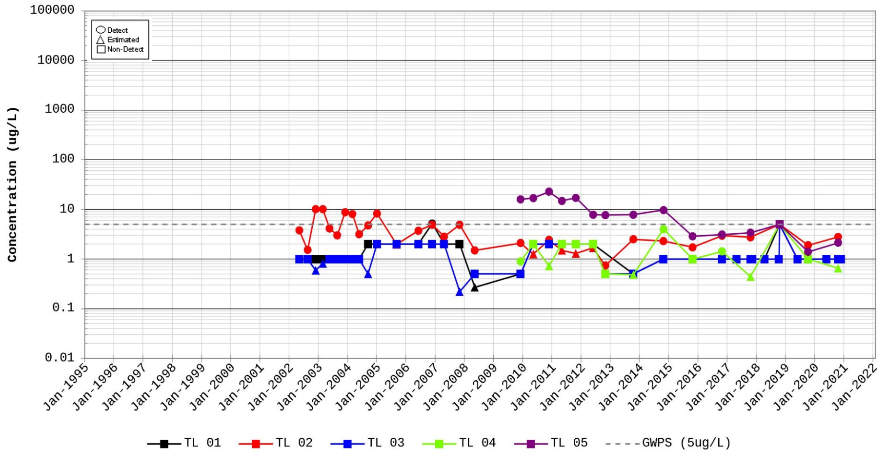
Figure C-119. Time Series Plot for Trichloroethylene (TCE) Station for TL 01
