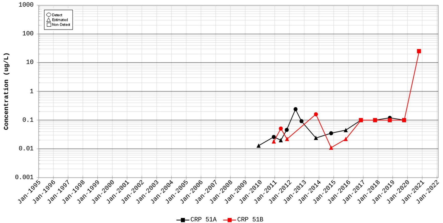
Time Series Plot for ETHYLENE Station for CRP 51
