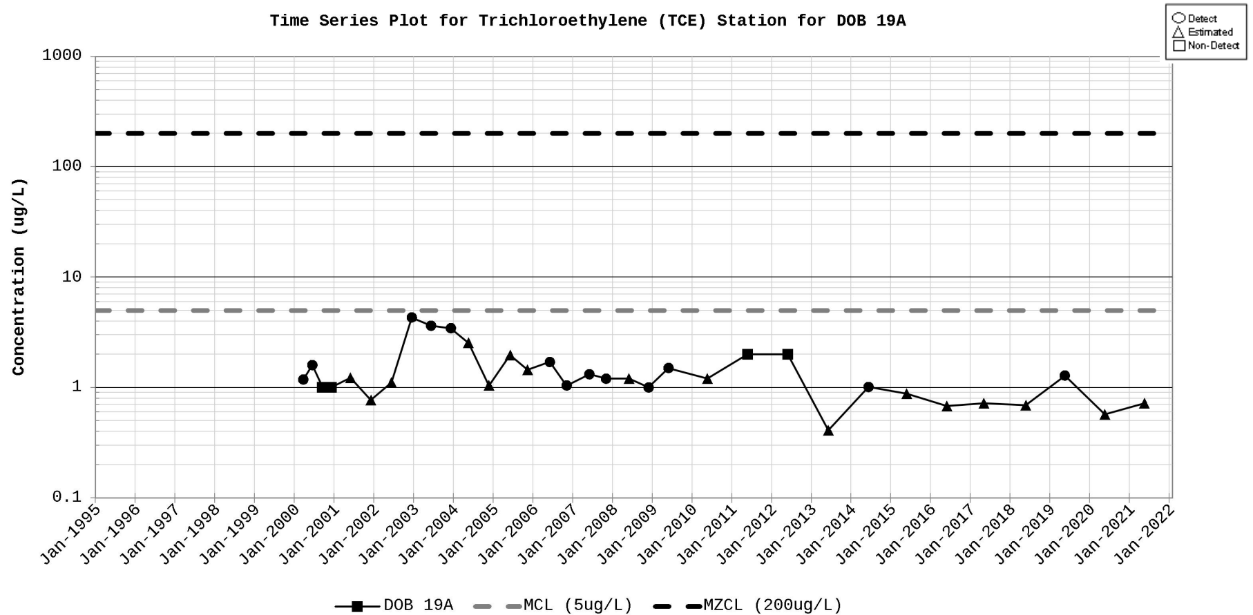
Figure D-81. Time Series Plot for Trichloroethylene (TCE) Station for DOB 19A
