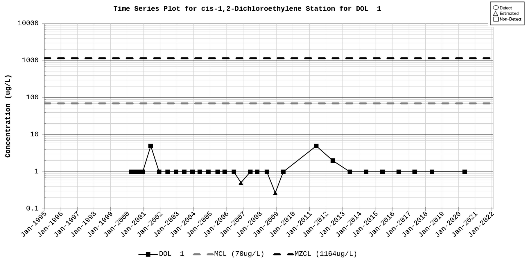
Figure D-45. Time Series Plot for cis-1,2-Dichloroethylene Station for DOL 1
