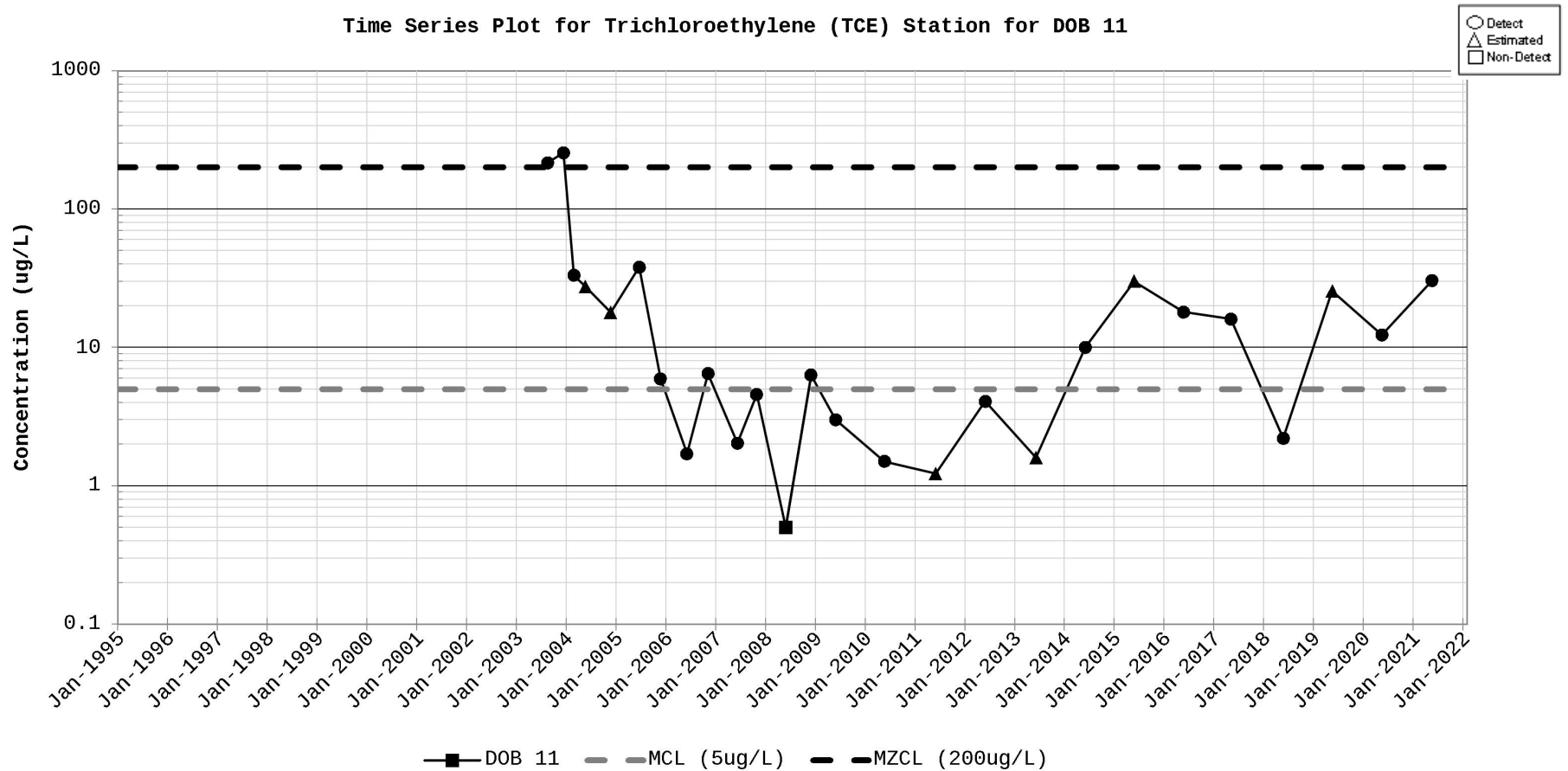
Figure D-71. Time Series Plot for Trichloroethylene (TCE) Station for DOB 11
