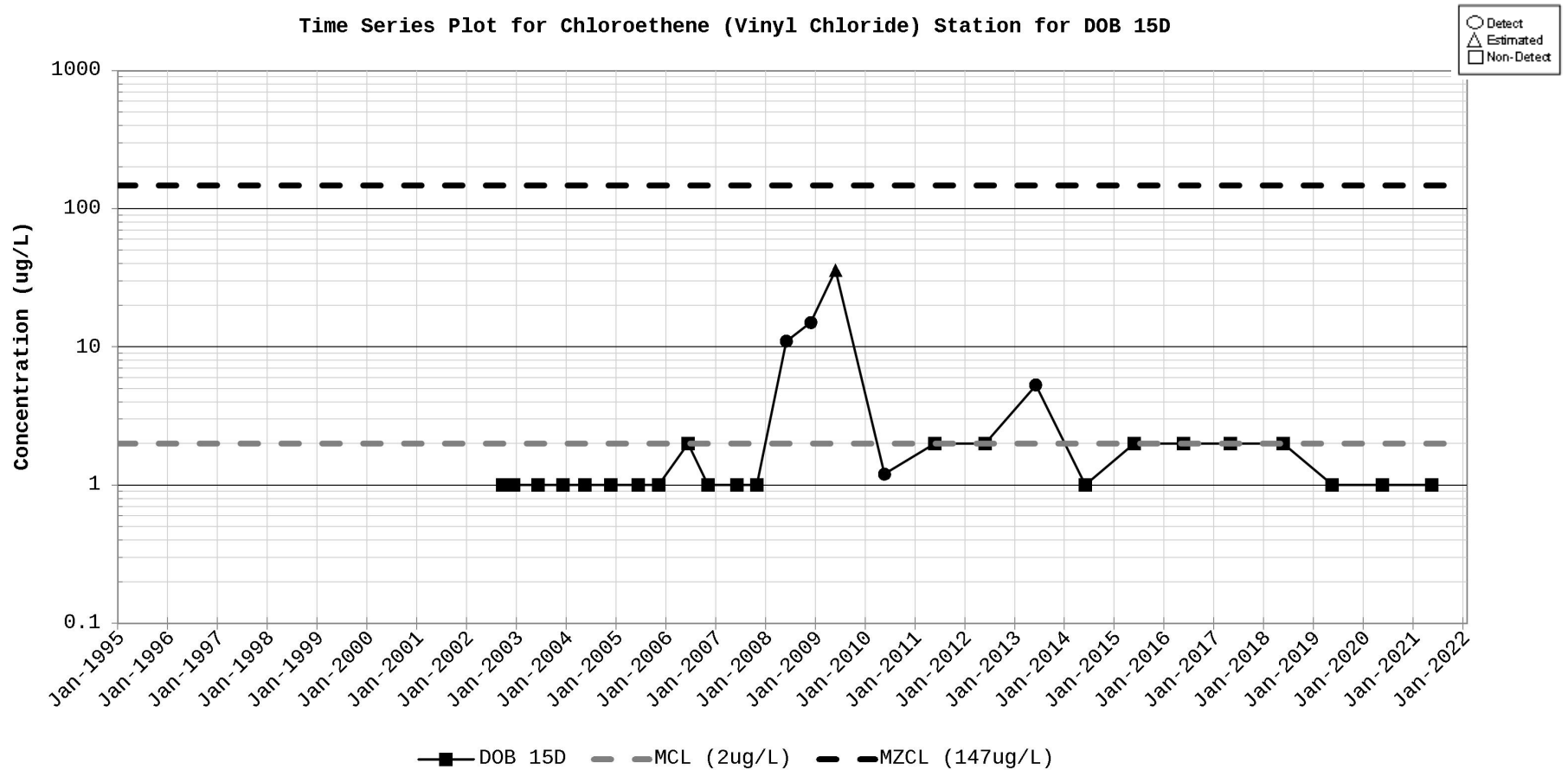
Figure D-9. Time Series Plot for Chloroethene (Vinyl chloride) Station for DOB 15D
