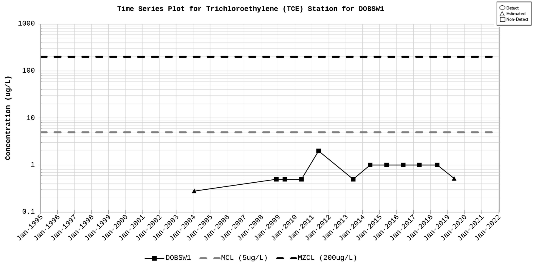
Figure D-90. Time Series Plot for Trichloroethylene (TCE) Station for DOBSW1
