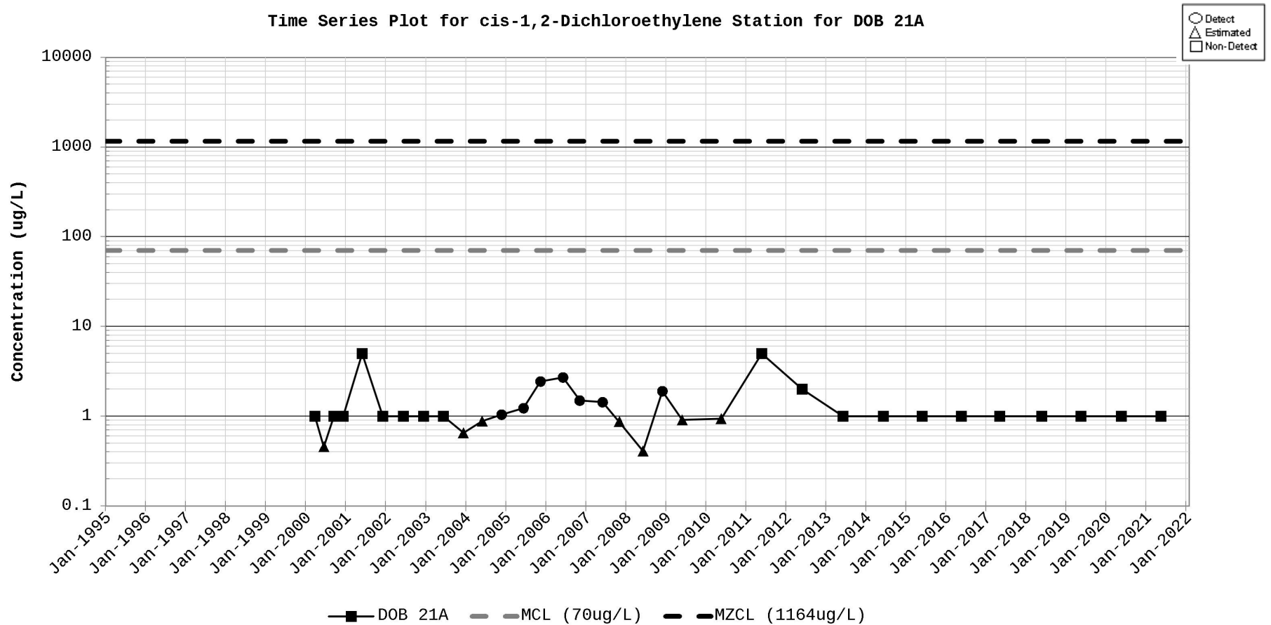
Figure D-38. Time Series Plot for cis-1,2-Dichloroethylene Station for DOB 21A
