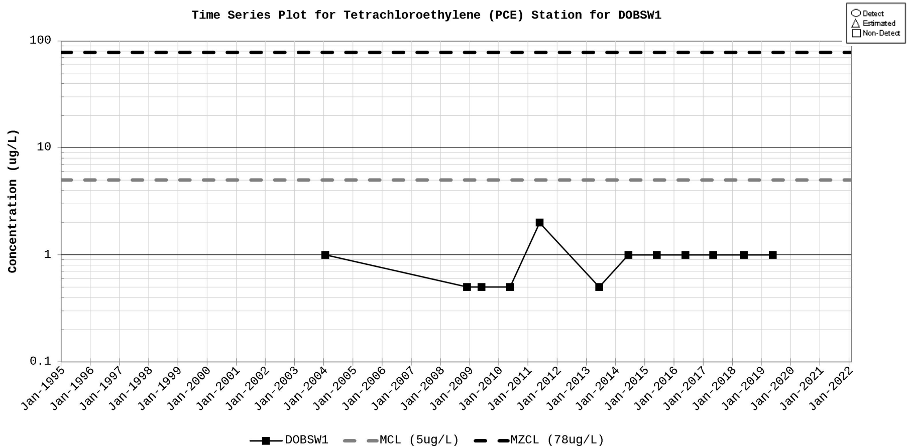
Figure D-67. Time Series Plot for Tetrachloroethylene (PCE) Station for DOBSW1
