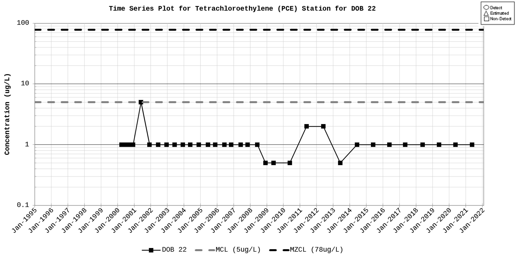
Figure D-65. Time Series Plot for Tetrachloroethylene (PCE) Station for DOB 22
