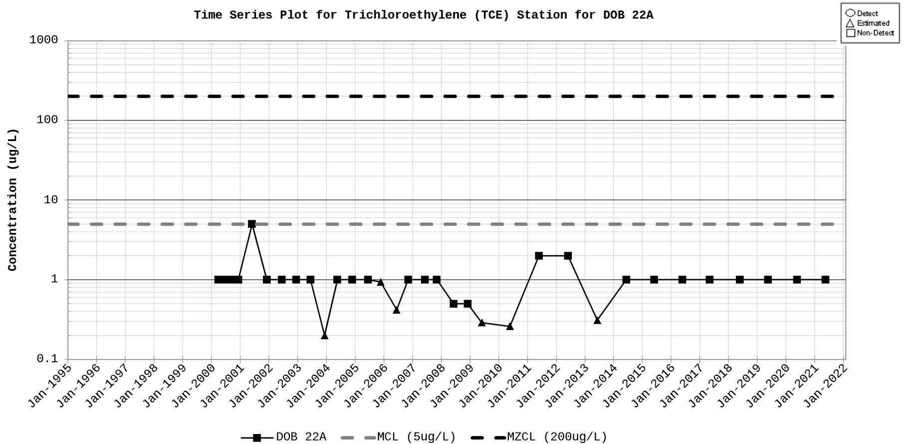
Figure D-87. Time Series Plot for Trichloroethylene (TCE) Station for DOB 22A
