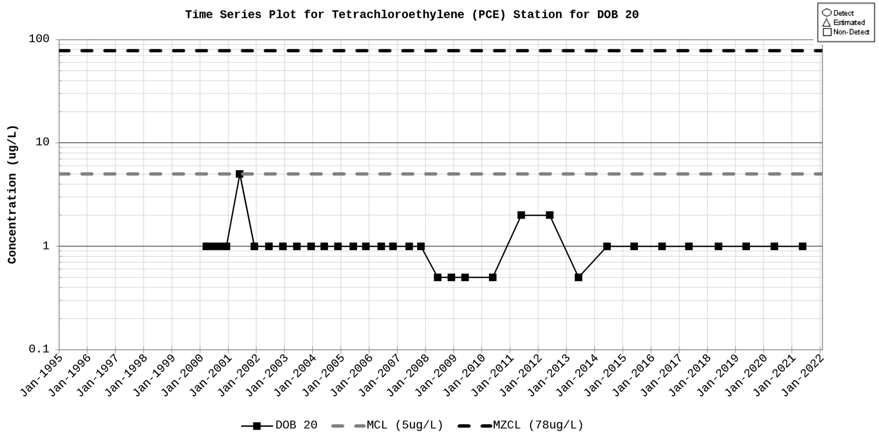
Figure D-60. Time Series Plot for Tetrachloroethylene (PCE) Station for DOB 20
