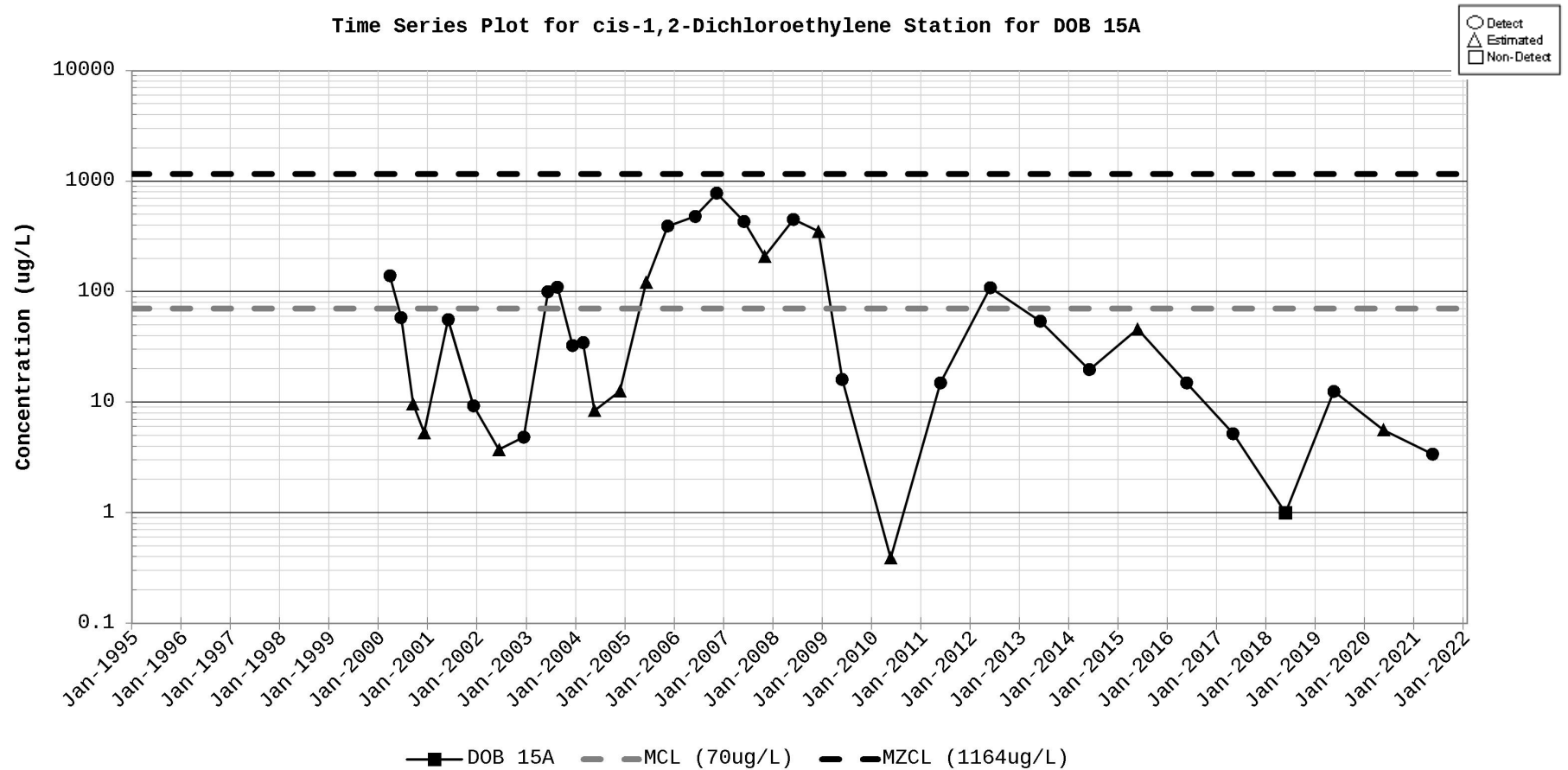
Figure D-30. Time Series Plot for cis-1,2-Dichloroethylene Station for DOB 15A
