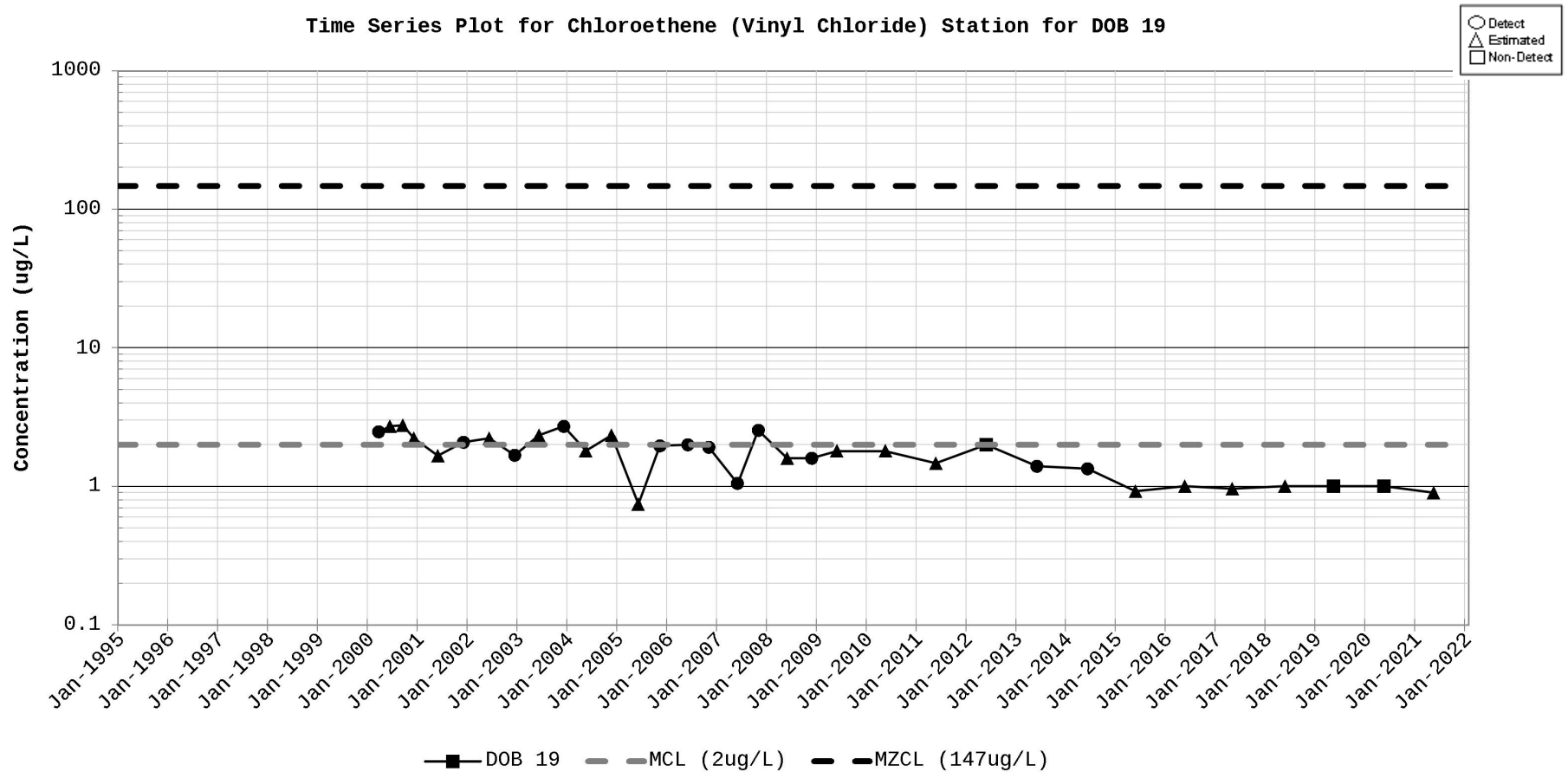
Figure D-11. Time Series Plot for Chloroethene (Vinyl chloride) Station for DOB 19
