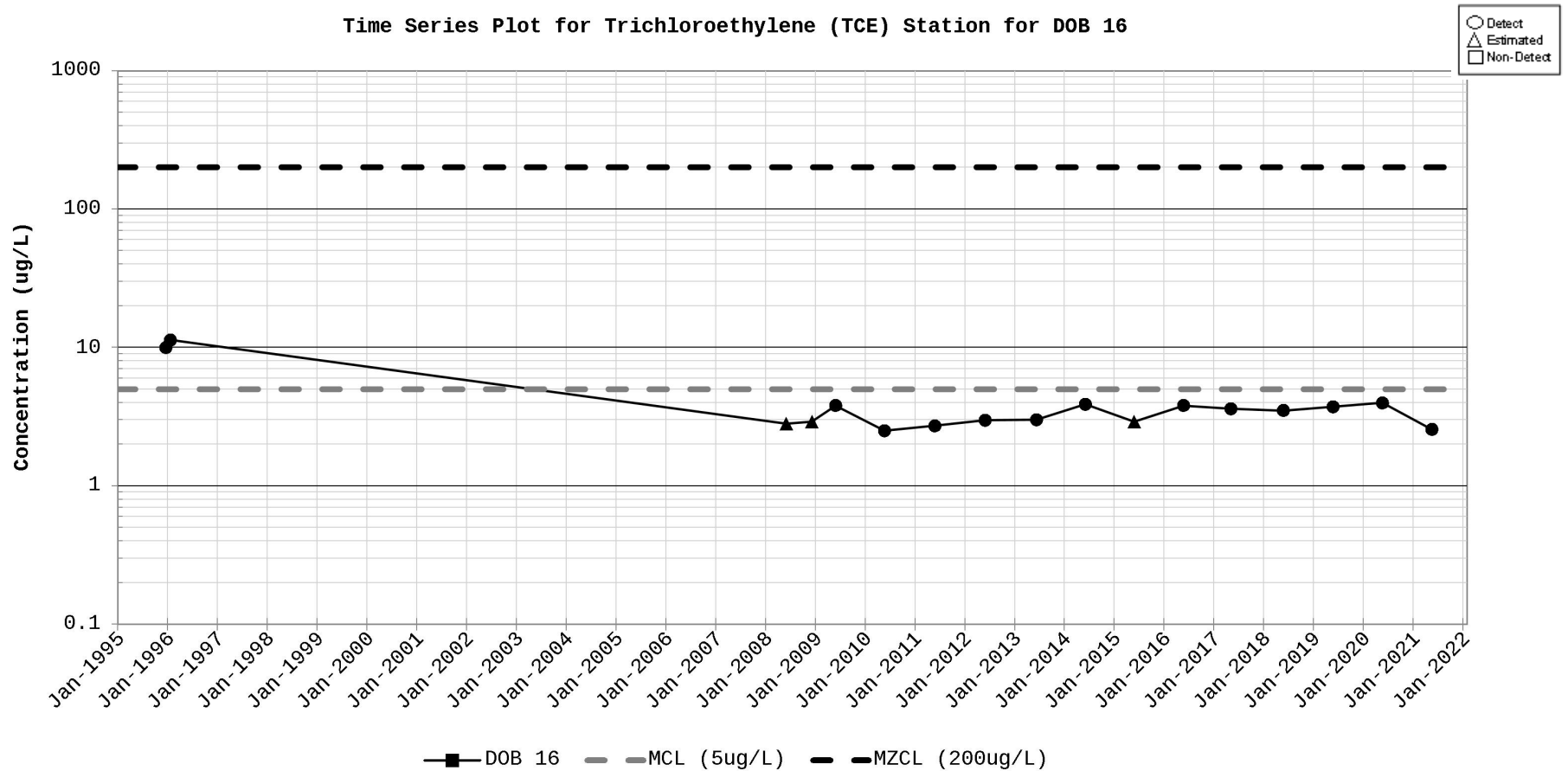
Figure D-79. Time Series Plot for Trichloroethylene (TCE) Station for DOB 16
