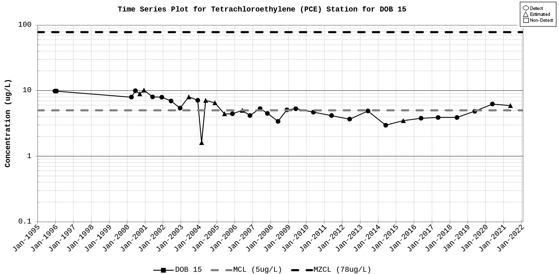
Figure D-52. Time Series Plot for Tetrachloroethylene (PCE) Station for DOB 15
