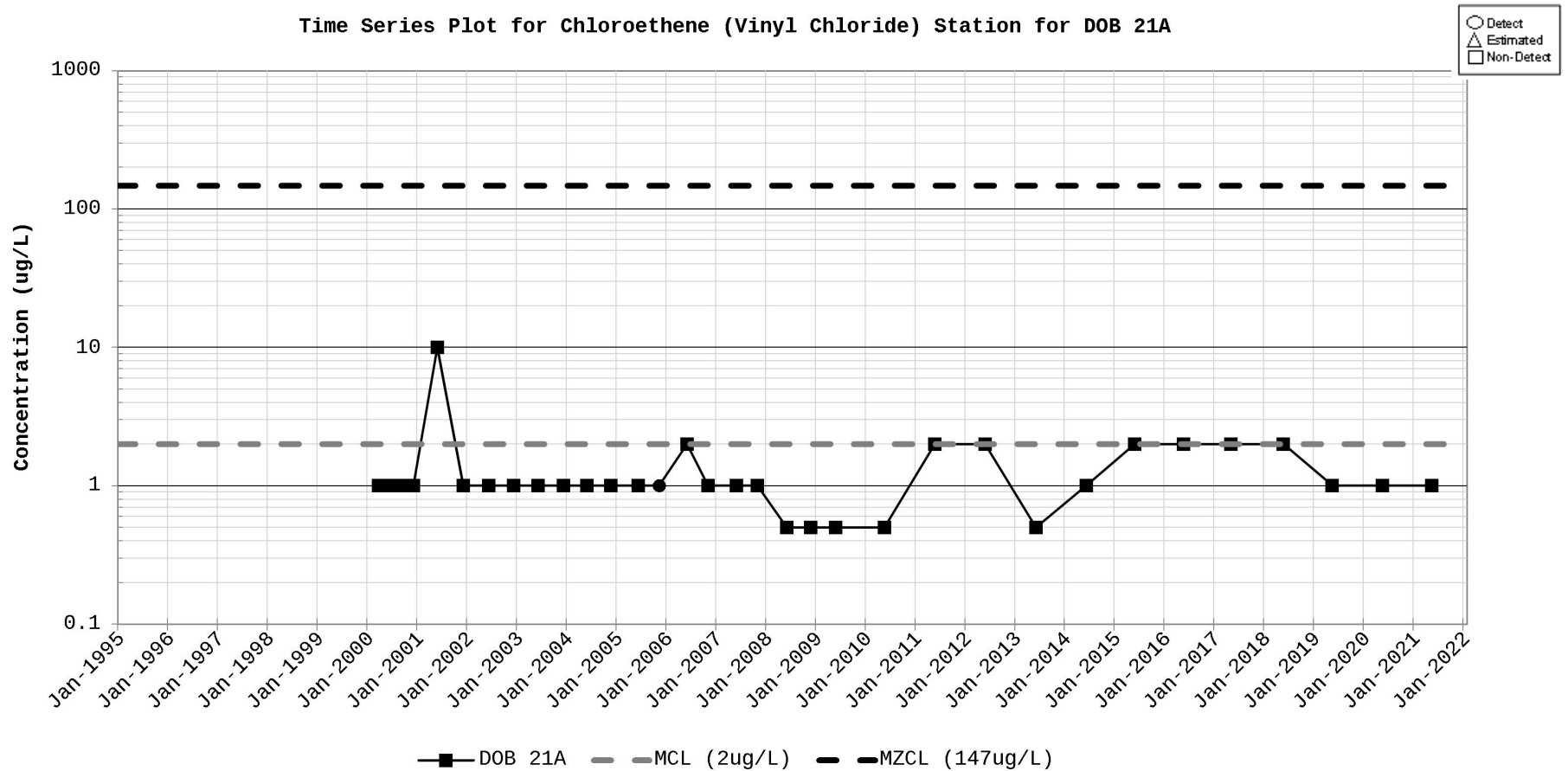
Figure D-15. Time Series Plot for Chloroethene (Vinyl chloride) Station for DOB 21A
