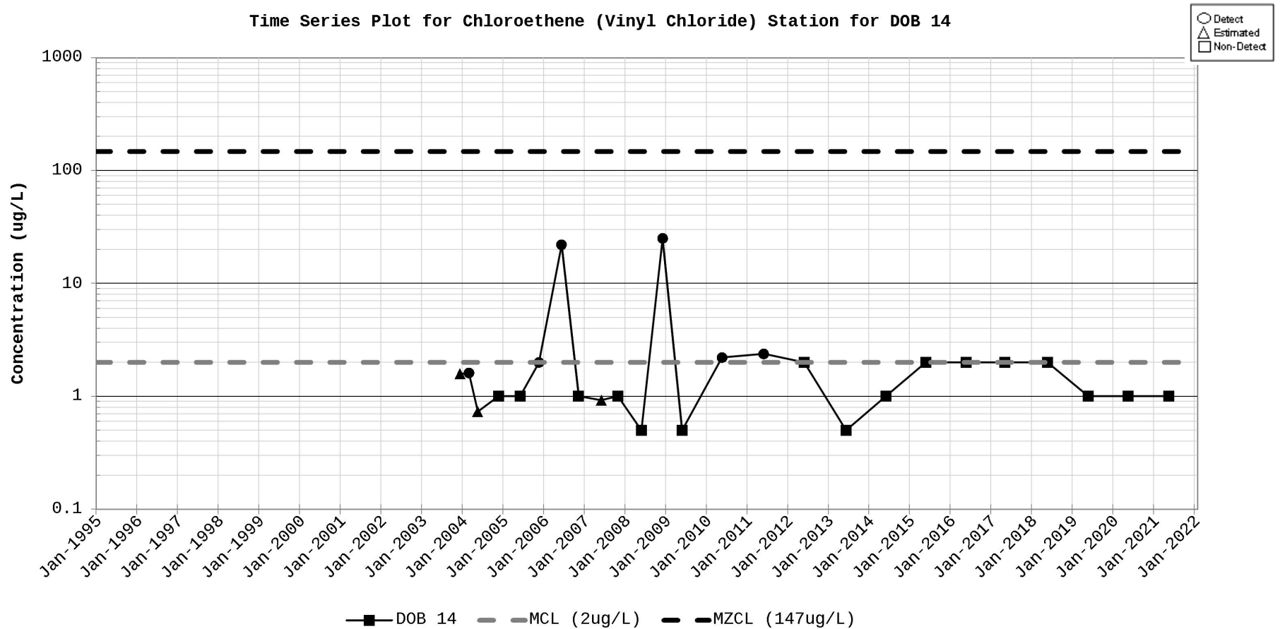
Figure D-5. Time Series Plot for Chloroethene (Vinyl chloride) Station for DOB 14
