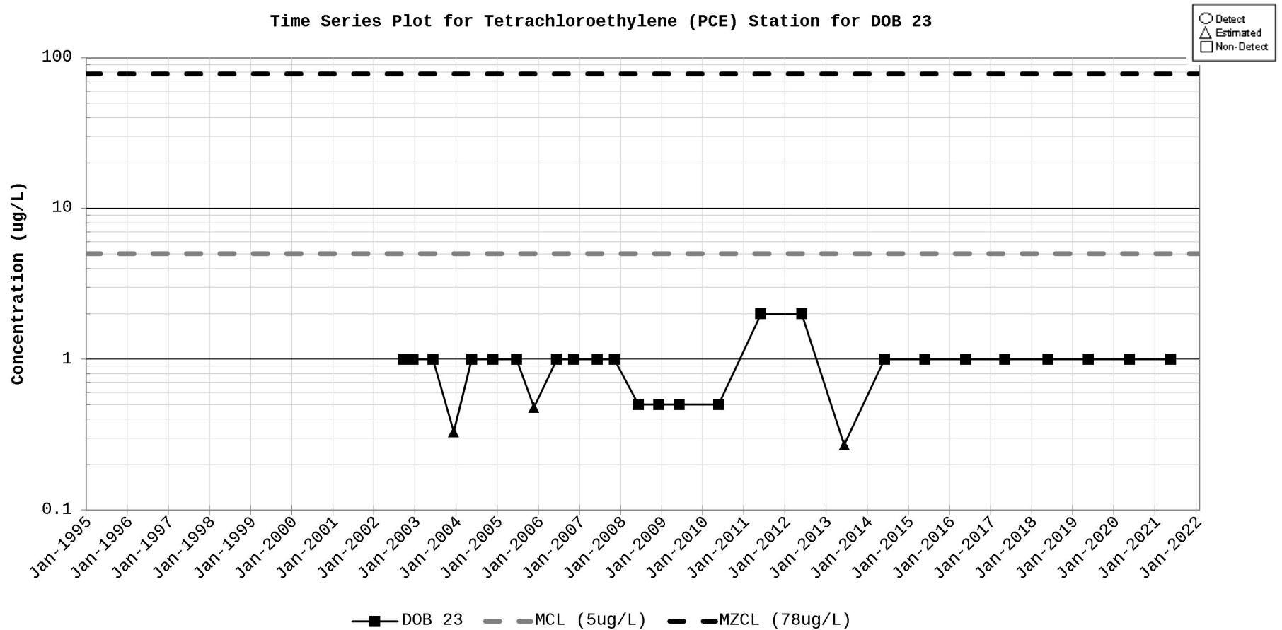
Figure D-66. Time Series Plot for Tetrachloroethylene (PCE) Station for DOB 23
