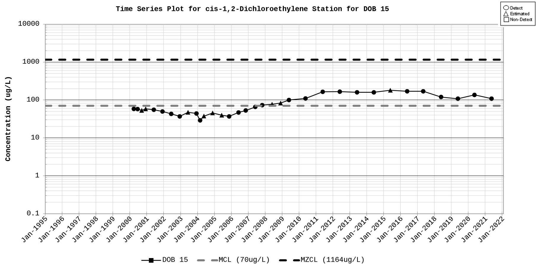
Figure D-29. Time Series Plot for cis-1,2-Dichloroethylene Station for DOB 15
