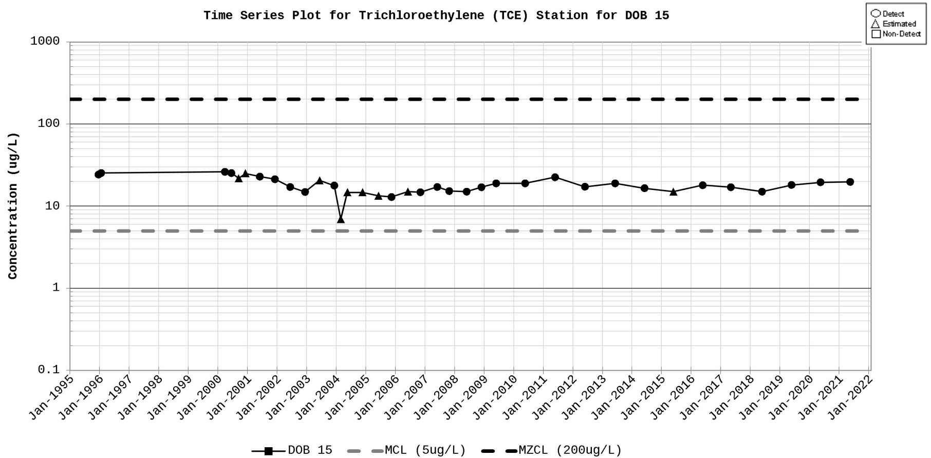
Figure D-75. Time Series Plot for Trichloroethylene (TCE) Station for DOB 15
