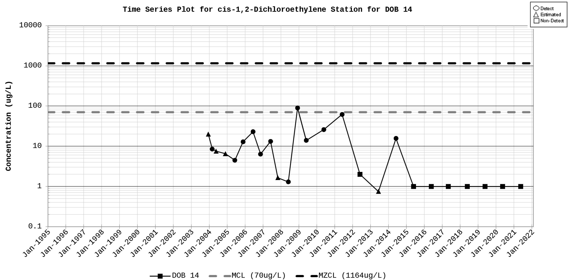
Figure D-28. Time Series Plot for cis-1,2-Dichloroethylene Station for DOB 14
