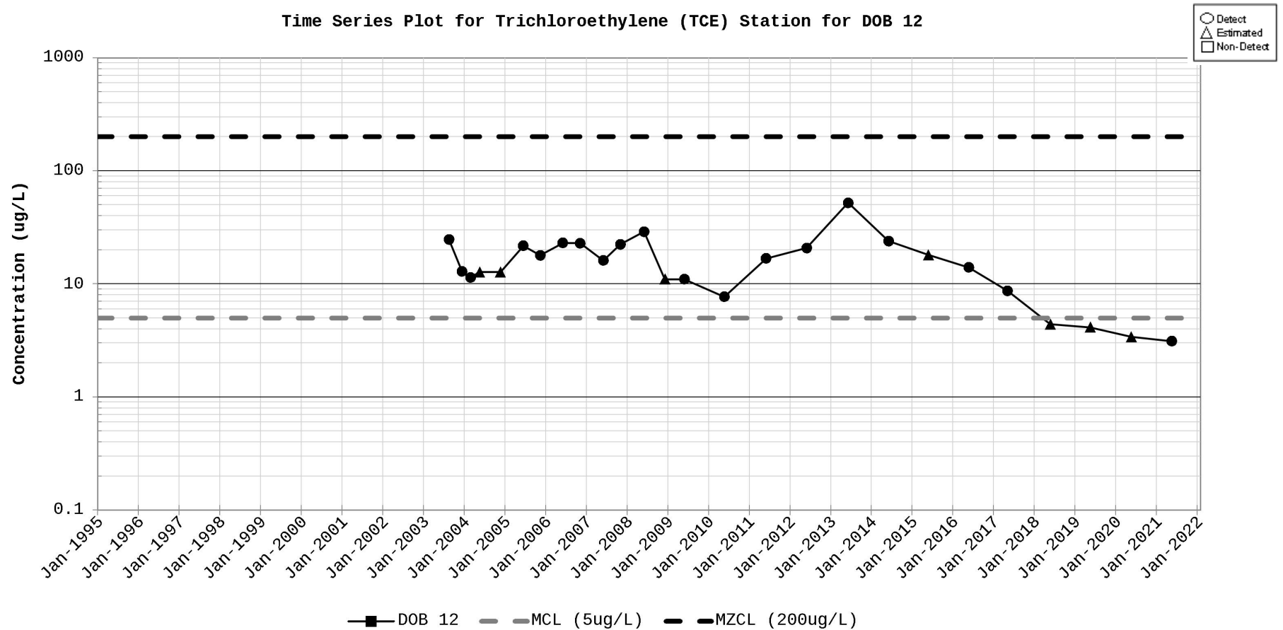
Figure D-72. Time Series Plot for Trichloroethylene (TCE) Station for DOB 12
