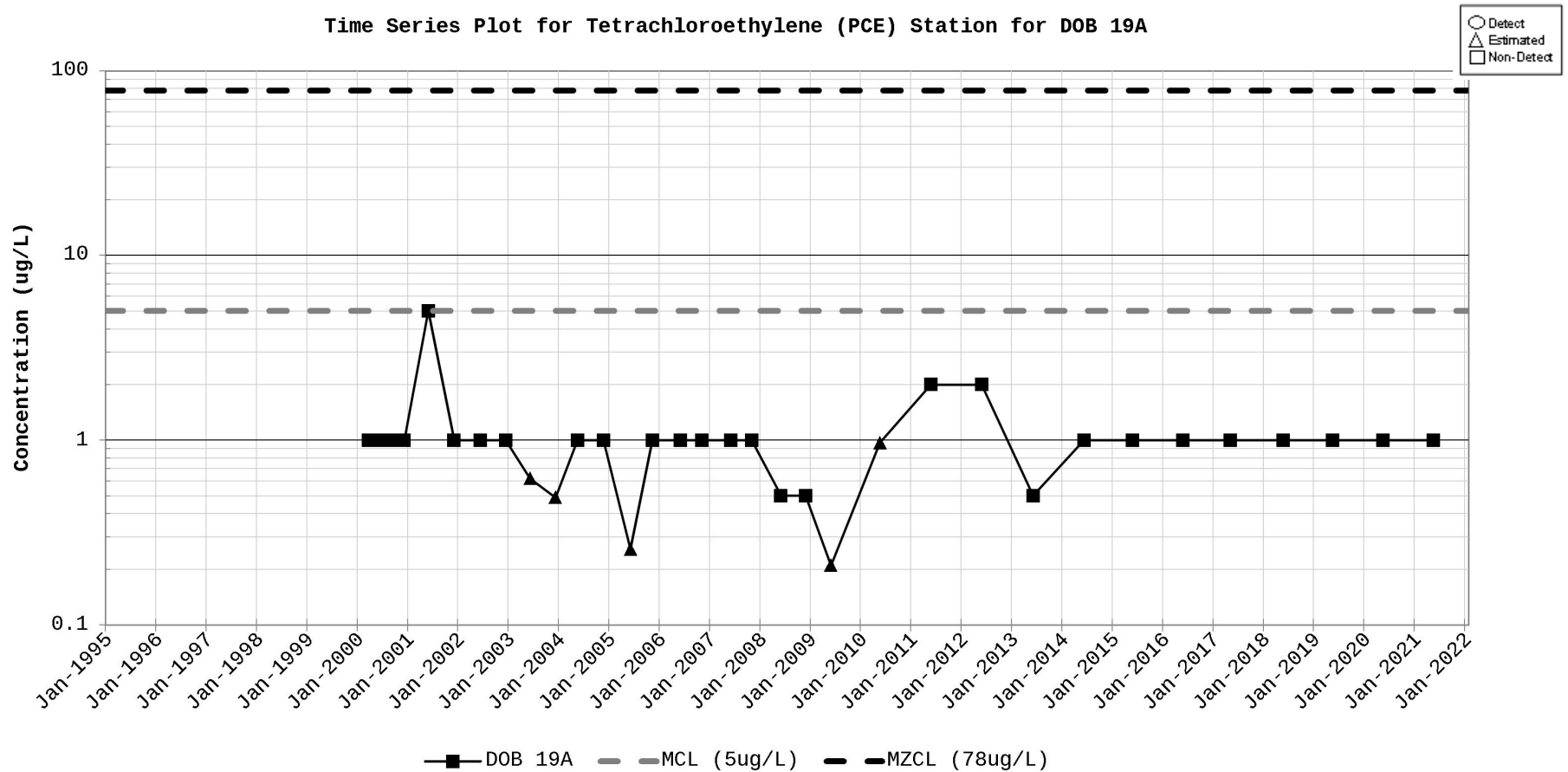
Figure D-59. Time Series Plot for Tetrachloroethylene (PCE) Station for DOB 19A
