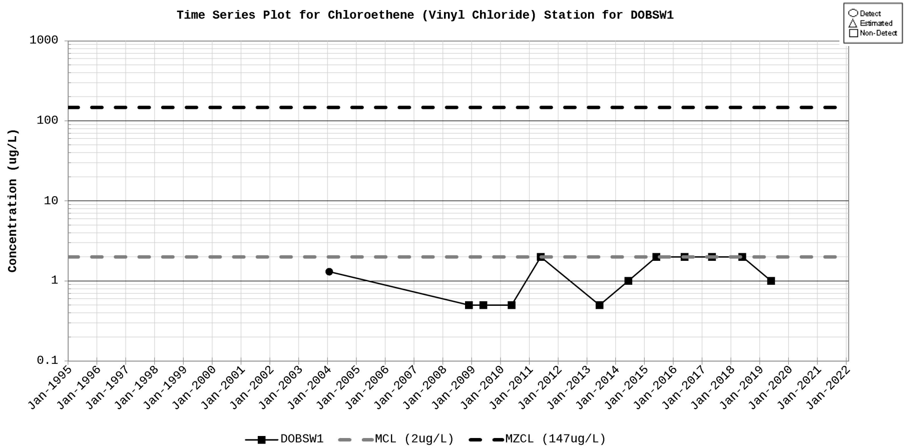
Figure D-21. Time Series Plot for Chloroethene (Vinyl chloride) Station for DOBSW1
