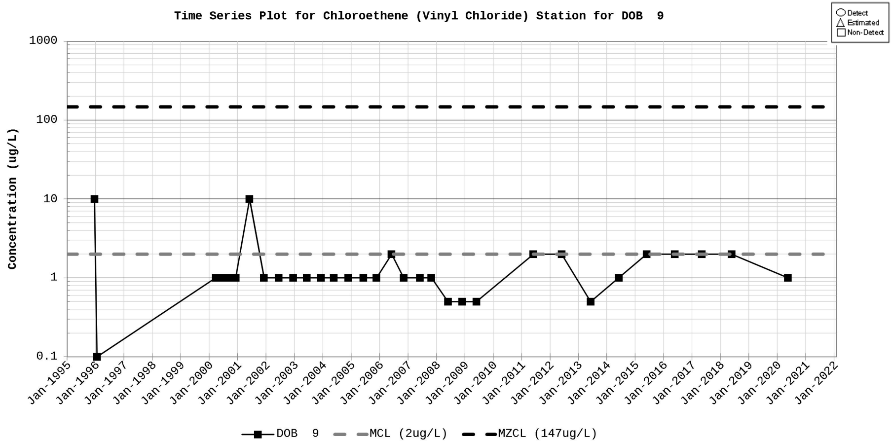
Figure D-1. Time Series Plot for Chloroethene (Vinyl chloride) Station for DOB 9
