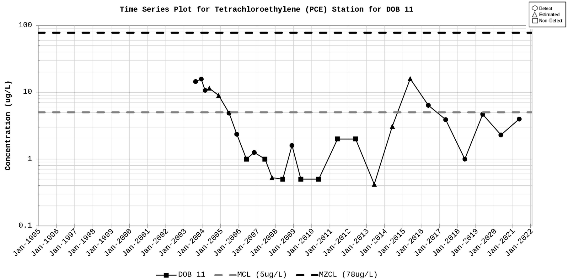
Figure D-48. Time Series Plot for Tetrachloroethylene (PCE) Station for DOB 11
