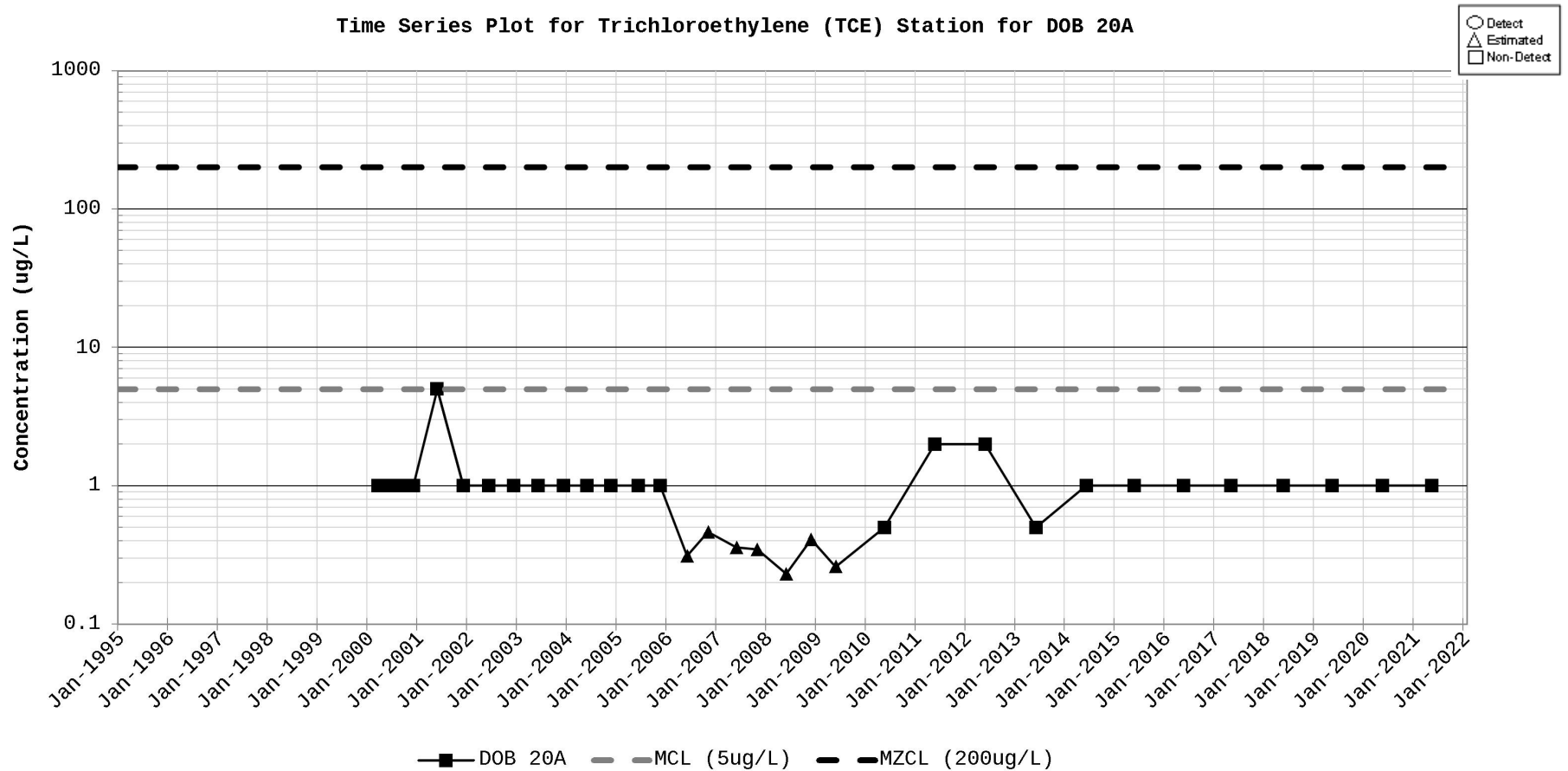
Figure D-82. Time Series Plot for Trichloroethylene (TCE) Station for DOB 20A
