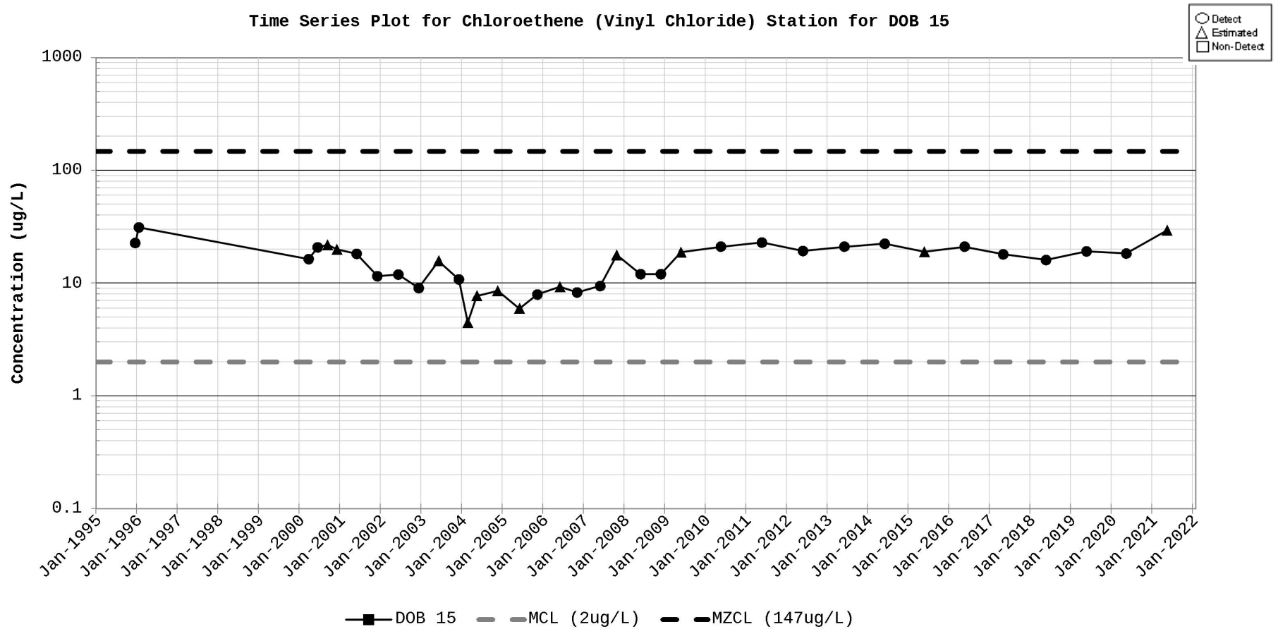
Figure D-6. Time Series Plot for Chloroethene (Vinyl chloride) Station for DOB 15
