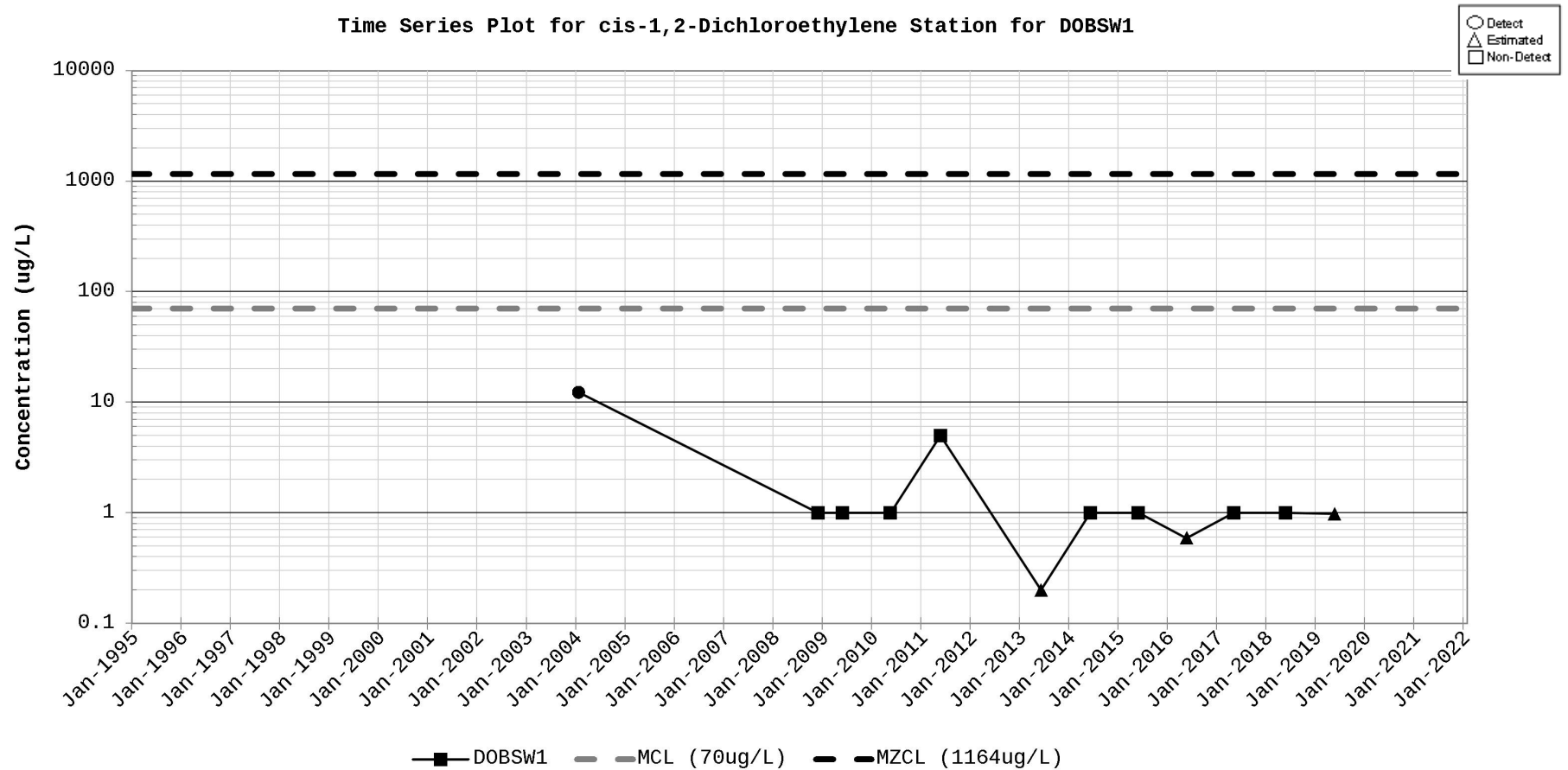
Figure D-44. Time Series Plot for cis-1,2-Dichloroethylene Station for DOBSW1
