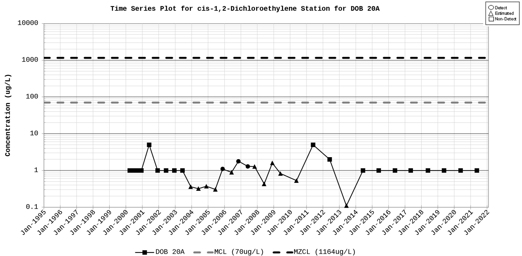
Figure D-36. Time Series Plot for cis-1,2-Dichloroethylene Station for DOB 20A
