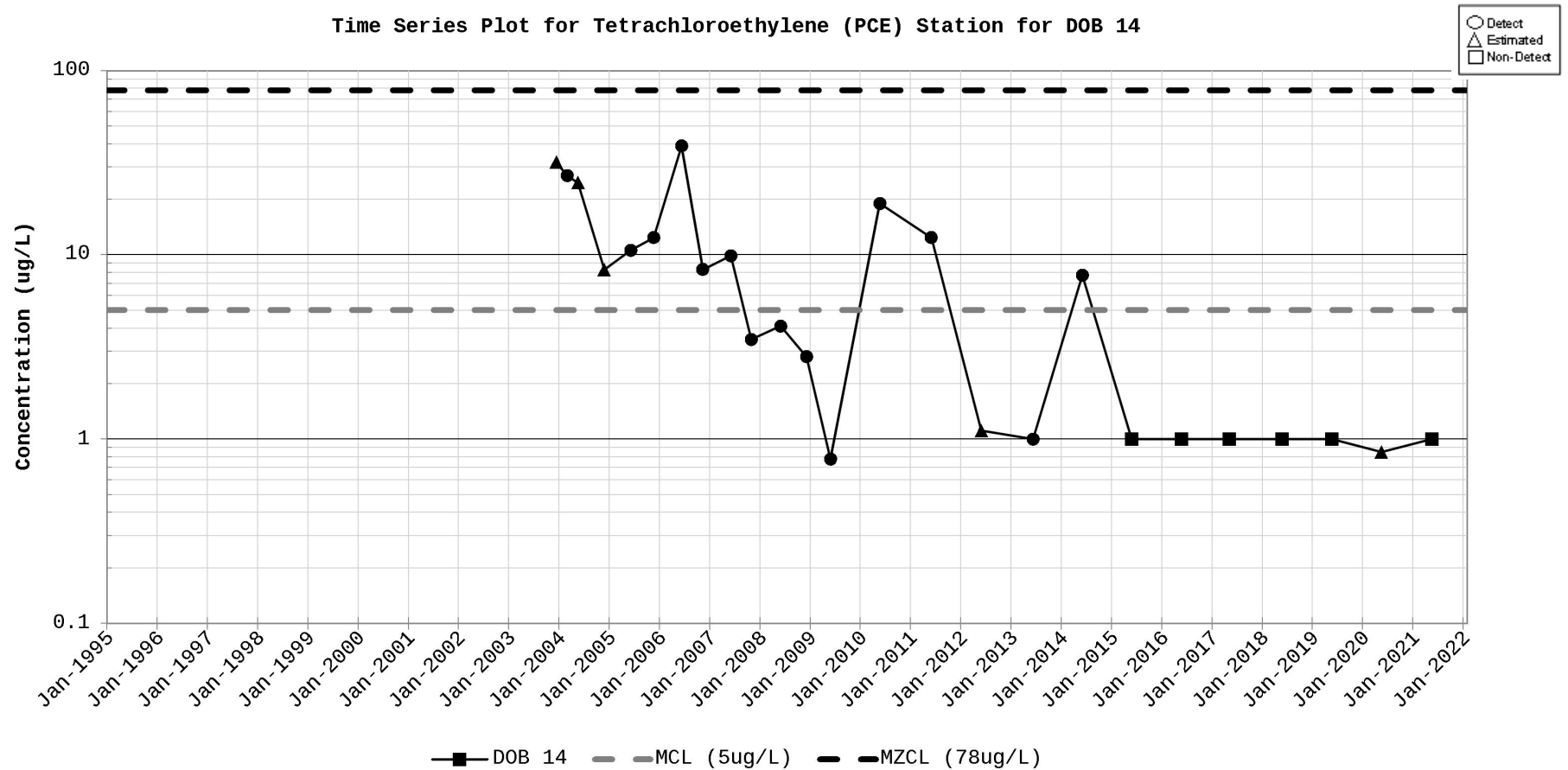
Figure D-51. Time Series Plot for Tetrachloroethylene (PCE) Station for DOB 14
