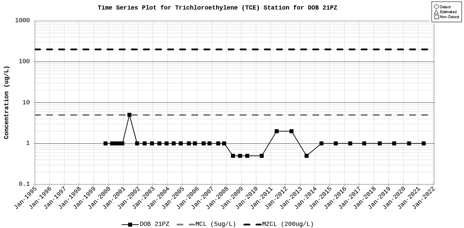
Figure D-86. Time Series Plot for Trichloroethylene (TCE) Station for DOB 21PZ
