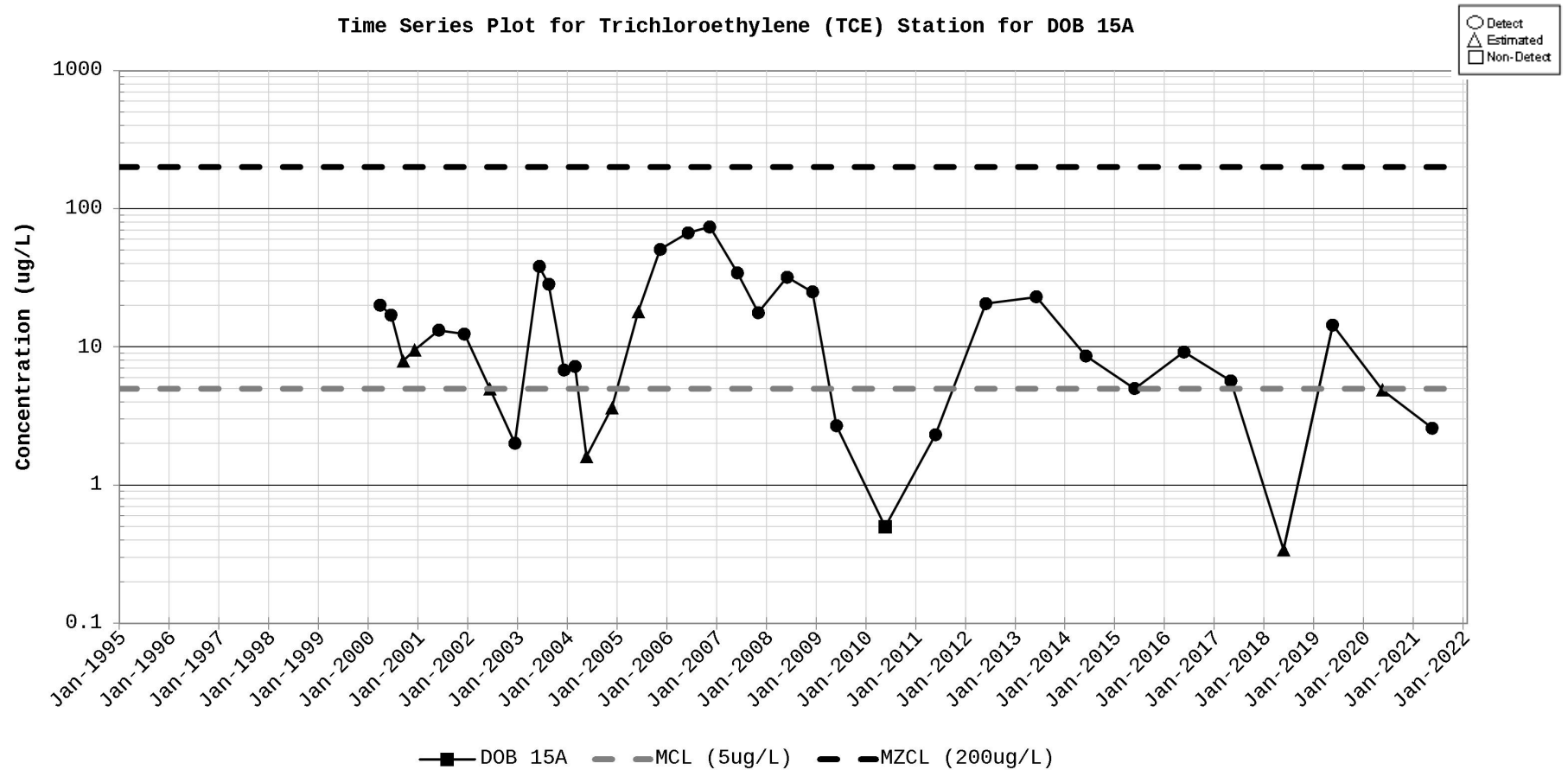
Figure D-76. Time Series Plot for Trichloroethylene (TCE) Station for DOB 15A
