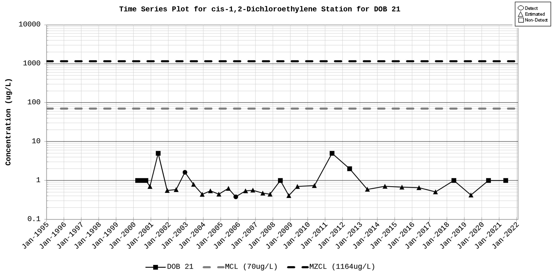
Figure D-39. Time Series Plot for cis-1,2-Dichloroethylene Station for DOB 21
