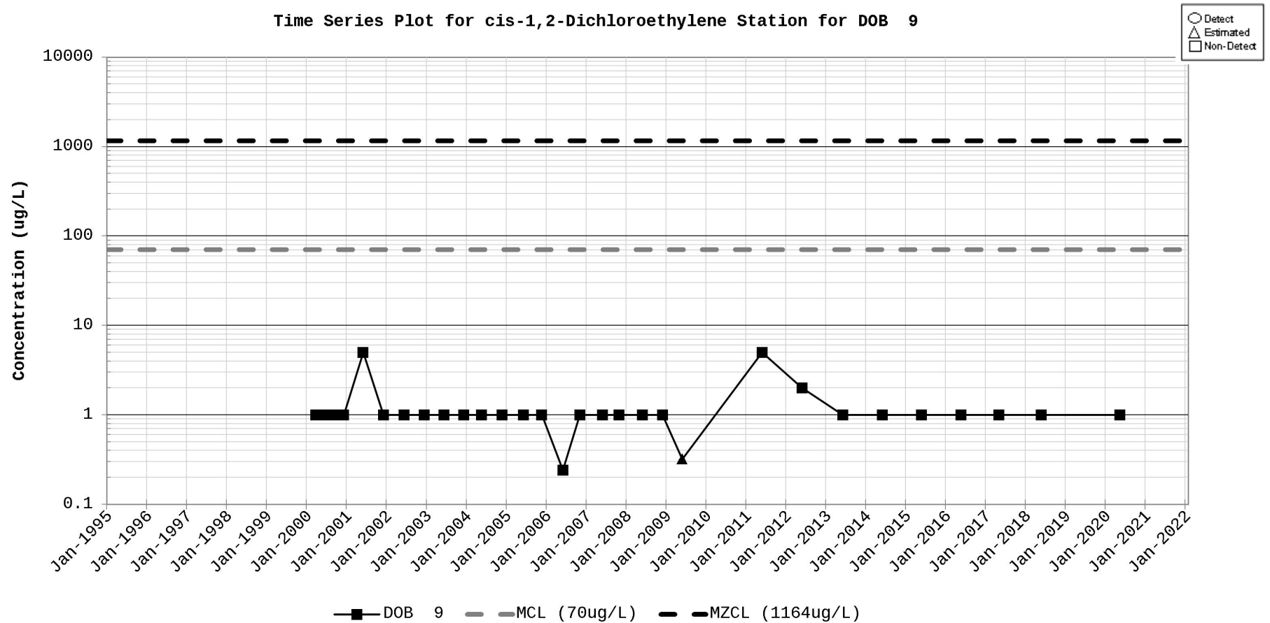
Figure D-24. Time Series Plot for cis-1,2-Dichloroethylene Station for DOB 9
