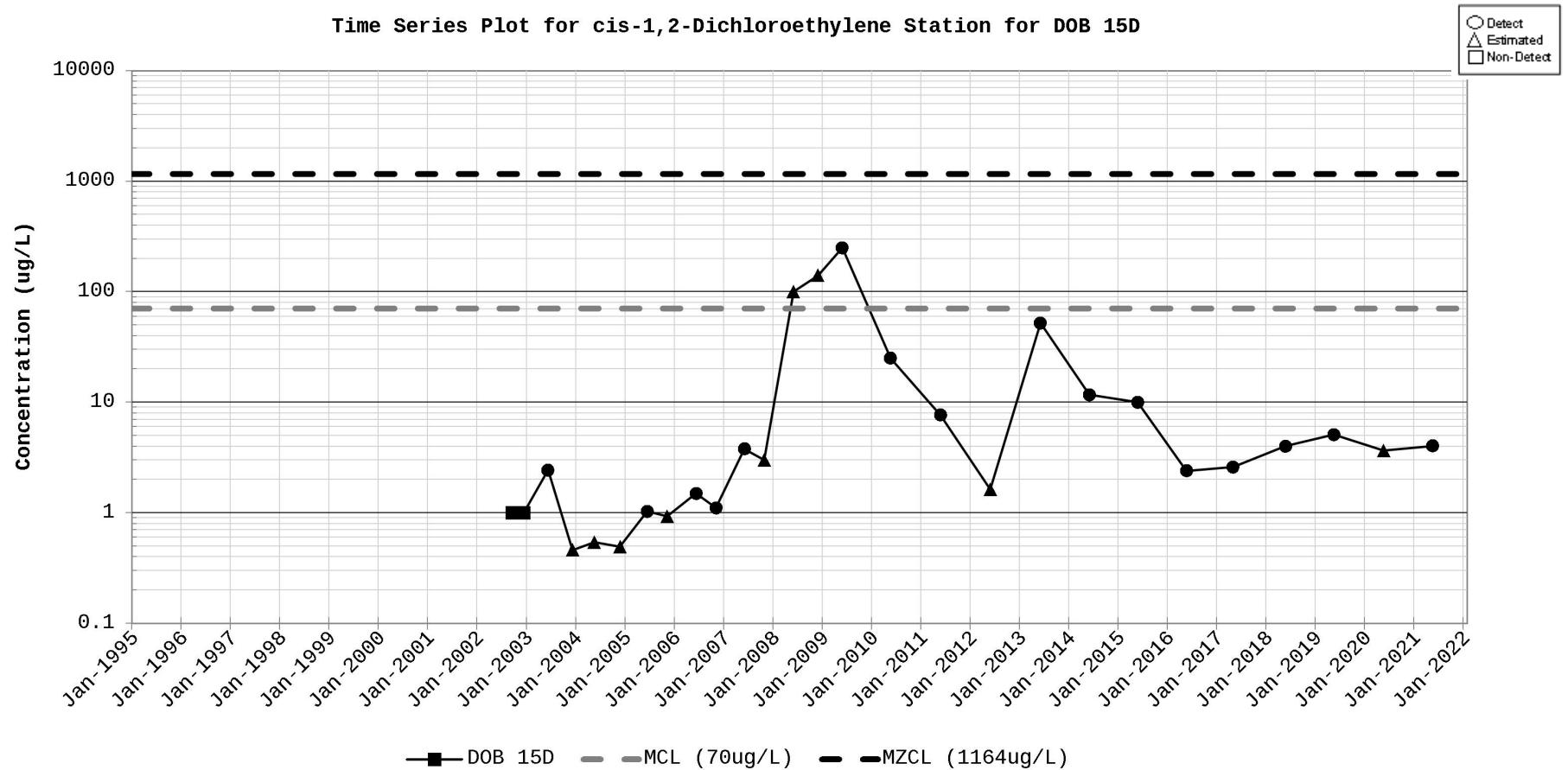
Figure D-32. Time Series Plot for cis-1,2-Dichloroethylene Station for DOB 15D
