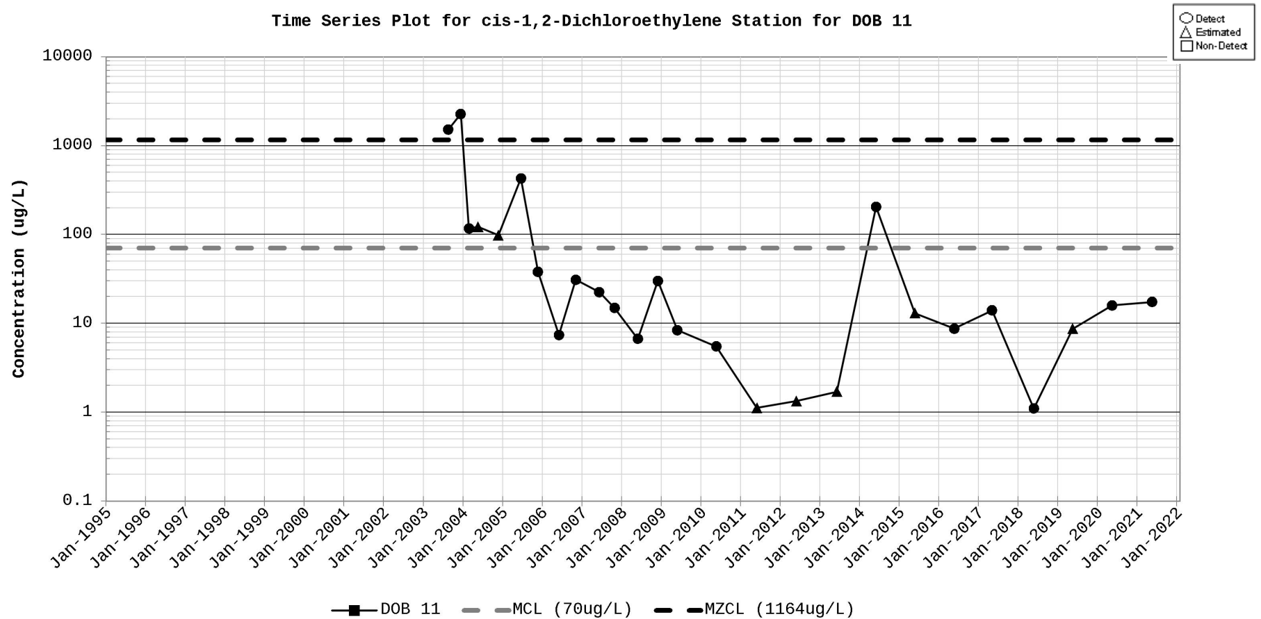
Figure D-25. Time Series Plot for cis-1,2-Dichloroethylene Station for DOB 11
