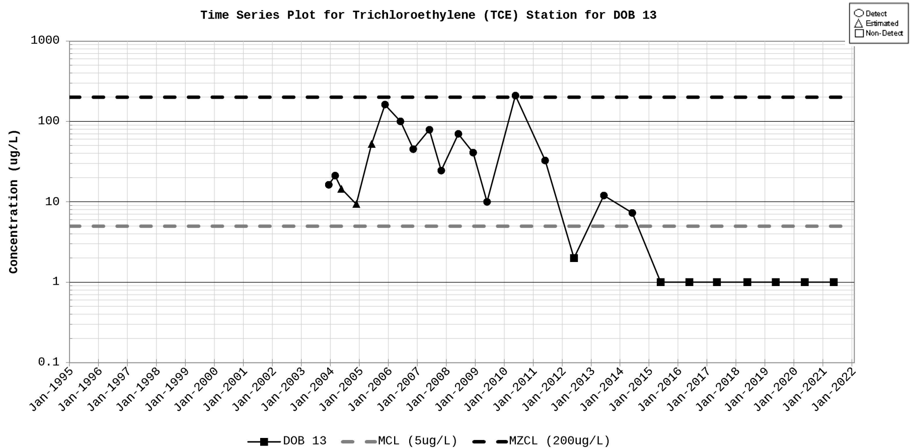
Figure D-73. Time Series Plot for Trichloroethylene (TCE) Station for DOB 13
