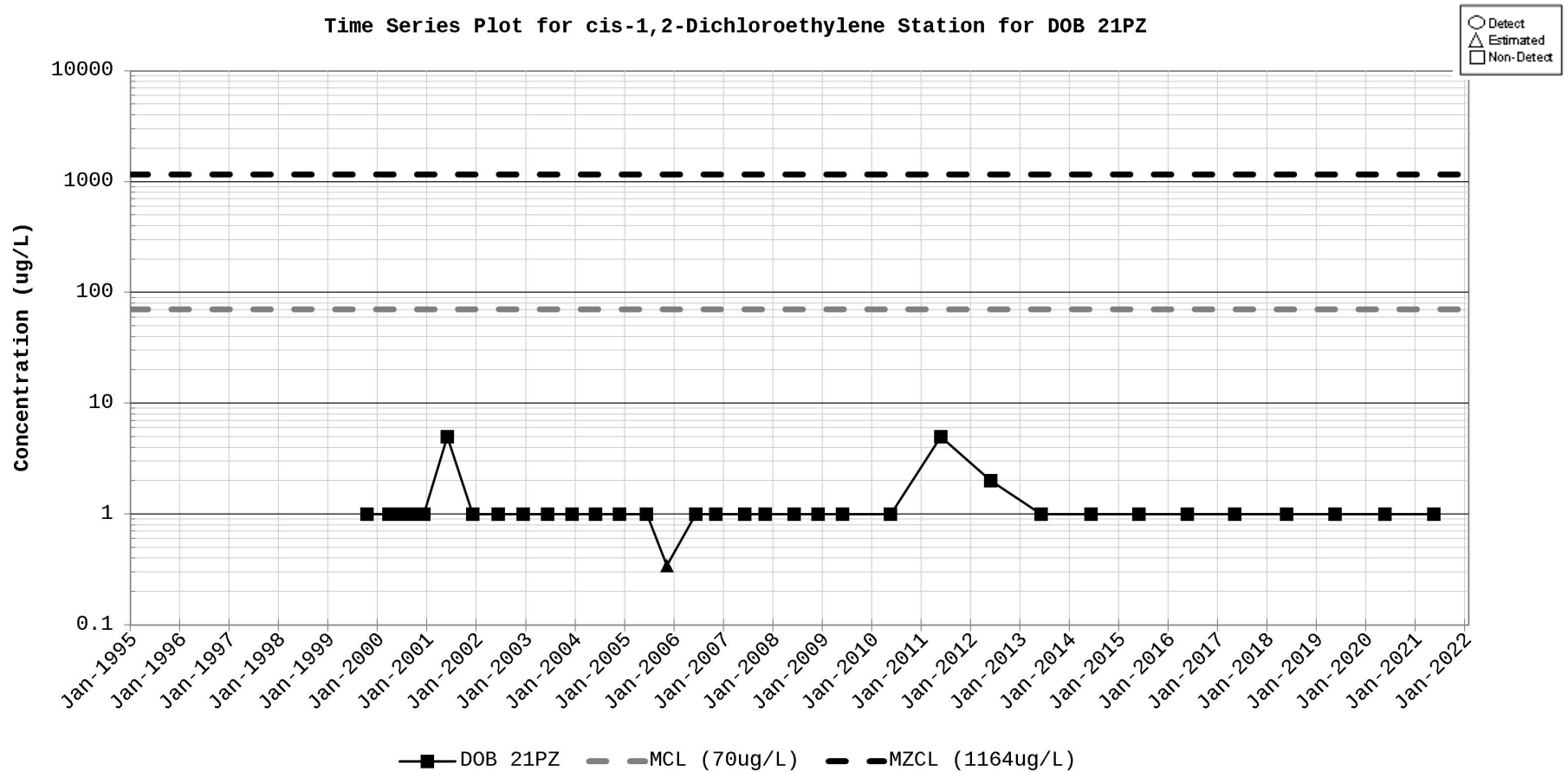
Figure D-40. Time Series Plot for cis-1,2-Dichloroethylene Station for DOB 21PZ
