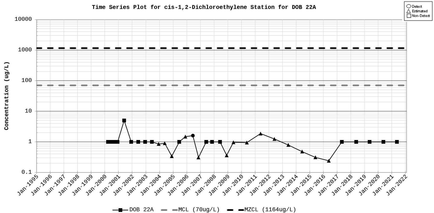
Figure D-41. Time Series Plot for cis-1,2-Dichloroethylene Station for DOB 22A
