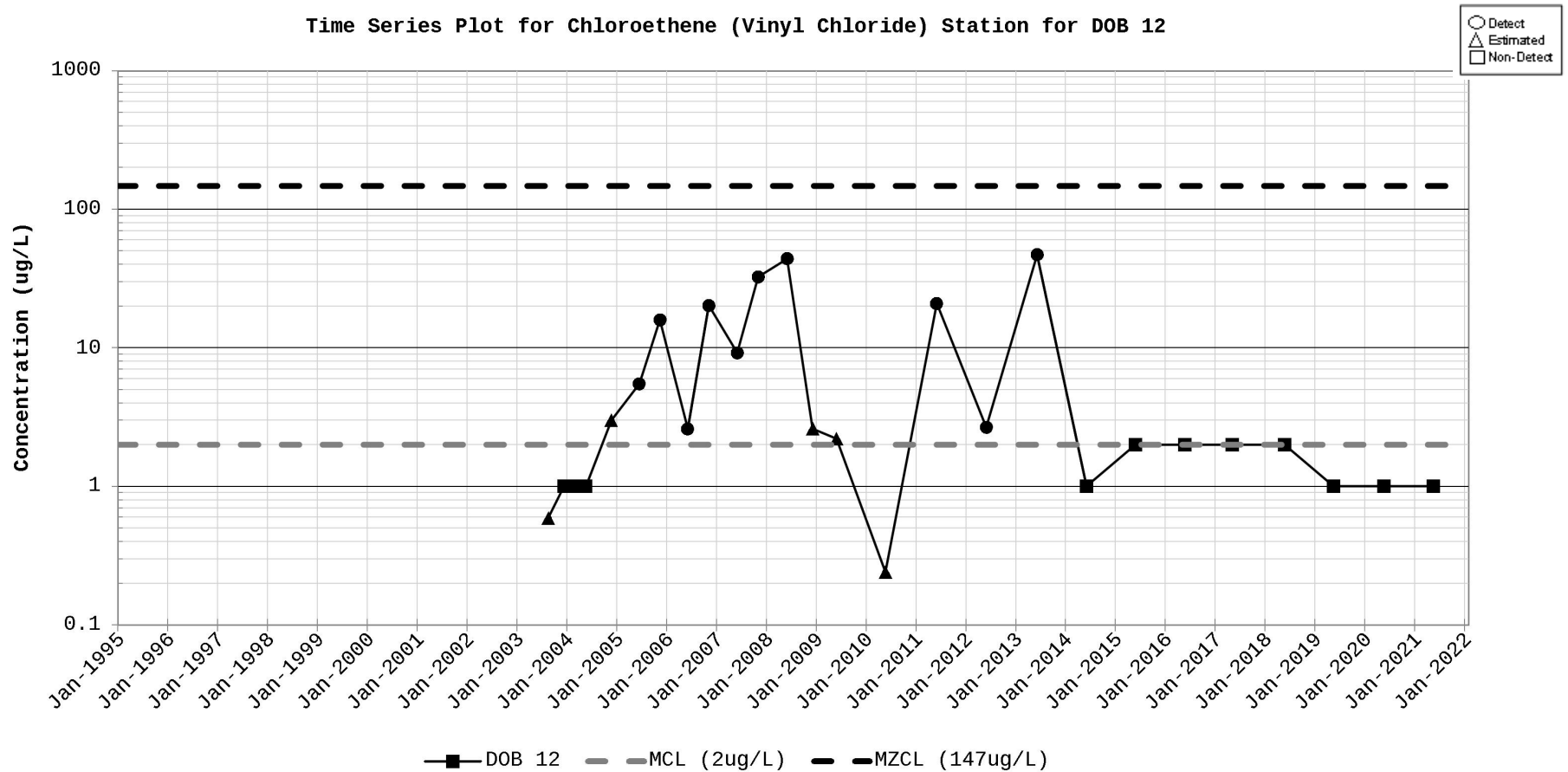
Figure D-3. Time Series Plot for Chloroethene (Vinyl chloride) Station for DOB 12
