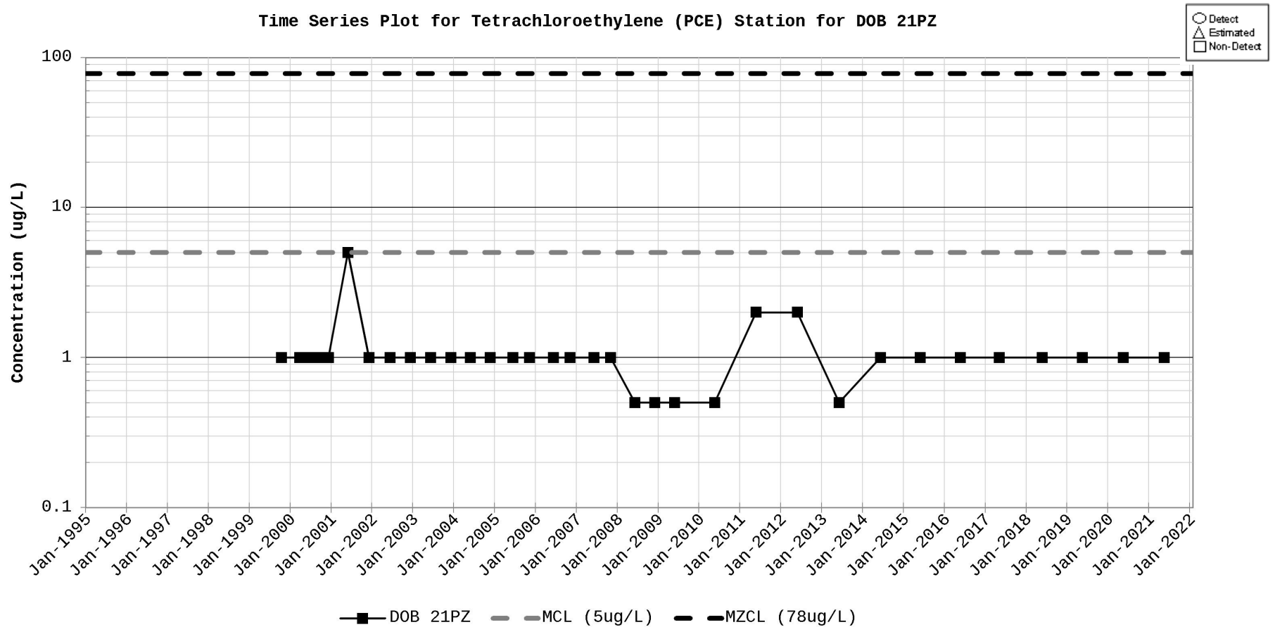
Figure D-63. Time Series Plot for Tetrachloroethylene (PCE) Station for DOB 21PZ
