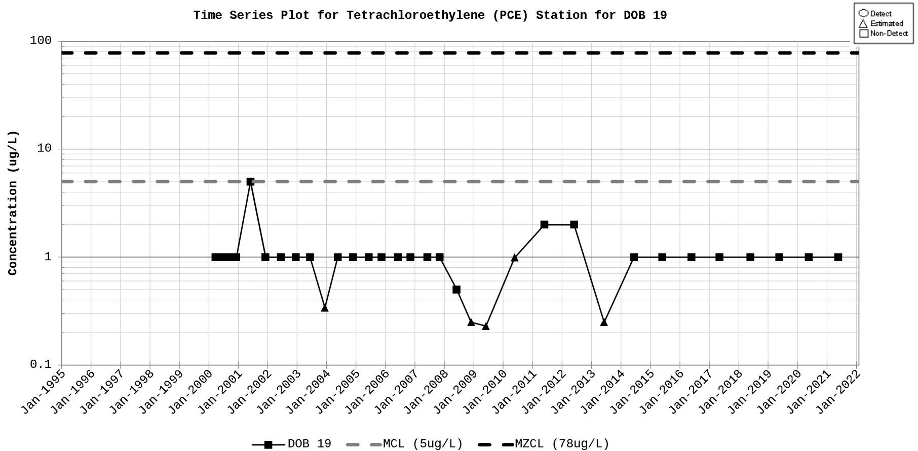
Figure D-57. Time Series Plot for Tetrachloroethylene (PCE) Station for DOB 19
