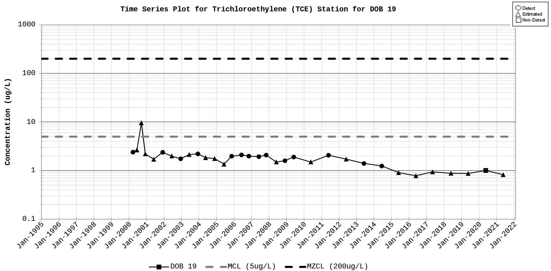
Figure D-80. Time Series Plot for Trichloroethylene (TCE) Station for DOB 19
