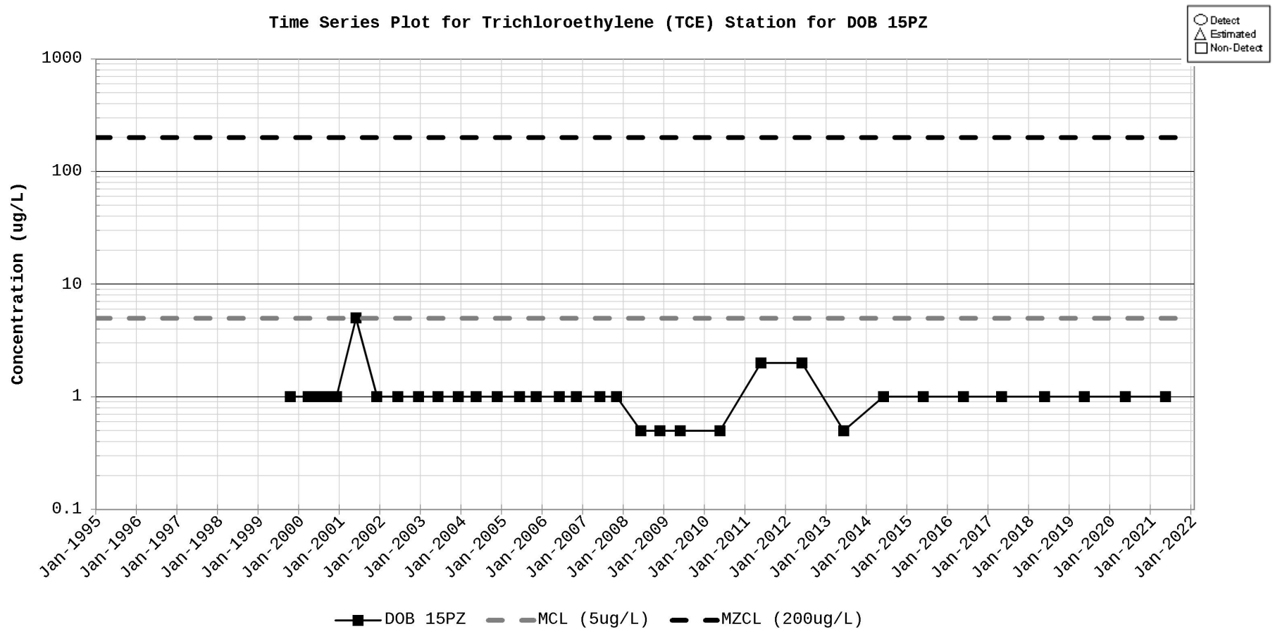
Figure D-77. Time Series Plot for Trichloroethylene (TCE) Station for DOB 15PZ
