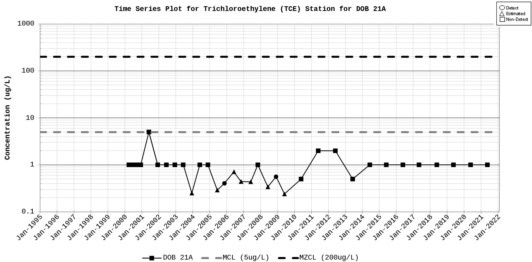
Figure D-84. Time Series Plot for Trichloroethylene (TCE) Station for DOB 21A
