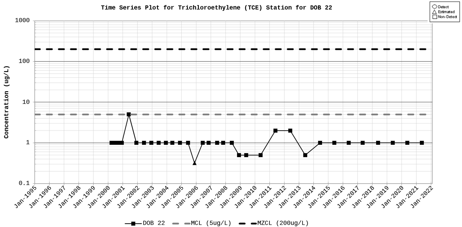
Figure D-88. Time Series Plot for Trichloroethylene (TCE) Station for DOB 22
