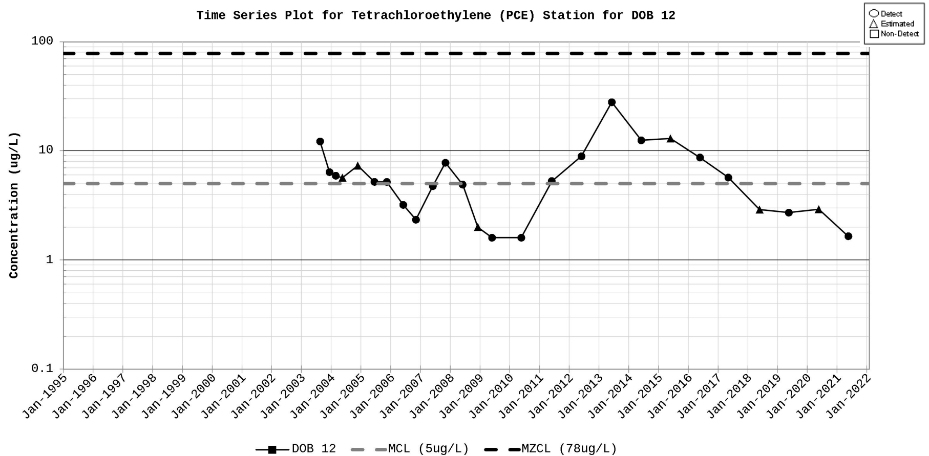
Figure D-49. Time Series Plot for Tetrachloroethylene (PCE) Station for DOB 12
