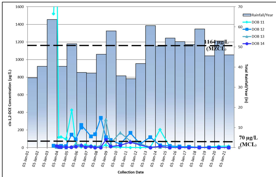
Figure 3. cis-1,2-DCE Concentrations Vs. Rainfall at Plume Compliance Wells (DOB 15, 15A, 15D and DOL 2) and Additional Wells (DOB 11, 12, 13 and 14) at the DOSB OU
