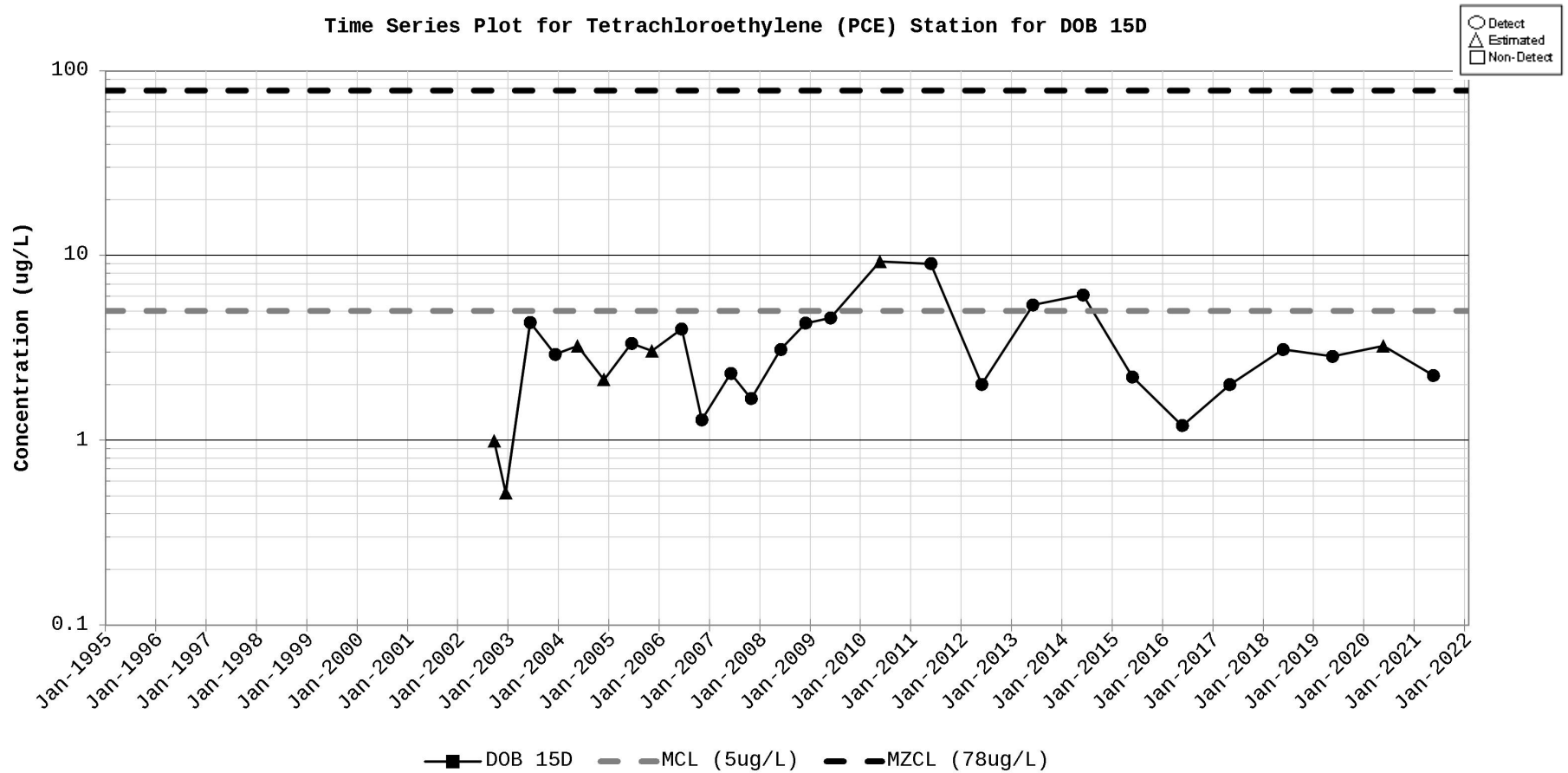
Figure D-55. Time Series Plot for Tetrachloroethylene (PCE) Station for DOB 15D
