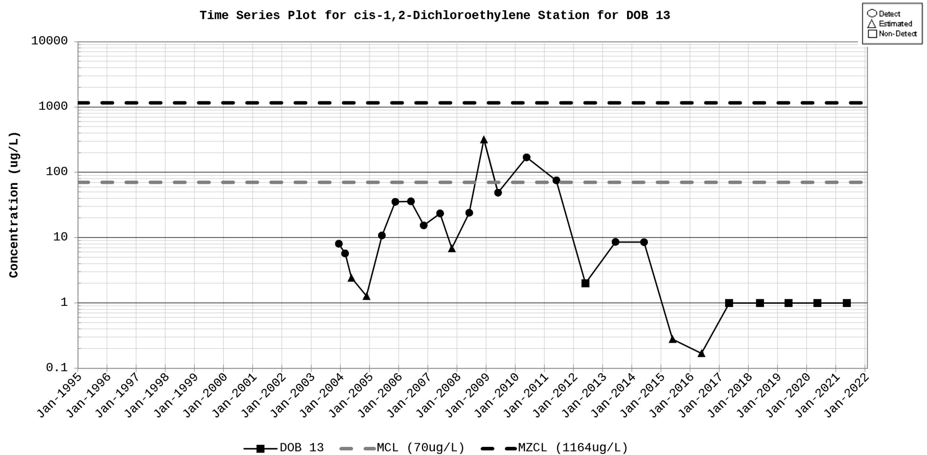
Figure D-27. Time Series Plot for cis-1,2-Dichloroethylene Station for DOB 13
