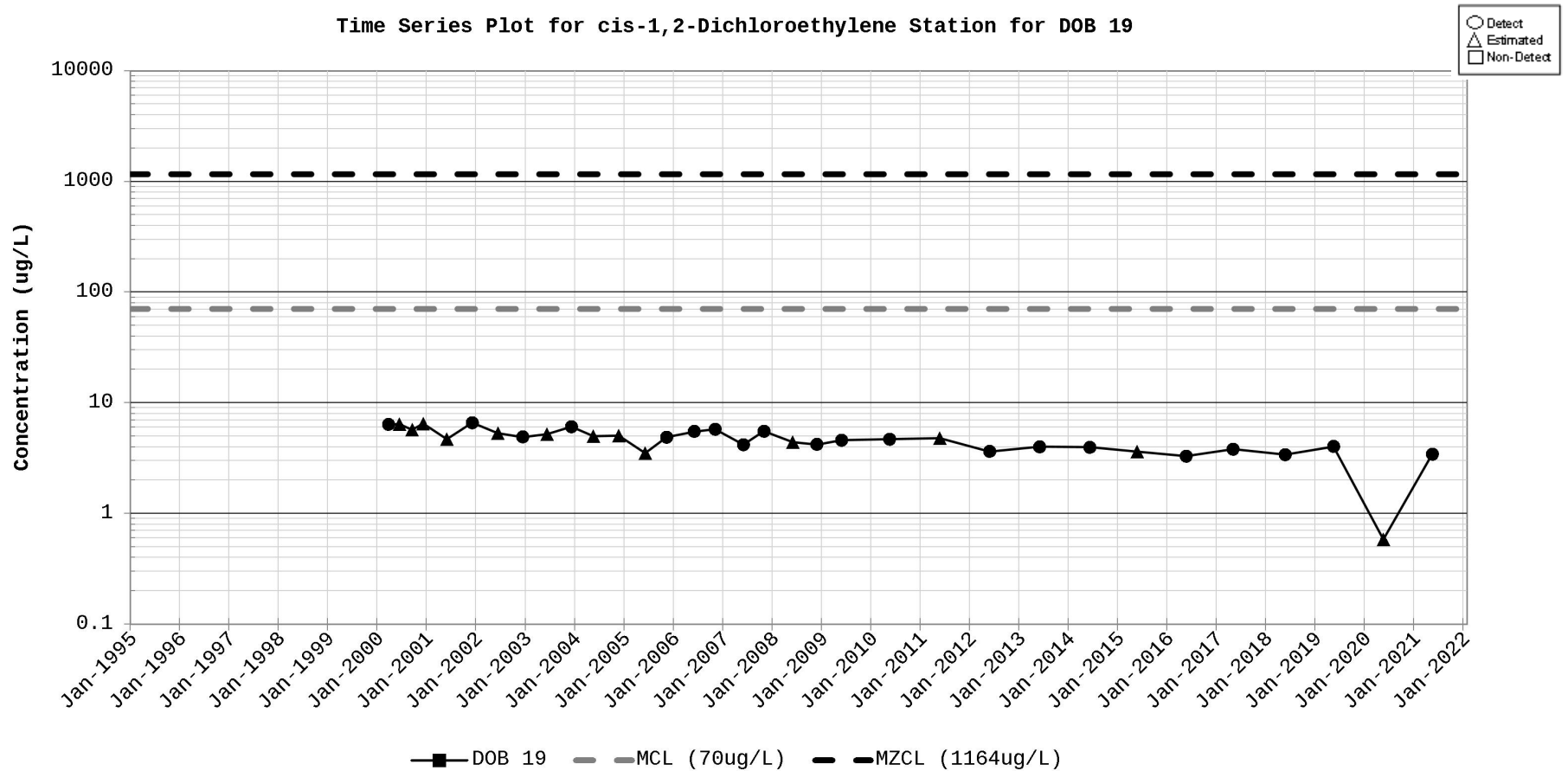
Figure D-34. Time Series Plot for cis-1,2-Dichloroethylene Station for DOB 19
