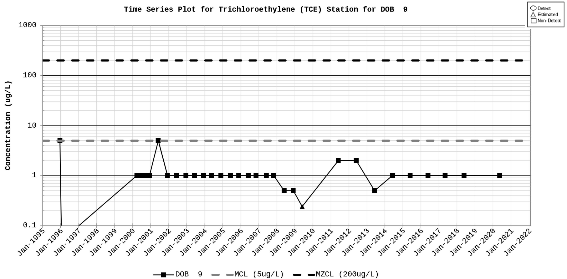
Figure D-70. Time Series Plot for Trichloroethylene (TCE) Station for DOB 9
