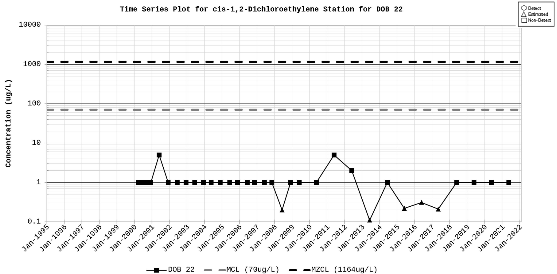
Figure D-42. Time Series Plot for cis-1,2-Dichloroethylene Station for DOB 22
