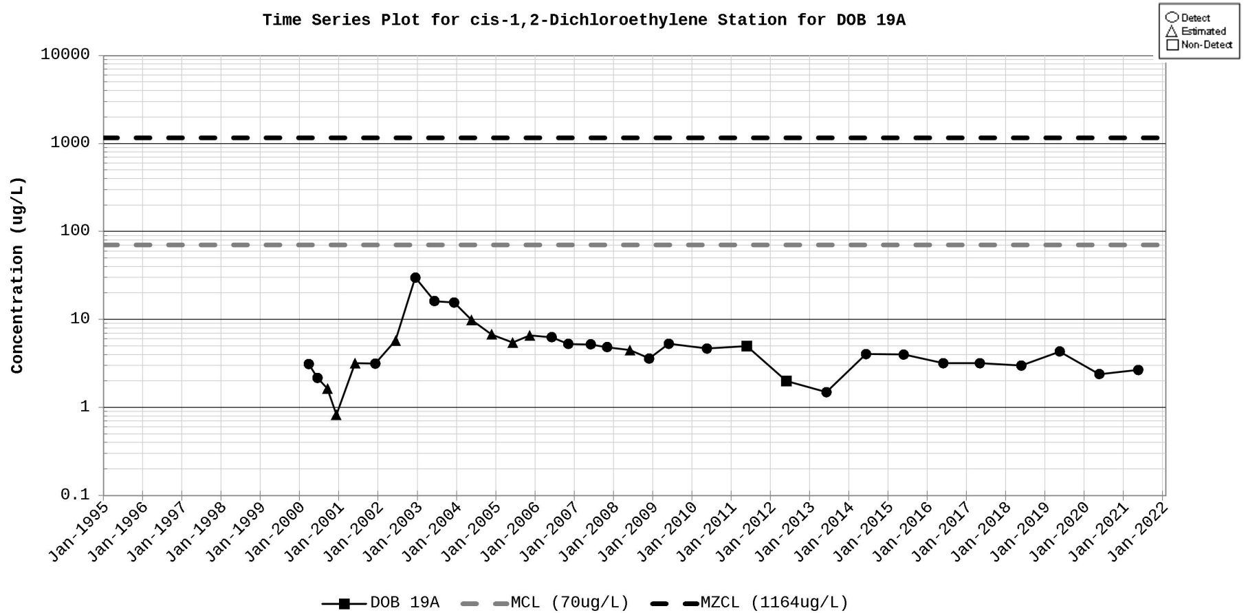
Figure D-35. Time Series Plot for cis-1,2-Dichloroethylene Station for DOB 19A
