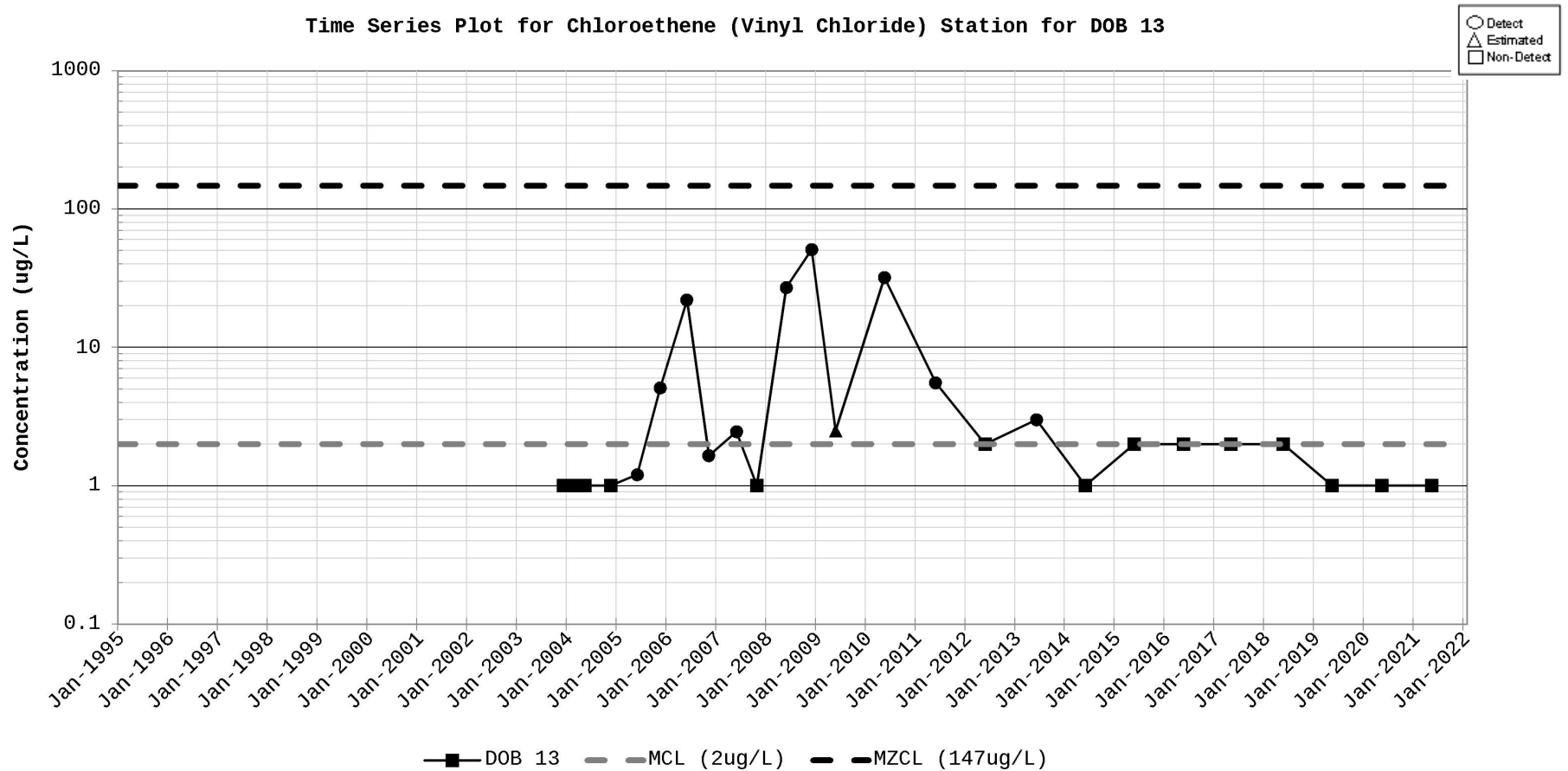
Figure D-4. Time Series Plot for Chloroethene (Vinyl chloride) Station for DOB 13
