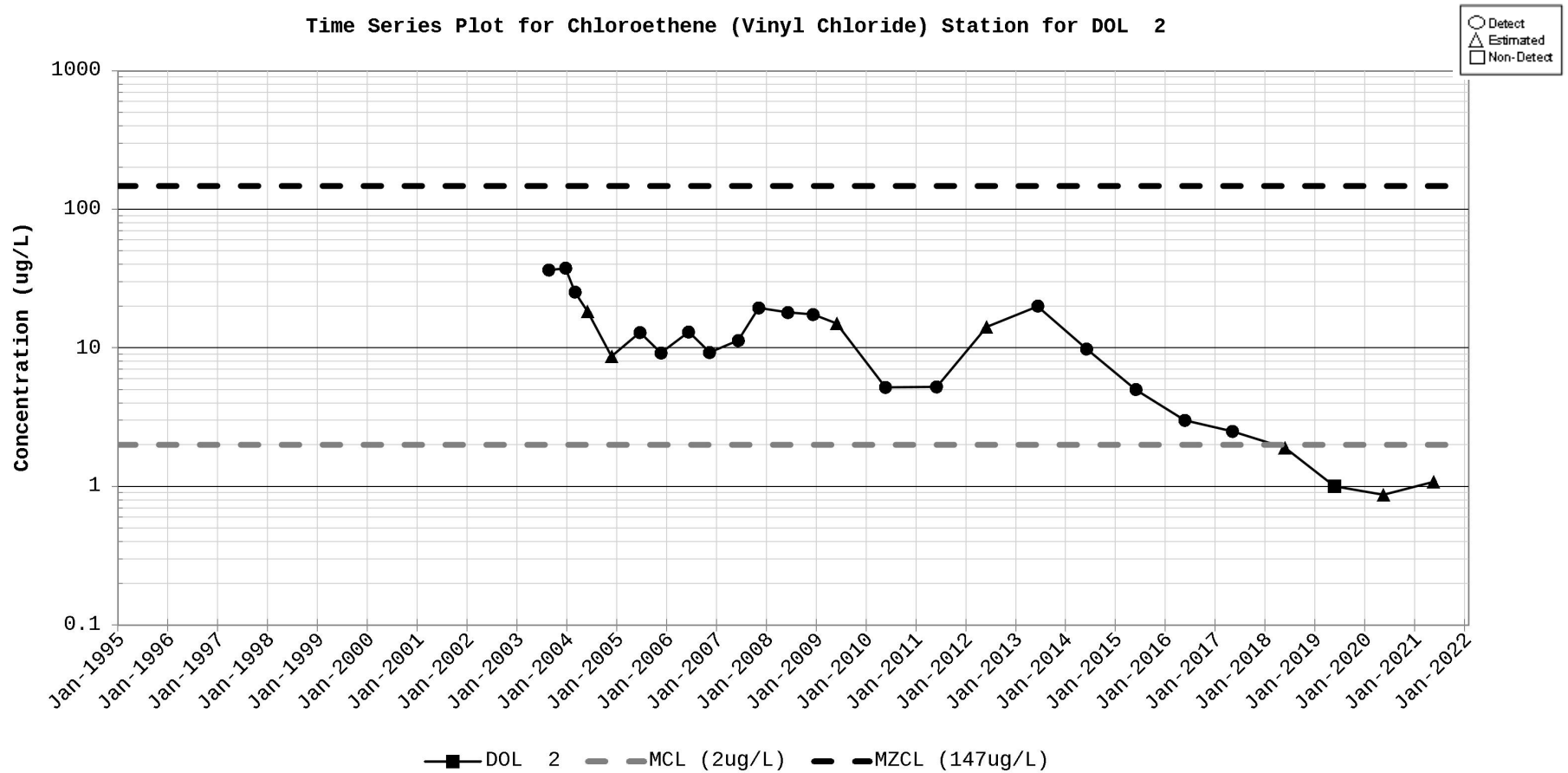
Figure D-23. Time Series Plot for Chloroethene (Vinyl chloride) Station for DOL 2
