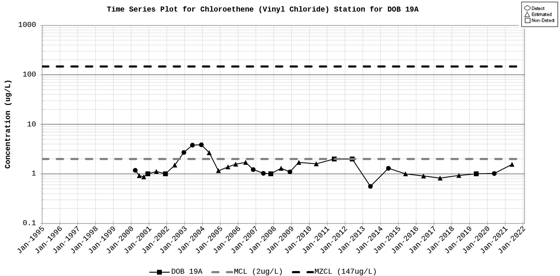
Figure D-12. Time Series Plot for Chloroethene (Vinyl chloride) Station for DOB 19A
