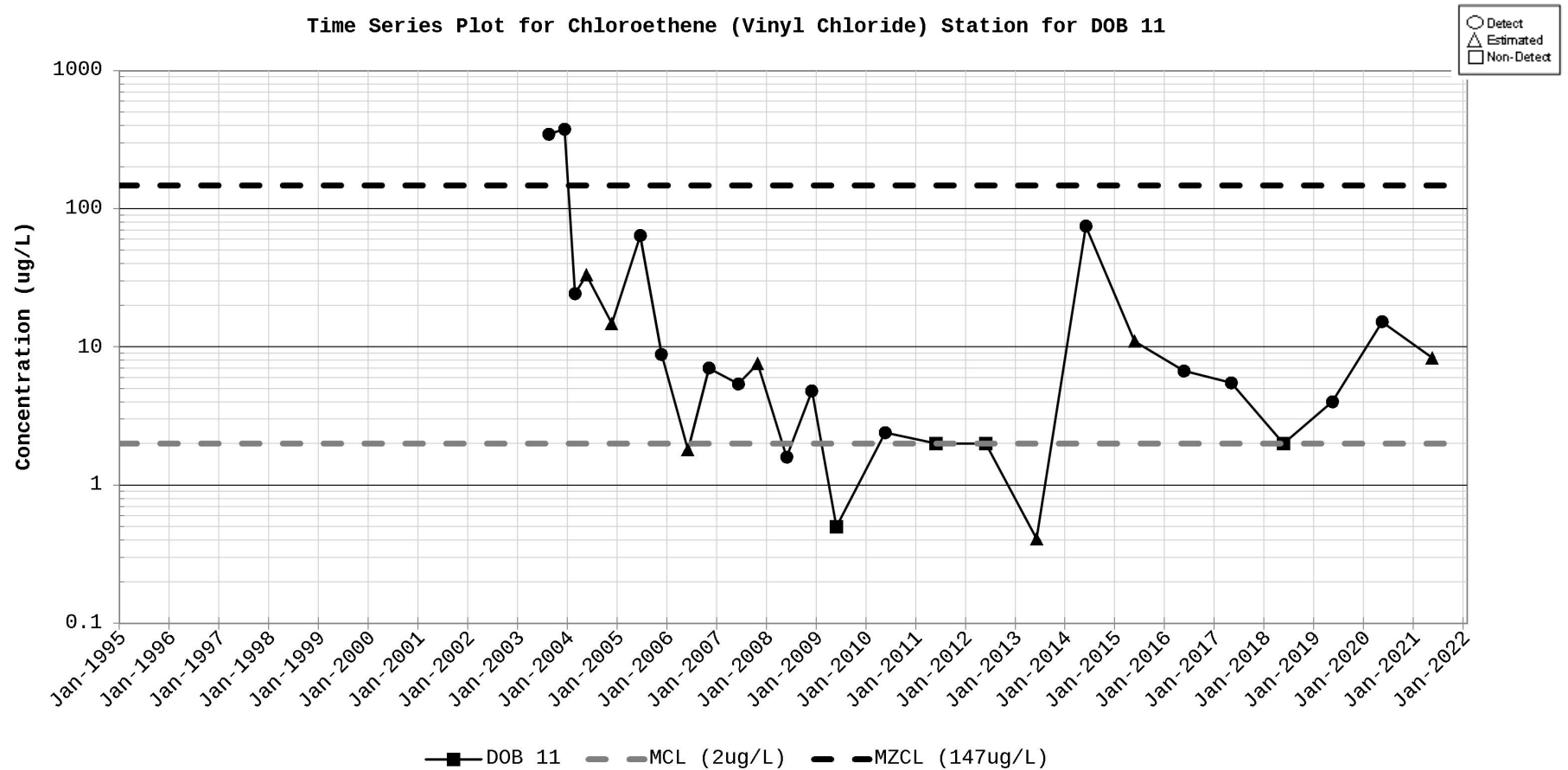
Figure D-2. Time Series Plot for Chloroethene (Vinyl chloride) Station for DOB 11
