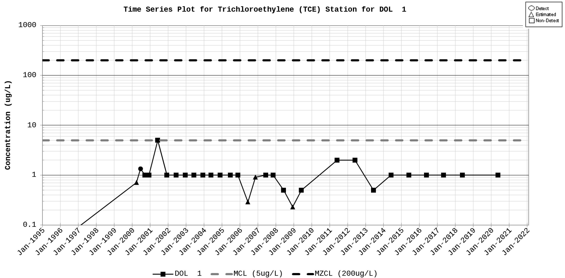
Figure D-91. Time Series Plot for Trichloroethylene (TCE) Station for DOL 1
