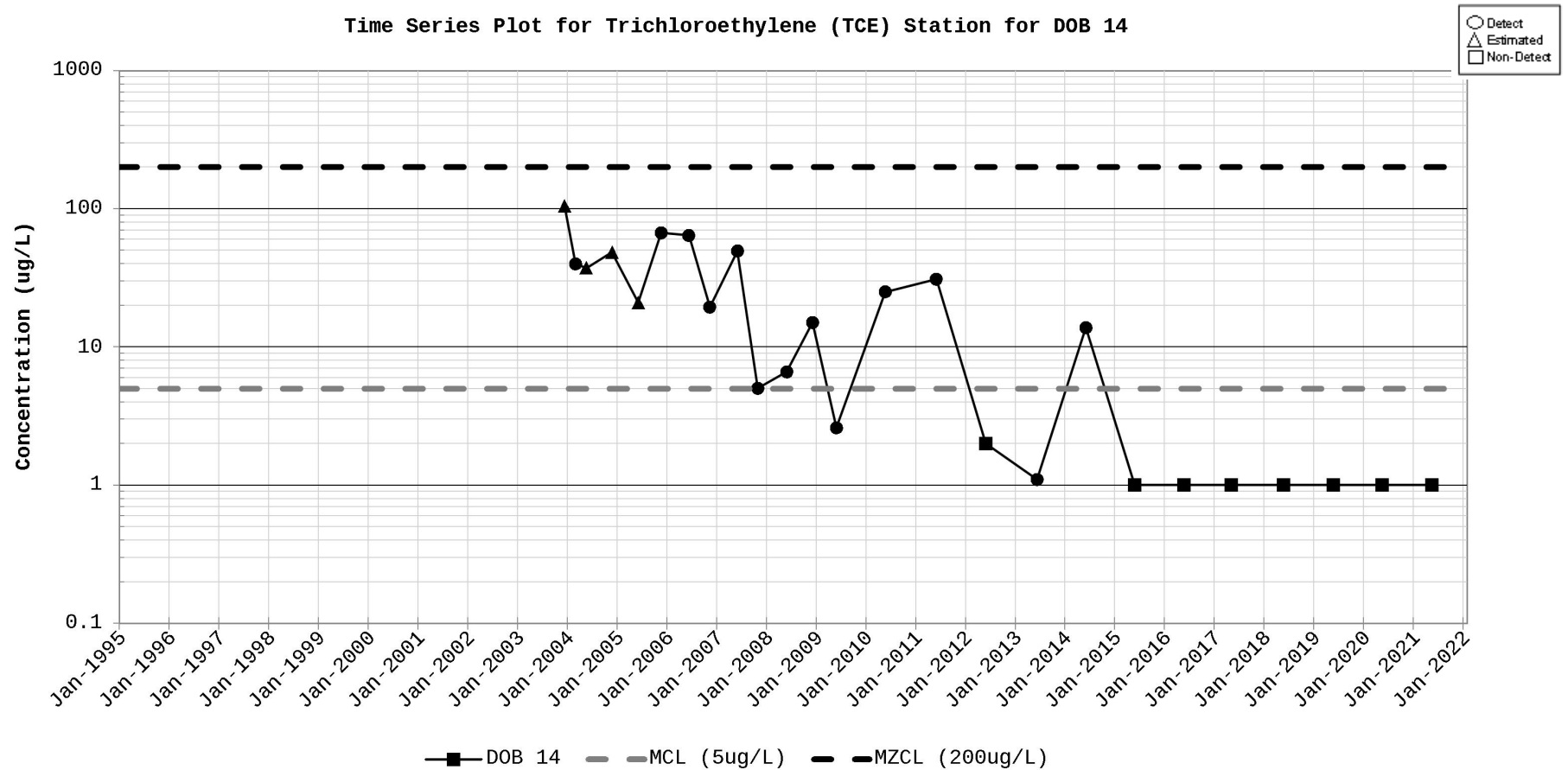
Figure D-74. Time Series Plot for Trichloroethylene (TCE) Station for DOB 14
