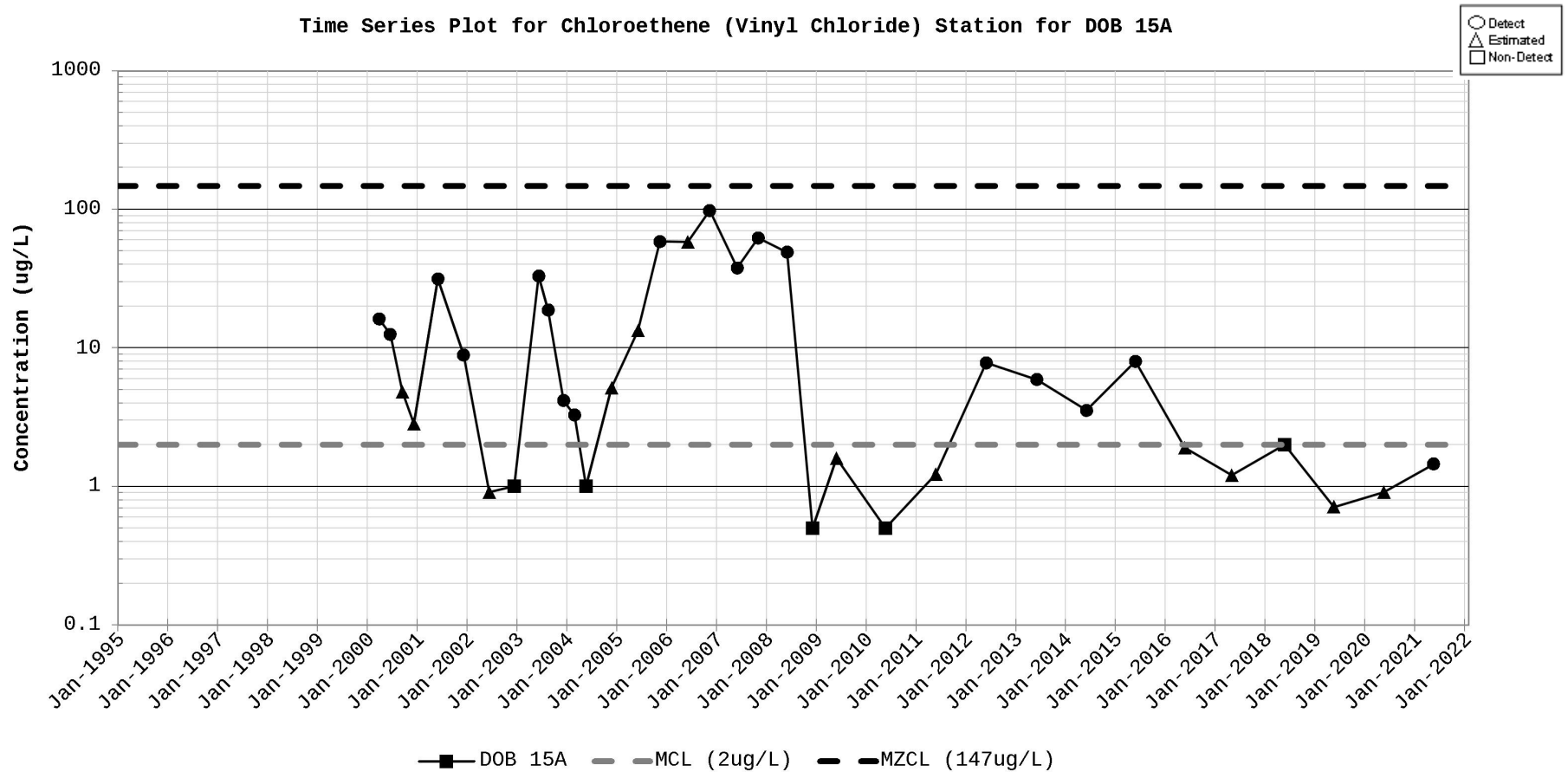
Figure D-7. Time Series Plot for Chloroethene (Vinyl chloride) Station for DOB 15A
