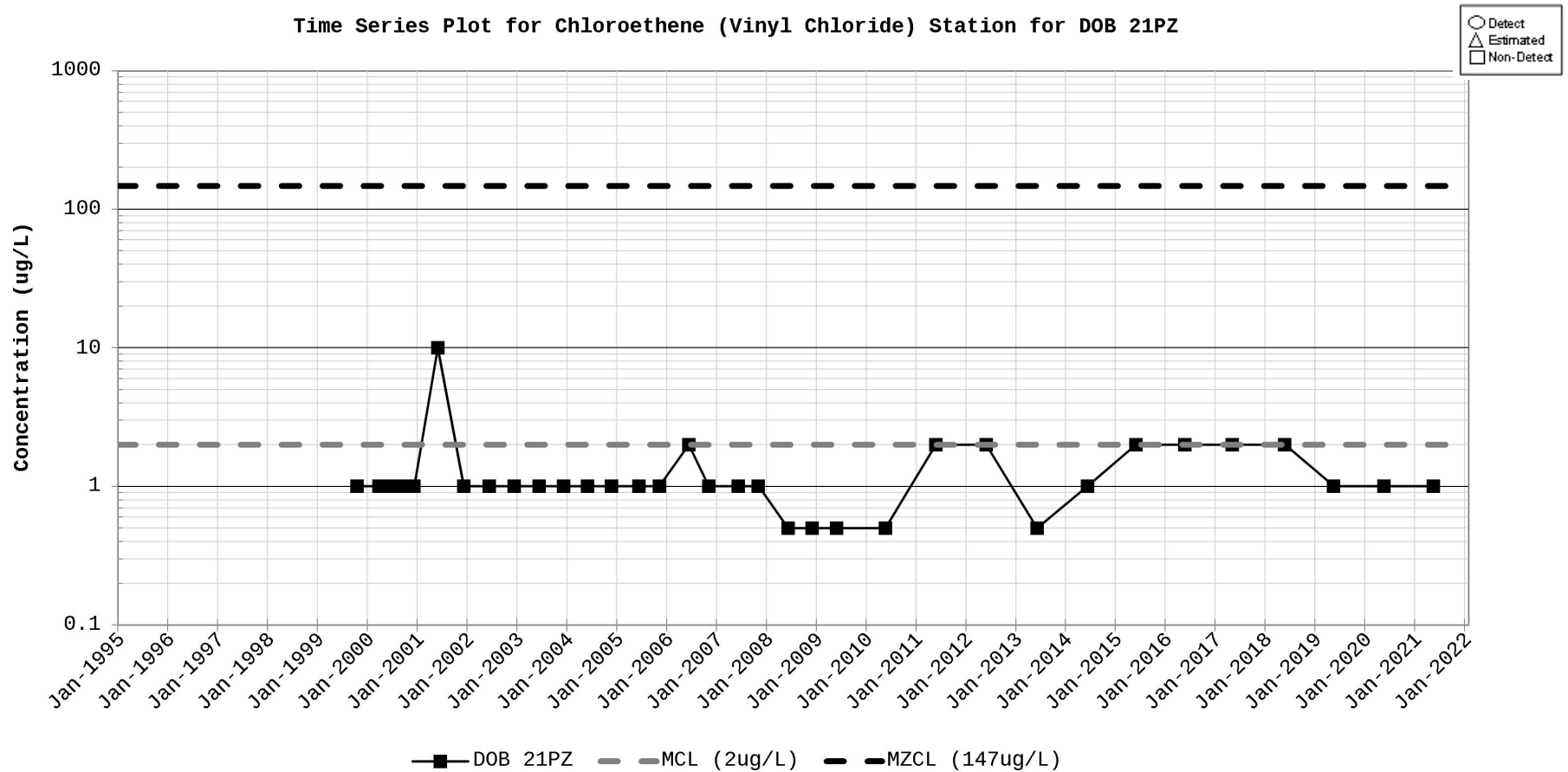
Figure D-17. Time Series Plot for Chloroethene (Vinyl chloride) Station for DOB 21PZ
