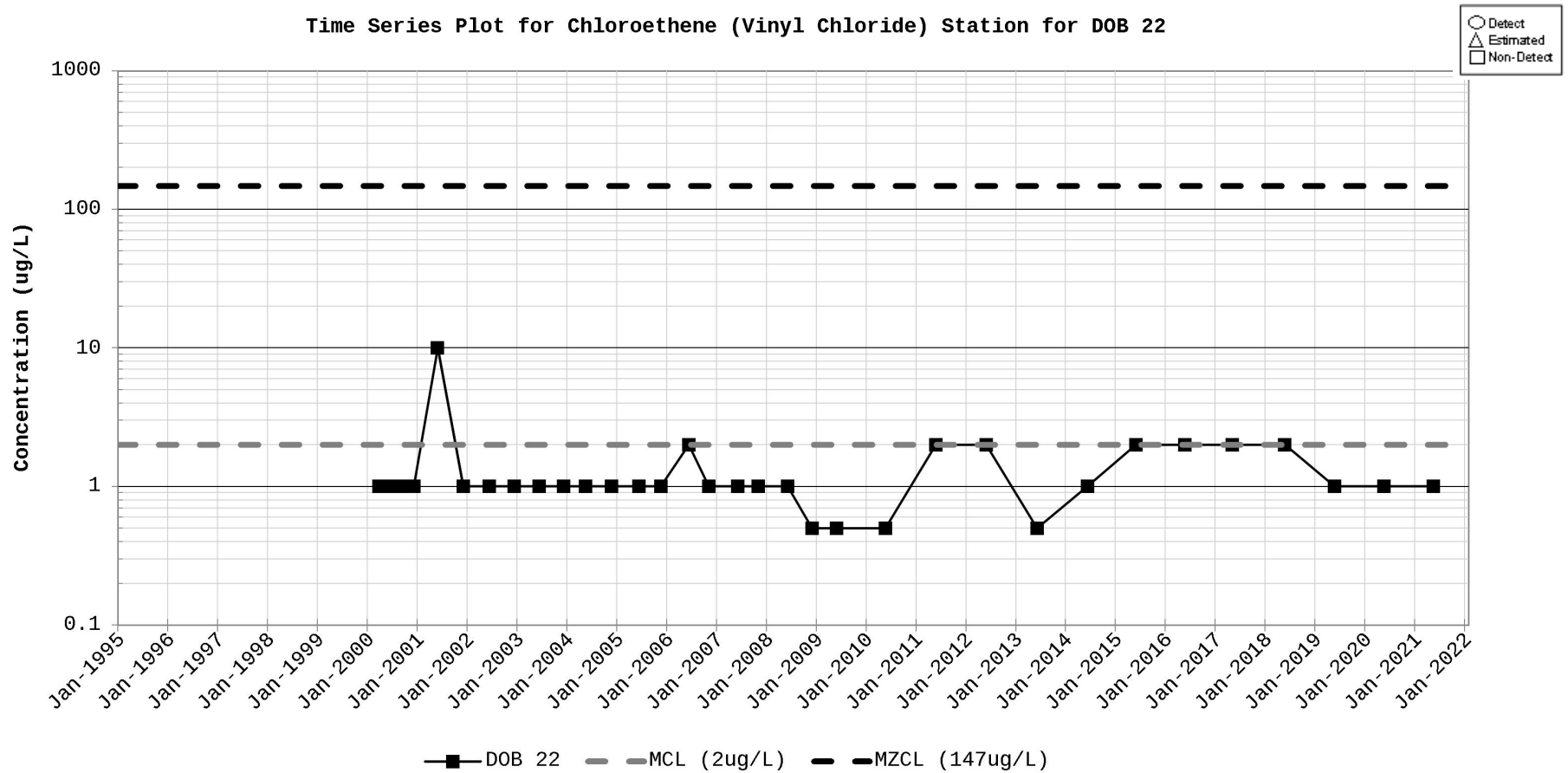
Figure D-19. Time Series Plot for Chloroethene (Vinyl chloride) Station for DOB 22
