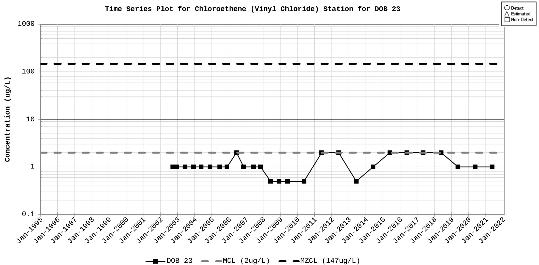
Figure D-20. Time Series Plot for Chloroethene (Vinyl chloride) Station for DOB 23
