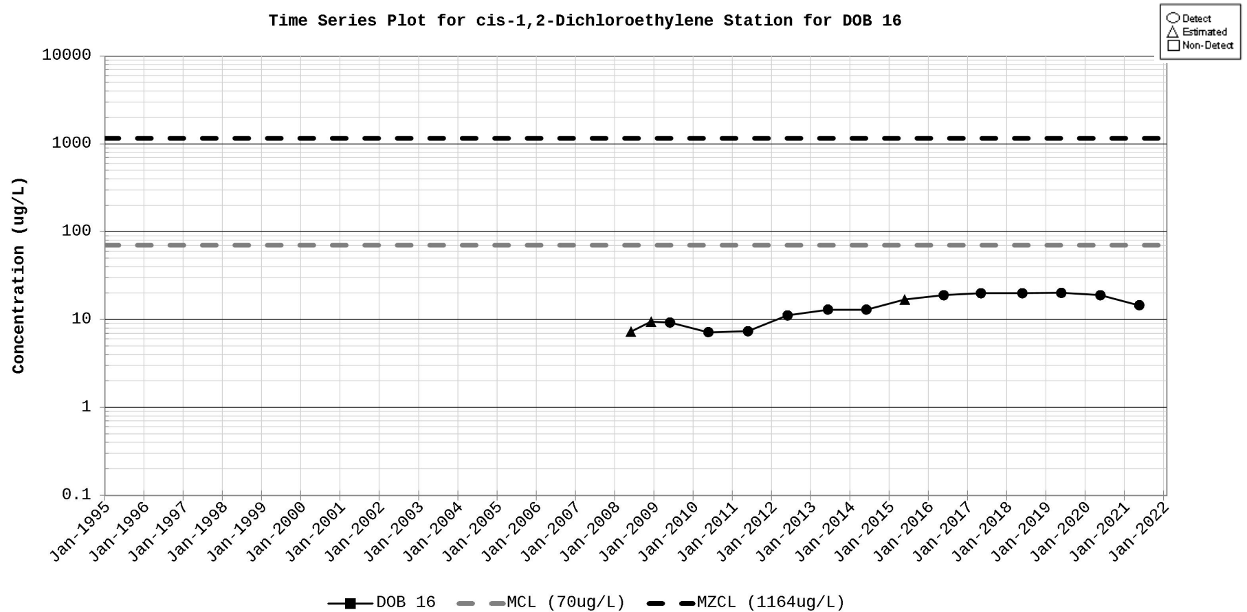
Figure D-33. Time Series Plot for cis-1,2-Dichloroethylene Station for DOB 16
