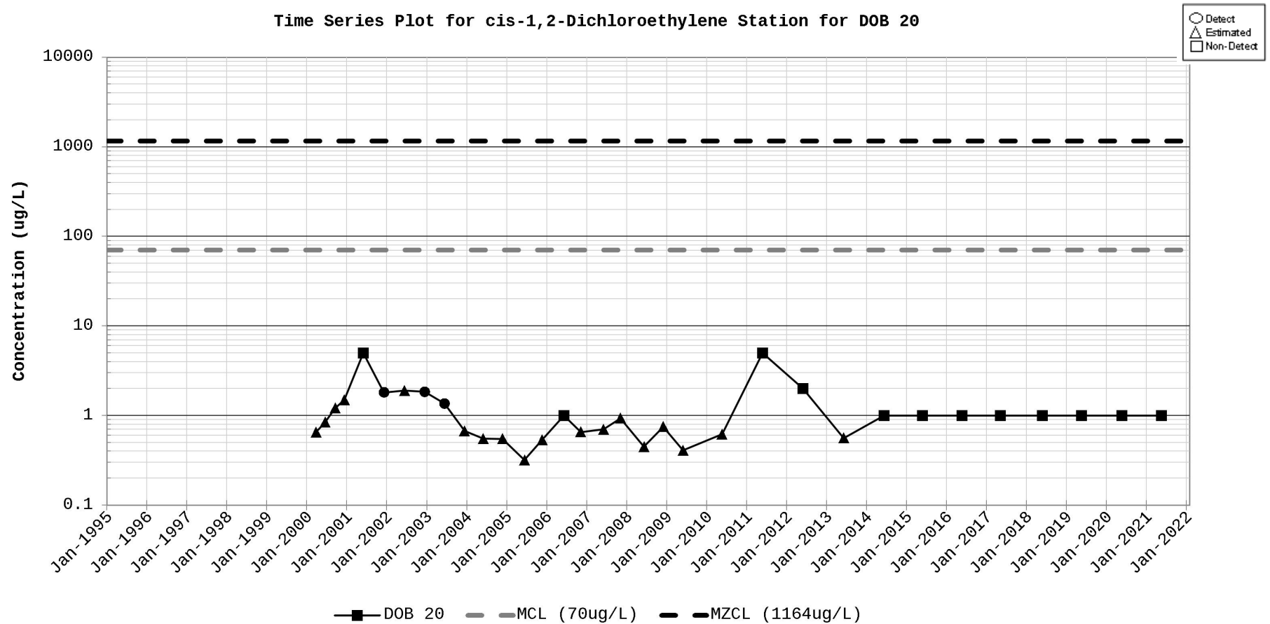
Figure D-37. Time Series Plot for cis-1,2-Dichloroethylene Station for DOB 20
