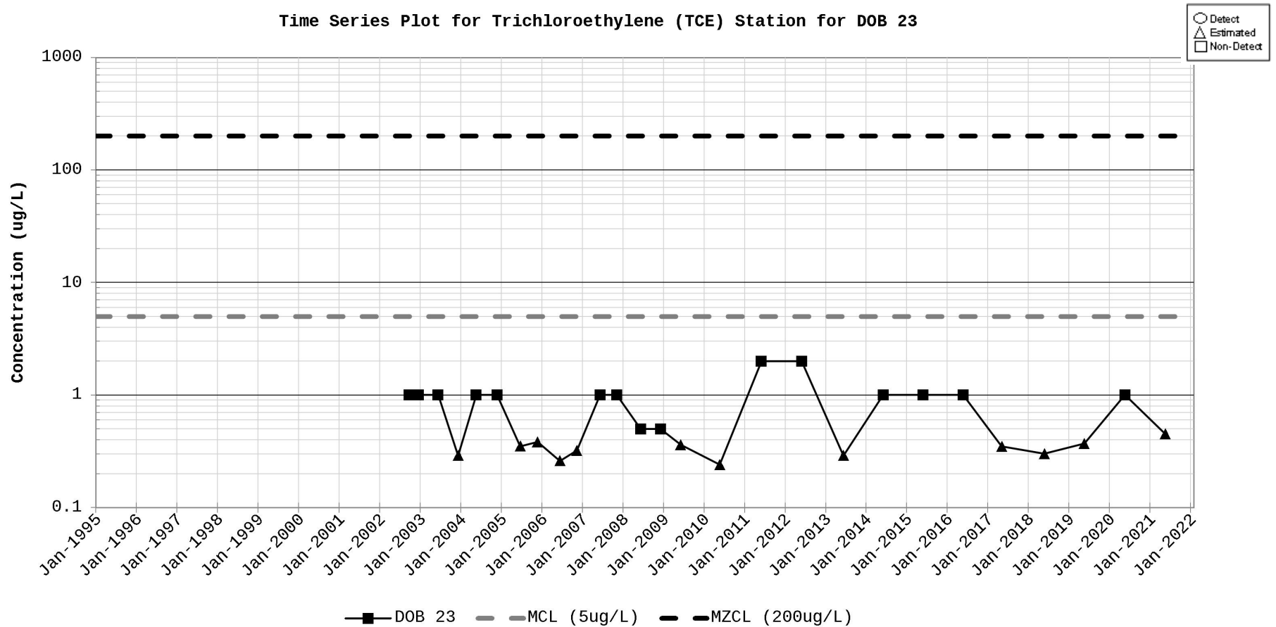
Figure D-89. Time Series Plot for Trichloroethylene (TCE) Station for DOB 23
