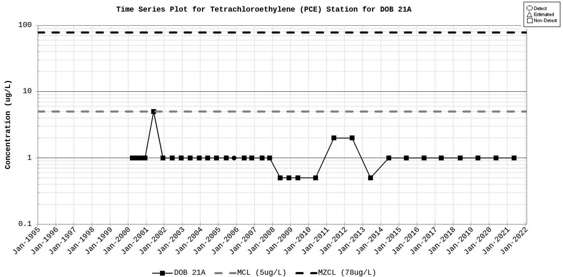
Figure D-61. Time Series Plot for Tetrachloroethylene (PCE) Station for DOB 21A
