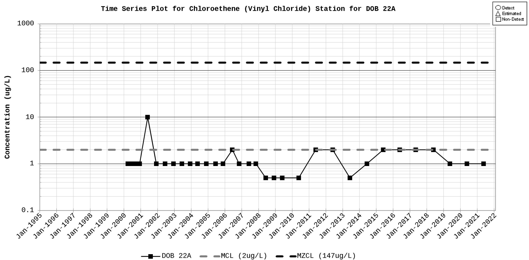
Figure D-18. Time Series Plot for Chloroethene (Vinyl chloride) Station for DOB 22A
