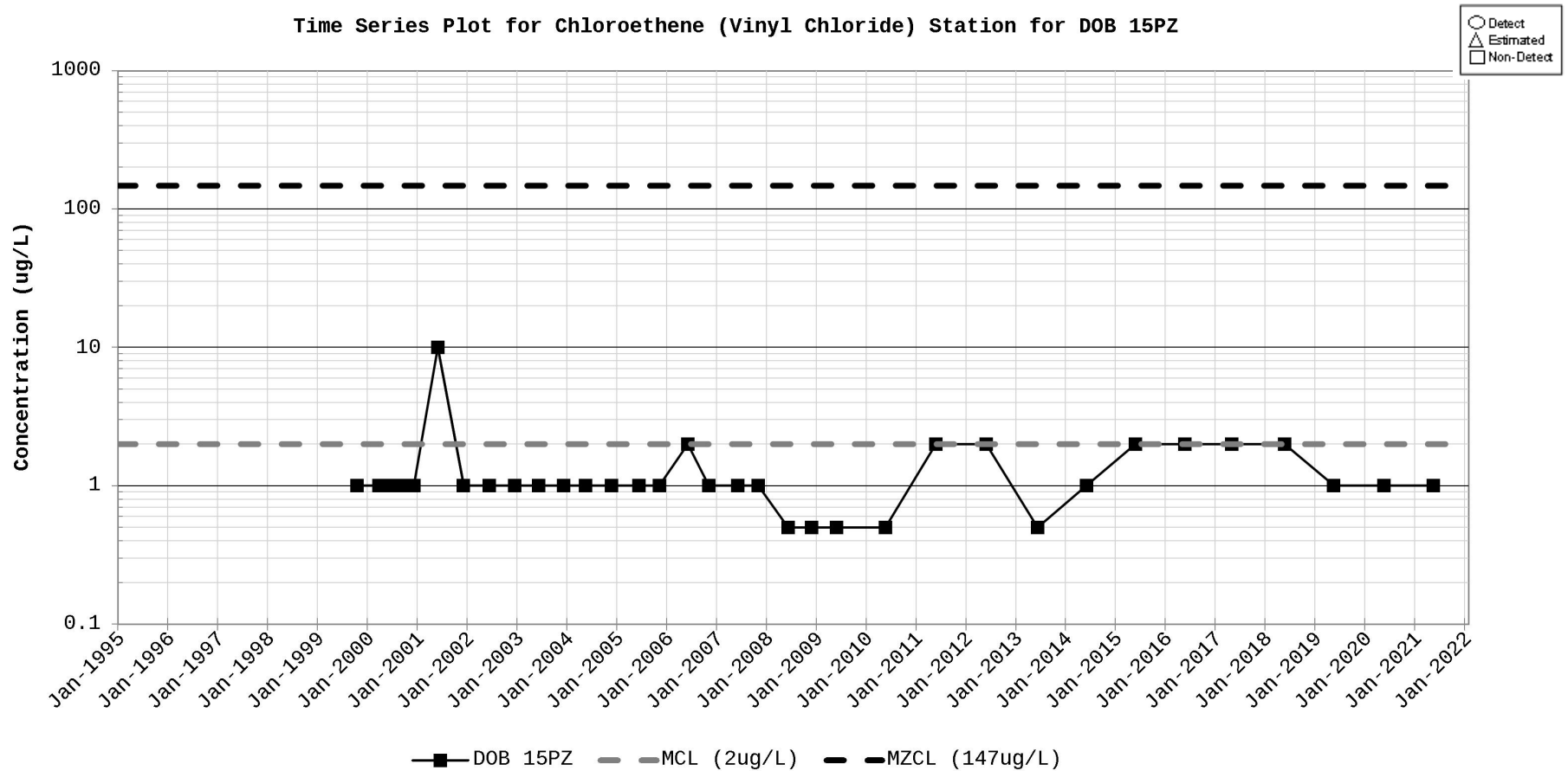
Figure D-8. Time Series Plot for Chloroethene (Vinyl chloride) Station for DOB 15PZ
