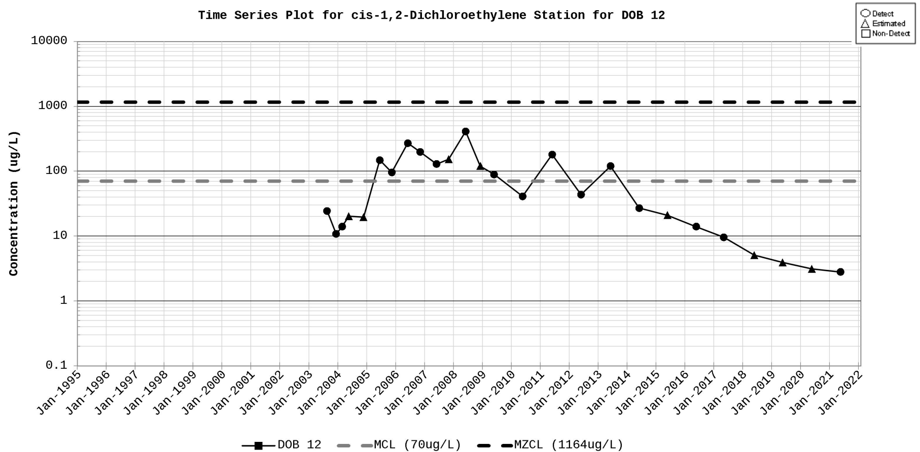
Figure D-26. Time Series Plot for cis-1,2-Dichloroethylene Station for DOB 12
