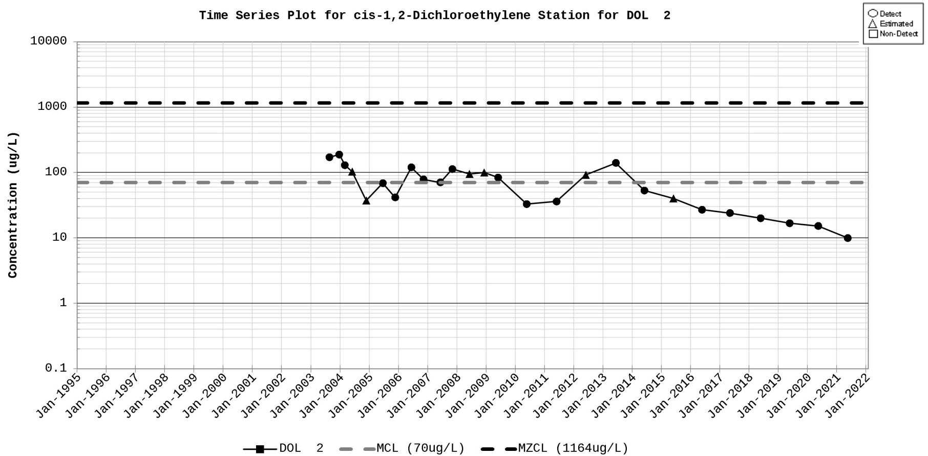
Figure D-46. Time Series Plot for cis-1,2-Dichloroethylene Station for DOL 2
