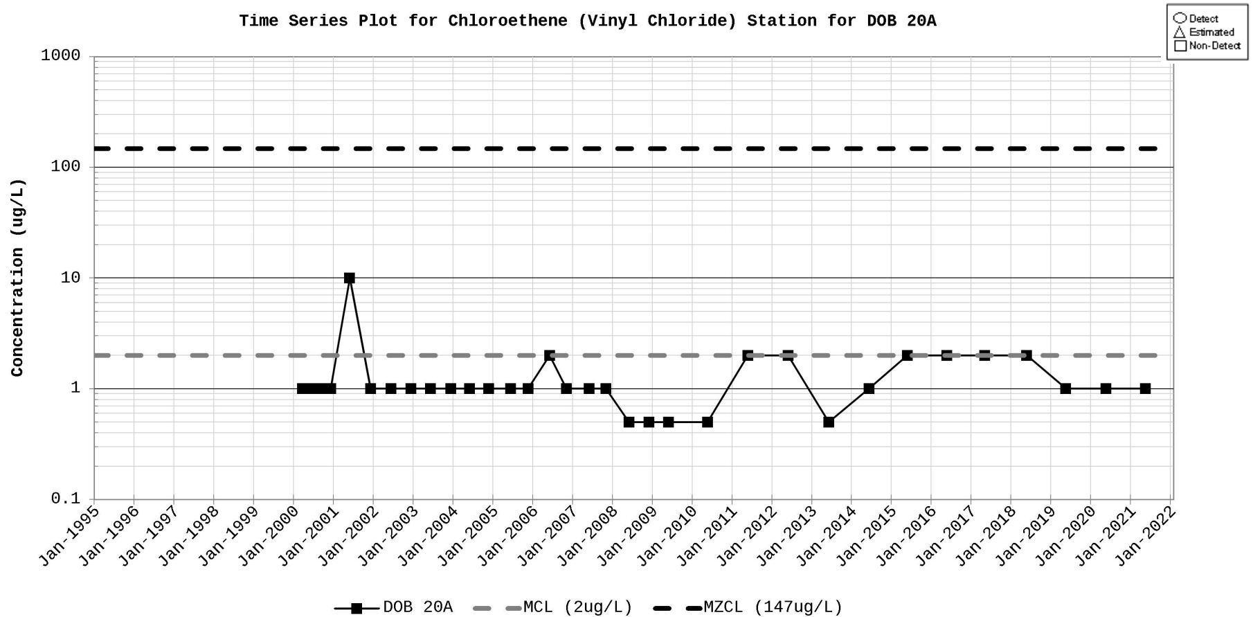
Figure D-13. Time Series Plot for Chloroethene (Vinyl chloride) Station for DOB 20A
