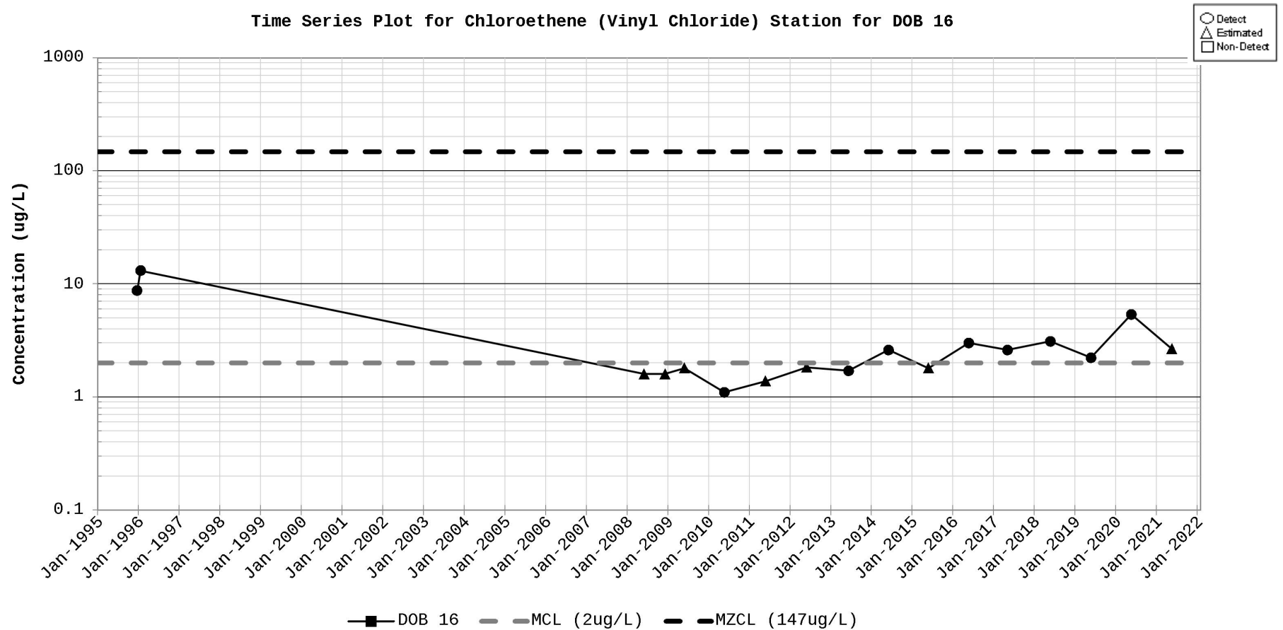
Figure D-10. Time Series Plot for Chloroethene (Vinyl chloride) Station for DOB 16
