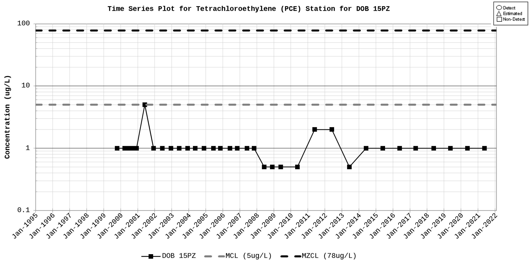
Figure D-54. Time Series Plot for Tetrachloroethylene (PCE) Station for DOB 15PZ
