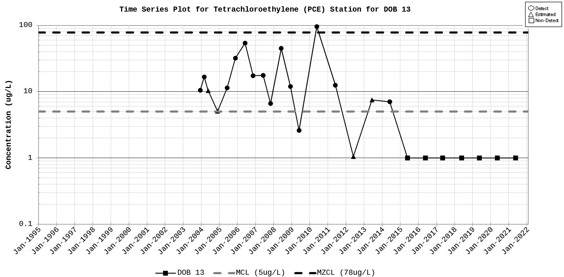
Figure D-50. Time Series Plot for Tetrachloroethylene (PCE) Station for DOB 13
