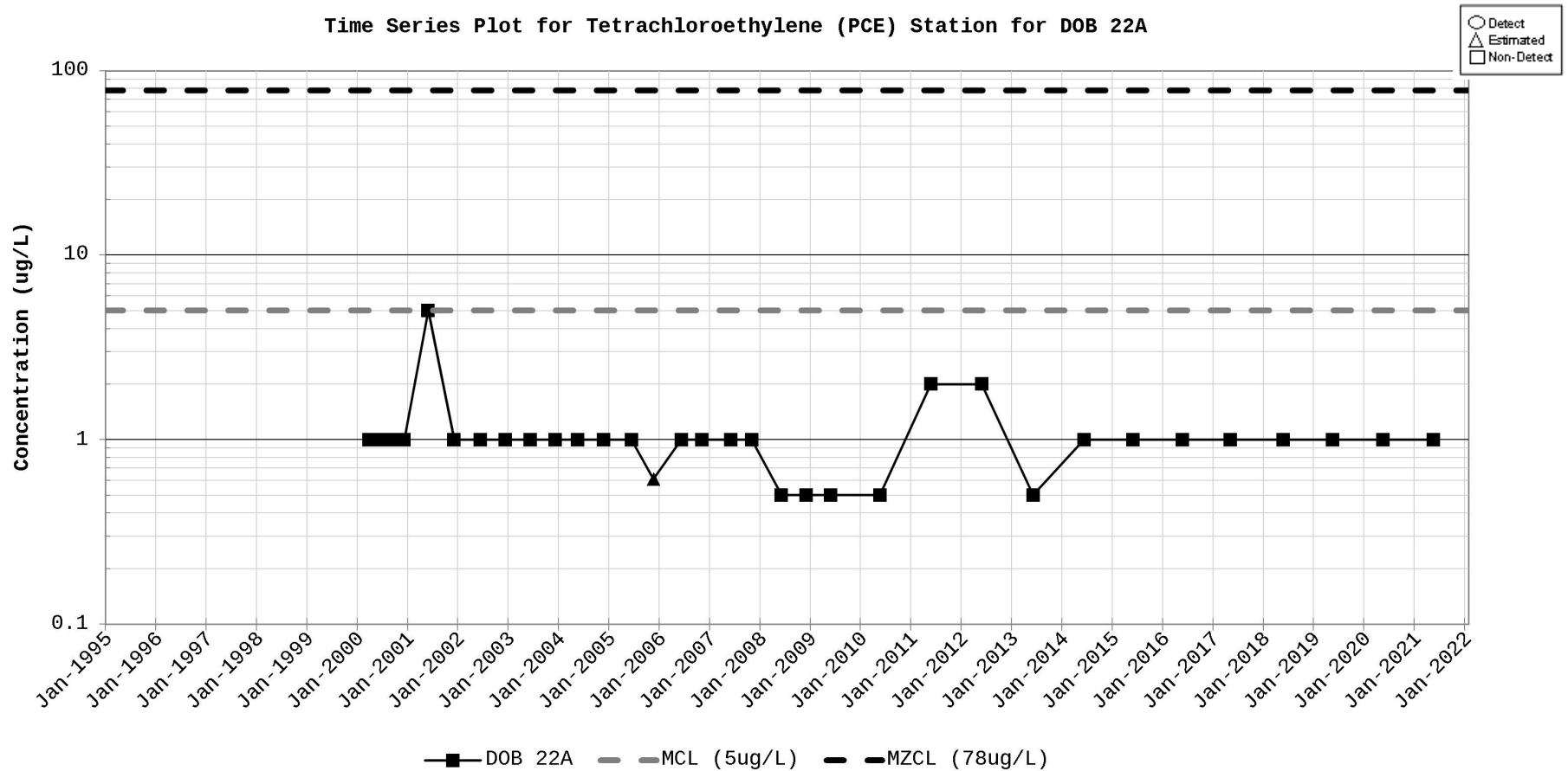
Figure D-64. Time Series Plot for Tetrachloroethylene (PCE) Station for DOB 22
