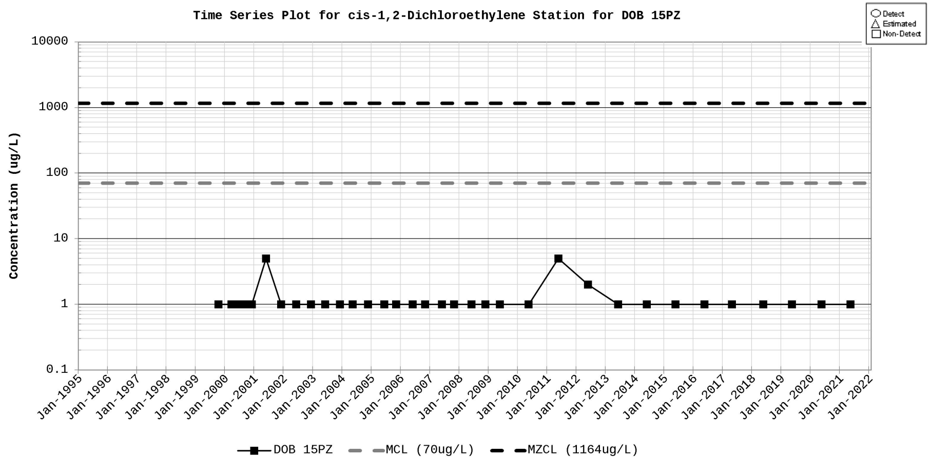
Figure D-31. Time Series Plot for cis-1,2-Dichloroethylene Station for DOB 15PZ
