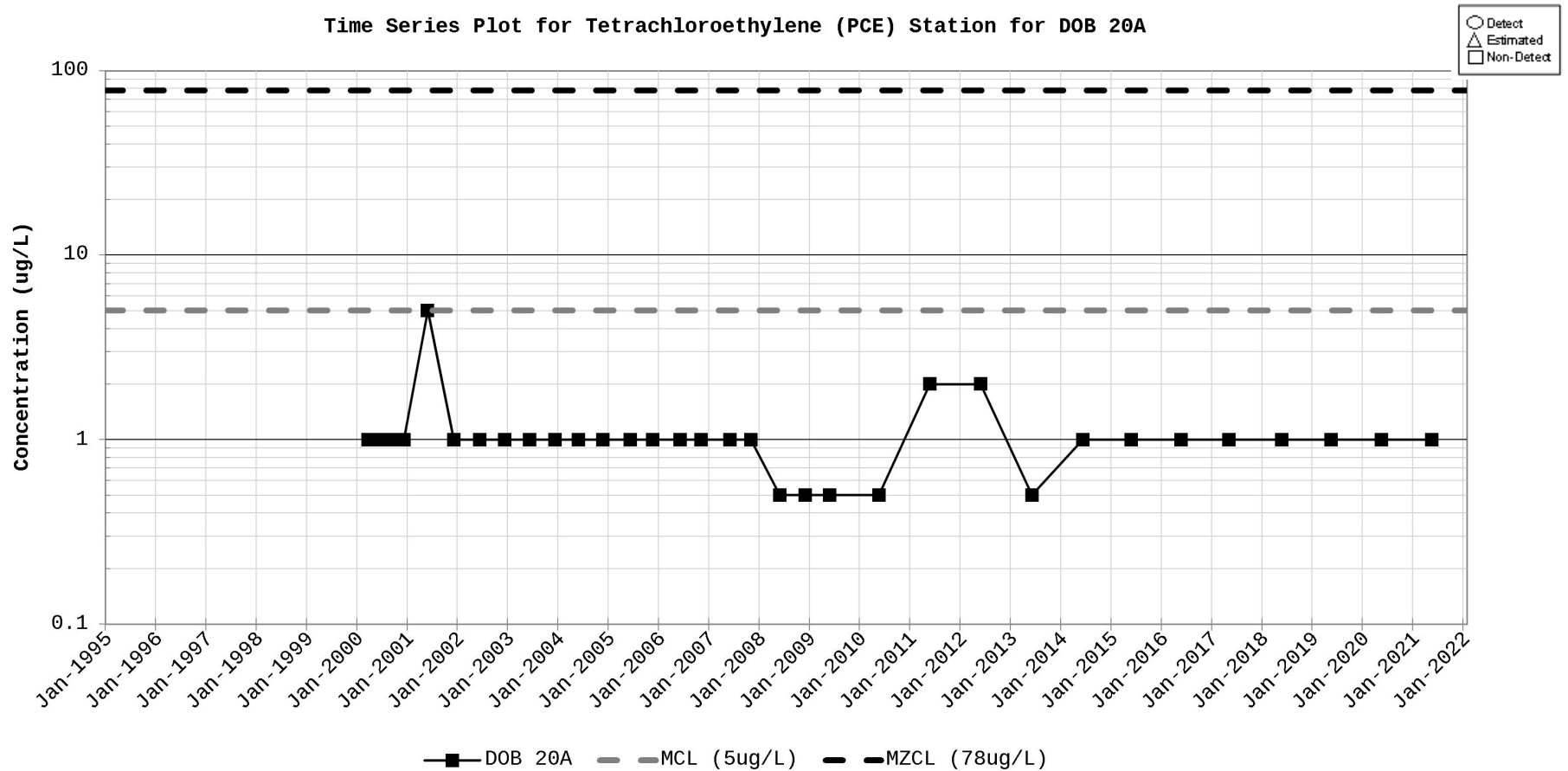
Figure D-59. Time Series Plot for Tetrachloroethylene (PCE) Station for DOB 20A
