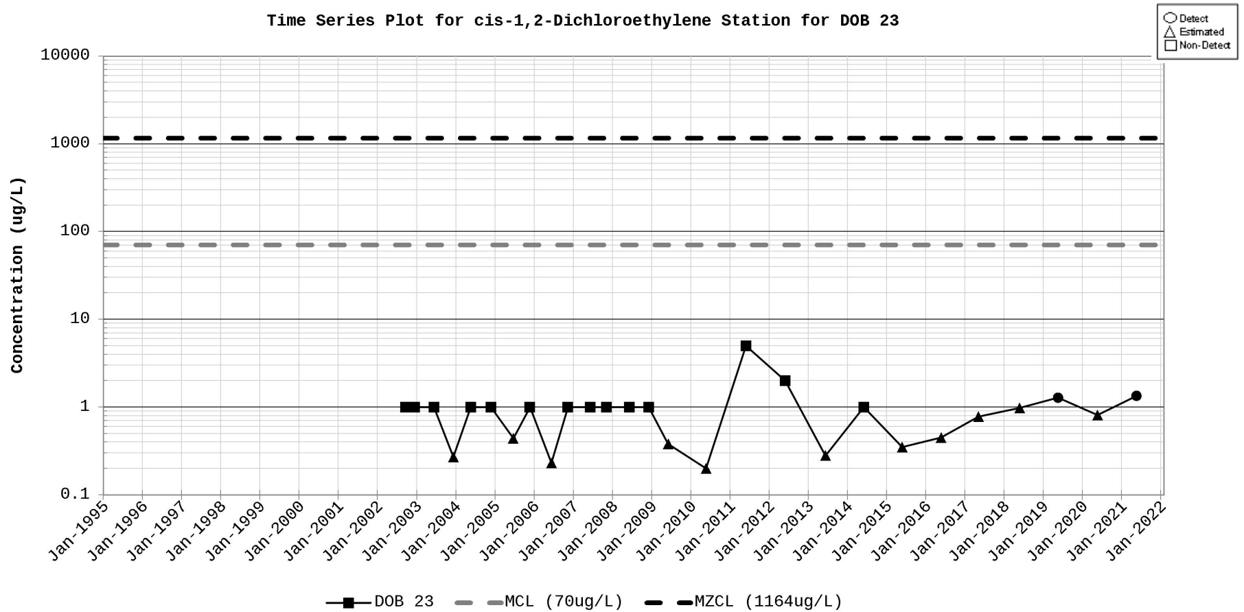
Figure D-43. Time Series Plot for cis-1,2-Dichloroethylene Station for DOB 23
