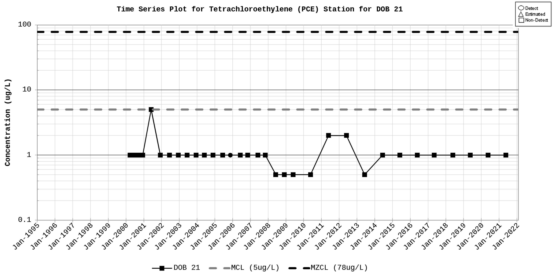
Figure D-62. Time Series Plot for Tetrachloroethylene (PCE) Station for DOB 21
