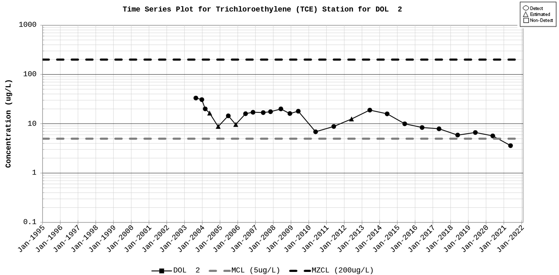
Figure D-92. Time Series Plot for Trichloroethylene (TCE) Station for DOL 2
