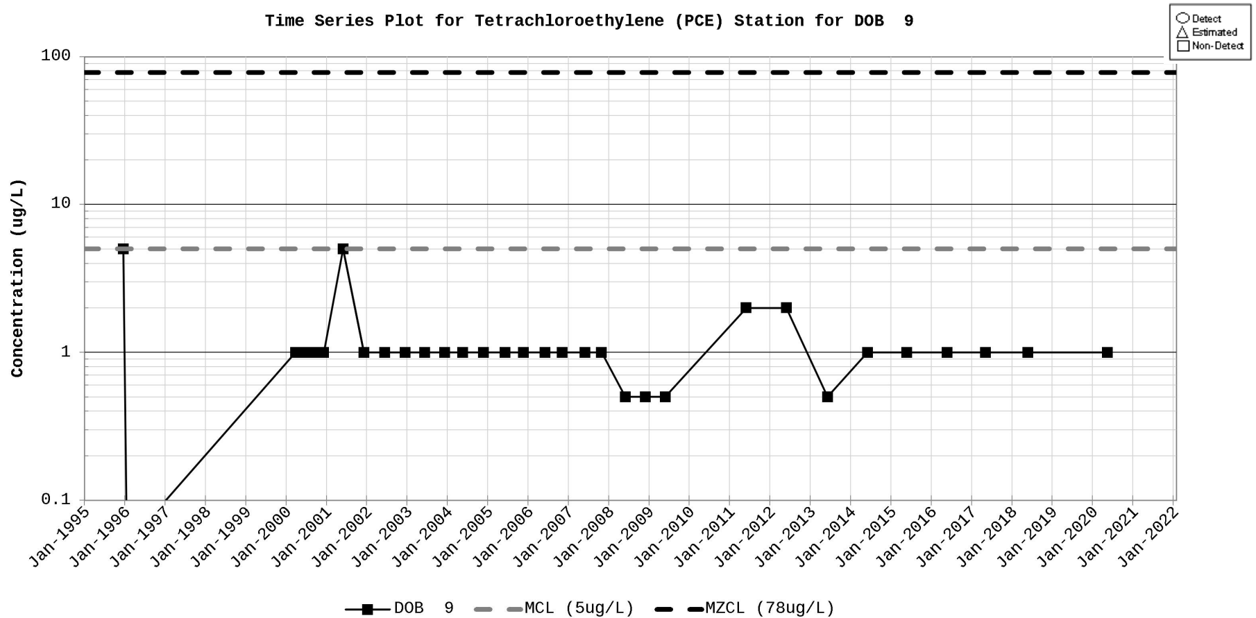
Figure D-47. Time Series Plot for Tetrachloroethylene (PCE) Station for DOB 9
