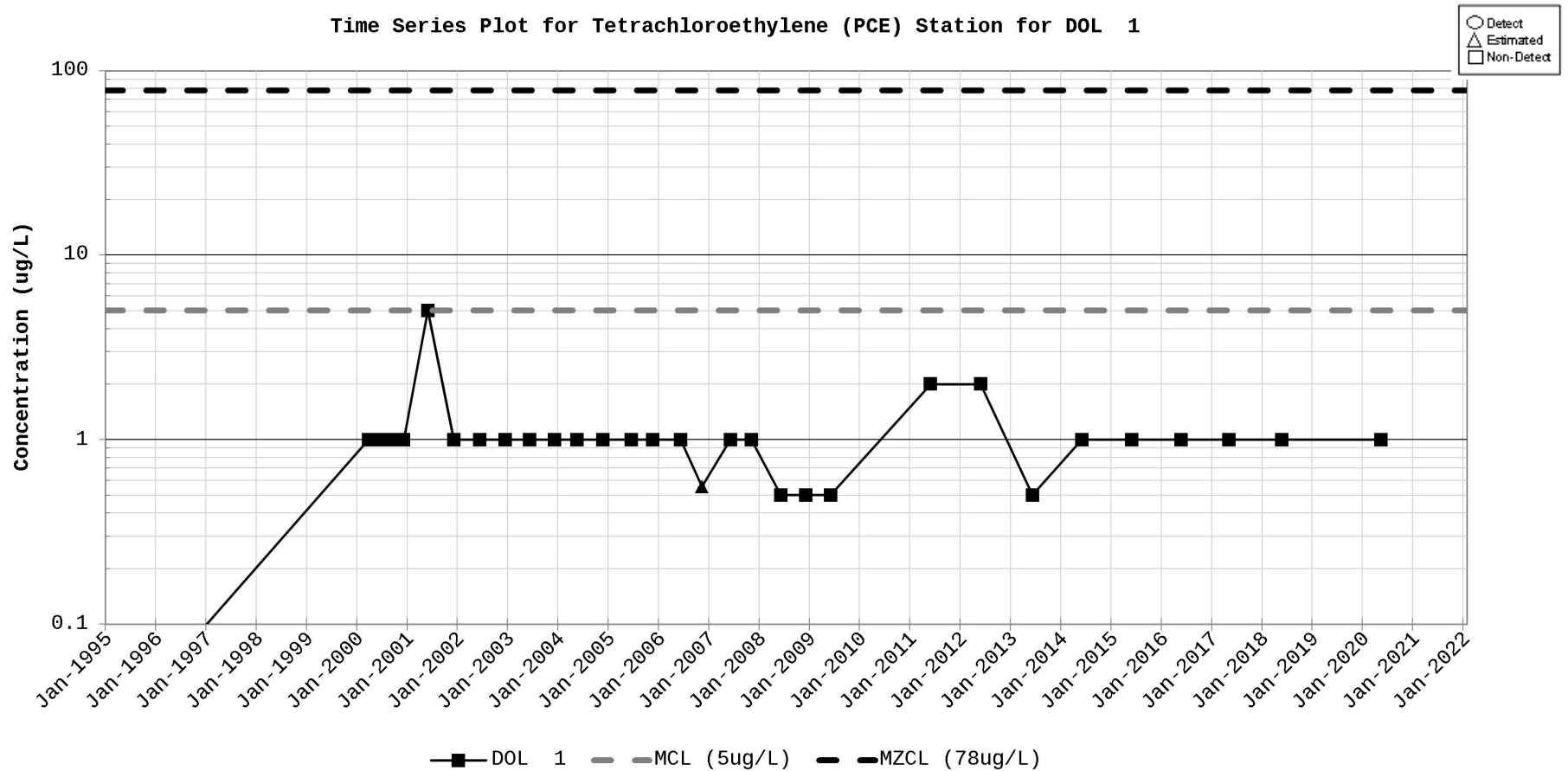
Figure D-68. Time Series Plot for Tetrachloroethylene (PCE) Station for DOL 1
