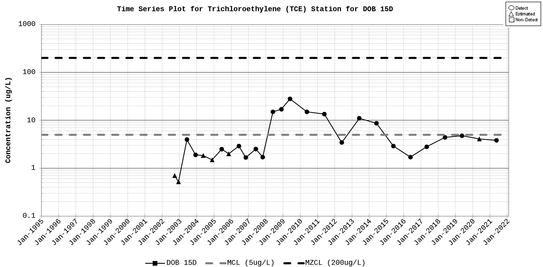
Figure D-78. Time Series Plot for Trichloroethylene (TCE) Station for DOB 15D
