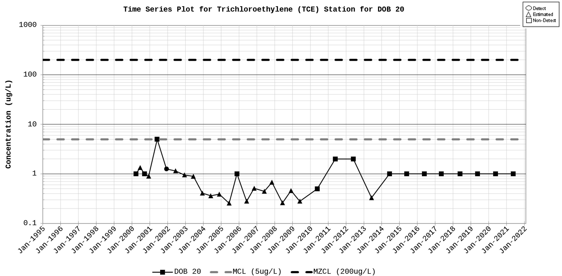
Figure D-83 Time Series Plot for Trichloroethylene (TCE) Station for DOB 20
