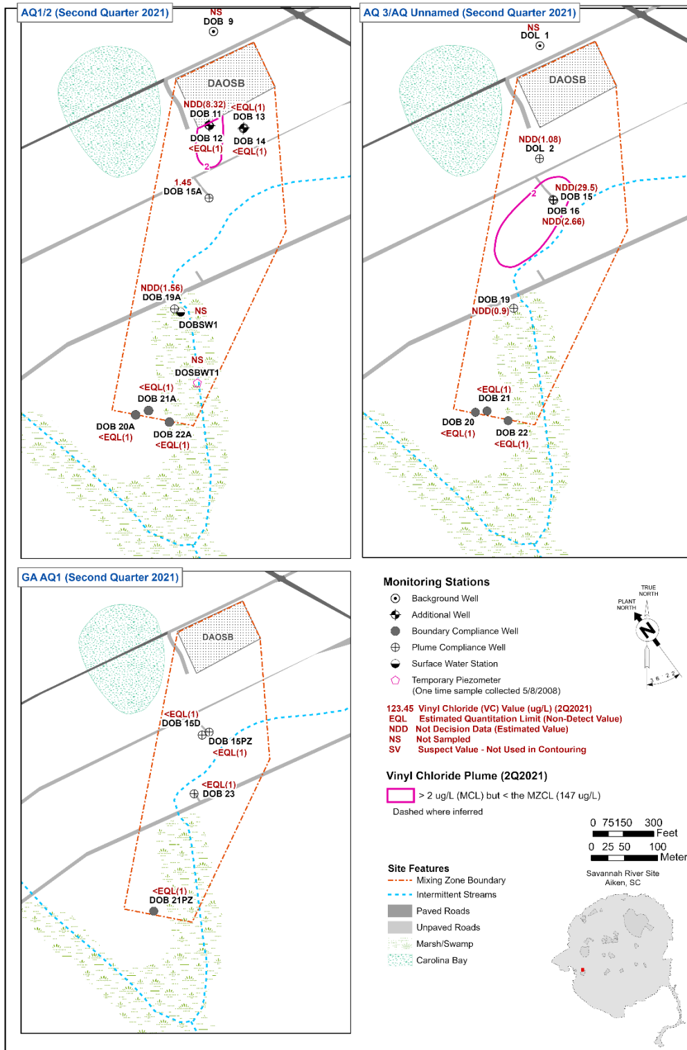
Figure B-9. DOSB Vinyl Chloride in AQ1/2, 3 and GA AQ1, 2021
