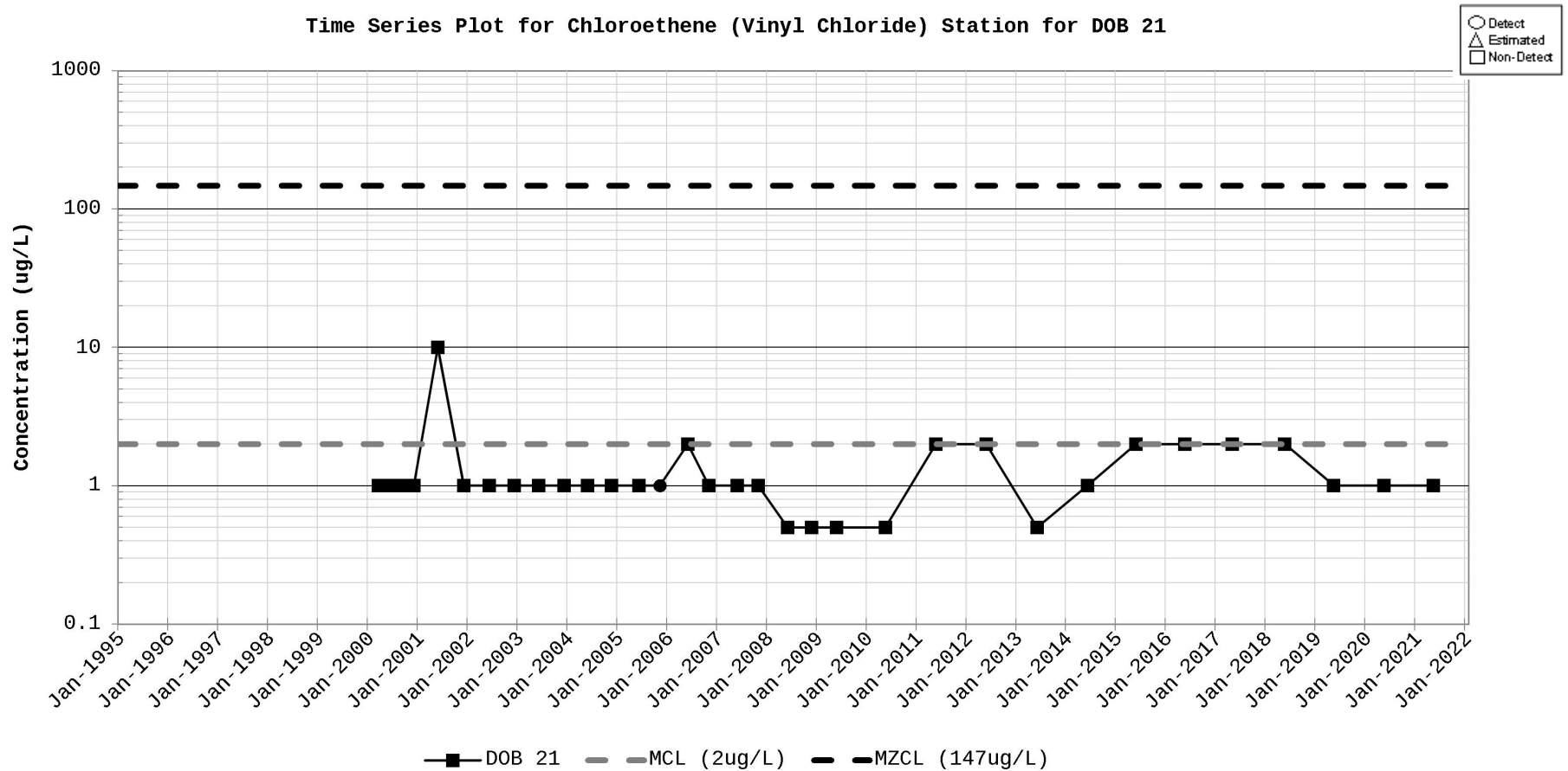
Figure D-16. Time Series Plot for Chloroethene (Vinyl chloride) Station for DOB 21
