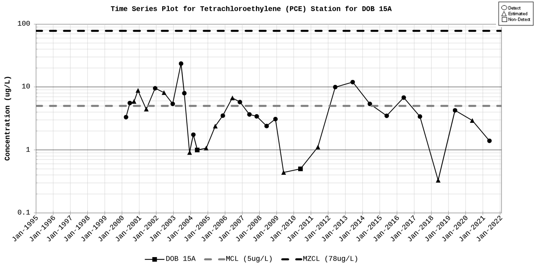
Figure D-53. Time Series Plot for Tetrachloroethylene (PCE) Station for DOB 15A
