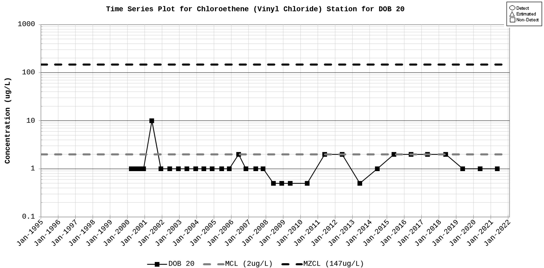
Figure D-14. Time Series Plot for Chloroethene (Vinyl chloride) Station for DOB 20
