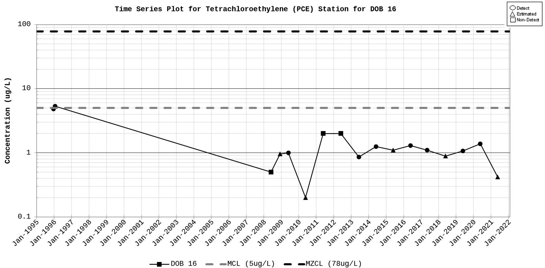
Figure D-56. Time Series Plot for Tetrachloroethylene (PCE) Station for DOB 16
