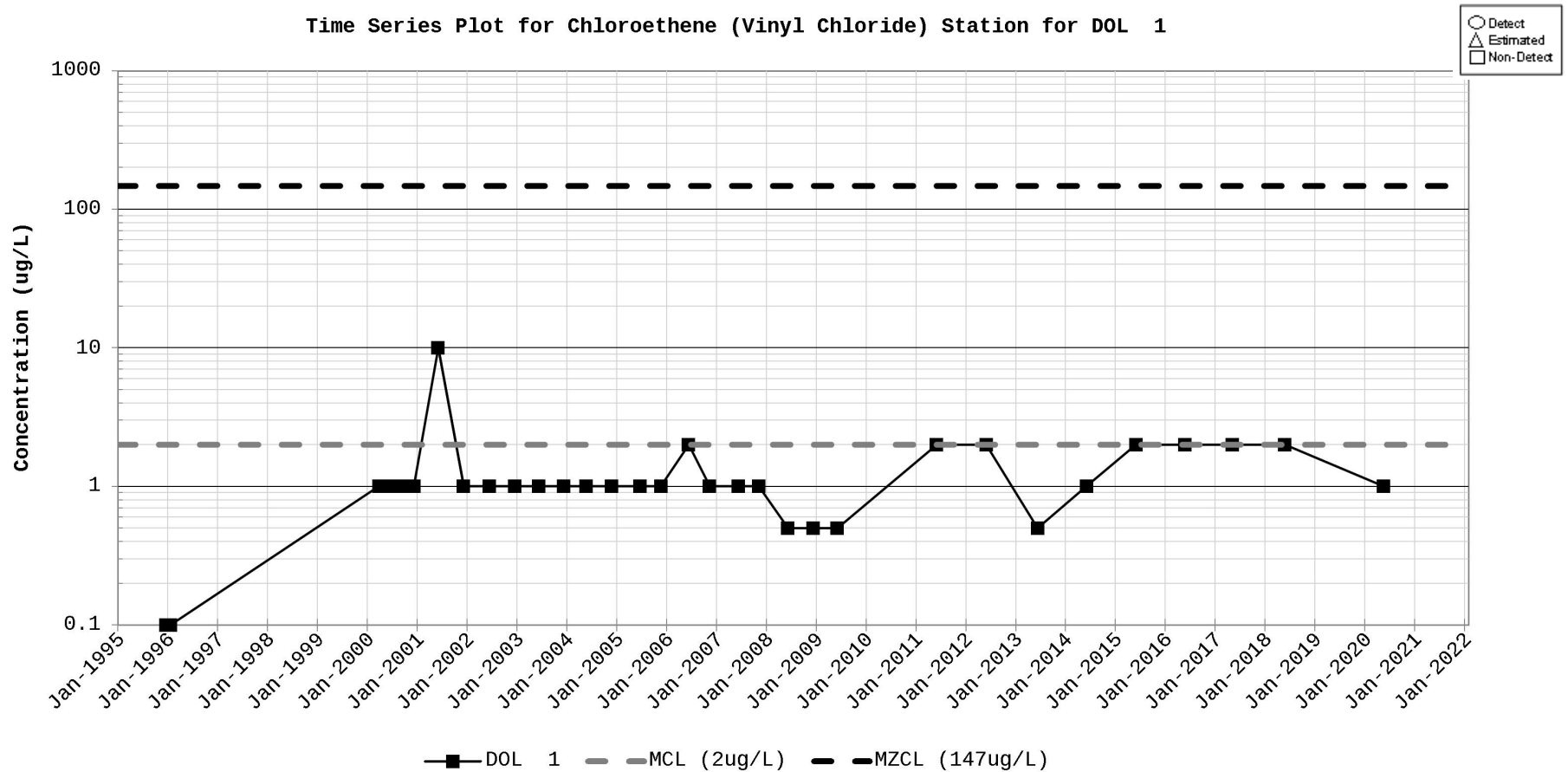
Figure D-22. Time Series Plot for Chloroethene (Vinyl chloride) Station for DOL 1
