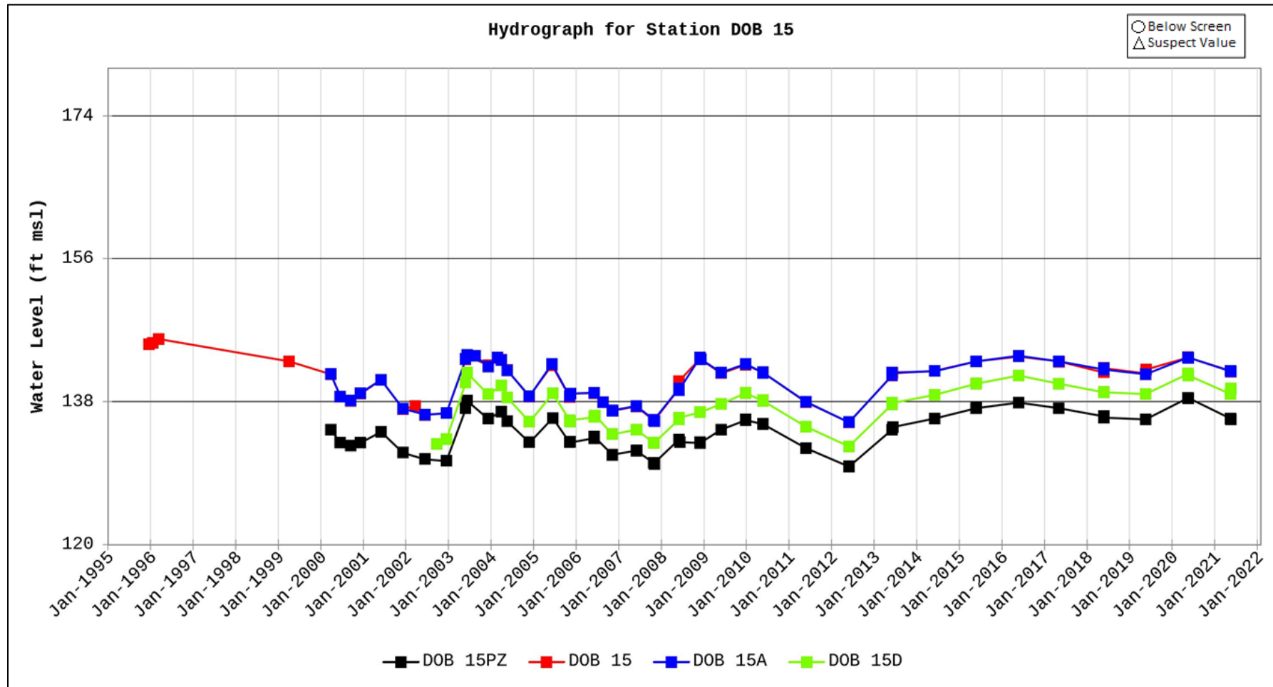
Figure C-6. Hydrograph for Station DOB15
