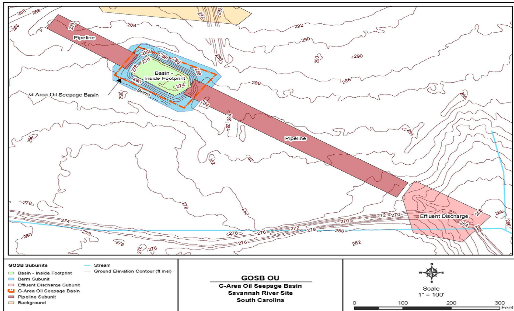
Figure 2. Layout of the GOSB OU
