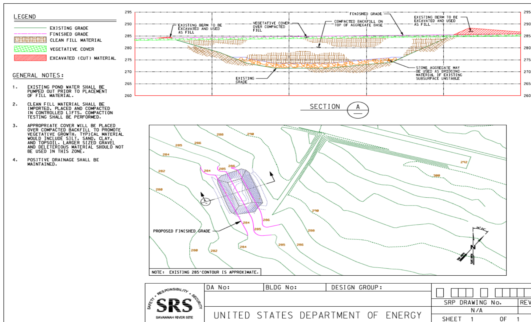
Figure 10. Basin Cross-Section – Alternative #4
